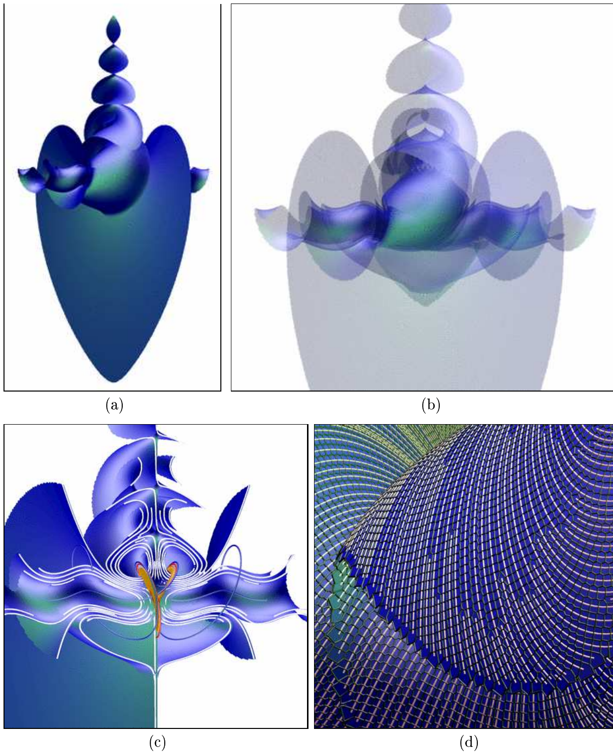
Figure 9: The Lorenz manifold computed with the method of Henderson up to a total trajectory arclength of 240. Panel (a) shows a view of the entire manifold, panel (b) a transparent enlargement near the main scroll, panel (c) shows the part of the manifold for x < 0 together with the Lorenz attractor and the one-dimensional stable manifolds of the two other equilibria, and panel (d) gives an impression of the computed mesh.
