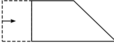
Figure 3: Moving an edge parallel to itself.
