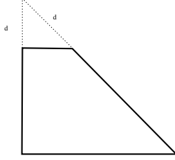
Figure 1: A corner chopping of size \varepsilon .
