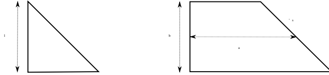
Figure 2: The Delzant triangle \Delta_\lambda and the Hirzebruch trapezoid H_{a,b,k} .
