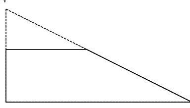
Figure 5: The vertex v is not smooth.
