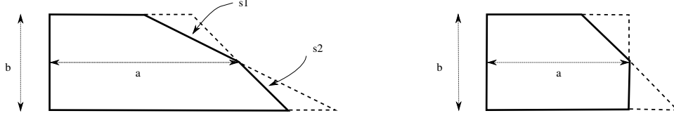
Figure 4: H'_{a,b,k} for k \geq 1 and H'_{a,b,0} .
