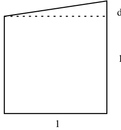
Figure 6: The polygon Q_\delta .
