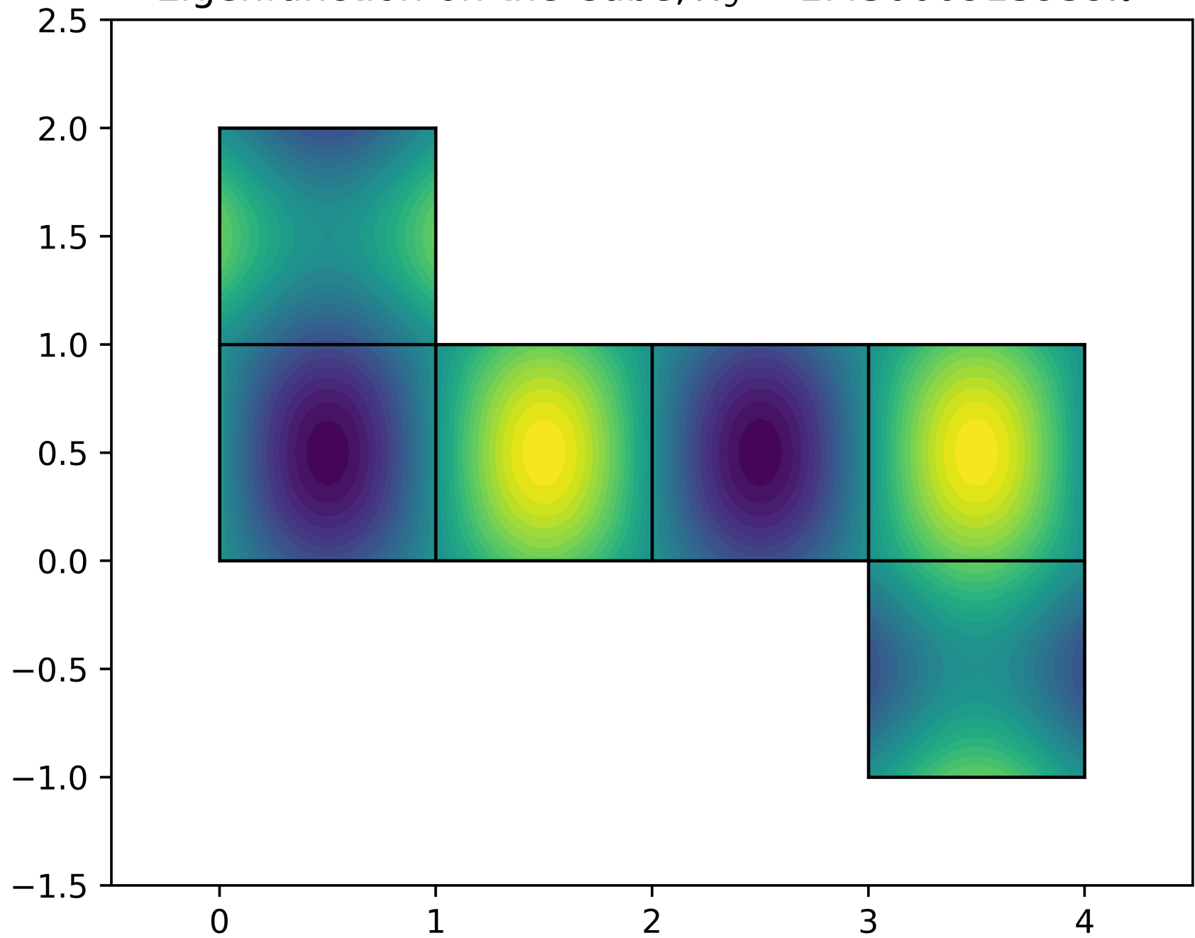
Eigenfunction on the Cube, \lambda_9 = 1.43000913939\pi^2
