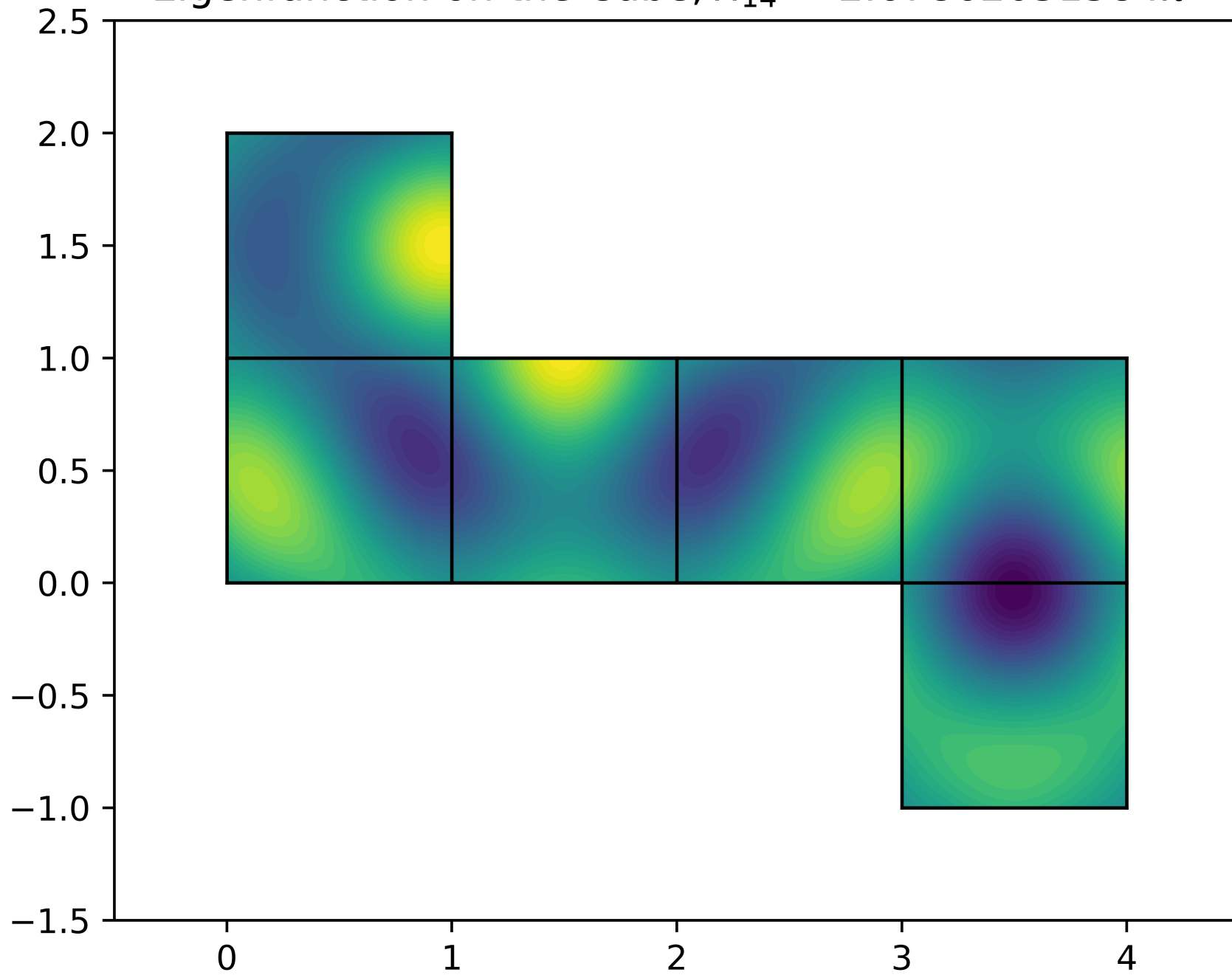
Eigenfunction on the Cube, \lambda_{14} = 2.67862031584\pi^2
