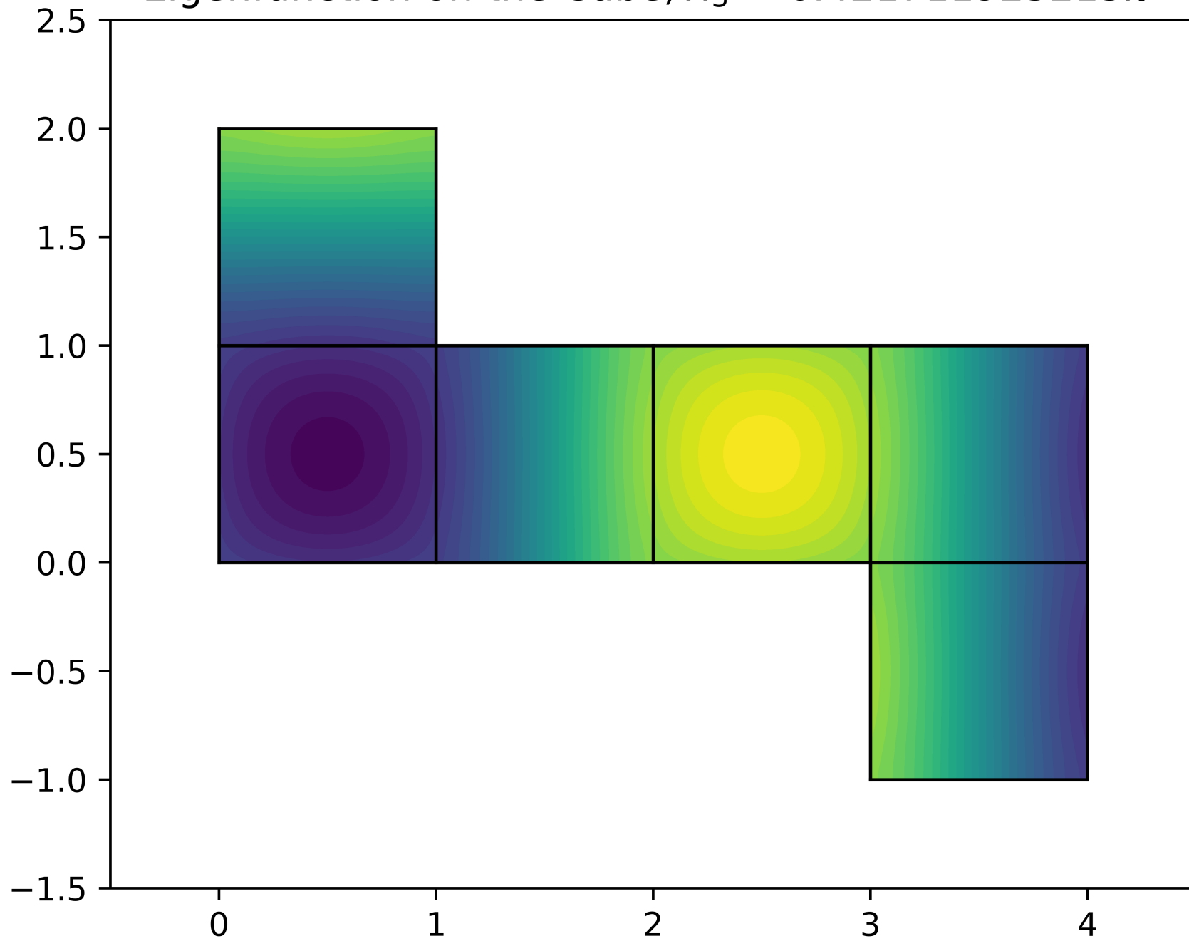
Eigenfunction on the Cube, \lambda_3 = 0.421711923215\pi^2
