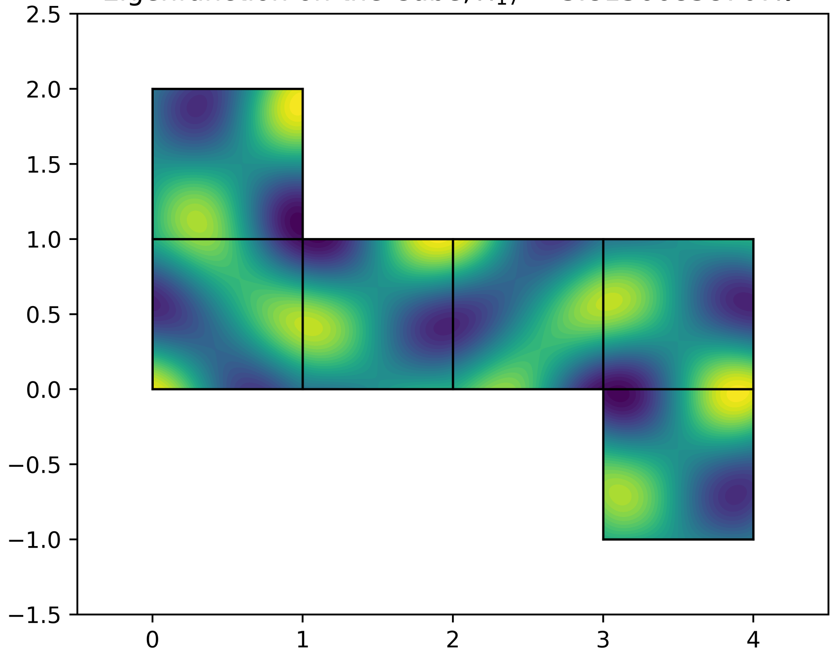
Eigenfunction on the Cube, \lambda_{17} = 3.81366838707\pi^2
