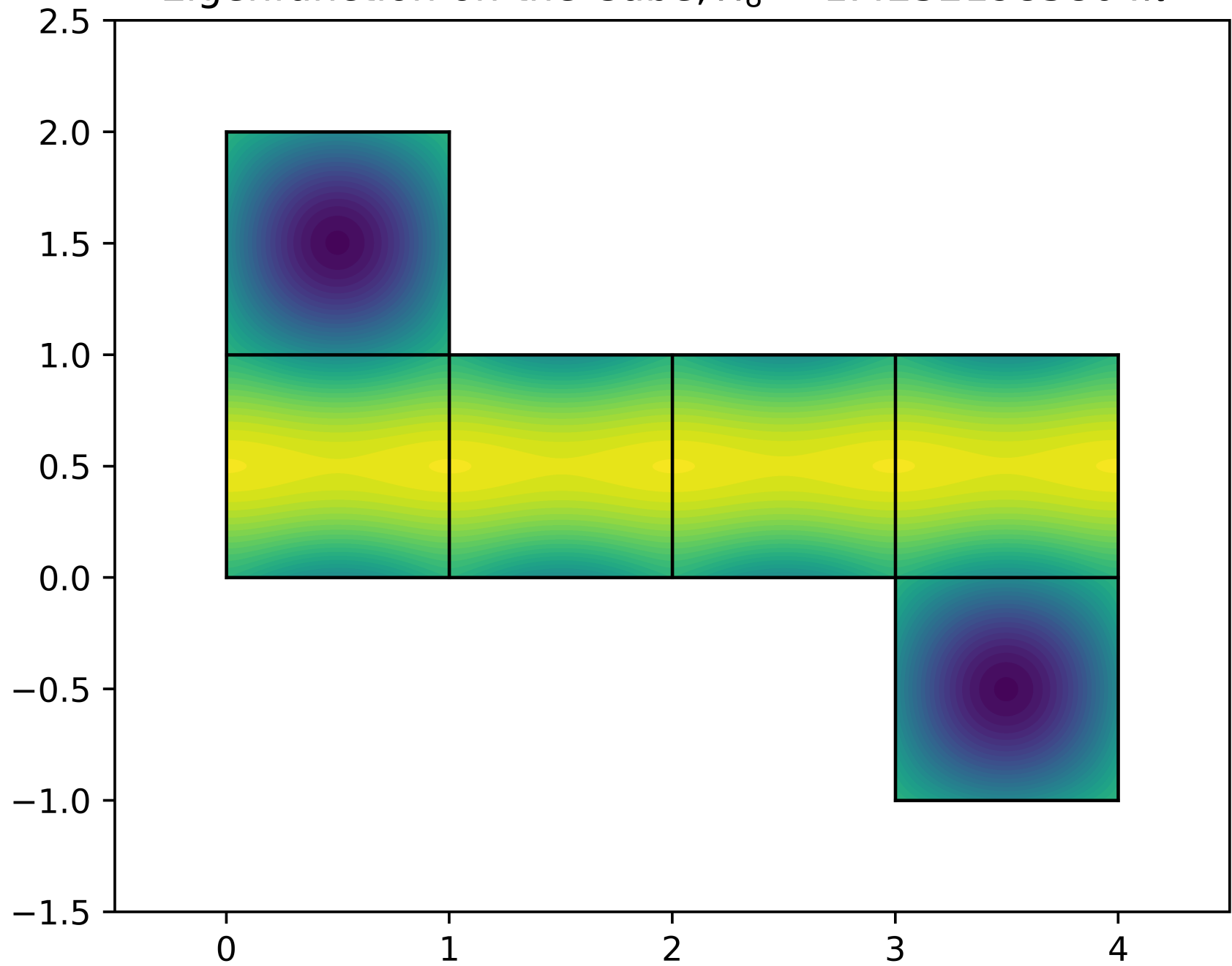
Eigenfunction on the Cube, \lambda_8 = 1.42521985804\pi^2
