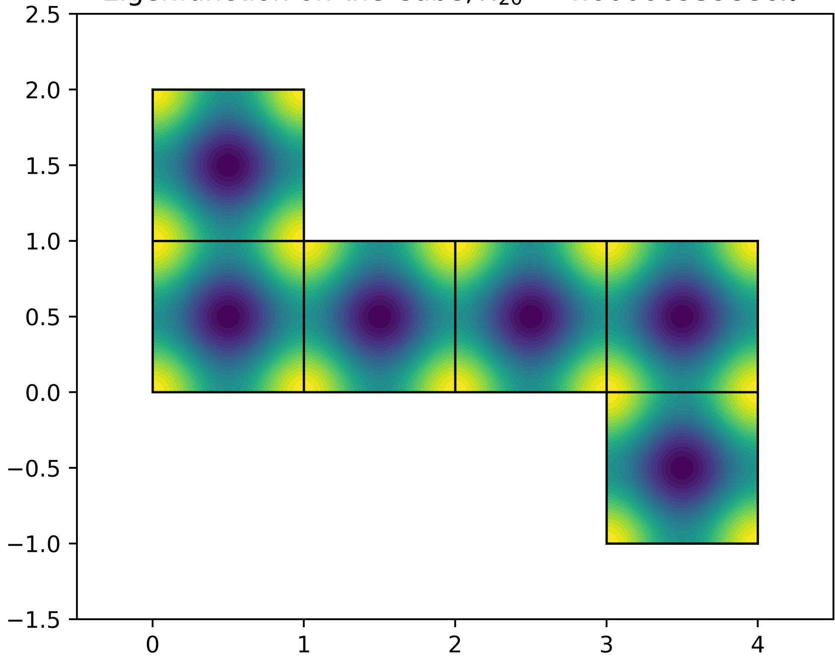
Eigenfunction on the Cube, \lambda_{20} = 4.00066939886\pi^2
