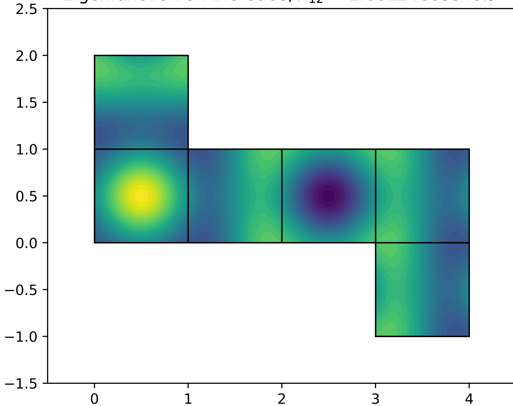
Eigenfunction on the Cube, \lambda_{12} = 2.60124605349\pi^2
