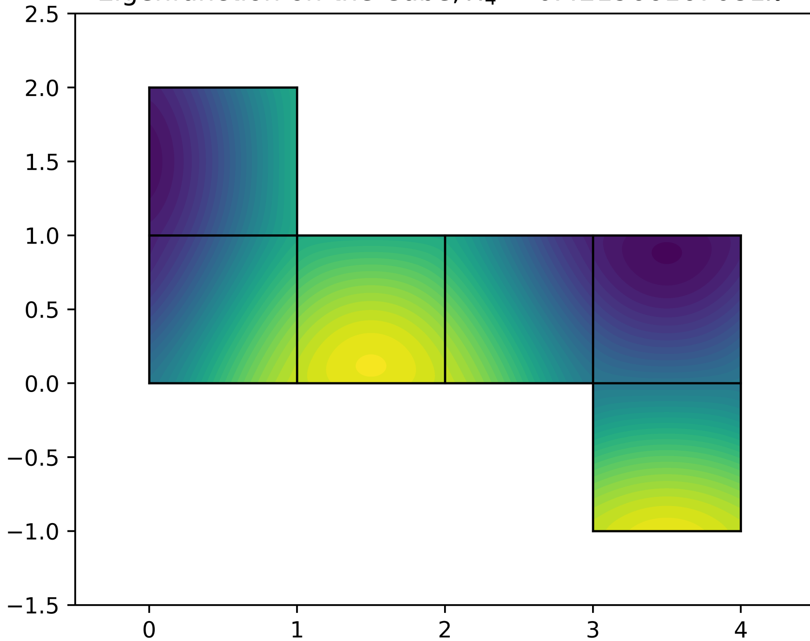
Eigenfunction on the Cube, \lambda_4 = 0.421966167081\pi^2
