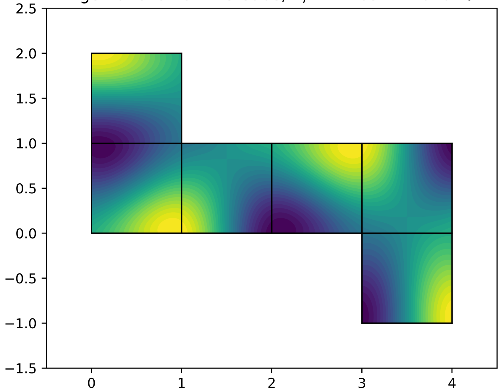
Eigenfunction on the Cube, \lambda_7 = 1.16512140407\pi^2
