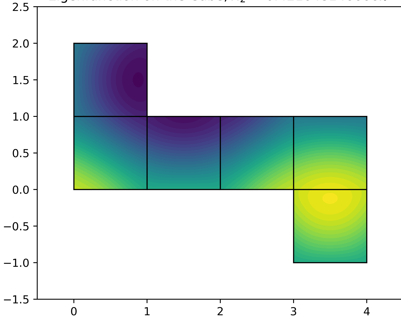
Eigenfunction on the Cube, \lambda_2 = 0.421048146666\pi^2
