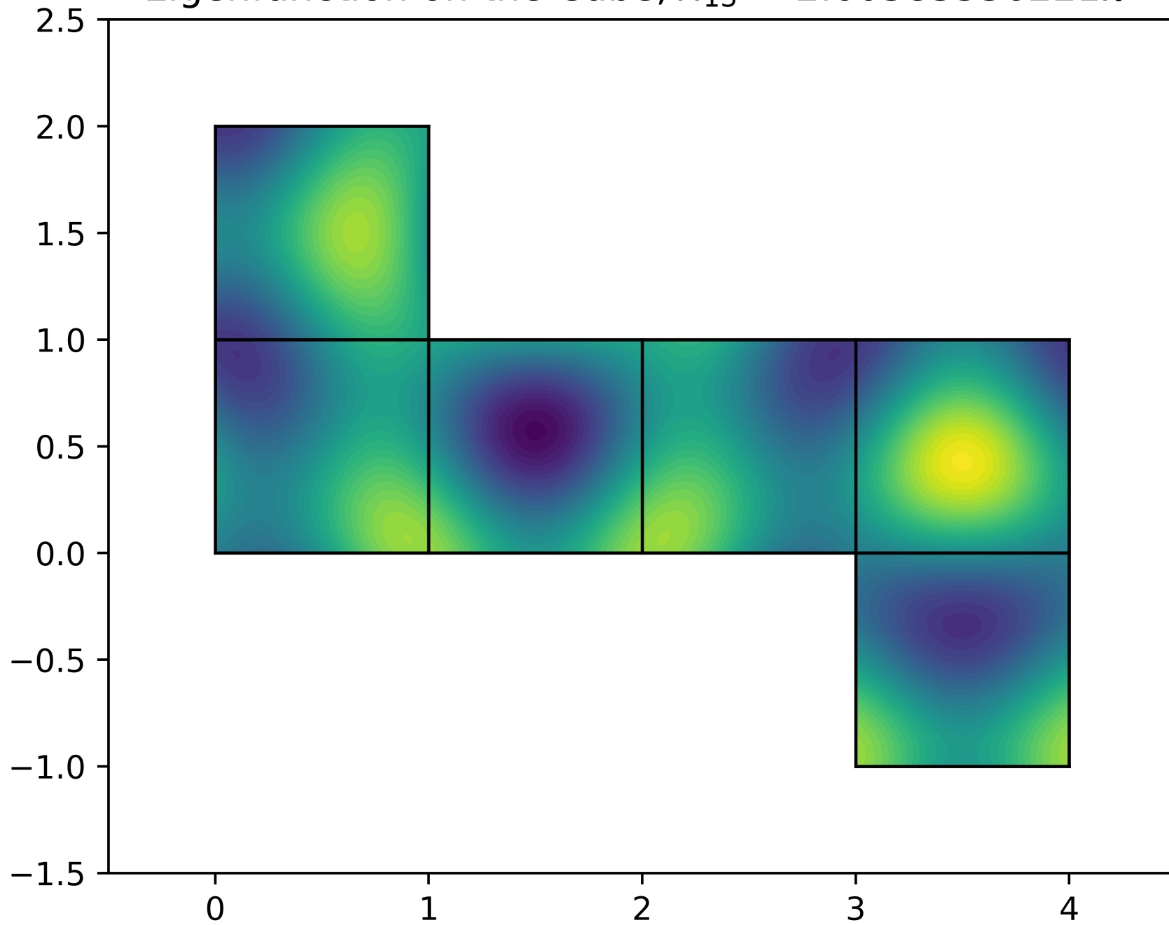
Eigenfunction on the Cube, \lambda_{13} = 2.60383536221\pi^2
