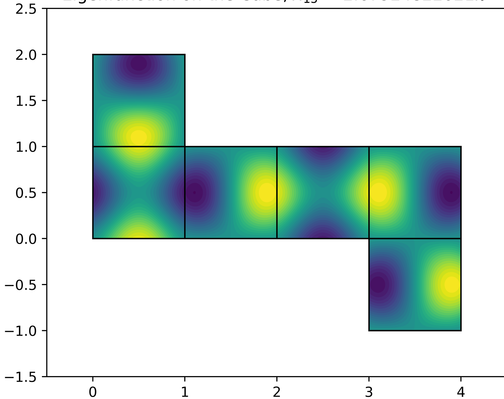
Eigenfunction on the Cube, \lambda_{15} = 2.67924822021\pi^2
