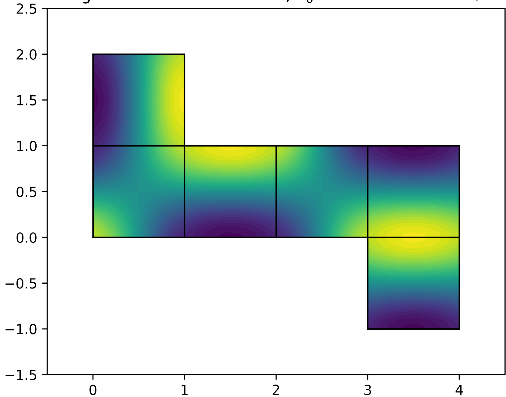
Eigenfunction on the Cube, \lambda_6 = 1.16501842198\pi^2
