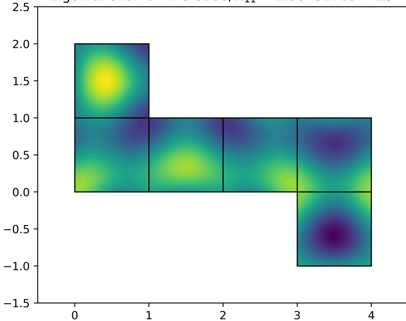
Eigenfunction on the Cube, \lambda_{11} = 2.59431769771\pi^2
