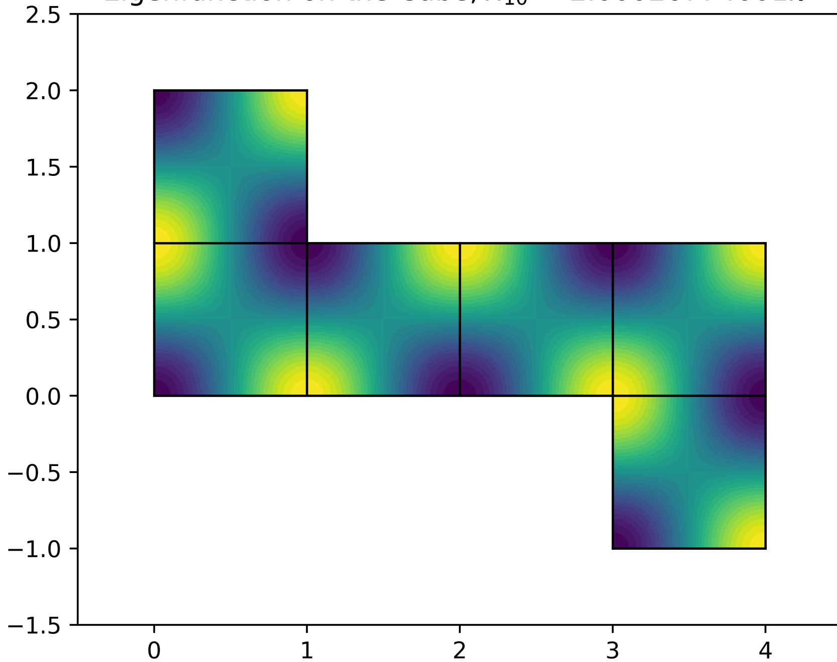
Eigenfunction on the Cube, \lambda_{10} = 2.00026774001\pi^2
