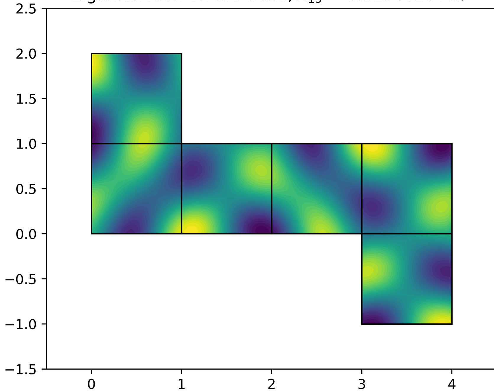
Eigenfunction on the Cube, \lambda_{19} = 3.819402644\pi^2
