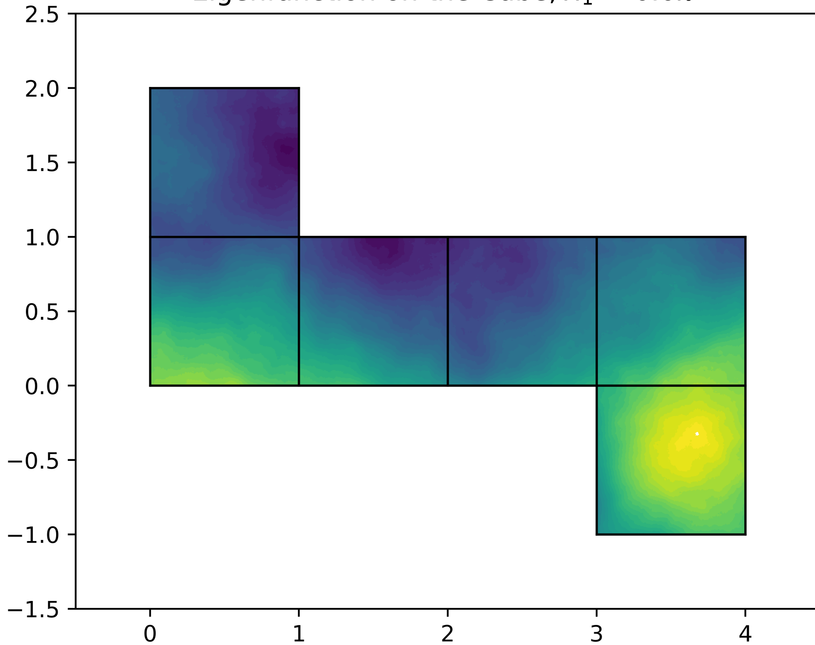
Eigenfunction on the Cube, \lambda_1 = 0.0\pi^2
