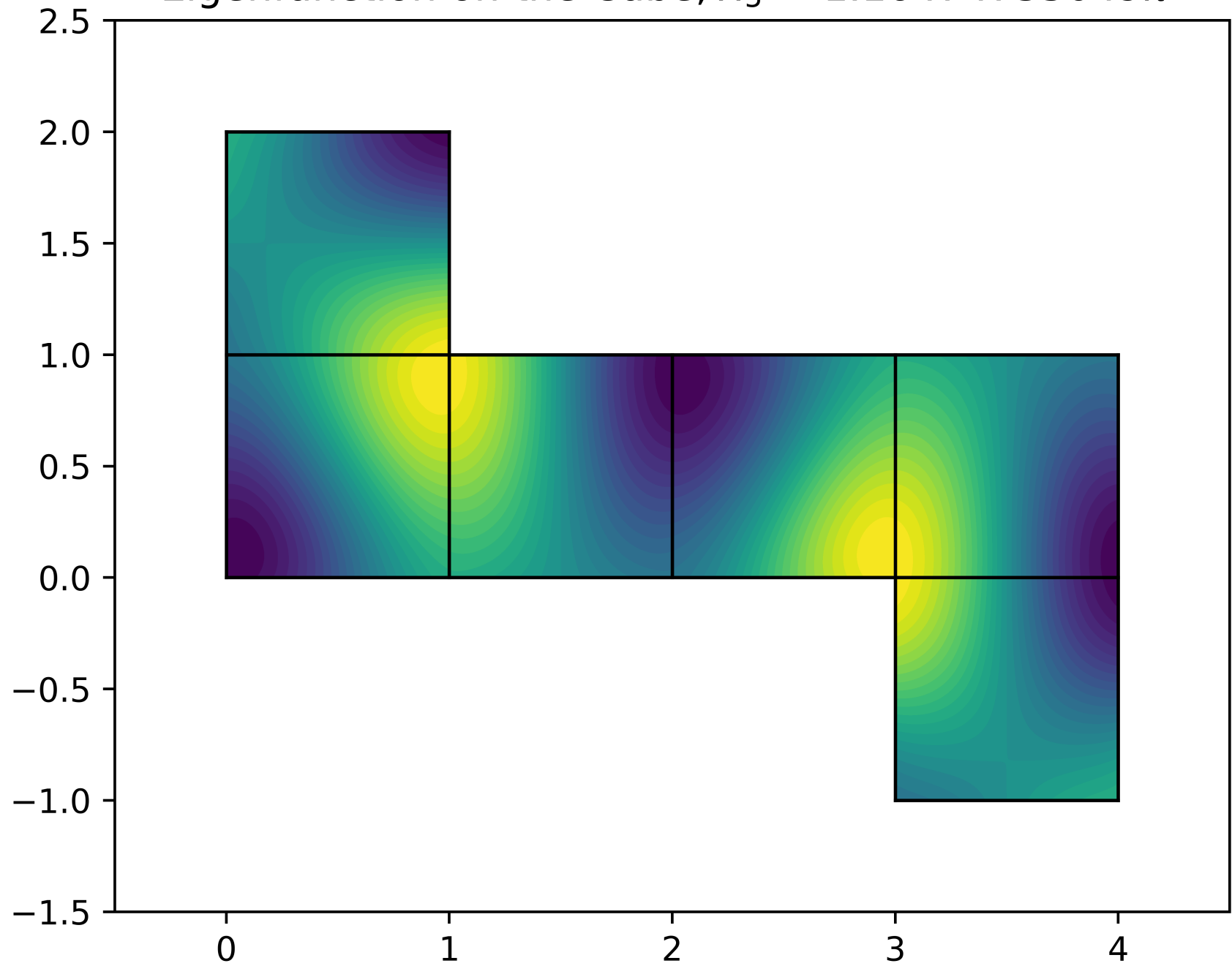
Eigenfunction on the Cube, \lambda_5 = 1.16474735049\pi^2
