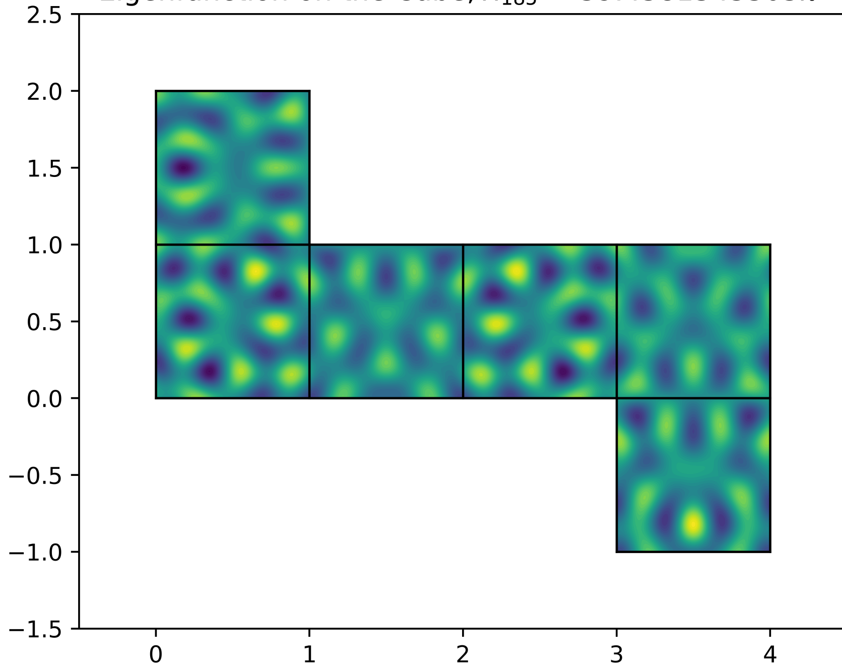
Eigenfunction on the Cube, \lambda_{185} = 39.4381343303\pi^2
