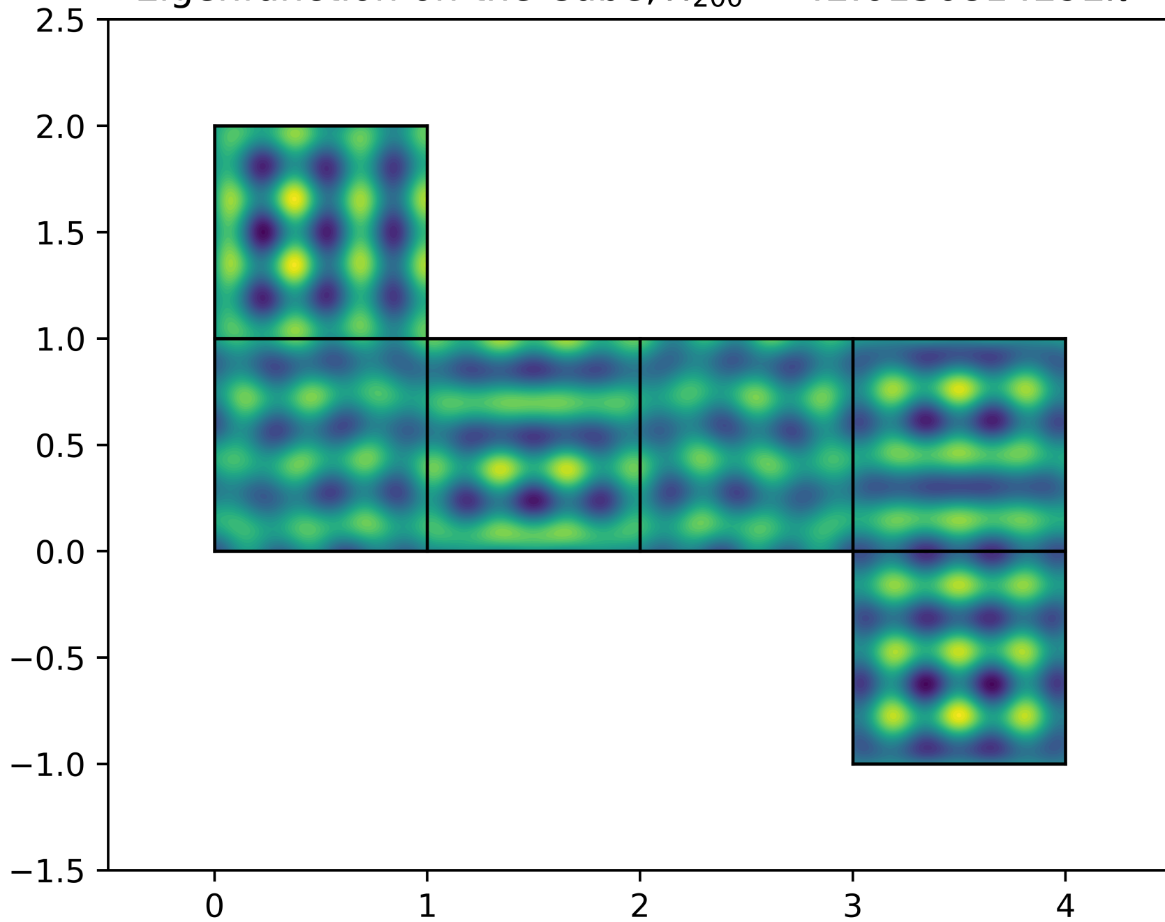
Eigenfunction on the Cube, \lambda_{200} = 42.6156814292\pi^2
