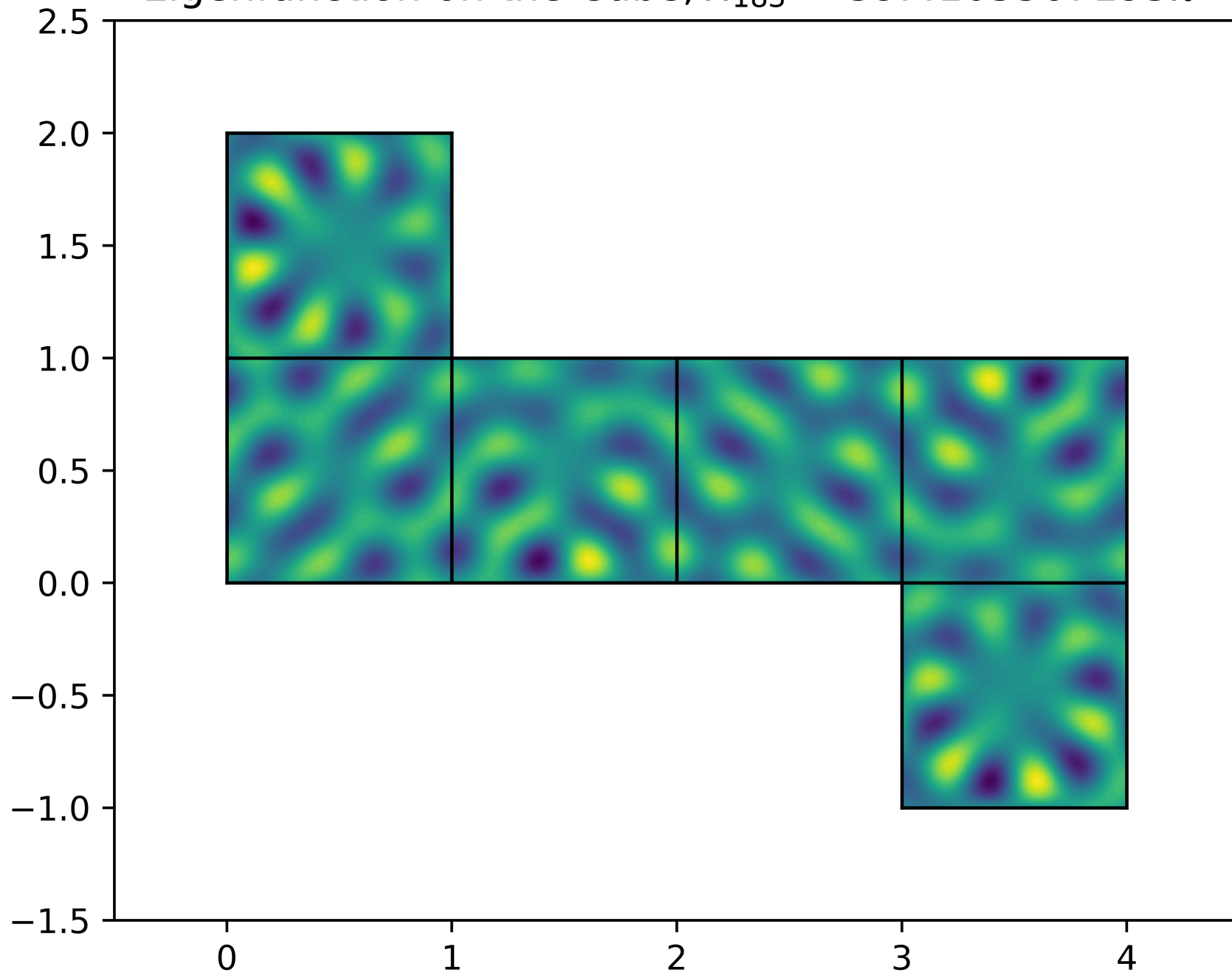
Eigenfunction on the Cube, \lambda_{183} = 39.4105567195\pi^2
