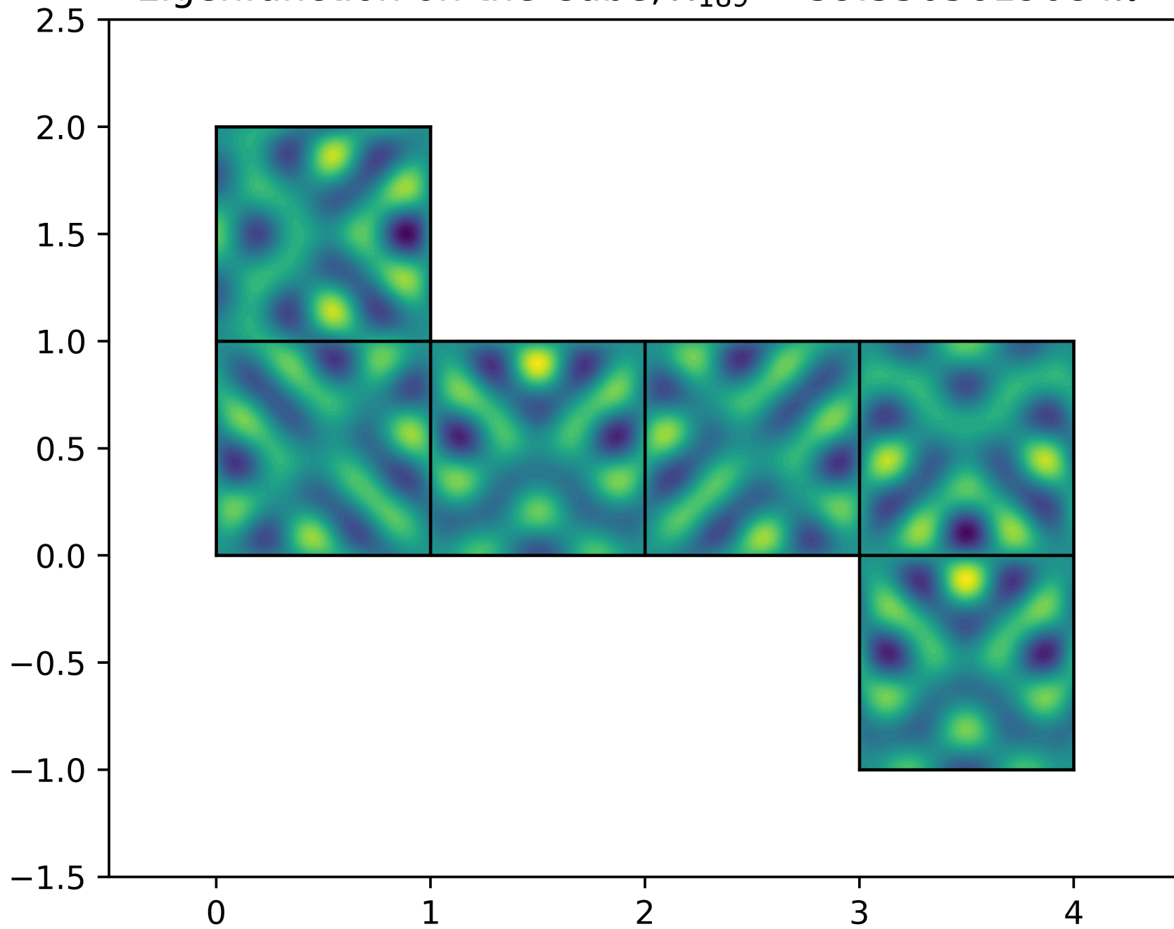
Eigenfunction on the Cube, \lambda_{189} = 39.5505619084\pi^2
