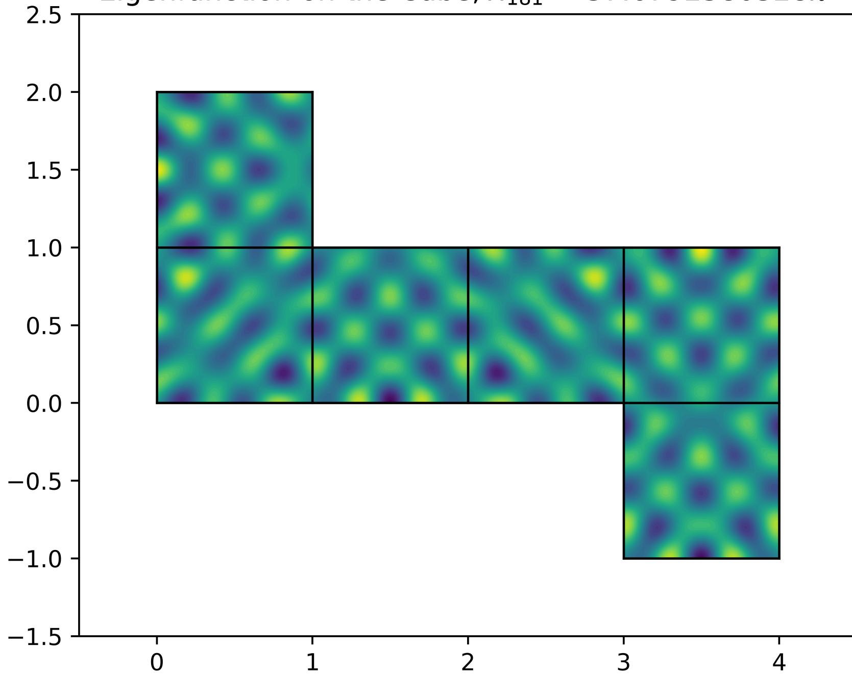
Eigenfunction on the Cube, \lambda_{181} = 37.6792580328\pi^2
