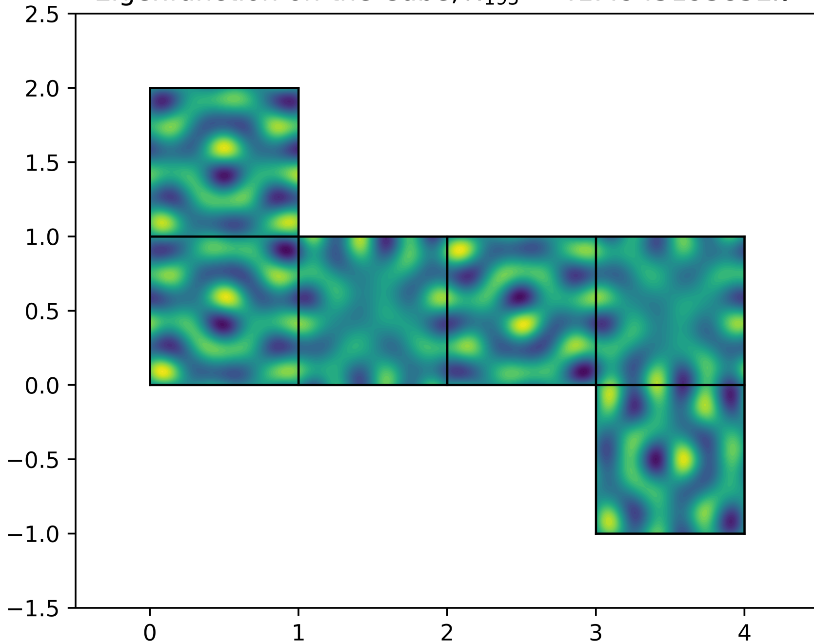
Eigenfunction on the Cube, \lambda_{195} = 41.4945193852\pi^2
