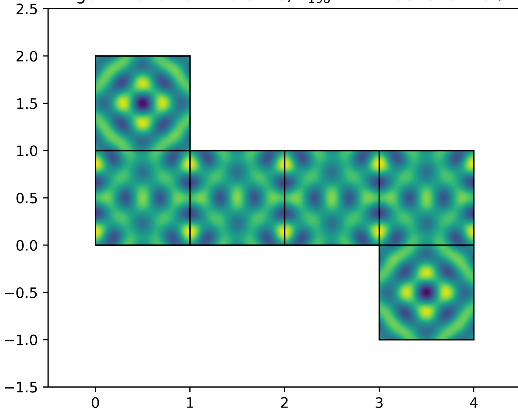
Eigenfunction on the Cube, \lambda_{198} = 42.0952543715\pi^2
