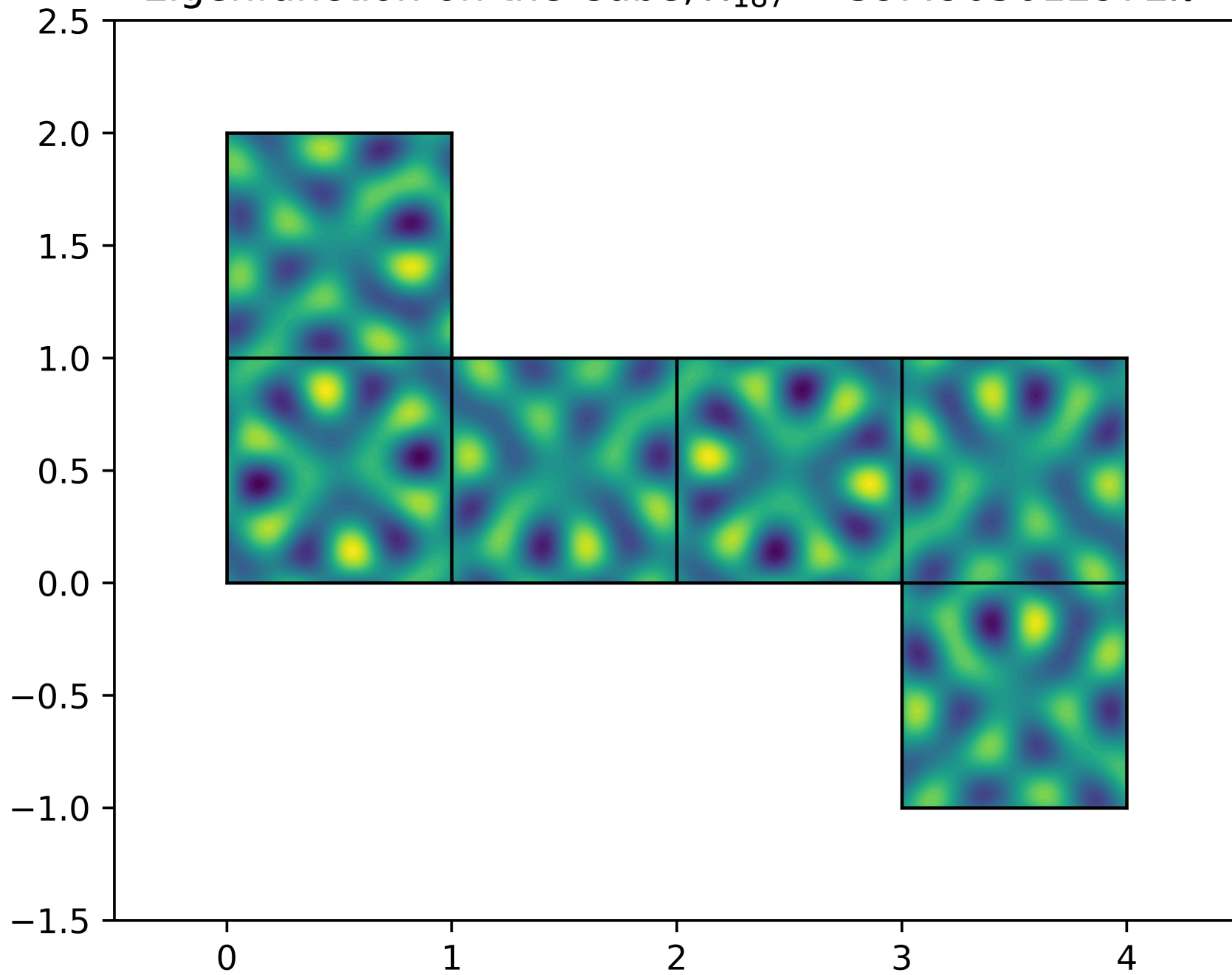
Eigenfunction on the Cube, \lambda_{187} = 39.4905012972\pi^2
