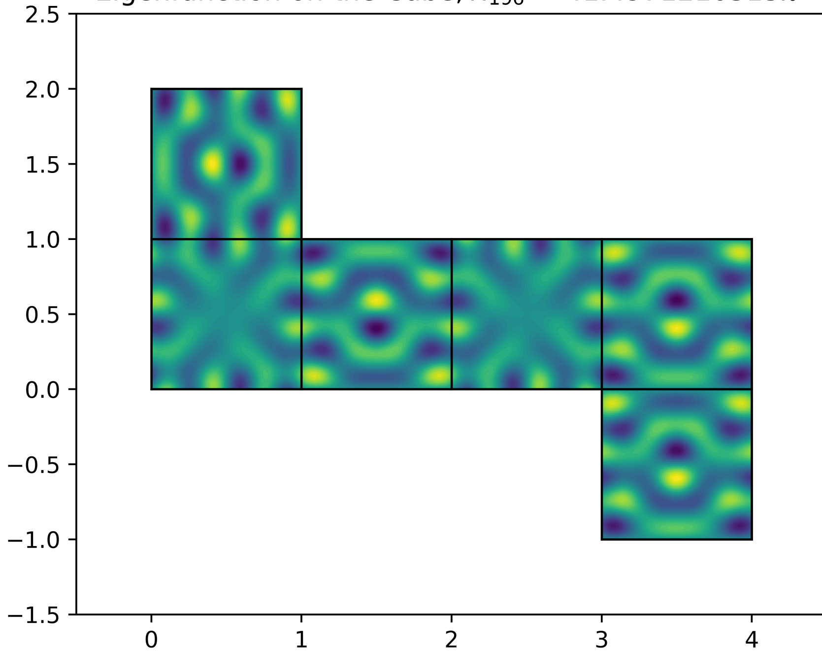
Eigenfunction on the Cube, \lambda_{196} = 41.4971210313\pi^2
