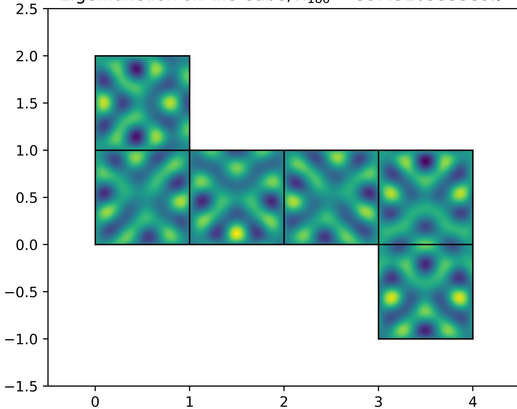
Eigenfunction on the Cube, \lambda_{186} = 39.4510935389\pi^2
