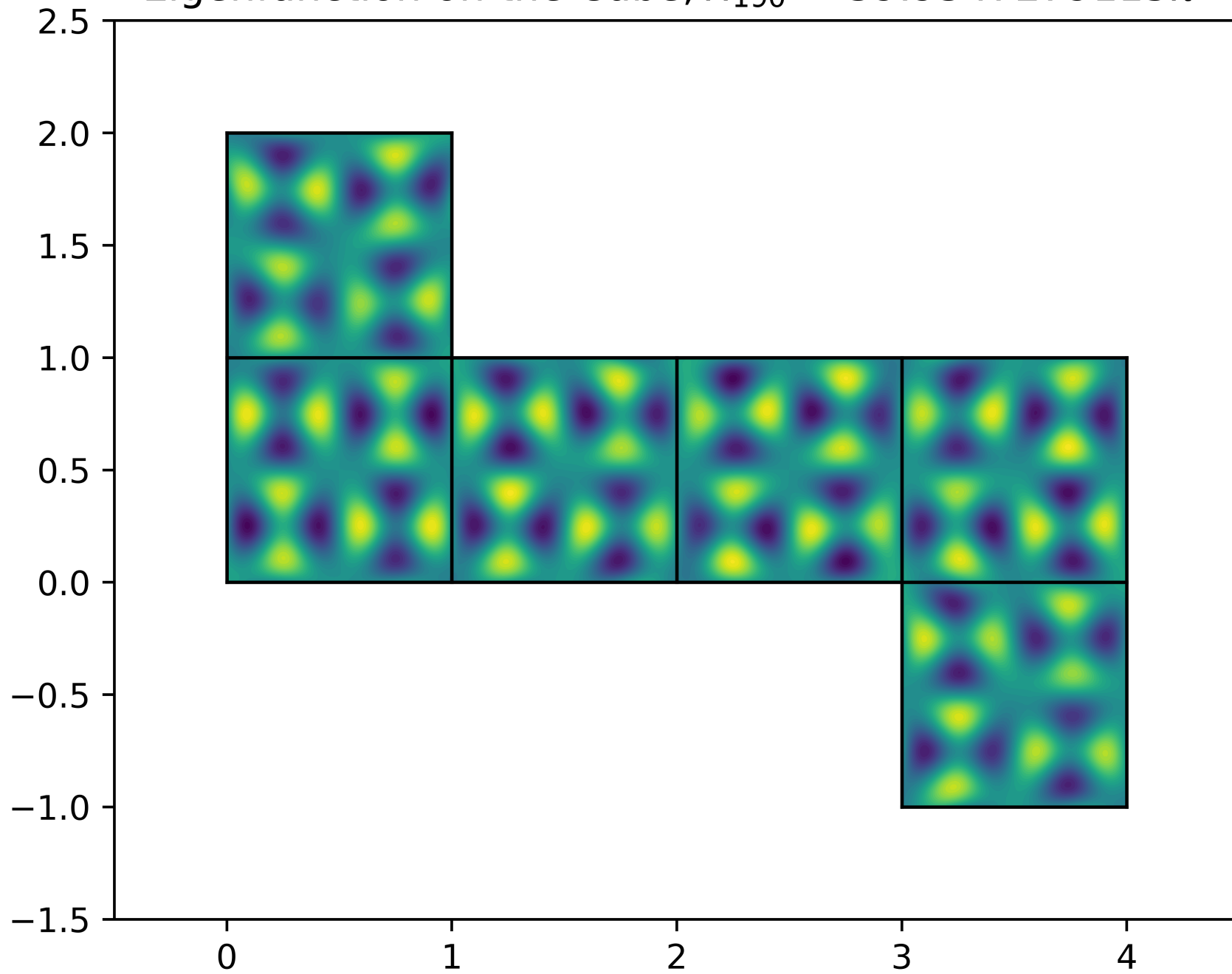
Eigenfunction on the Cube, \lambda_{190} = 39.9347279115\pi^2
