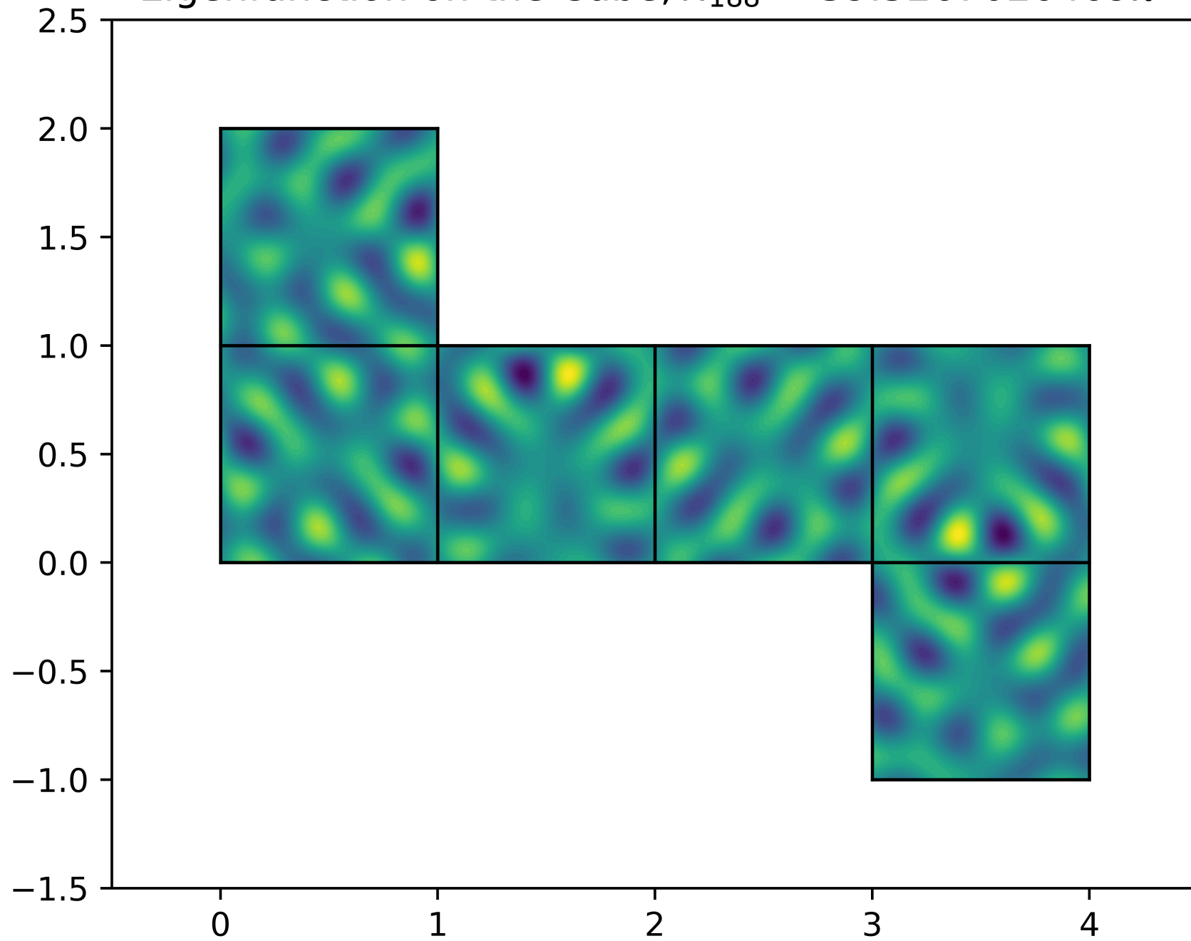
Eigenfunction on the Cube, \lambda_{188} = 39.5267026469\pi^2
