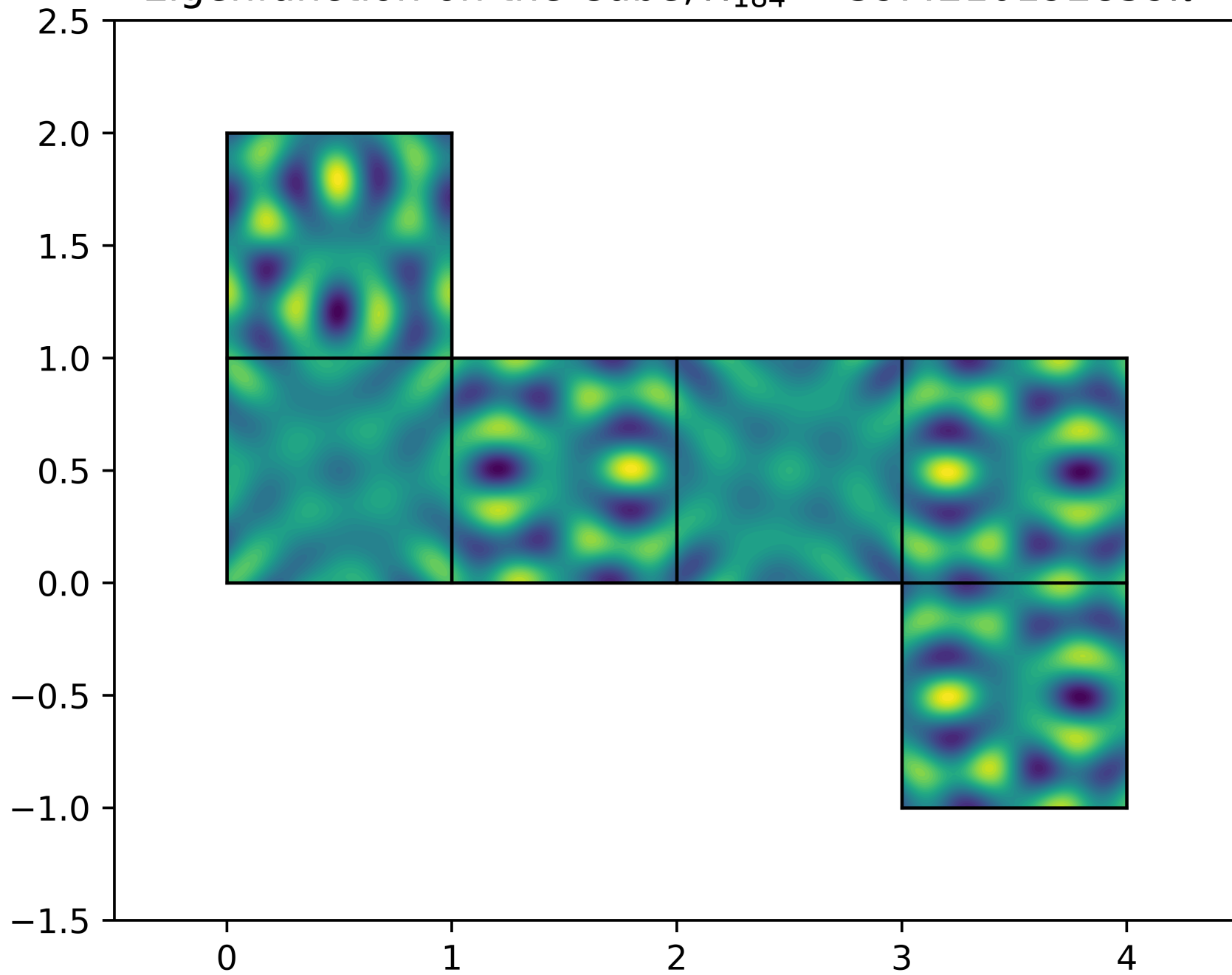
Eigenfunction on the Cube, \lambda_{184} = 39.4210192859\pi^2
