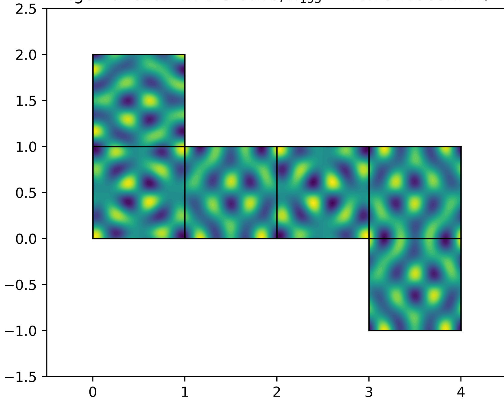
Eigenfunction on the Cube, \lambda_{193} = 40.1516909277\pi^2
