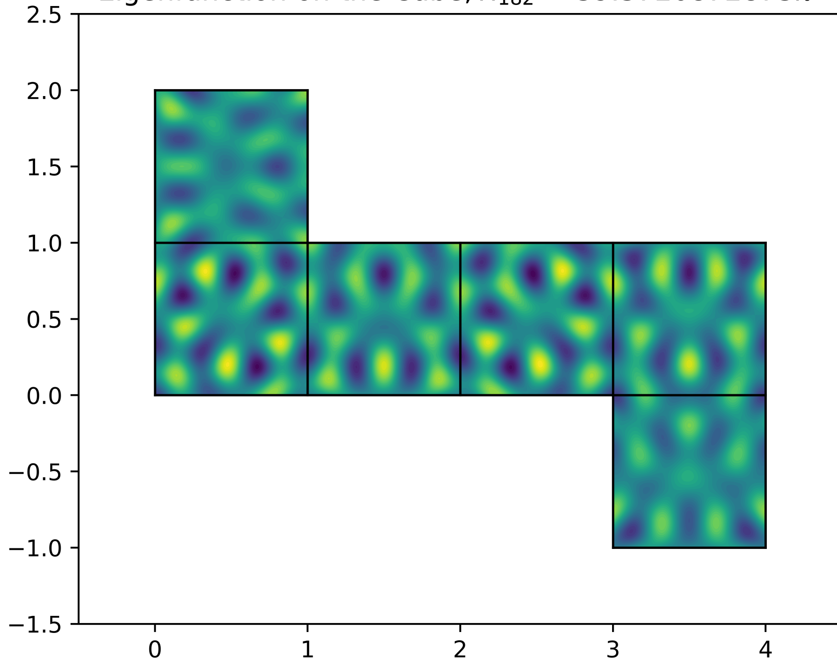
Eigenfunction on the Cube, \lambda_{182} = 39.3720872873\pi^2
