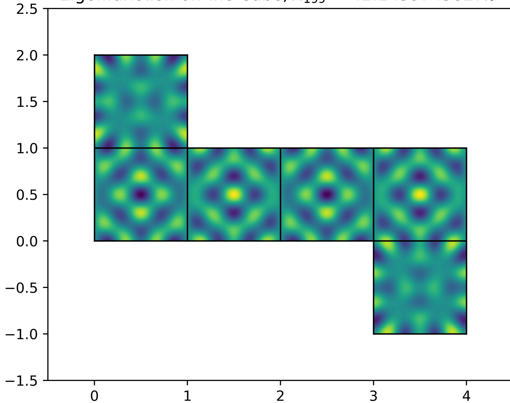
Eigenfunction on the Cube, \lambda_{199} = 42.1459745827\pi^2
