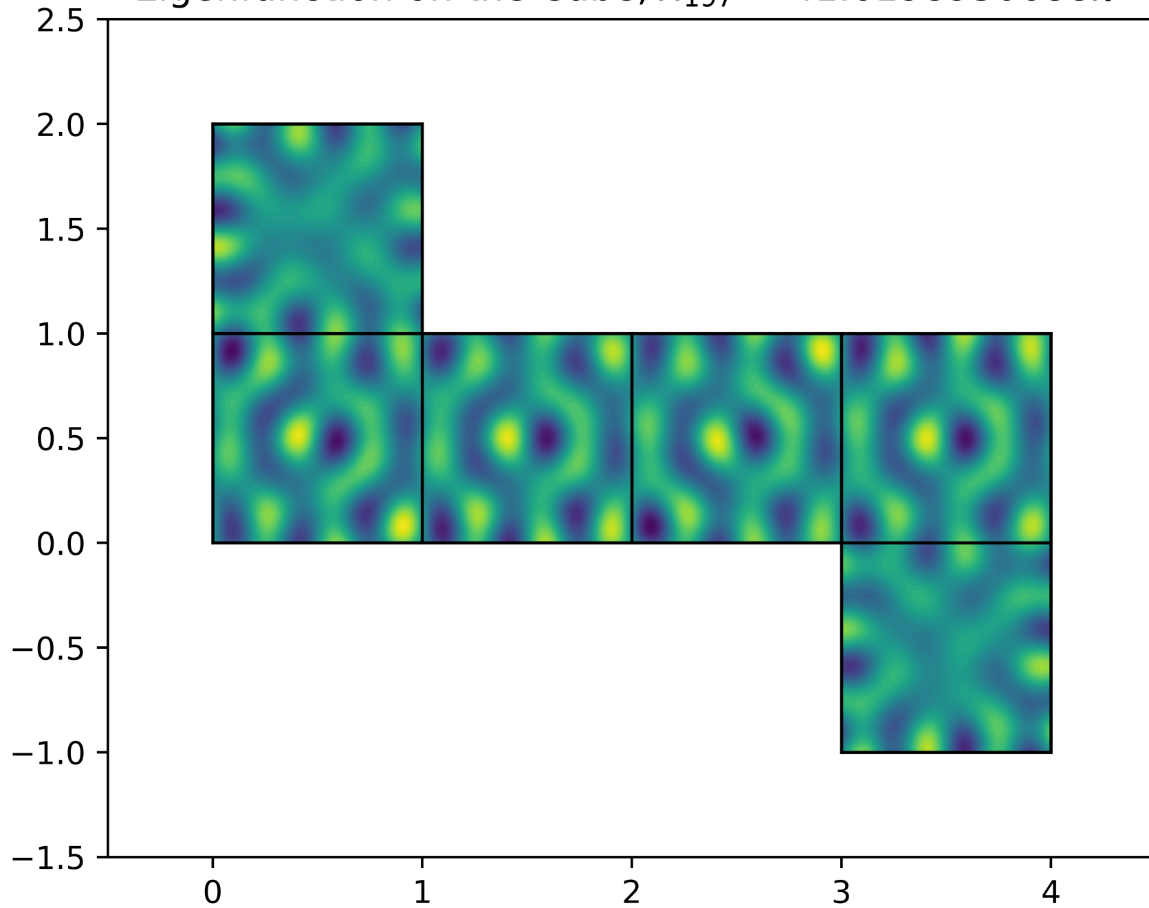
Eigenfunction on the Cube, \lambda_{197} = 41.6198930688\pi^2
