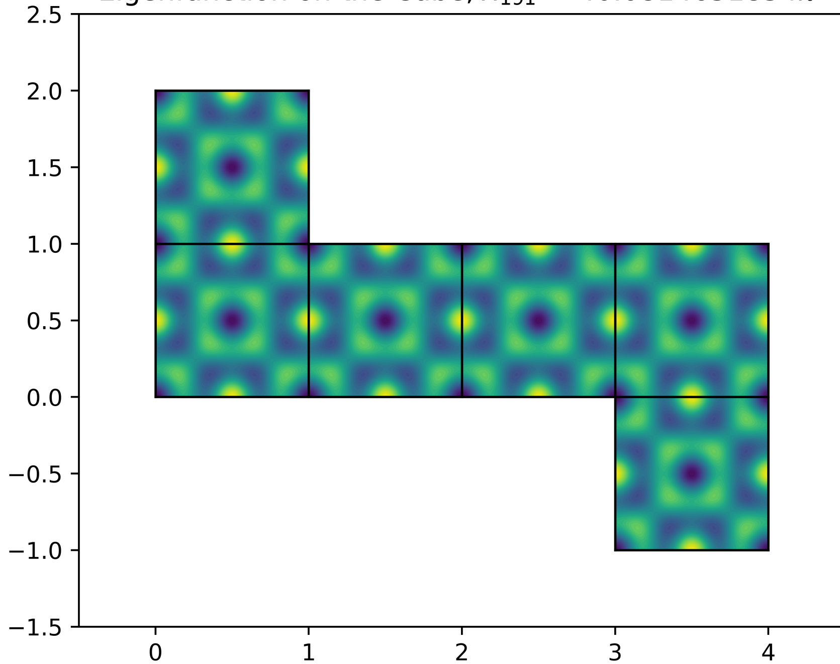
Eigenfunction on the Cube, \lambda_{191} = 40.0814651834\pi^2
