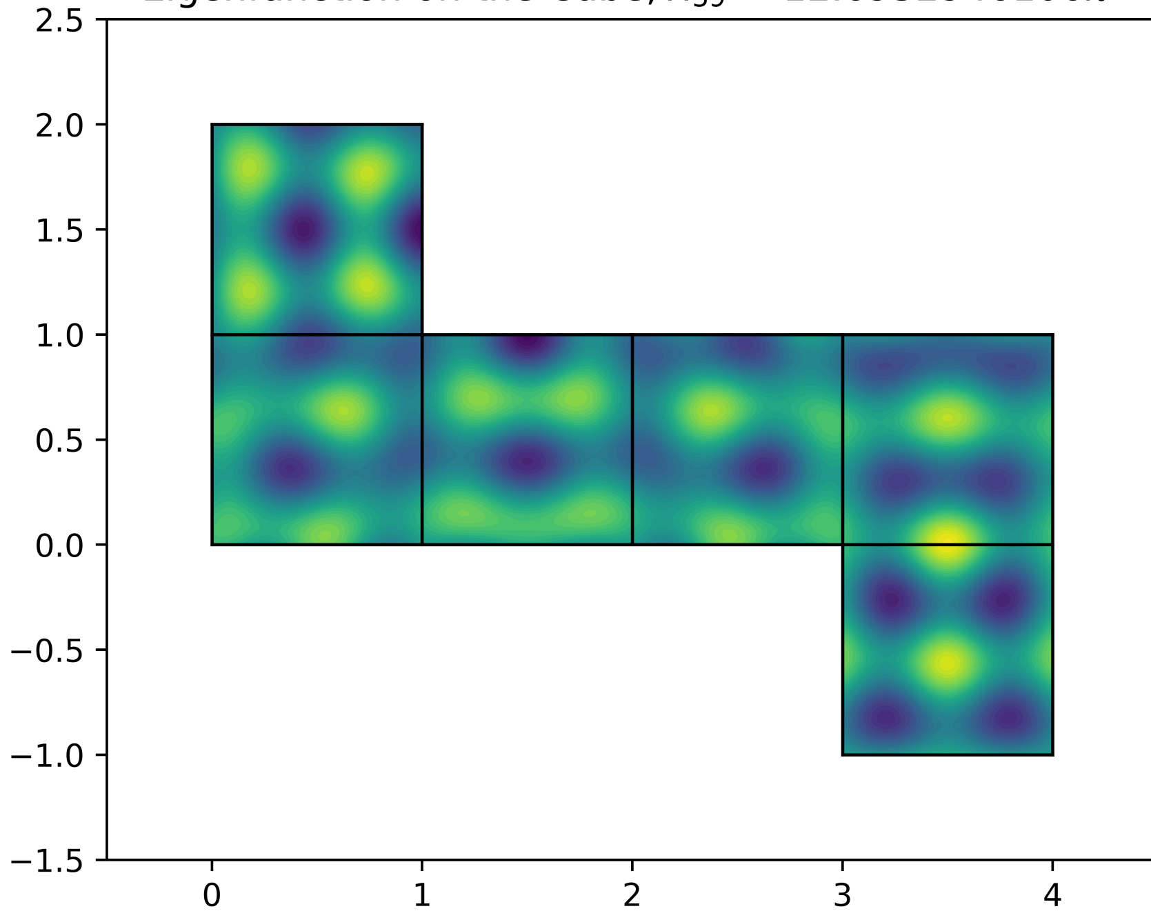
Eigenfunction on the Cube, \lambda_{59} = 12.6932946106\pi^2
