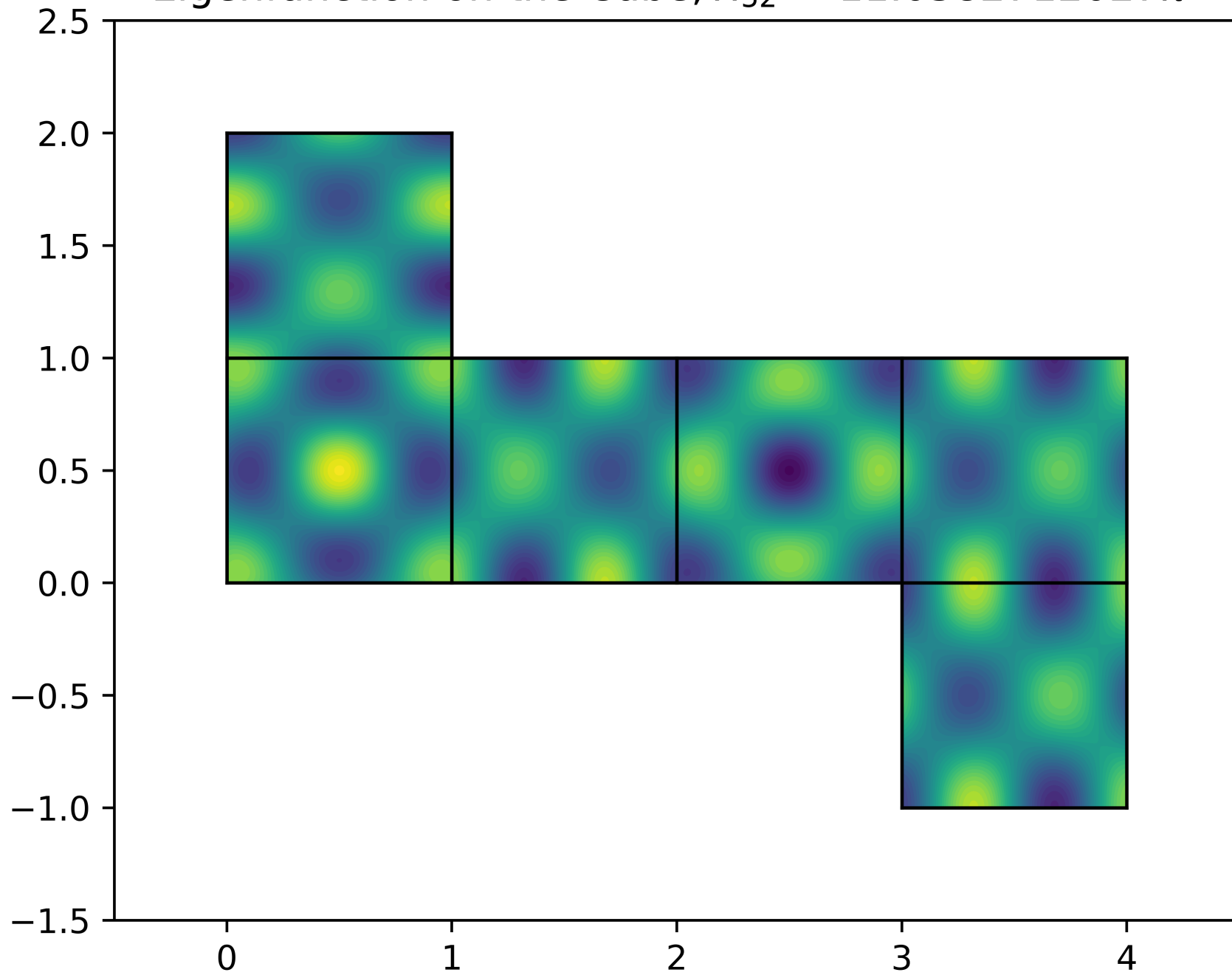
Eigenfunction on the Cube, \lambda_{52} = 11.0382712027\pi^2
