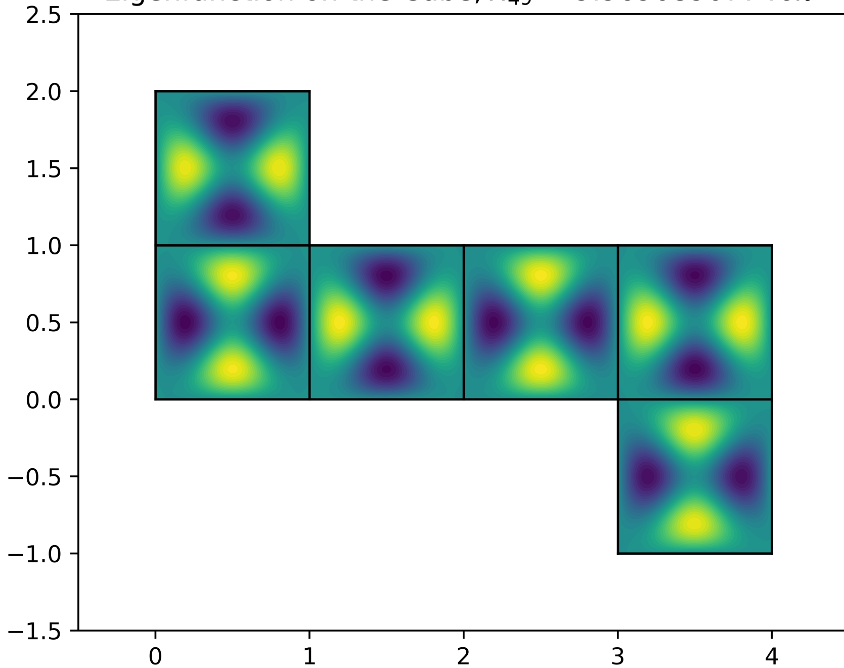
Eigenfunction on the Cube, \lambda_{49} = 9.96908907746\pi^2
