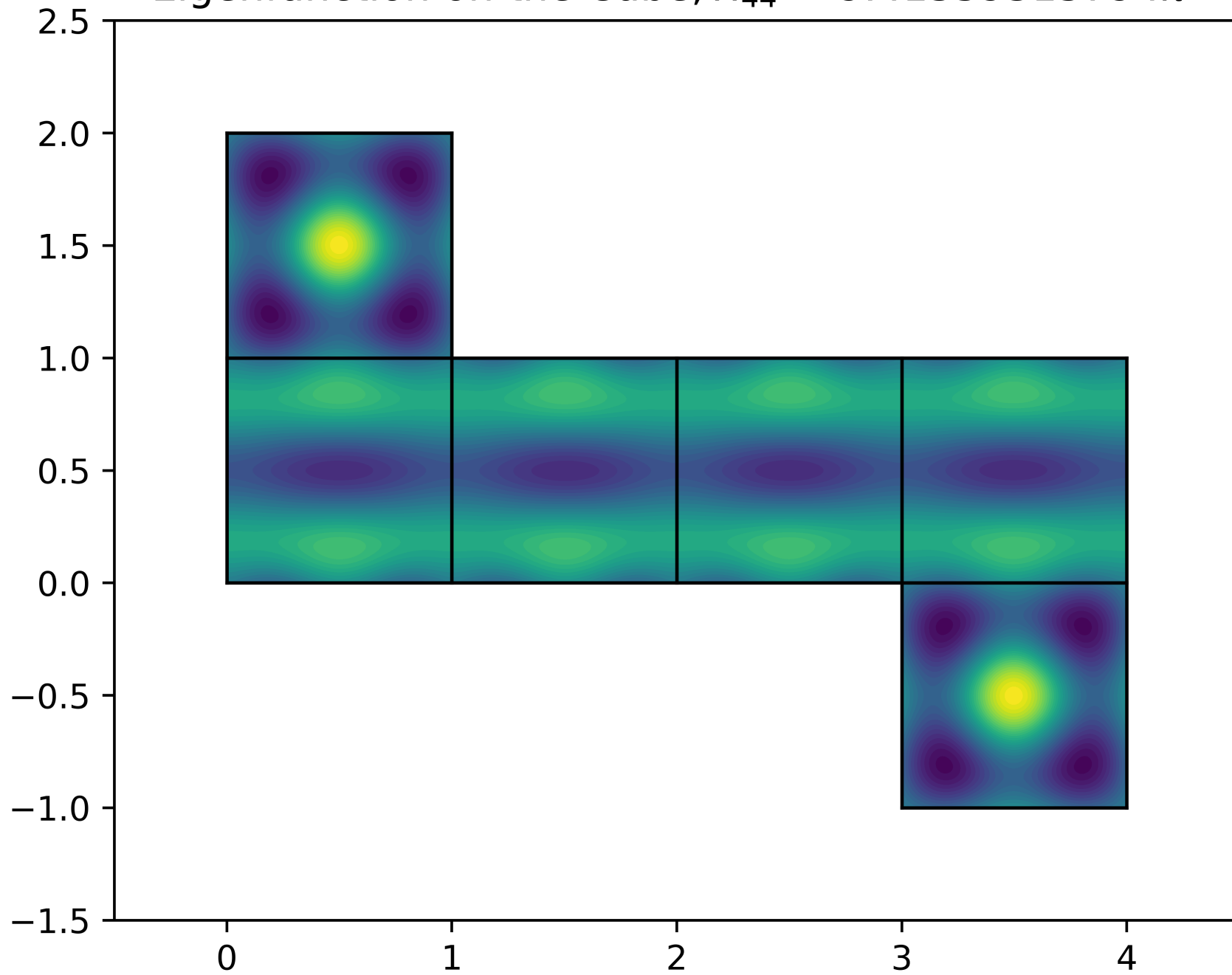
Eigenfunction on the Cube, \lambda_{44} = 9.41359315794\pi^2
