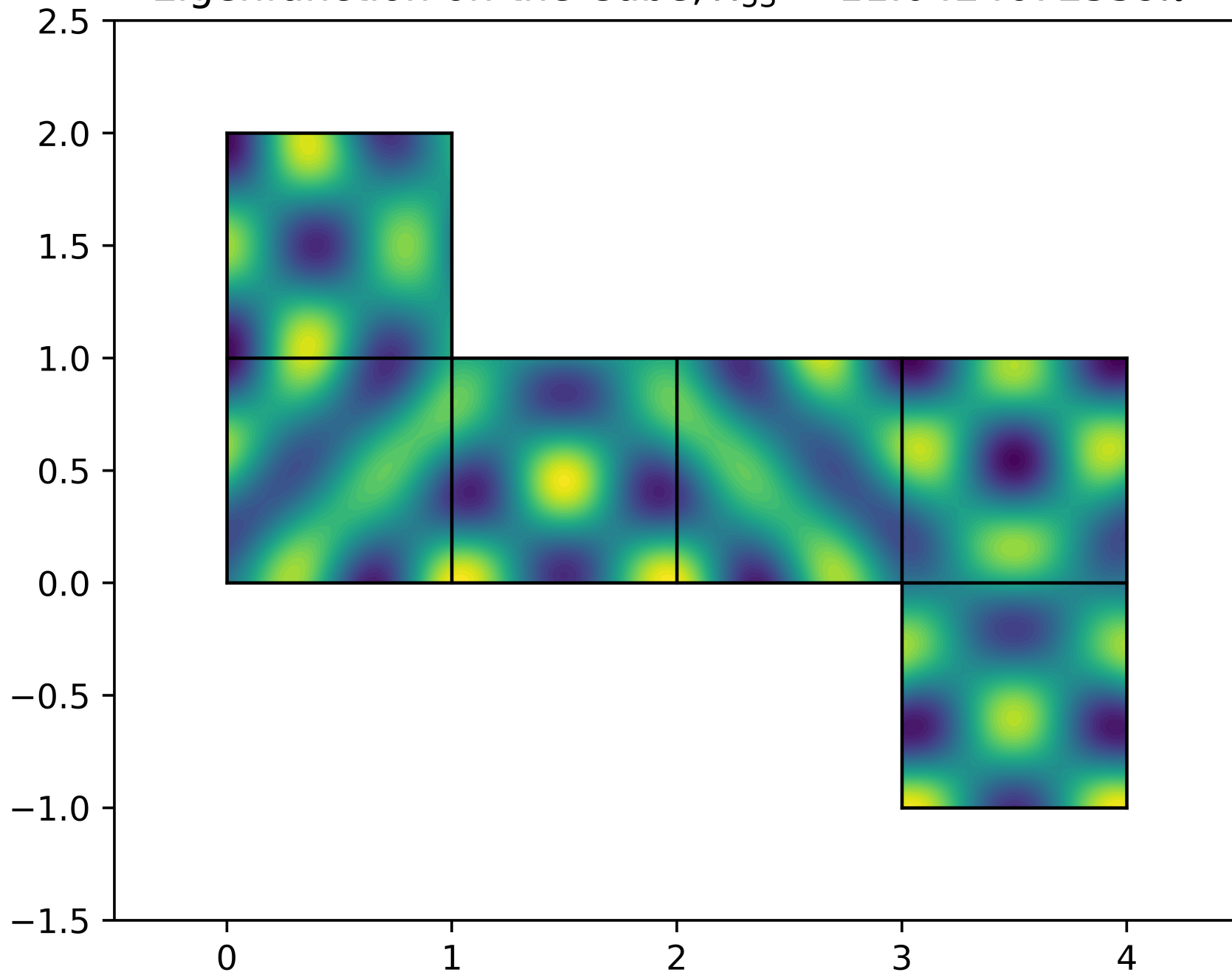
Eigenfunction on the Cube, \lambda_{53} = 11.0424672559\pi^2
