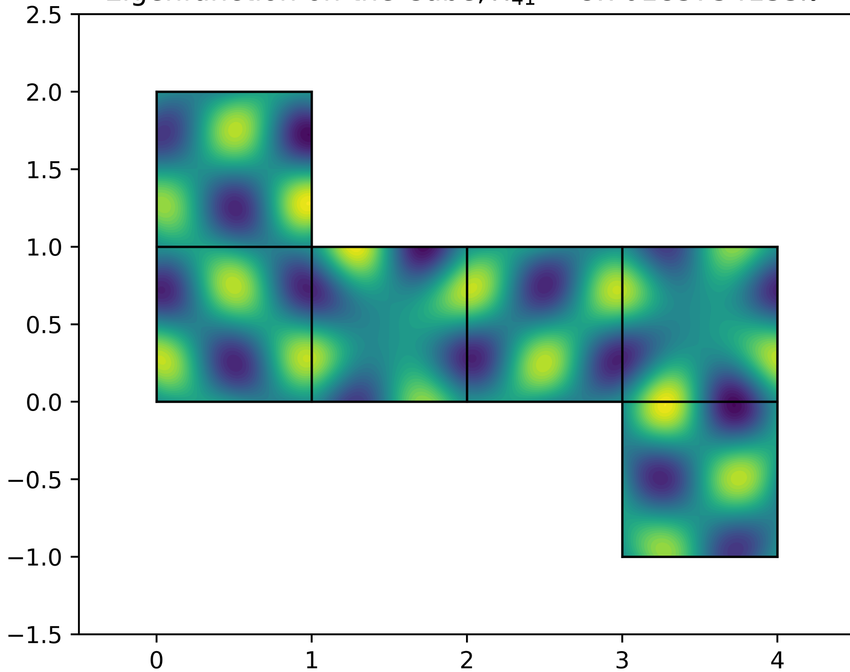
Eigenfunction on the Cube, \lambda_{41} = 8.70183754133\pi^2
