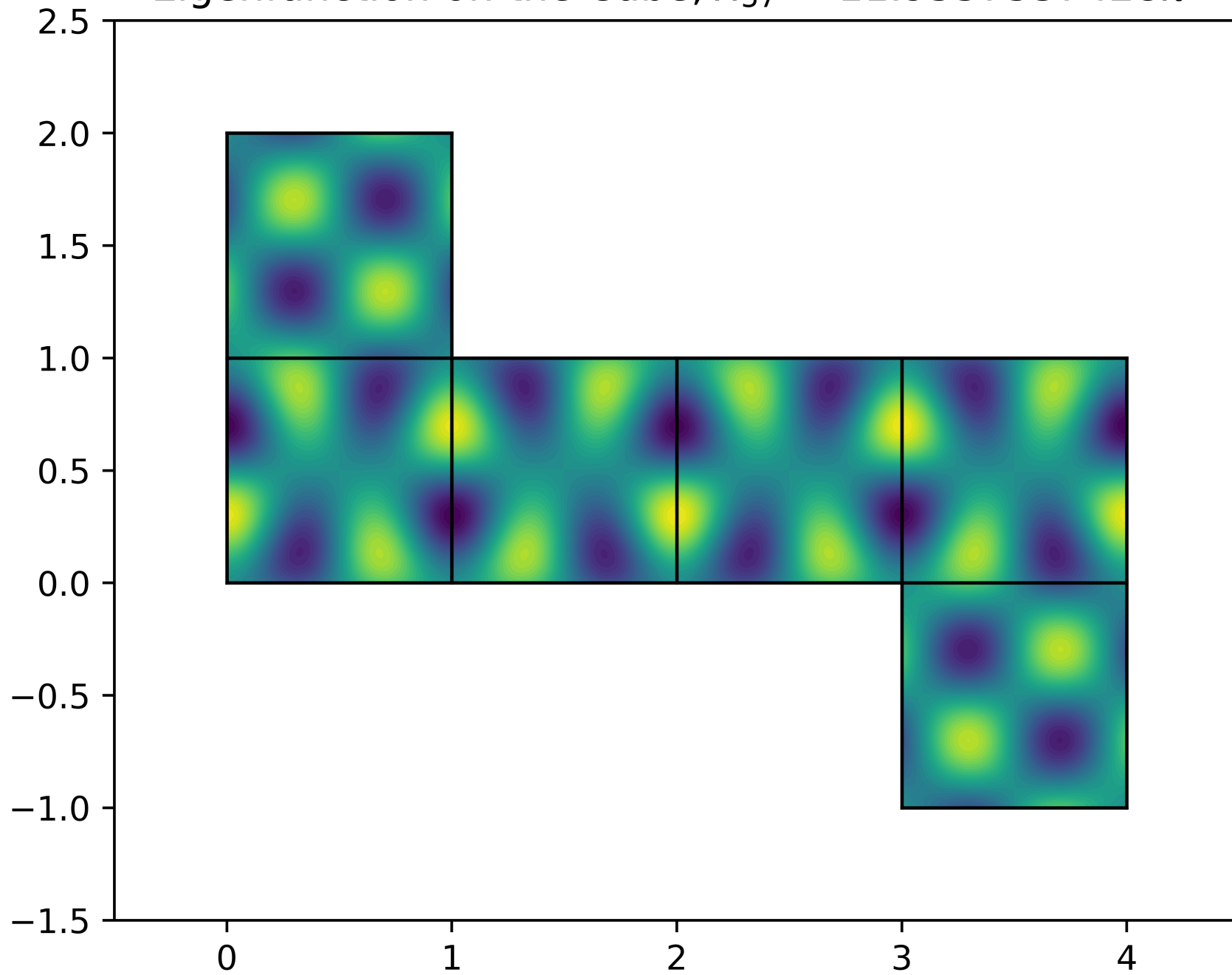
Eigenfunction on the Cube, \lambda_{57} = 11.9557537428\pi^2
