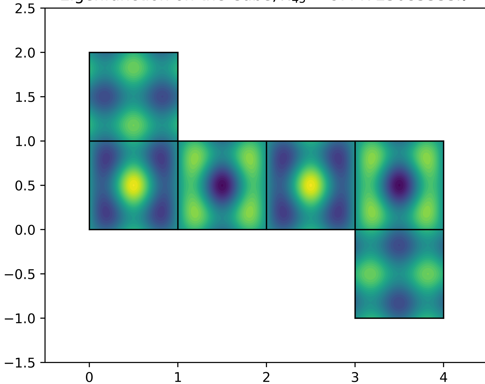
Eigenfunction on the Cube, \lambda_{45} = 9.44725085335\pi^2
