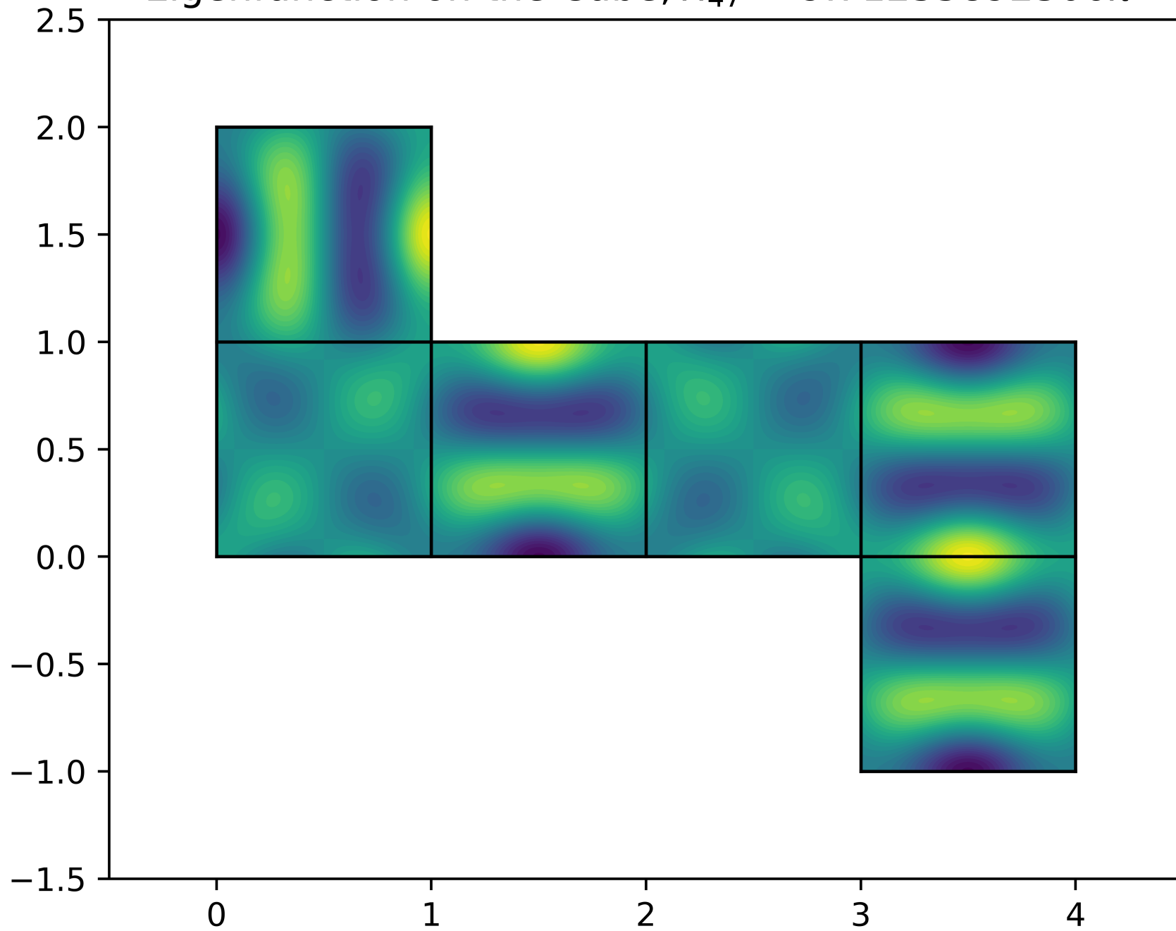
Eigenfunction on the Cube, \lambda_{47} = 9.71255892306\pi^2
