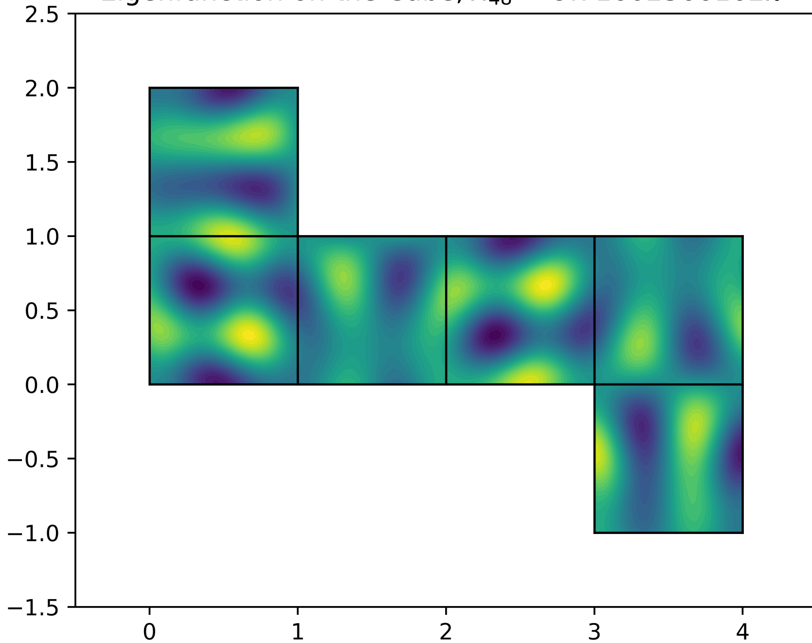
Eigenfunction on the Cube, \lambda_{48} = 9.71602366162\pi^2
