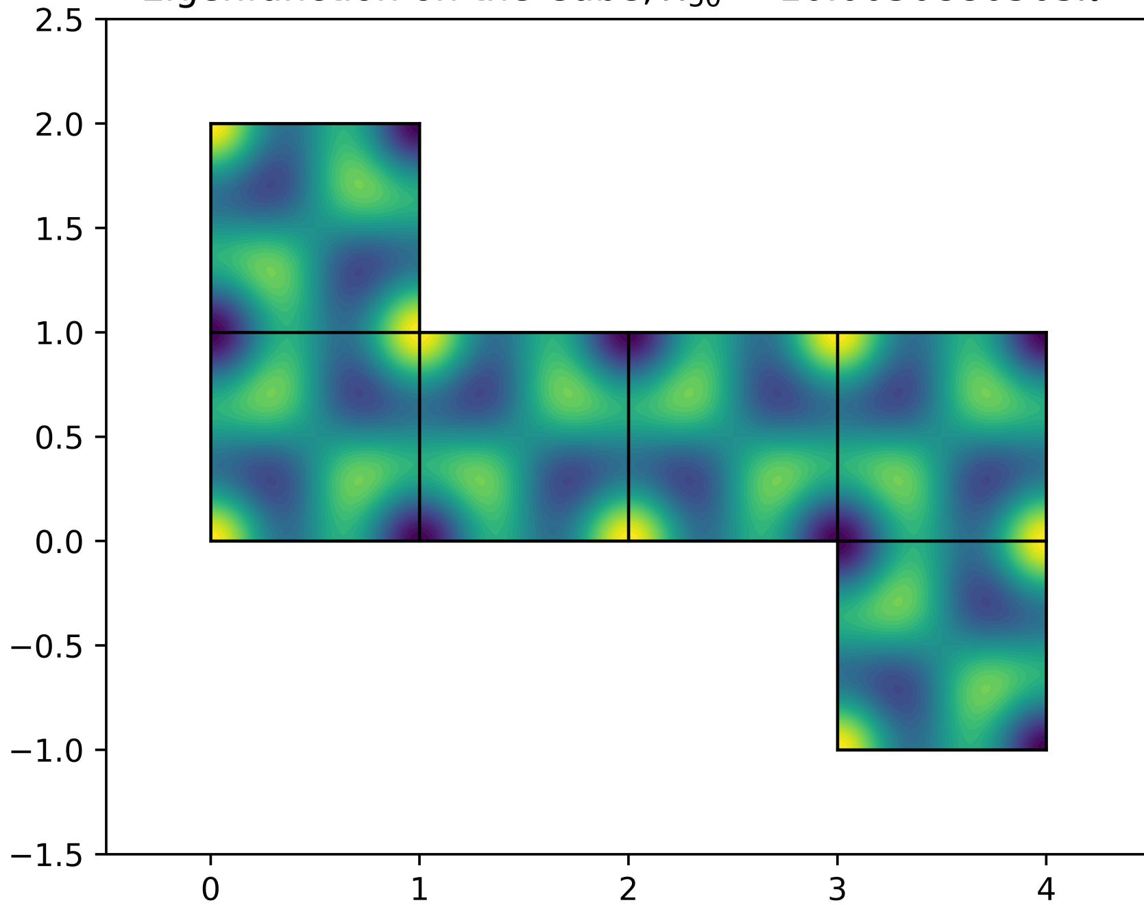
Eigenfunction on the Cube, \lambda_{50} = 10.0050880505\pi^2
