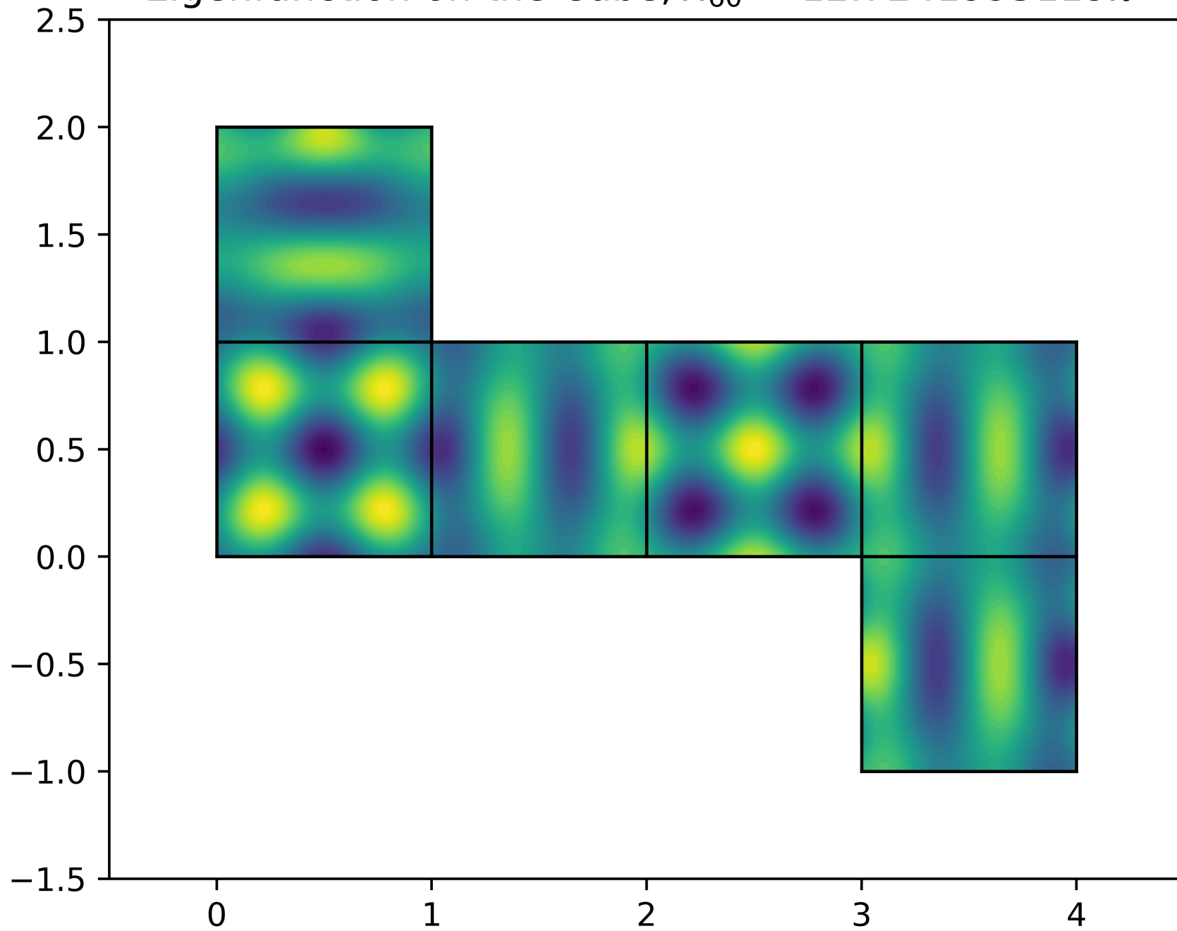
Eigenfunction on the Cube, \lambda_{60} = 12.7241995119\pi^2
