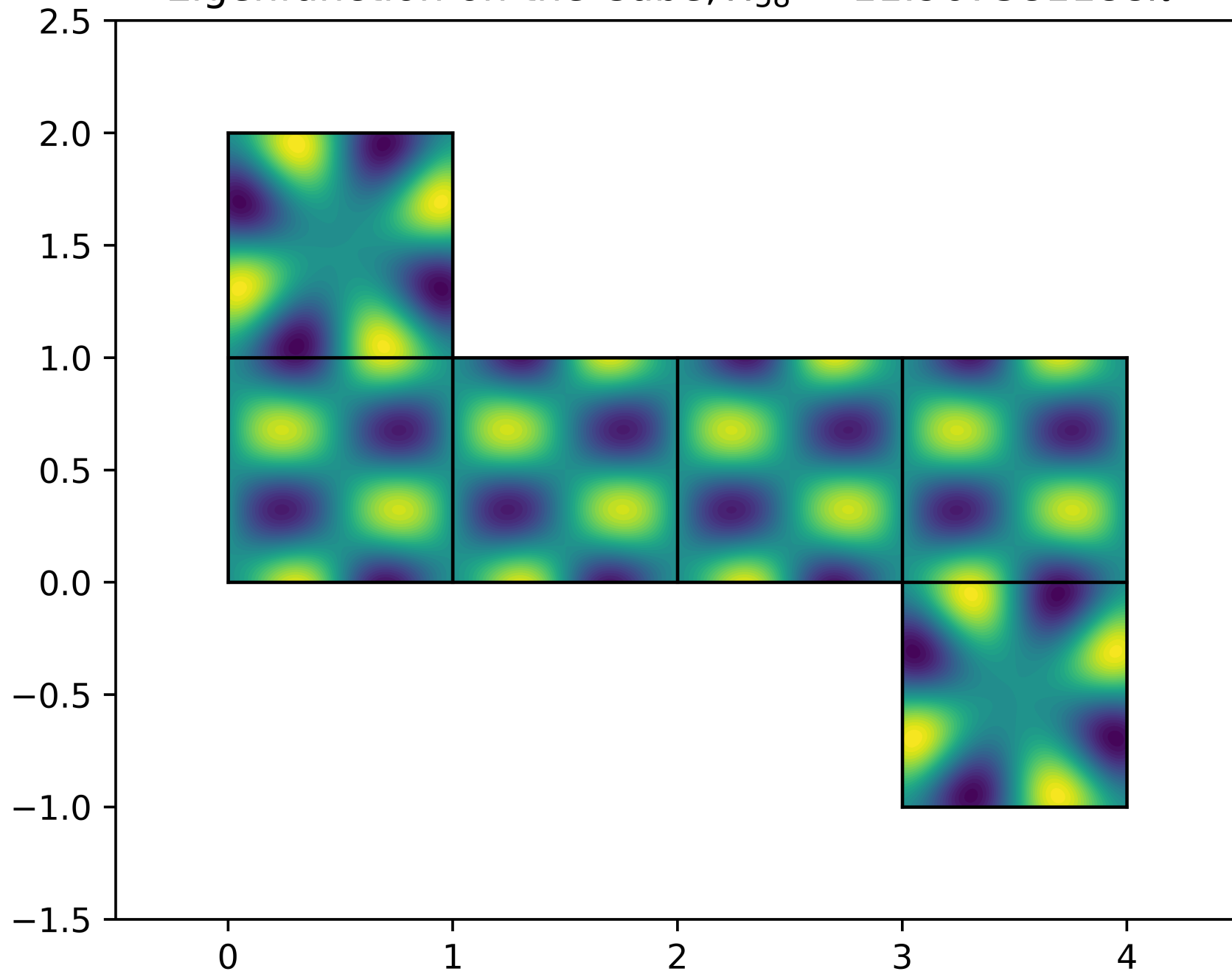
Eigenfunction on the Cube, \lambda_{58} = 11.967381188\pi^2
