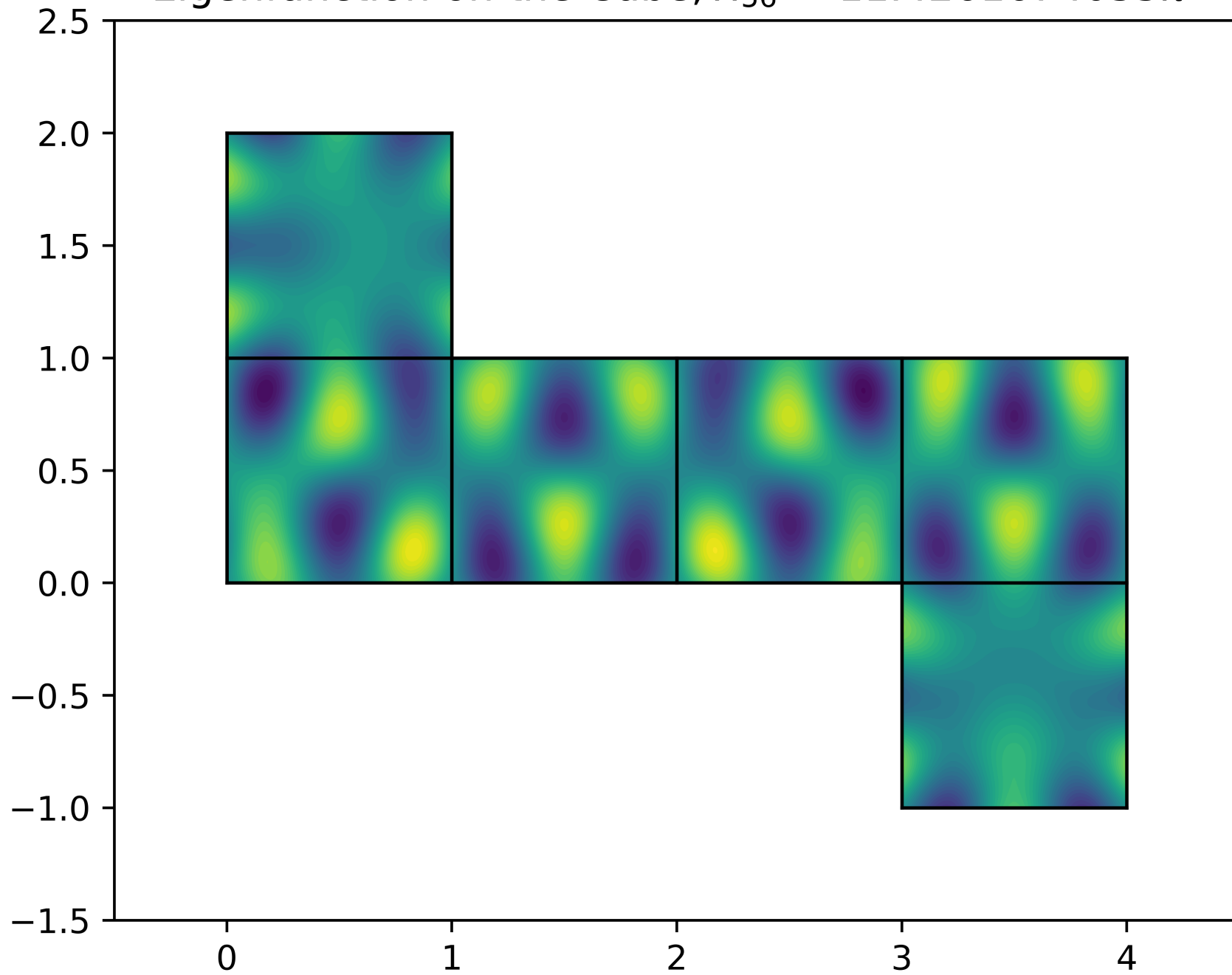
Eigenfunction on the Cube, \lambda_{56} = 11.4261674055\pi^2
