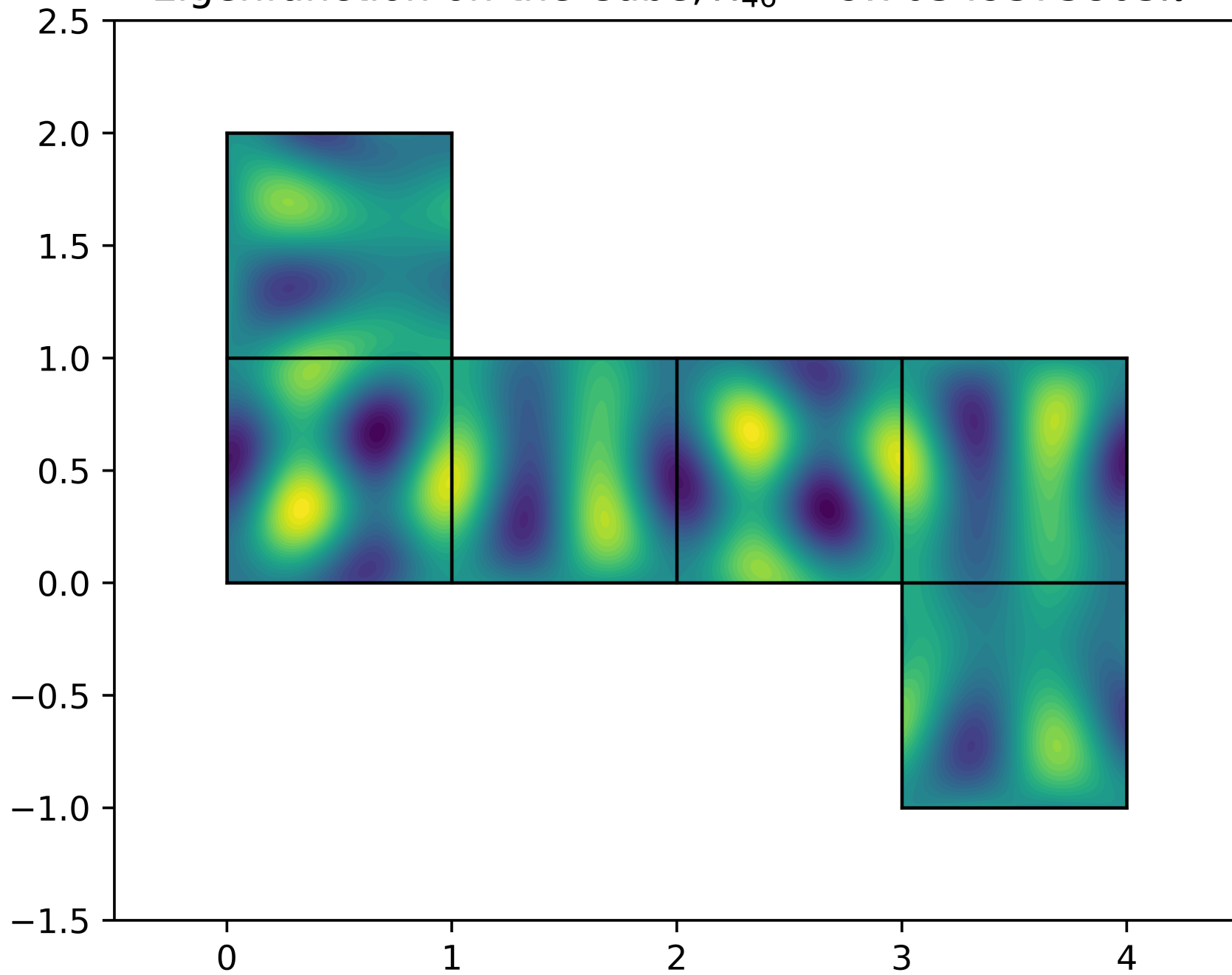
Eigenfunction on the Cube, \lambda_{46} = 9.70349373803\pi^2
