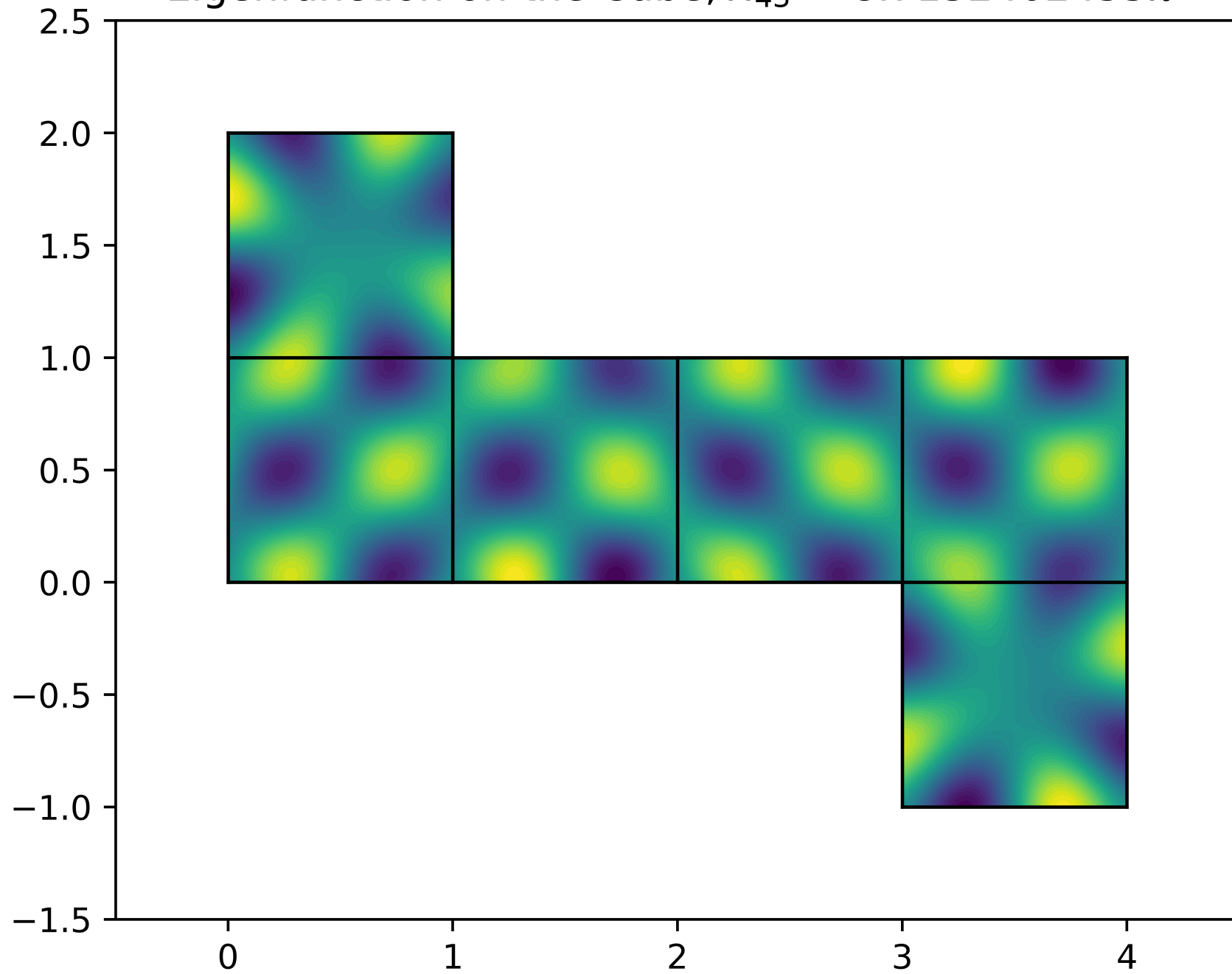
Eigenfunction on the Cube, \lambda_{43} = 8.7132402455\pi^2
