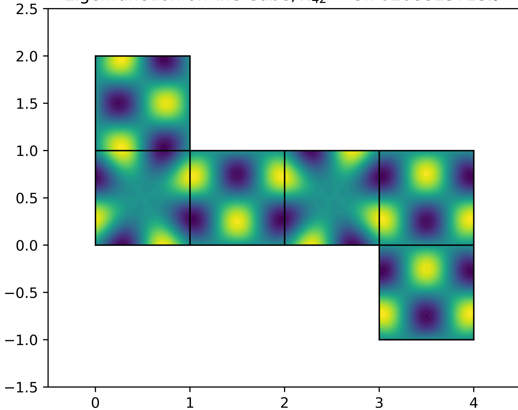
Eigenfunction on the Cube, \lambda_{42} = 8.70208813725\pi^2
