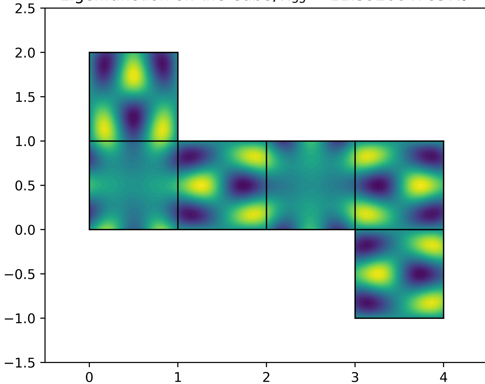
Eigenfunction on the Cube, \lambda_{55} = 11.3926647857\pi^2
