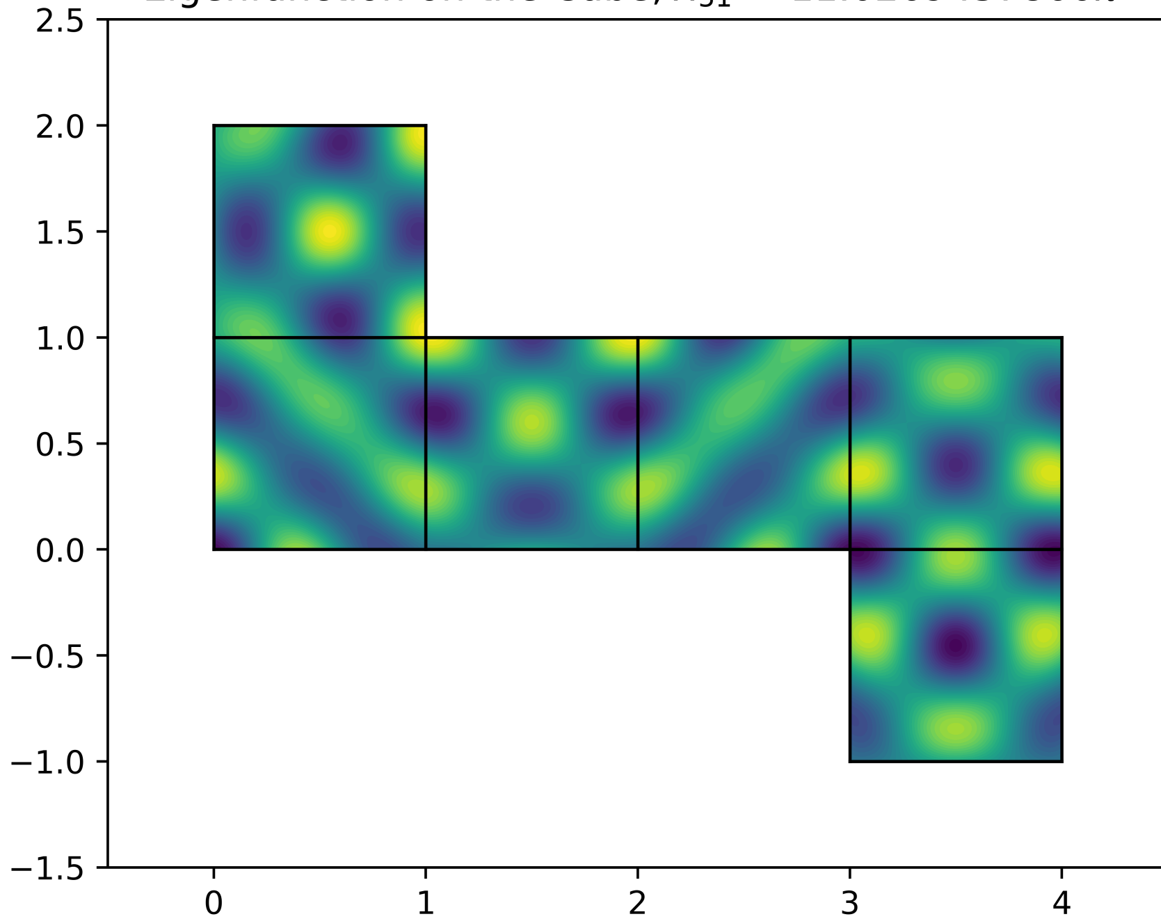
Eigenfunction on the Cube, \lambda_{51} = 11.0269437866\pi^2
