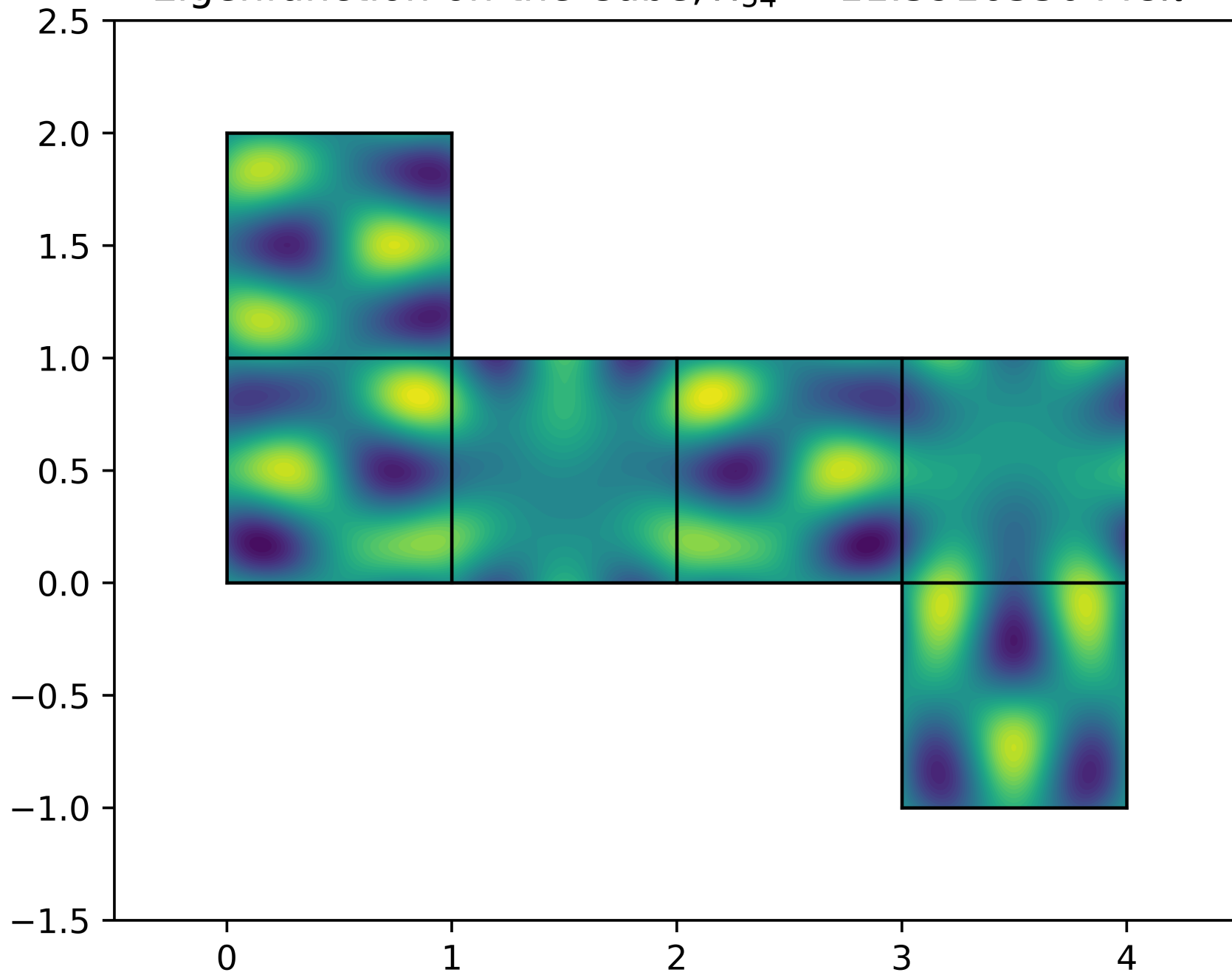
Eigenfunction on the Cube, \lambda_{54} = 11.3916330448\pi^2
