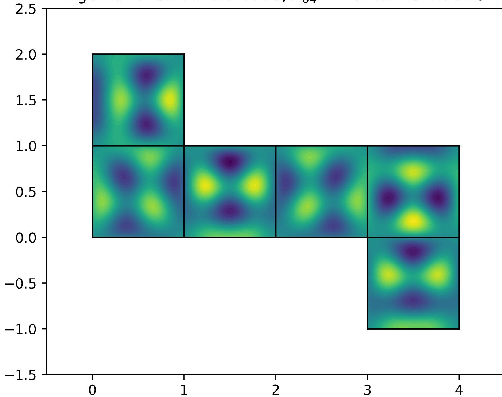
Eigenfunction on the Cube, \lambda_{64} = 13.1821342381\pi^2
