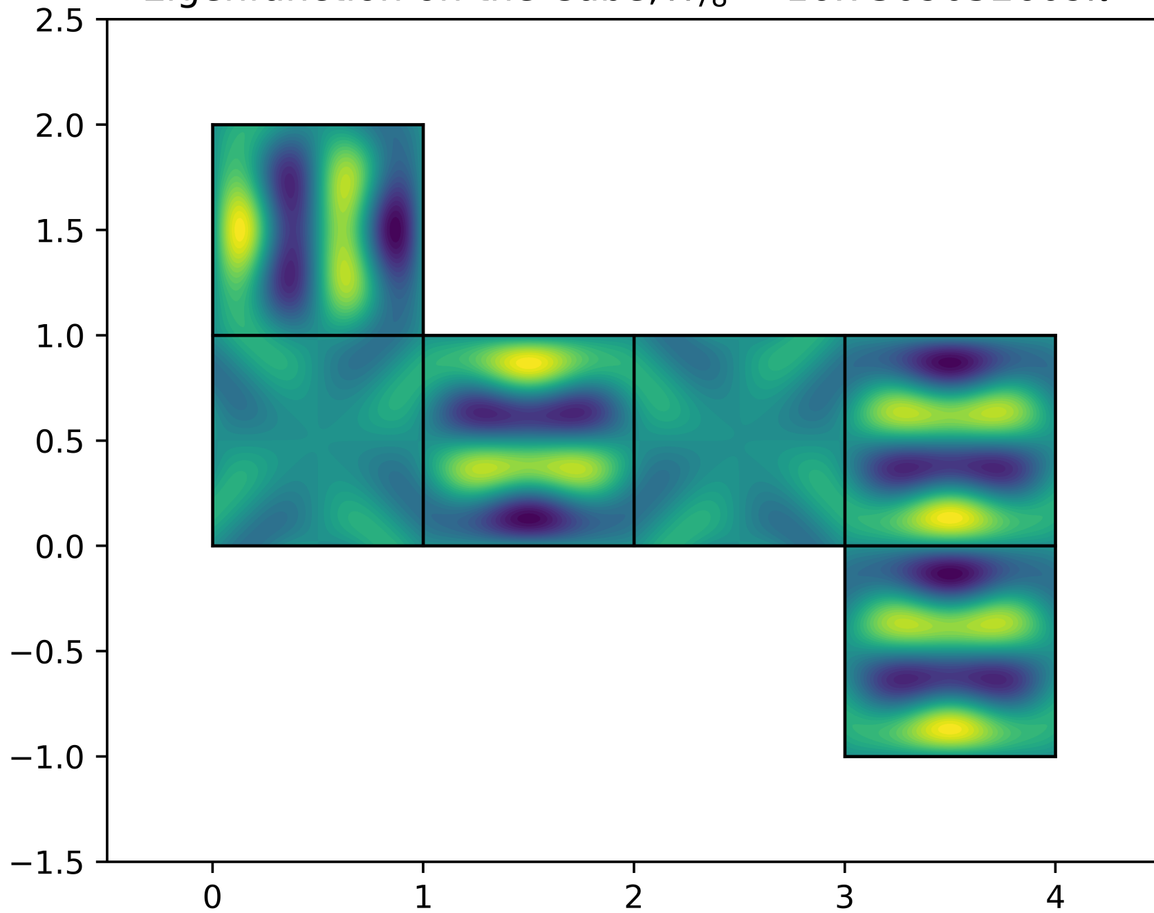
Eigenfunction on the Cube, \lambda_{78} = 16.7309052609\pi^2
