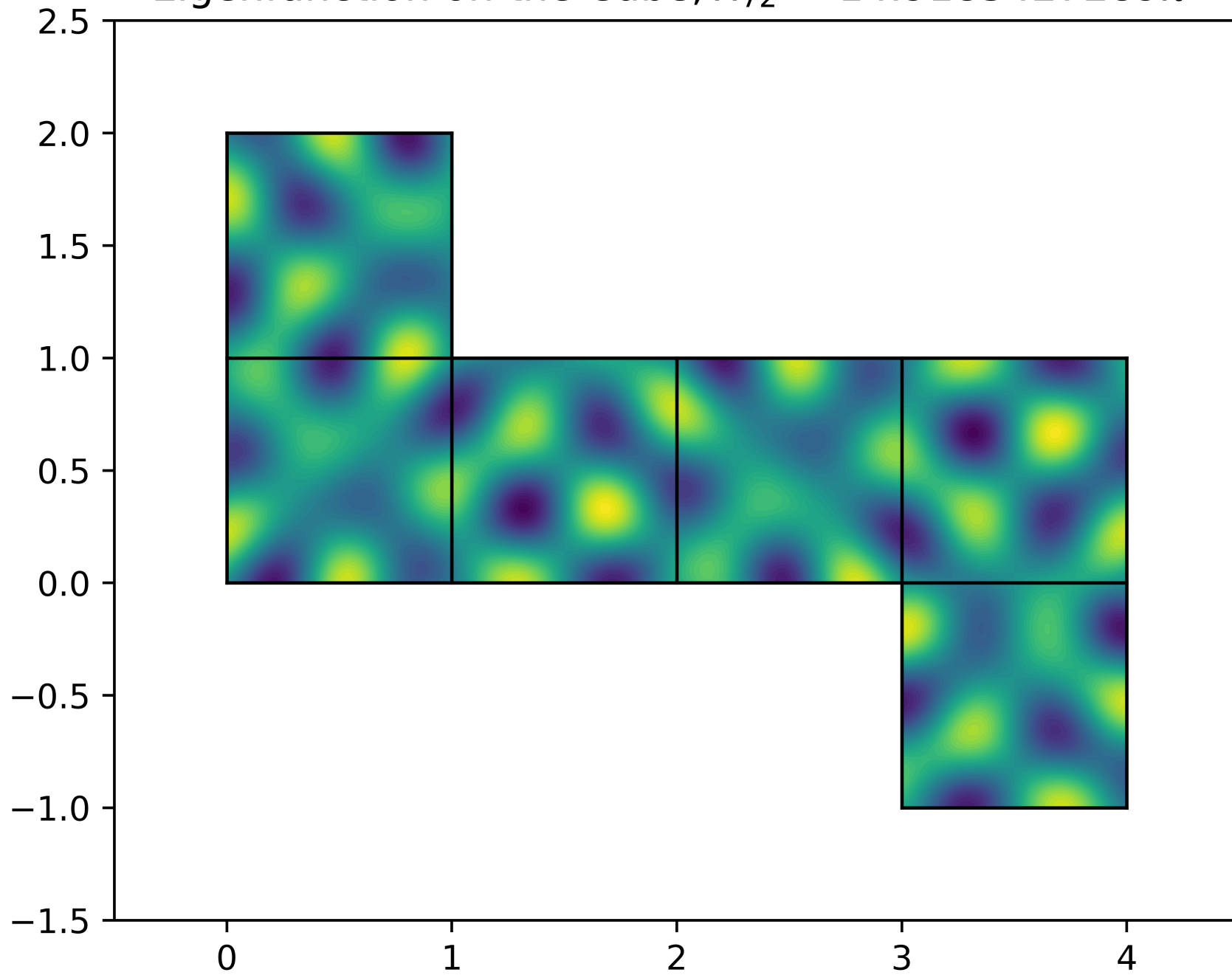
Eigenfunction on the Cube, \lambda_{72} = 14.9183427289\pi^2
