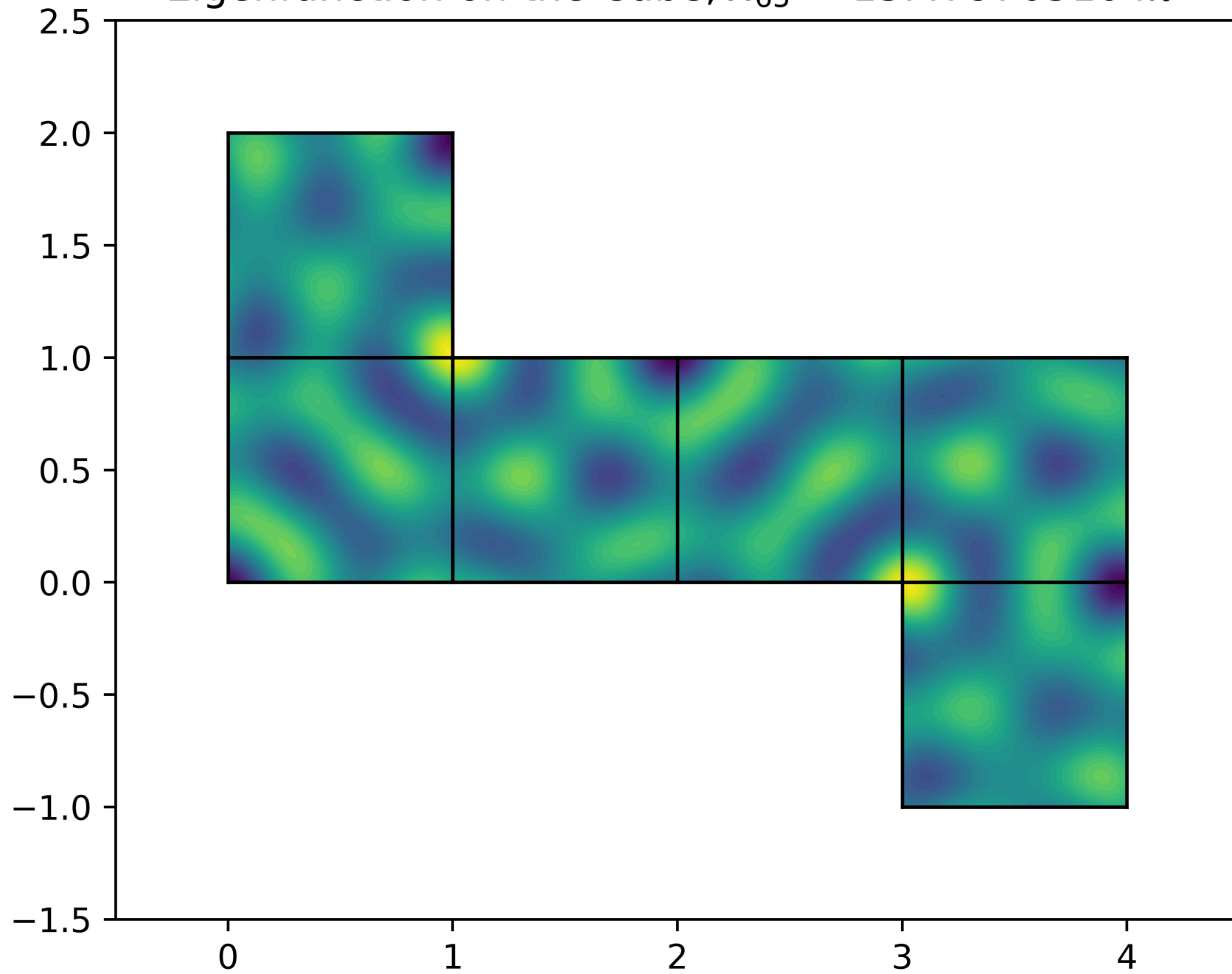
Eigenfunction on the Cube, \lambda_{65} = 13.479703104\pi^2
