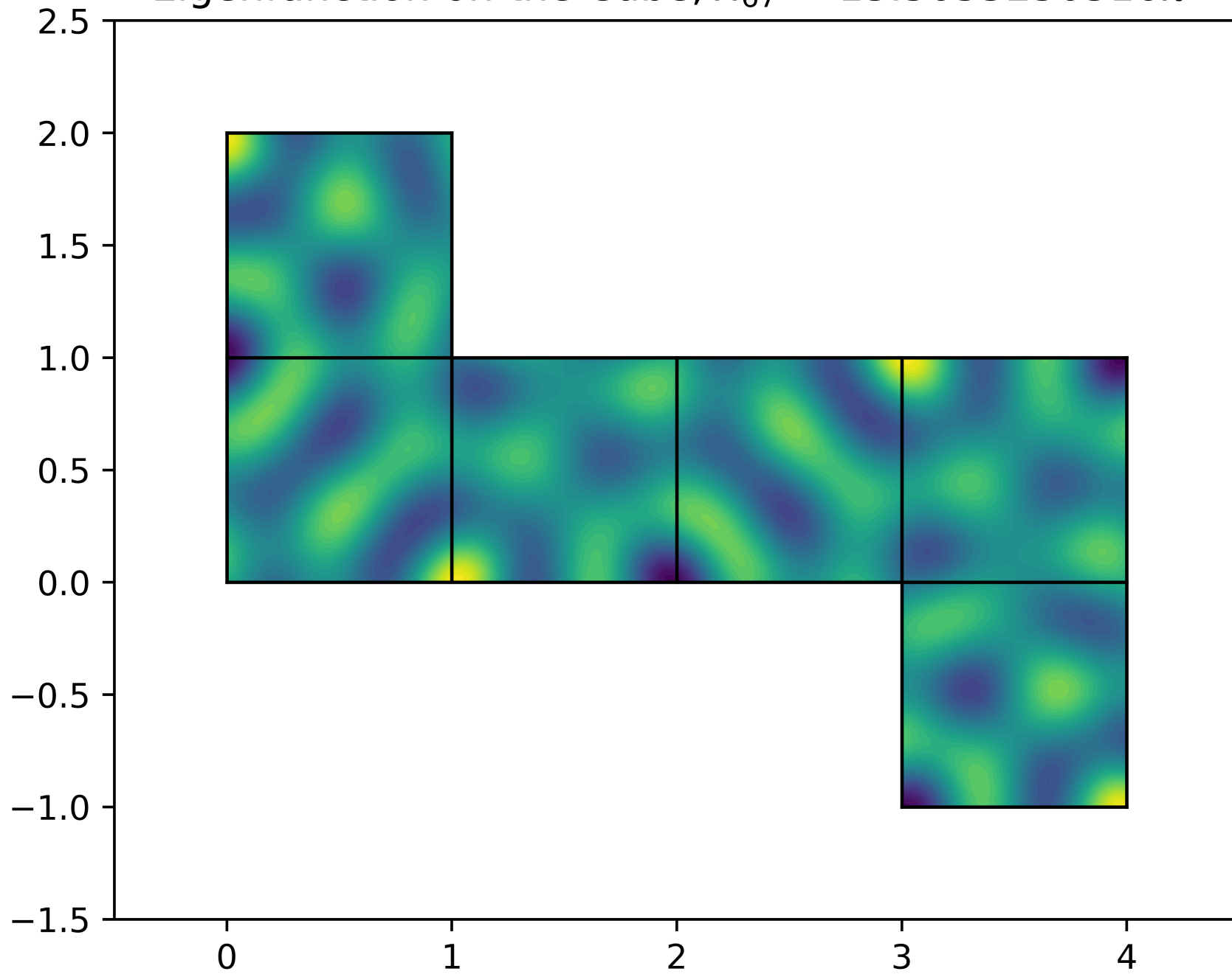
Eigenfunction on the Cube, \lambda_{67} = 13.5055250316\pi^2
