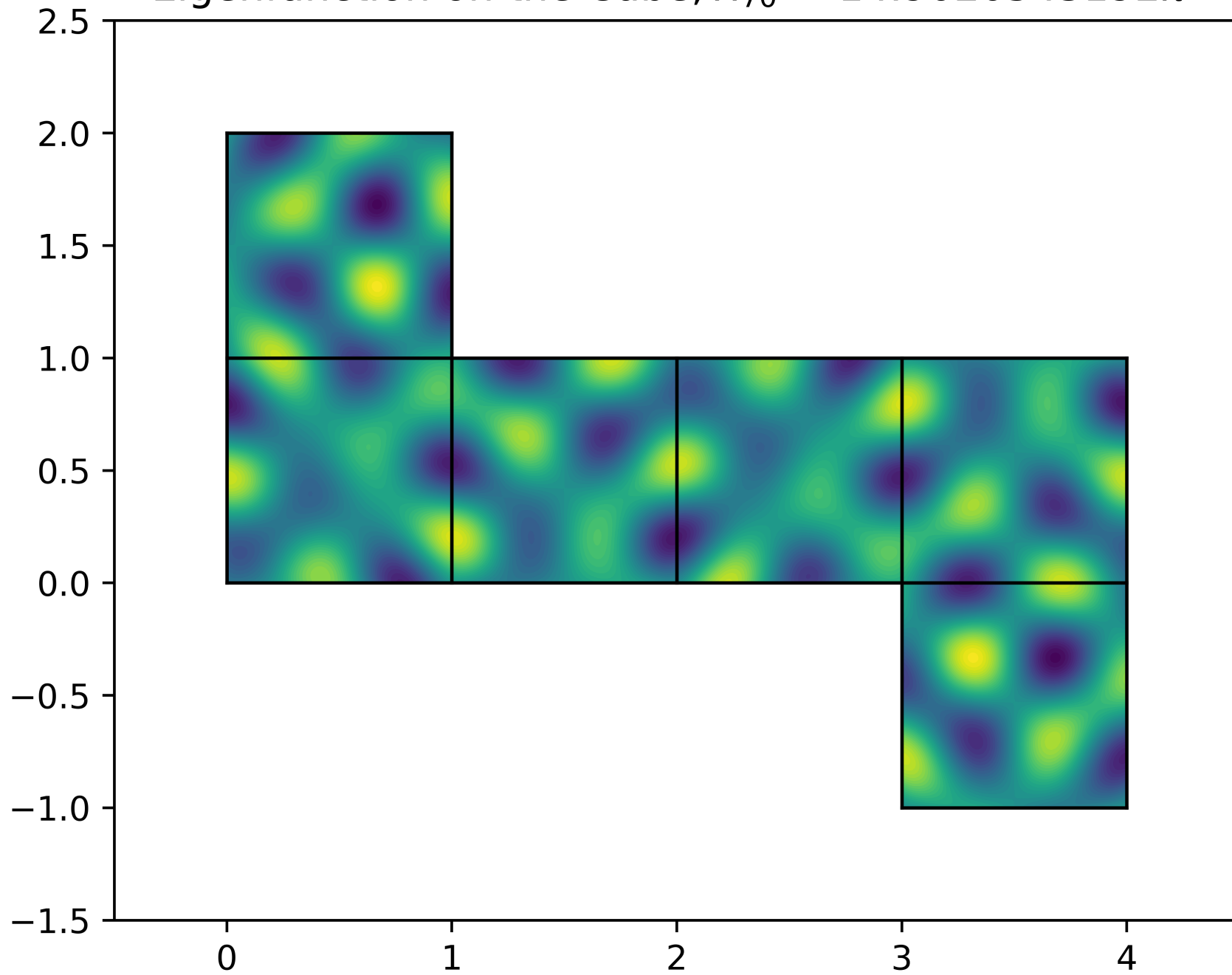
Eigenfunction on the Cube, \lambda_{70} = 14.9020543192\pi^2
