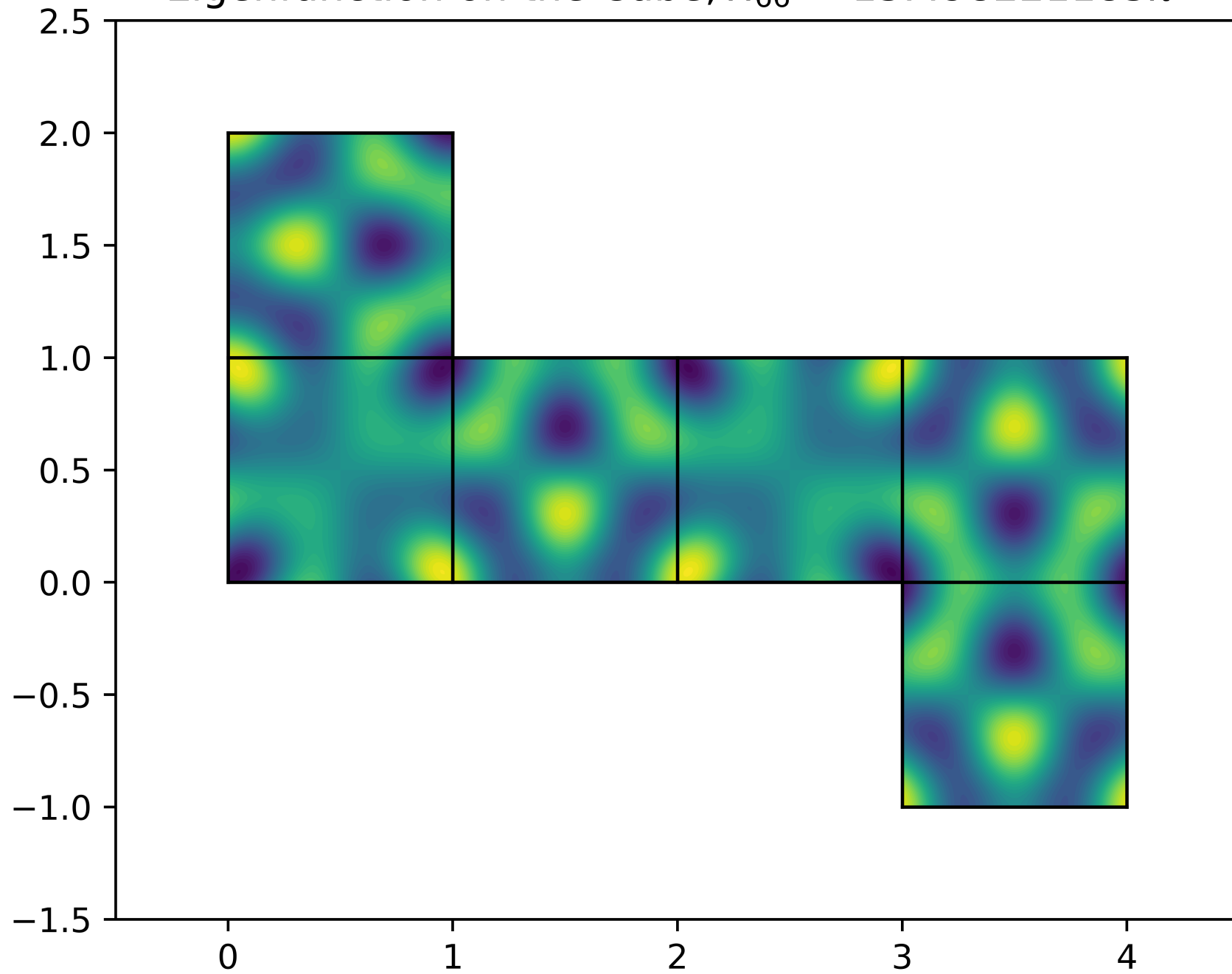
Eigenfunction on the Cube, \lambda_{66} = 13.498221183\pi^2
