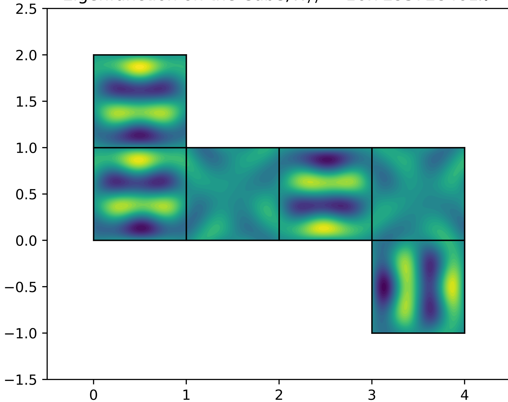
Eigenfunction on the Cube, \lambda_{77} = 16.7295728461\pi^2
