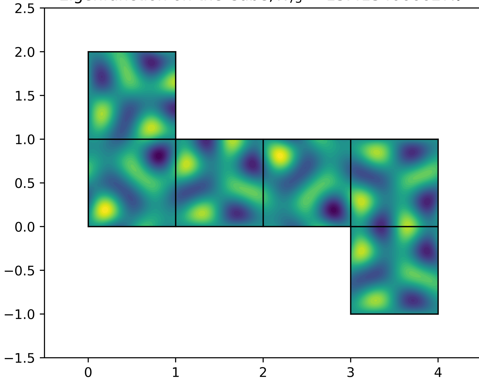
Eigenfunction on the Cube, \lambda_{73} = 15.4134066627\pi^2
