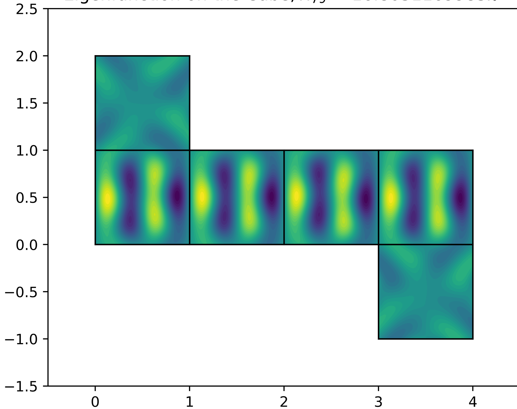
Eigenfunction on the Cube, \lambda_{79} = 16.8031169983\pi^2
