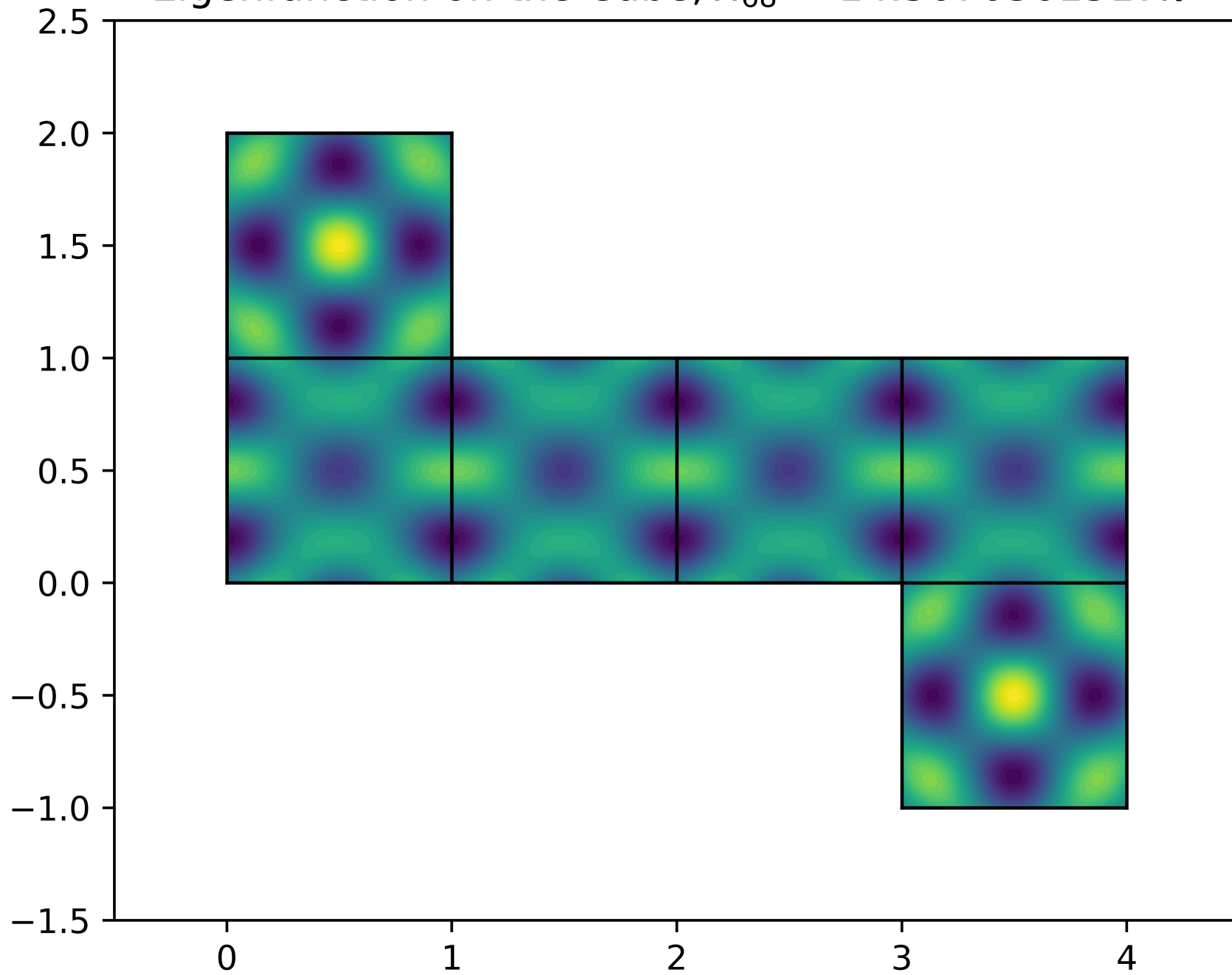
Eigenfunction on the Cube, \lambda_{68} = 14.5070361517\pi^2
