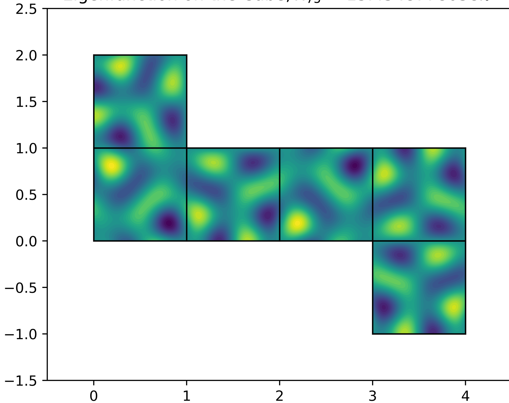
Eigenfunction on the Cube, \lambda_{75} = 15.4548778038\pi^2
