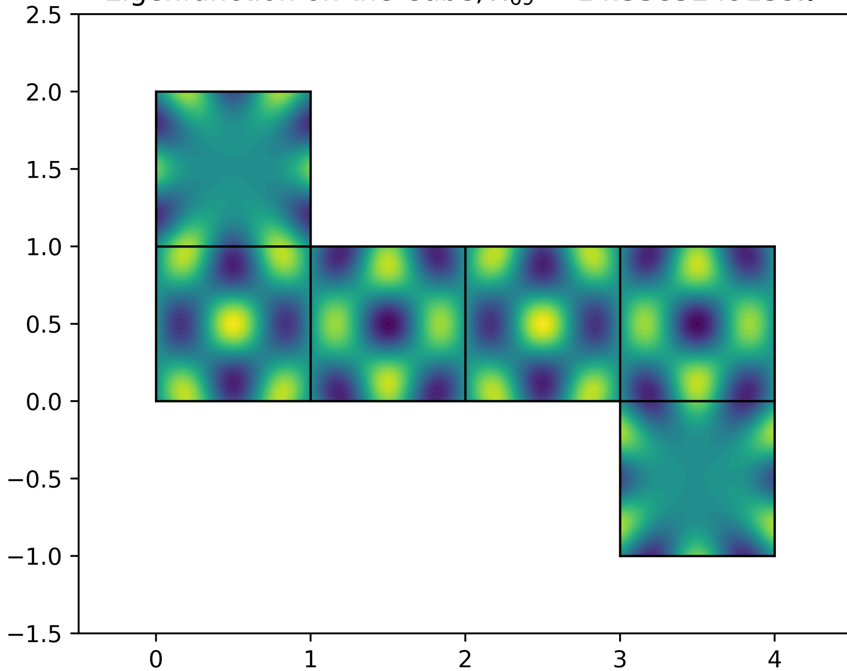
Eigenfunction on the Cube, \lambda_{69} = 14.5385249139\pi^2
