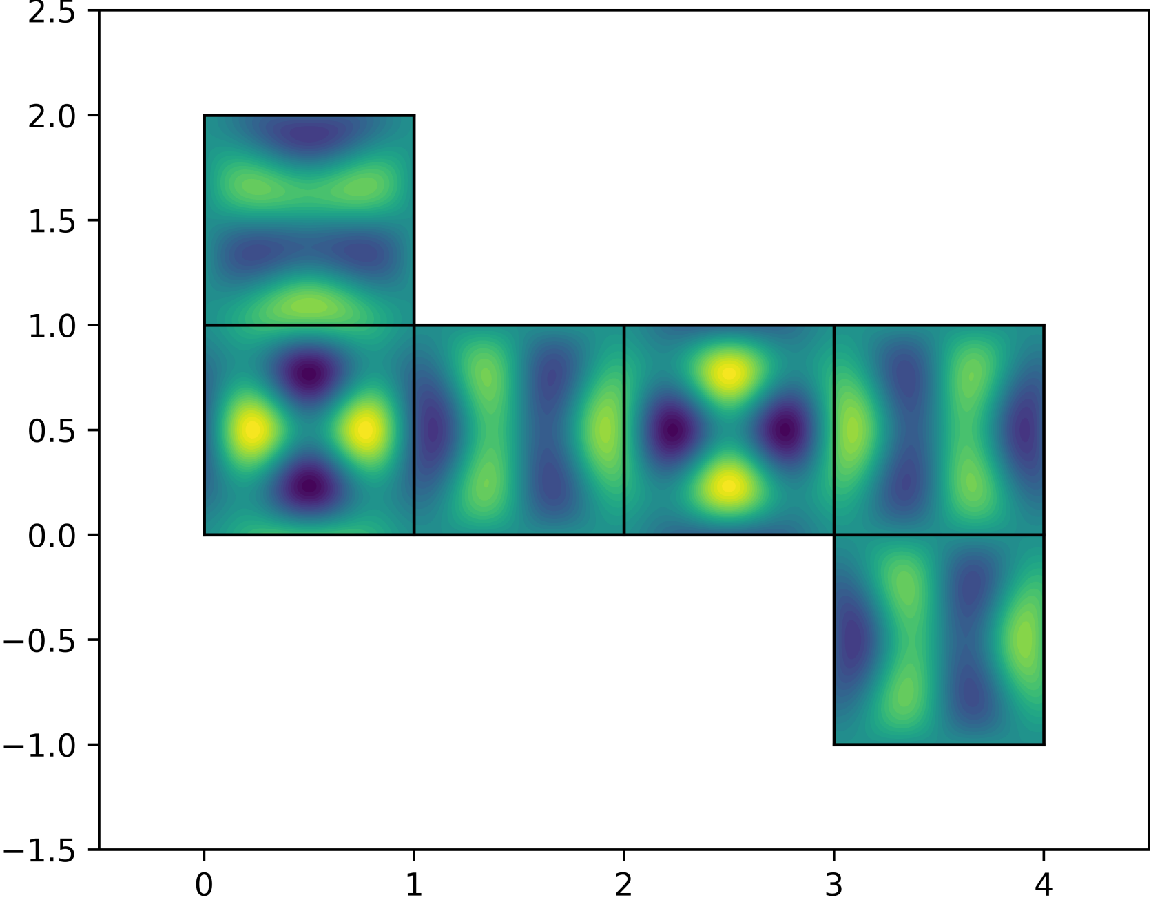
Eigenfunction on the Cube, \lambda_{63} = 13.169670311\pi^2
