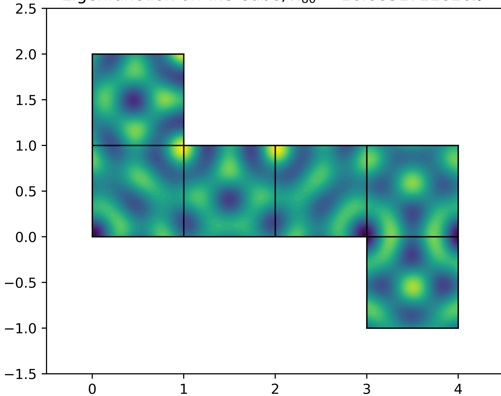
Eigenfunction on the Cube, \lambda_{80} = 16.8851722826\pi^2
