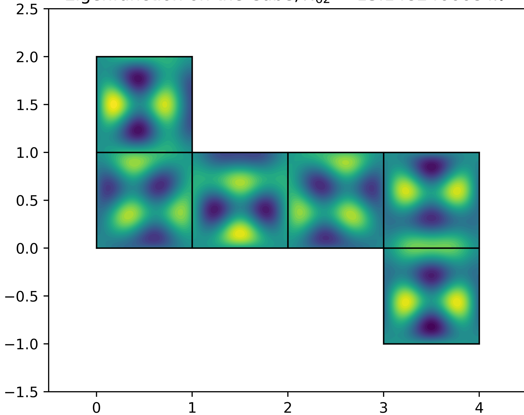
Eigenfunction on the Cube, \lambda_{62} = 13.1482466684\pi^2
