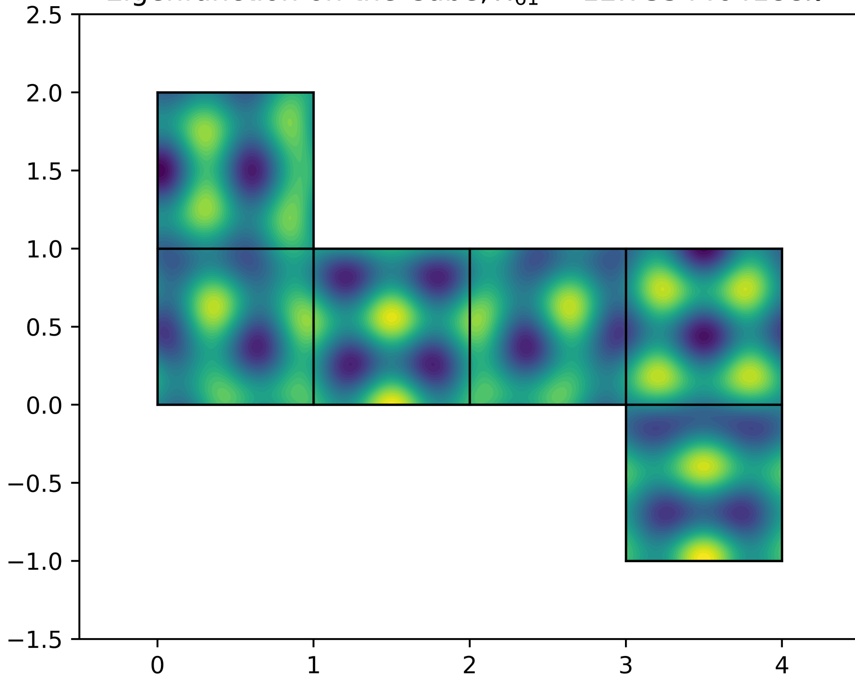
Eigenfunction on the Cube, \lambda_{61} = 12.7354464188\pi^2
