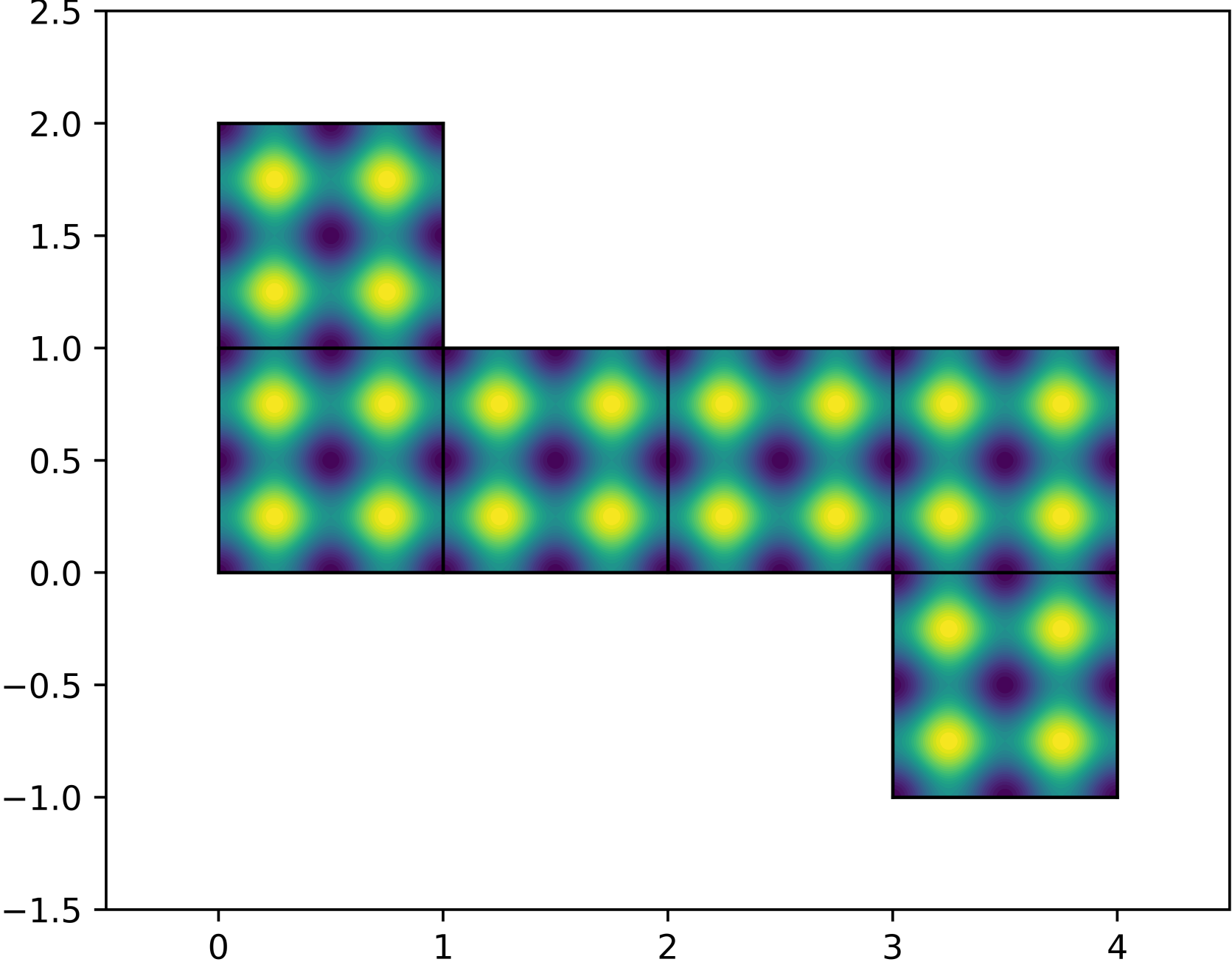
Eigenfunction on the Cube, \lambda_{76} = 16.010713907\pi^2
