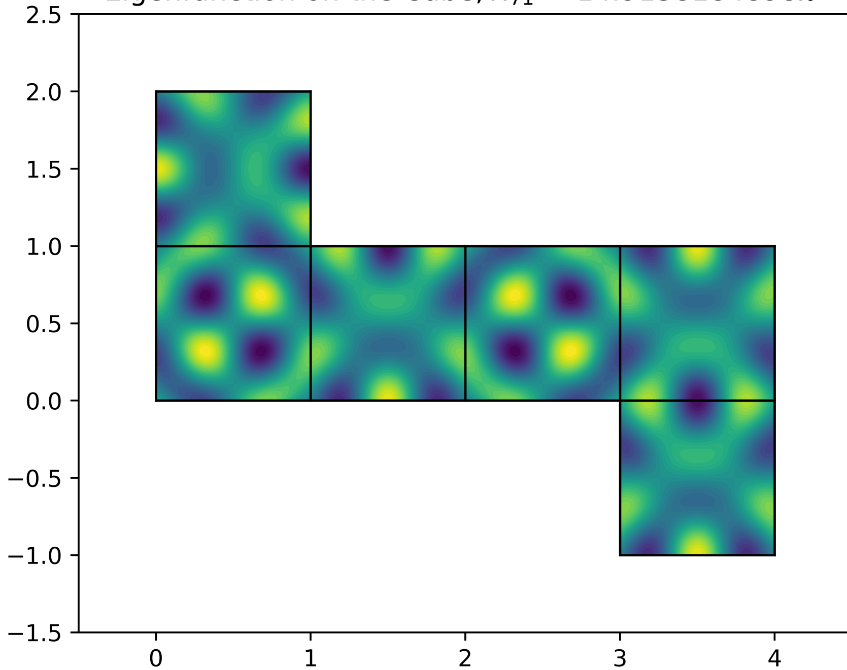
Eigenfunction on the Cube, \lambda_{71} = 14.9138184898\pi^2
