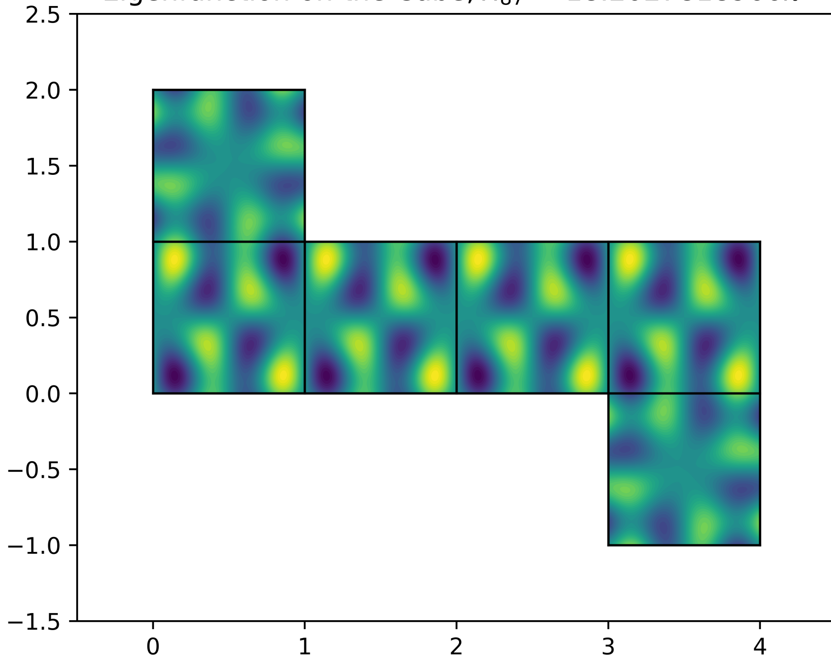
Eigenfunction on the Cube, \lambda_{87} = 18.2027818966\pi^2
