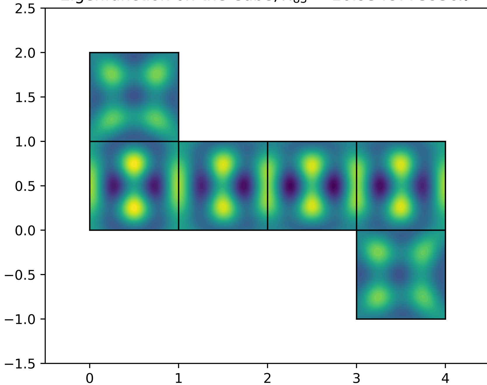
Eigenfunction on the Cube, \lambda_{83} = 16.9348773936\pi^2
