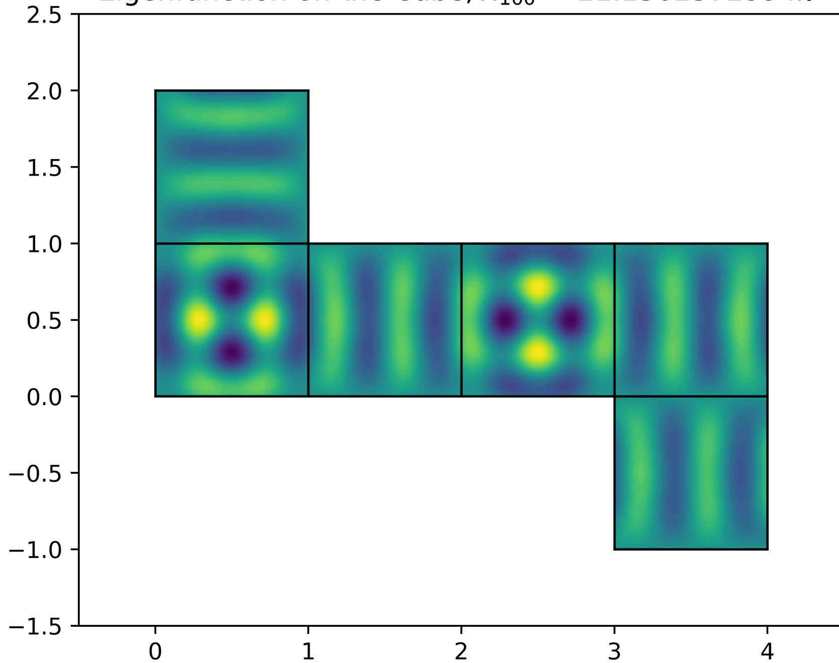
Eigenfunction on the Cube, \lambda_{100} = 21.1502572994\pi^2
