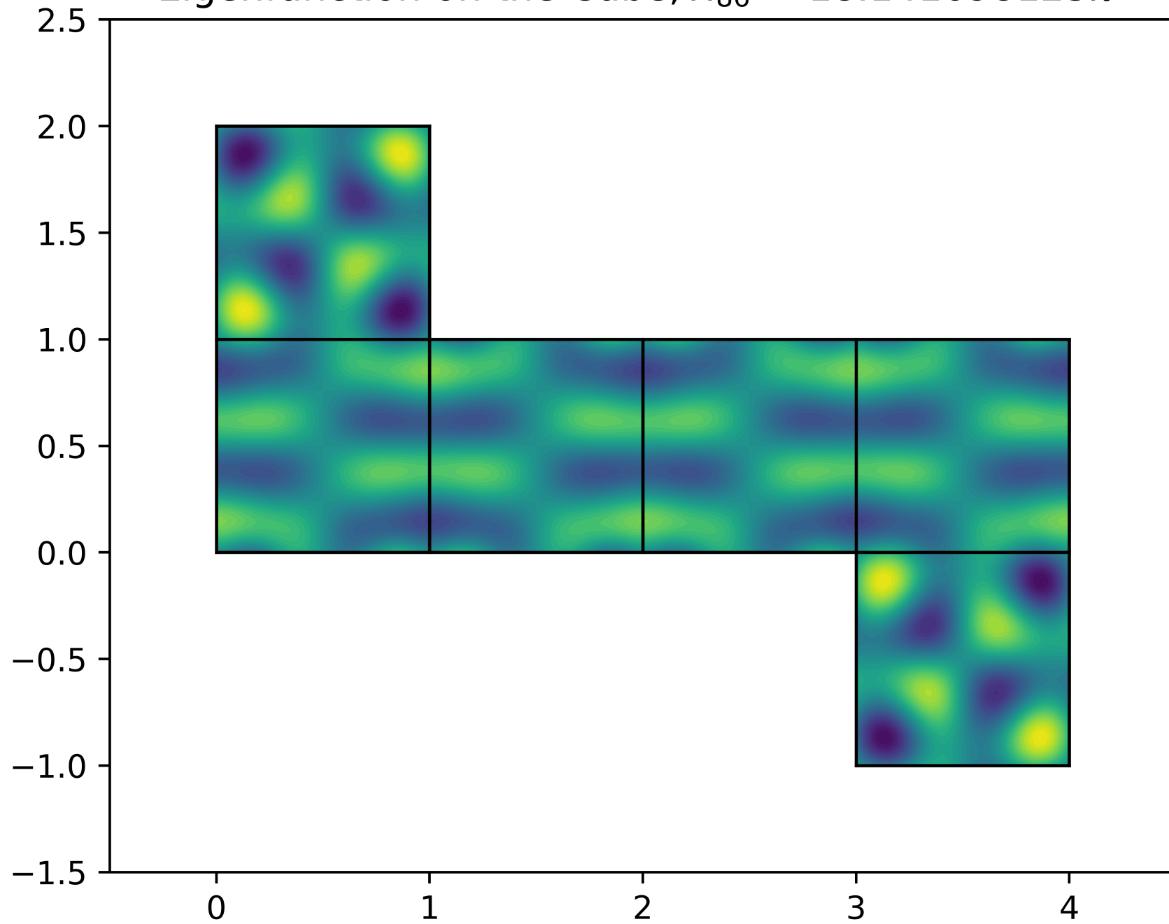
Eigenfunction on the Cube, \lambda_{86} = 18.141698123\pi^2
