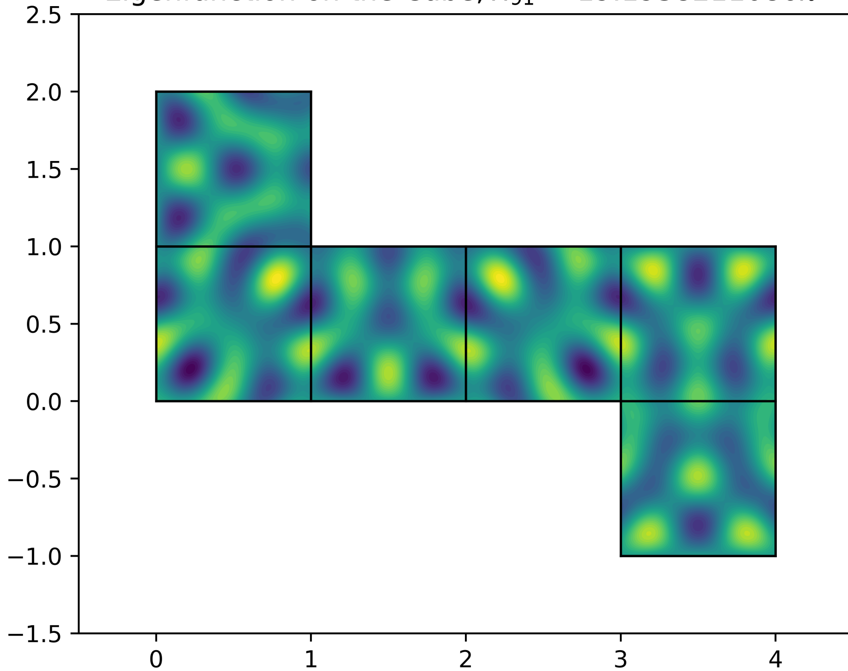
Eigenfunction on the Cube, \lambda_{91} = 19.1938211086\pi^2
