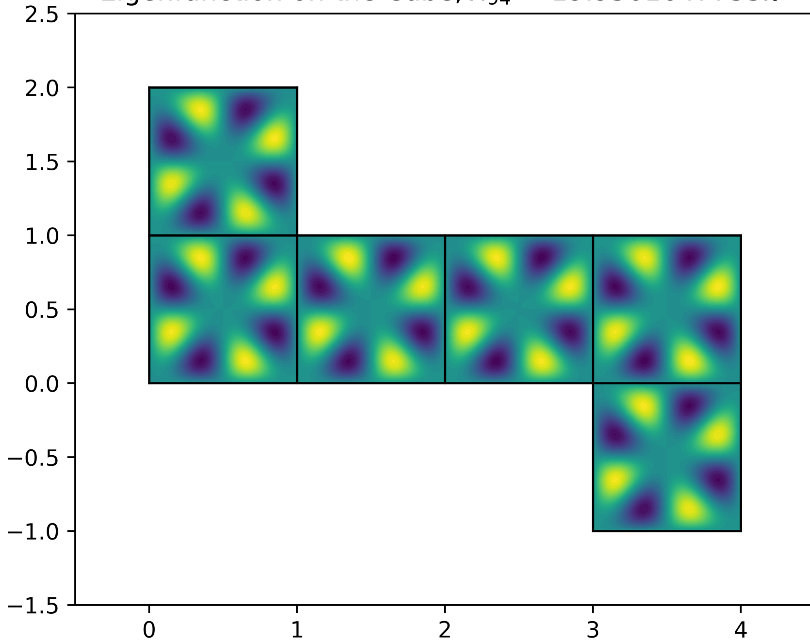
Eigenfunction on the Cube, \lambda_{94} = 19.9501647755\pi^2
