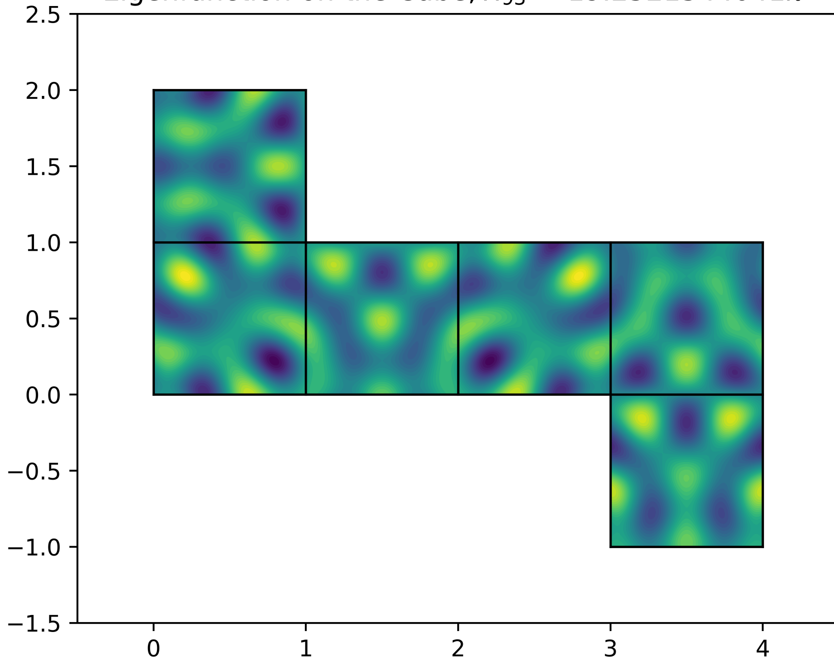
Eigenfunction on the Cube, \lambda_{93} = 19.2521544041\pi^2
