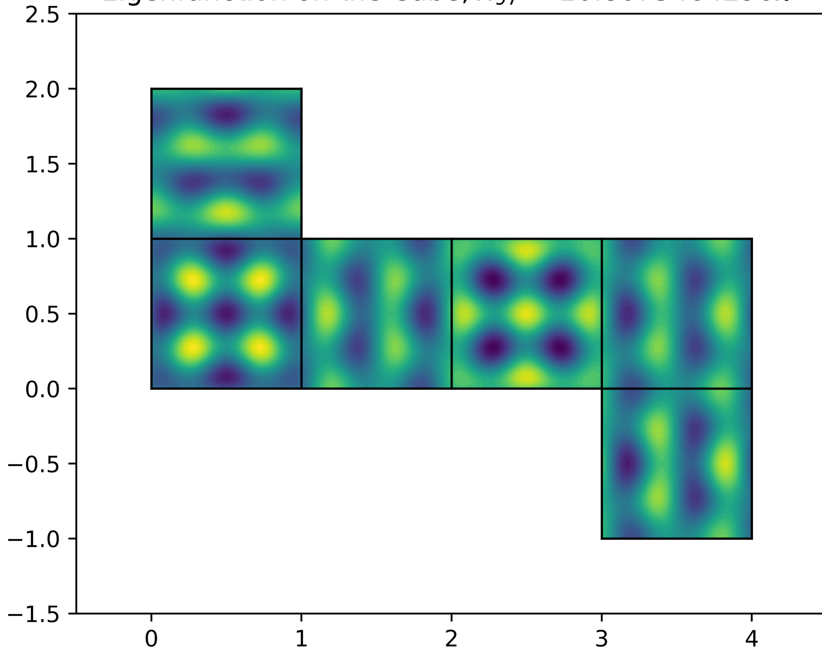
Eigenfunction on the Cube, \lambda_{97} = 20.8075464296\pi^2
