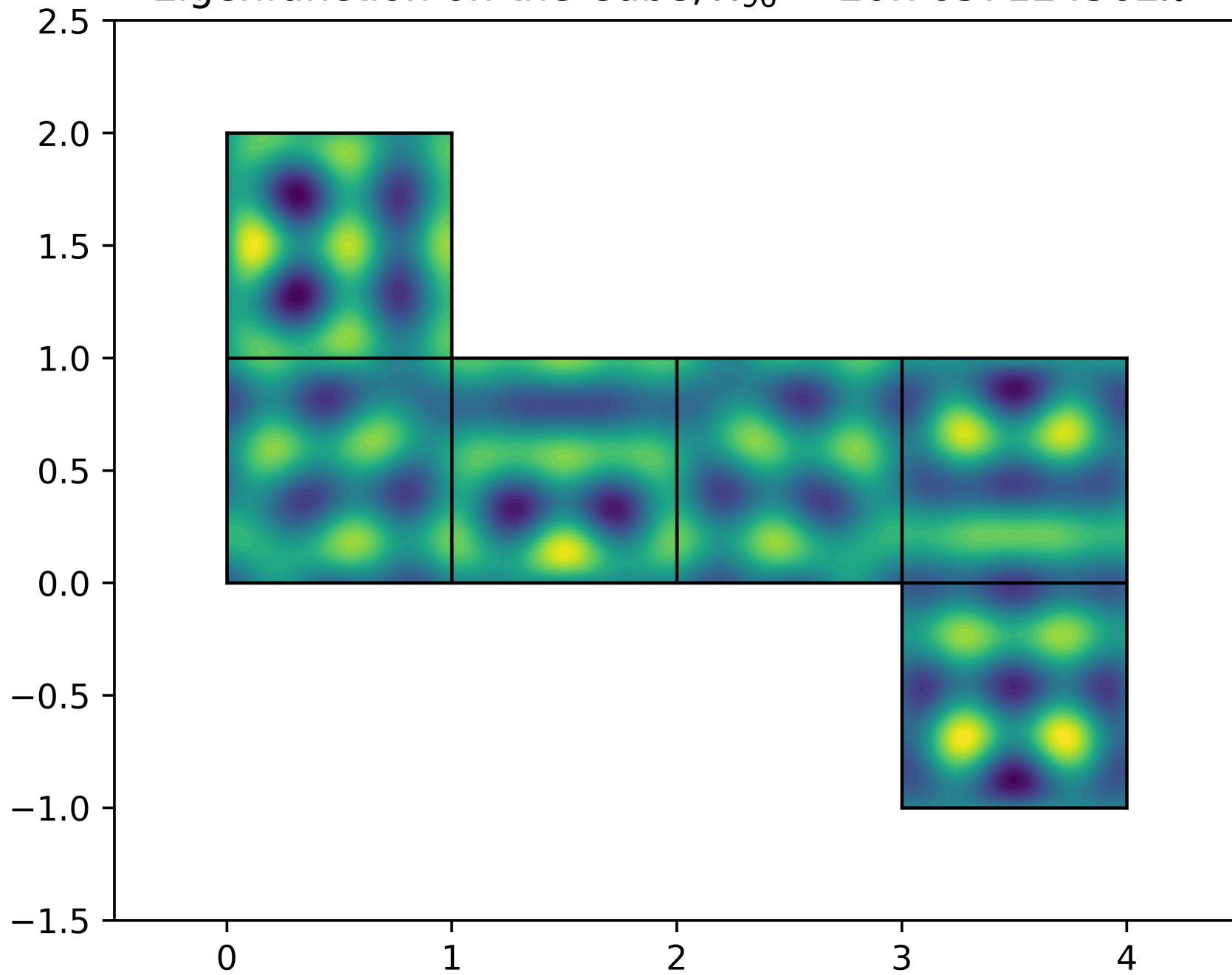
Eigenfunction on the Cube, \lambda_{96} = 20.7657124562\pi^2
