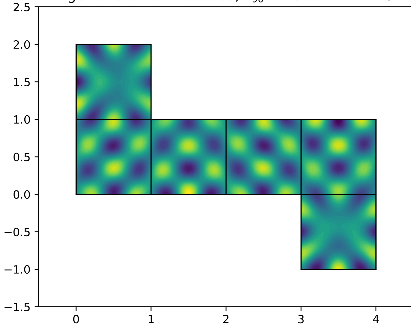
Eigenfunction on the Cube, \lambda_{90} = 18.602211711\pi^2
