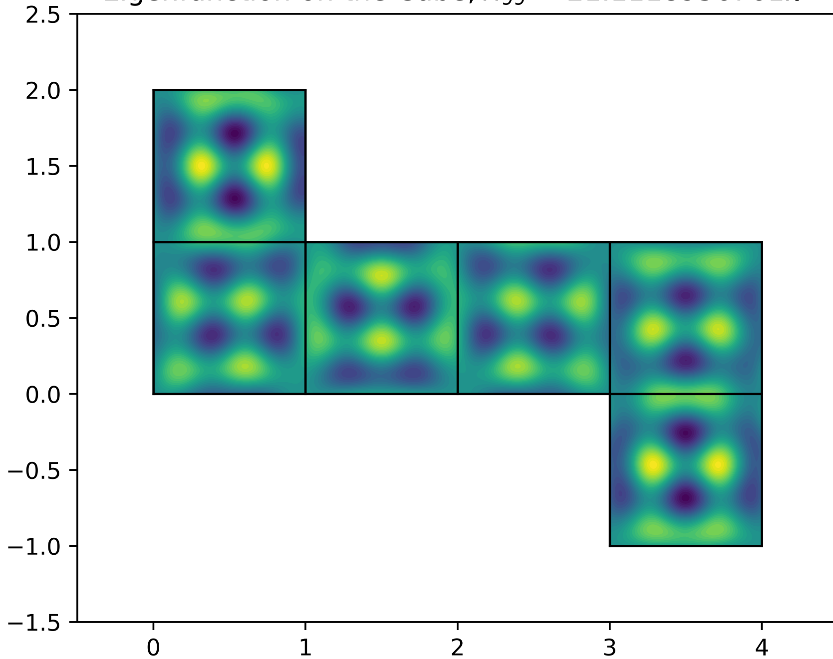
Eigenfunction on the Cube, \lambda_{99} = 21.1118956761\pi^2
