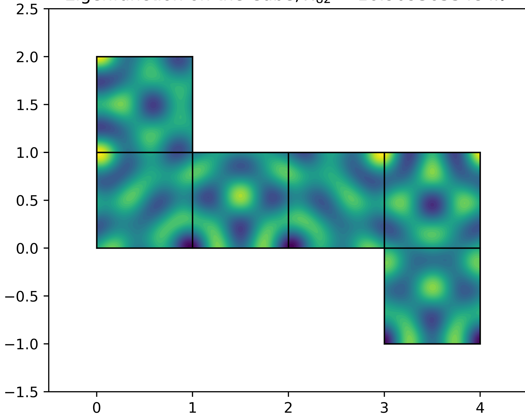
Eigenfunction on the Cube, \lambda_{82} = 16.9093655484\pi^2
