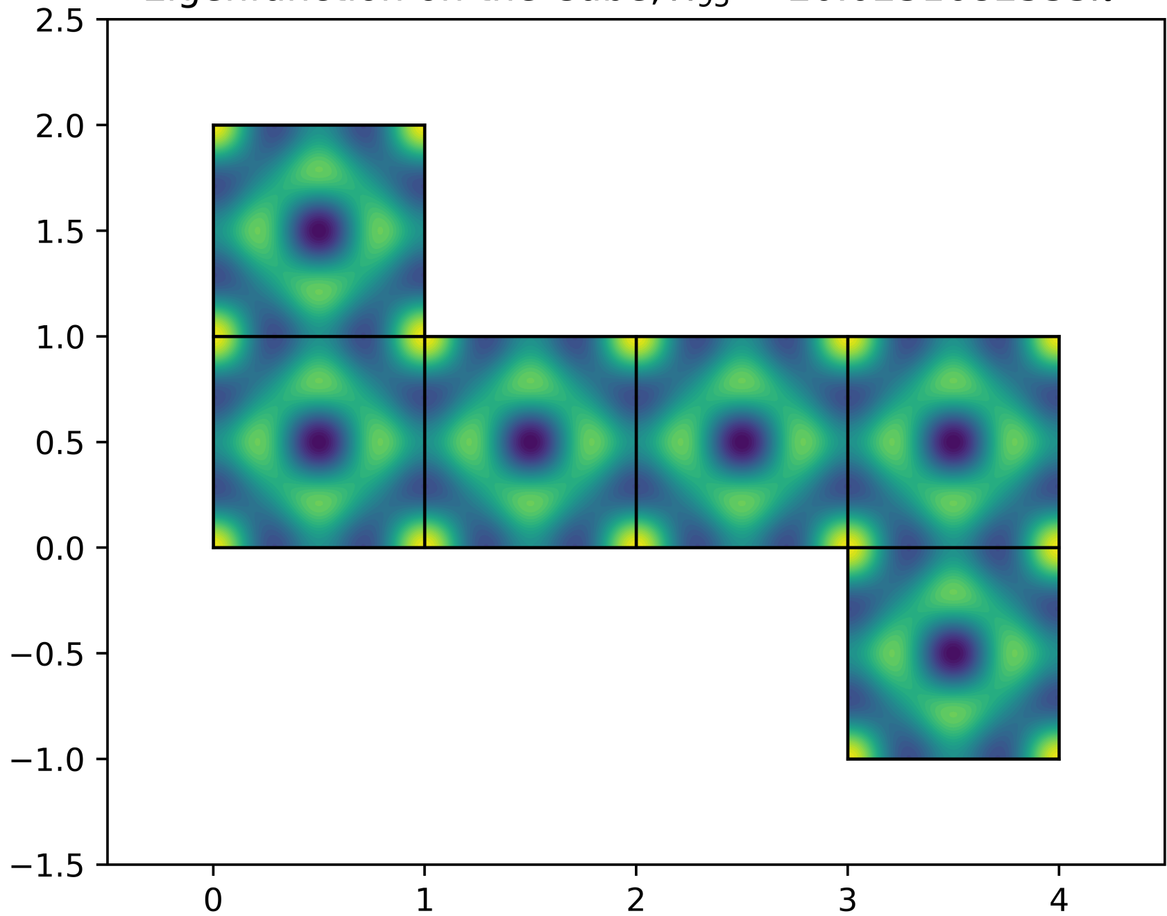
Eigenfunction on the Cube, \lambda_{95} = 20.0231682533\pi^2
