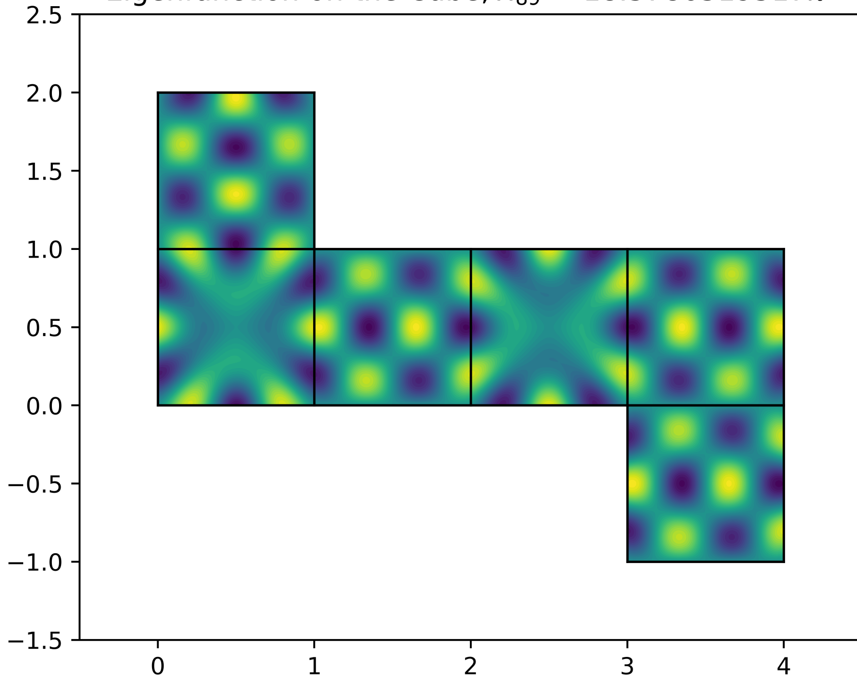
Eigenfunction on the Cube, \lambda_{89} = 18.5786319517\pi^2
