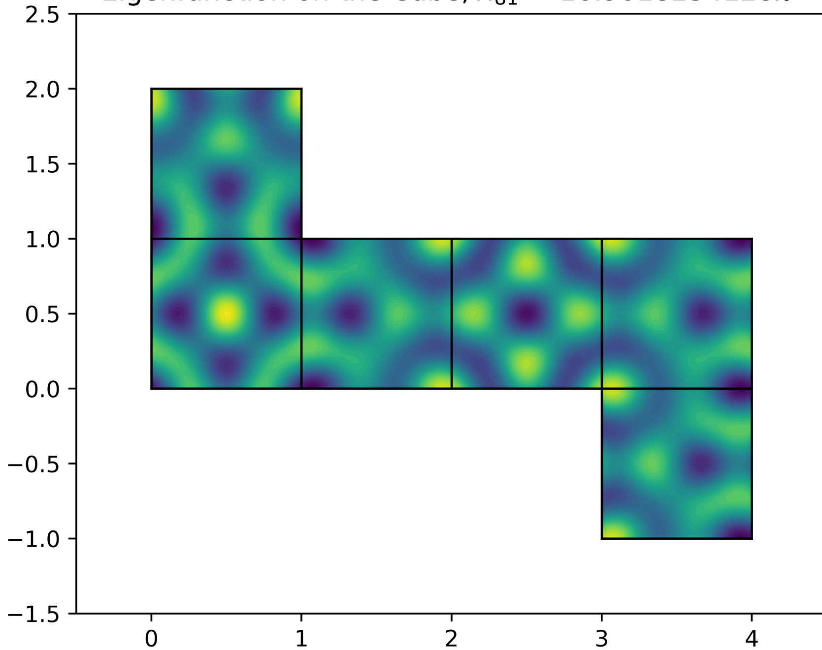
Eigenfunction on the Cube, \lambda_{81} = 16.9018254128\pi^2
