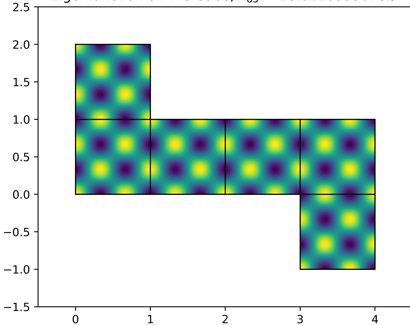
Eigenfunction on the Cube, \lambda_{85} = 18.0216933078\pi^2
