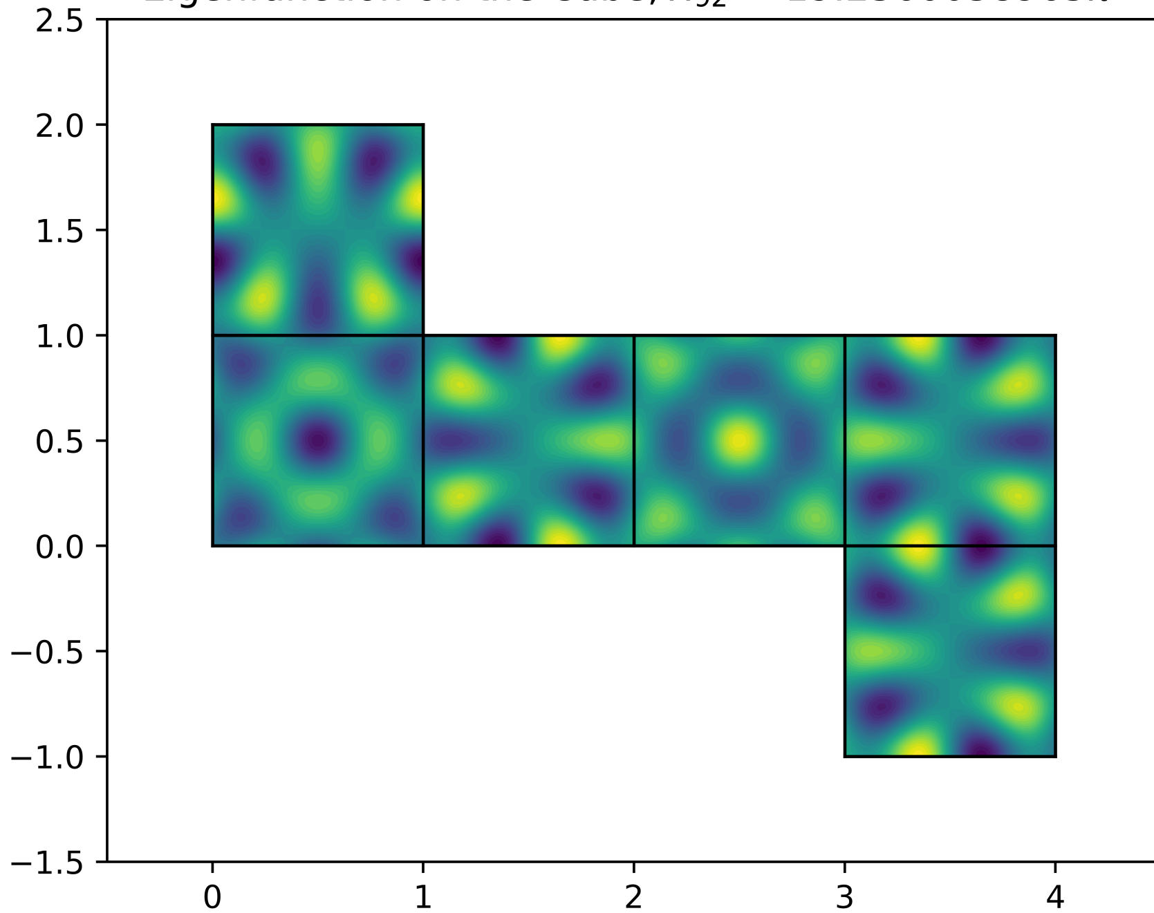
Eigenfunction on the Cube, \lambda_{92} = 19.2360038965\pi^2
