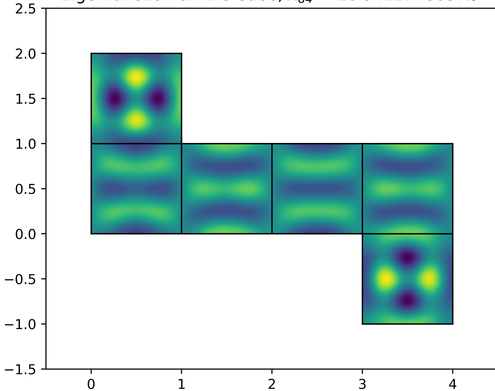
Eigenfunction on the Cube, \lambda_{84} = 16.9412778037\pi^2
