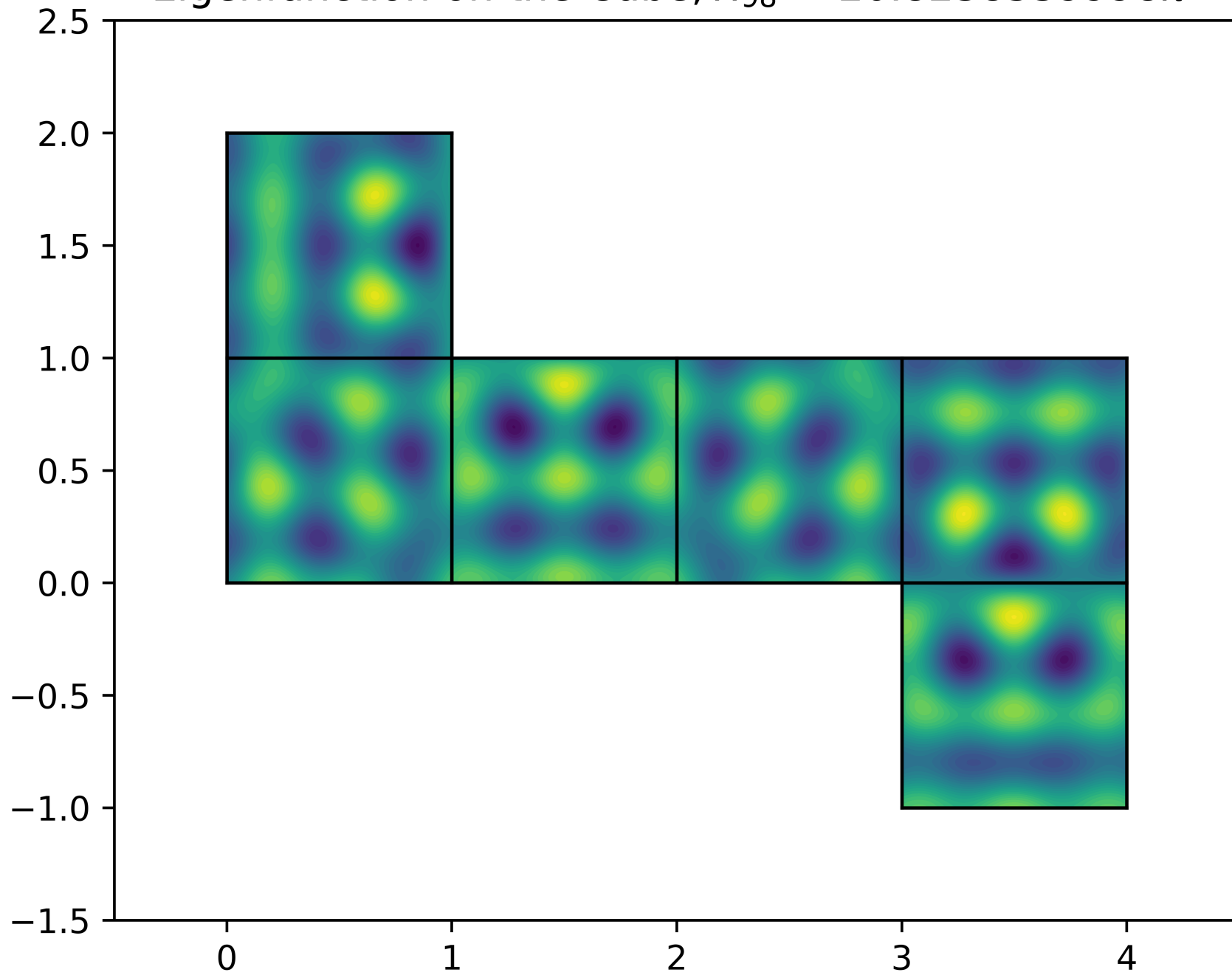
Eigenfunction on the Cube, \lambda_{98} = 20.8238539998\pi^2
