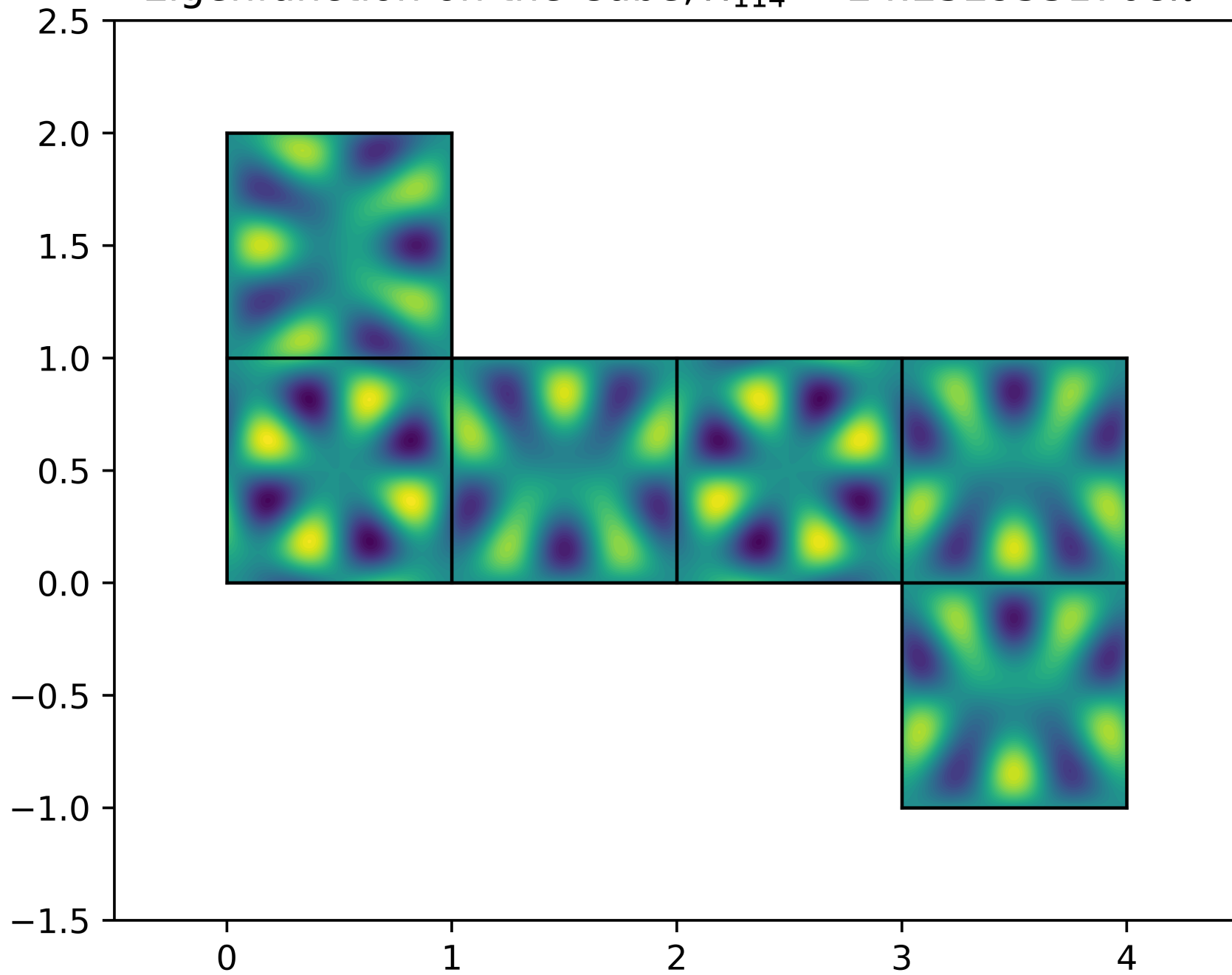
Eigenfunction on the Cube, \lambda_{114} = 24.2529531708\pi^2
