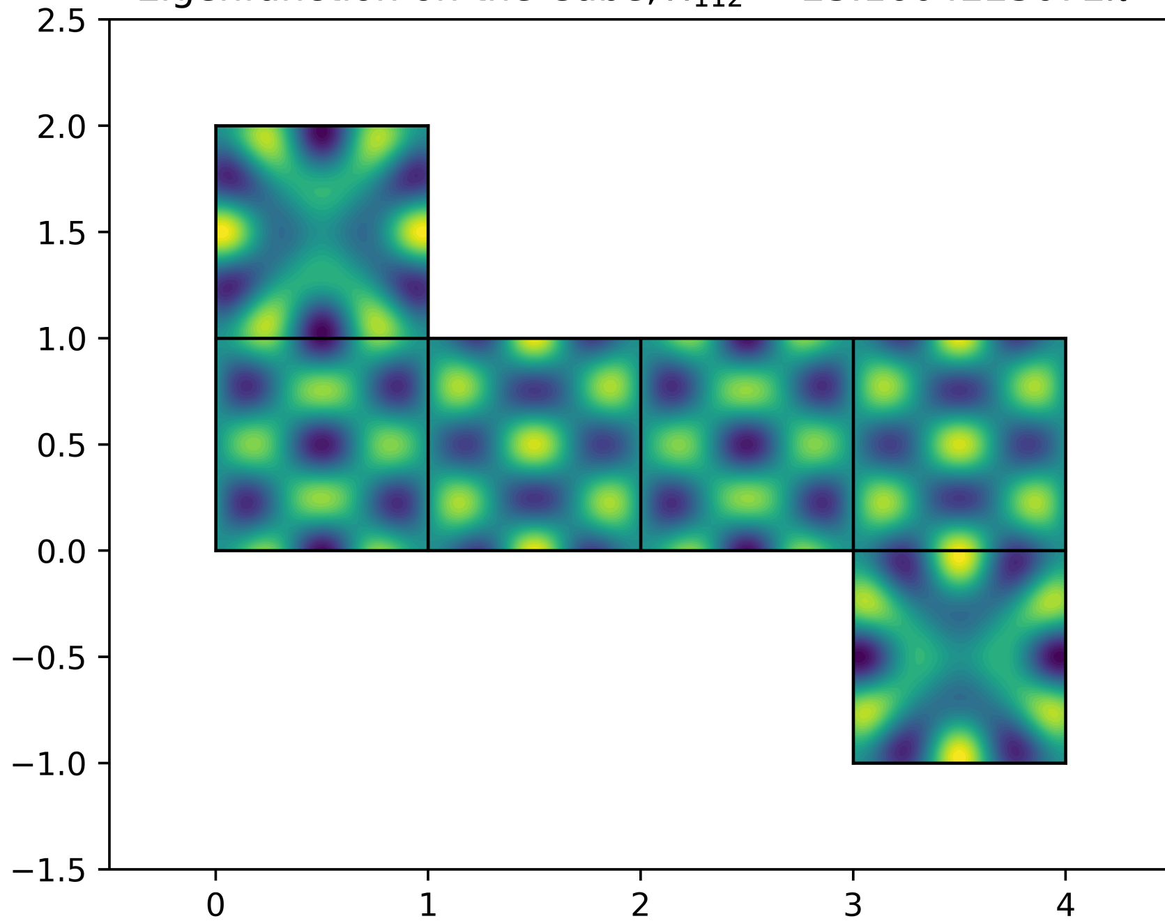
Eigenfunction on the Cube, \lambda_{112} = 23.1604223072\pi^2
