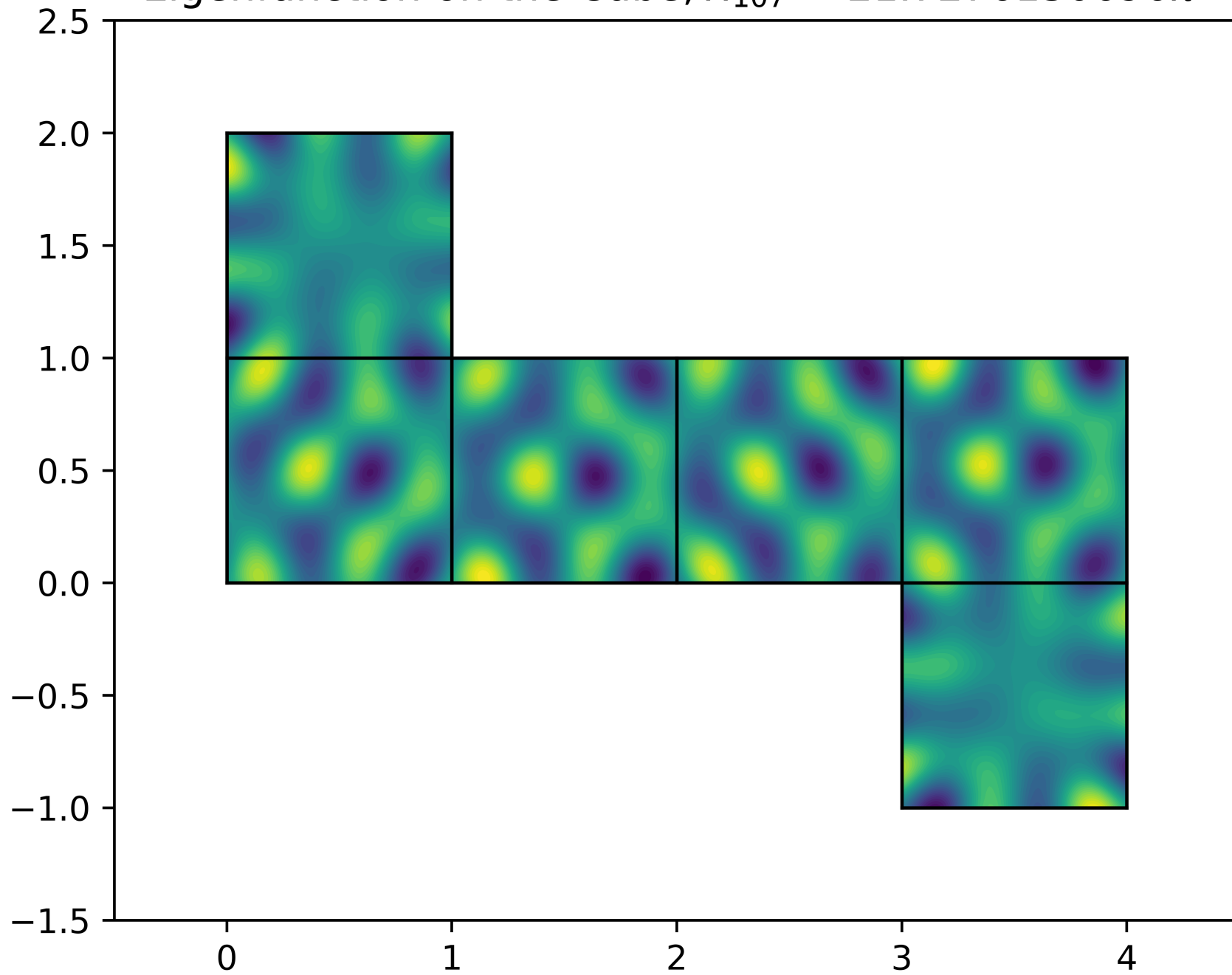
Eigenfunction on the Cube, \lambda_{107} = 21.7276130696\pi^2
