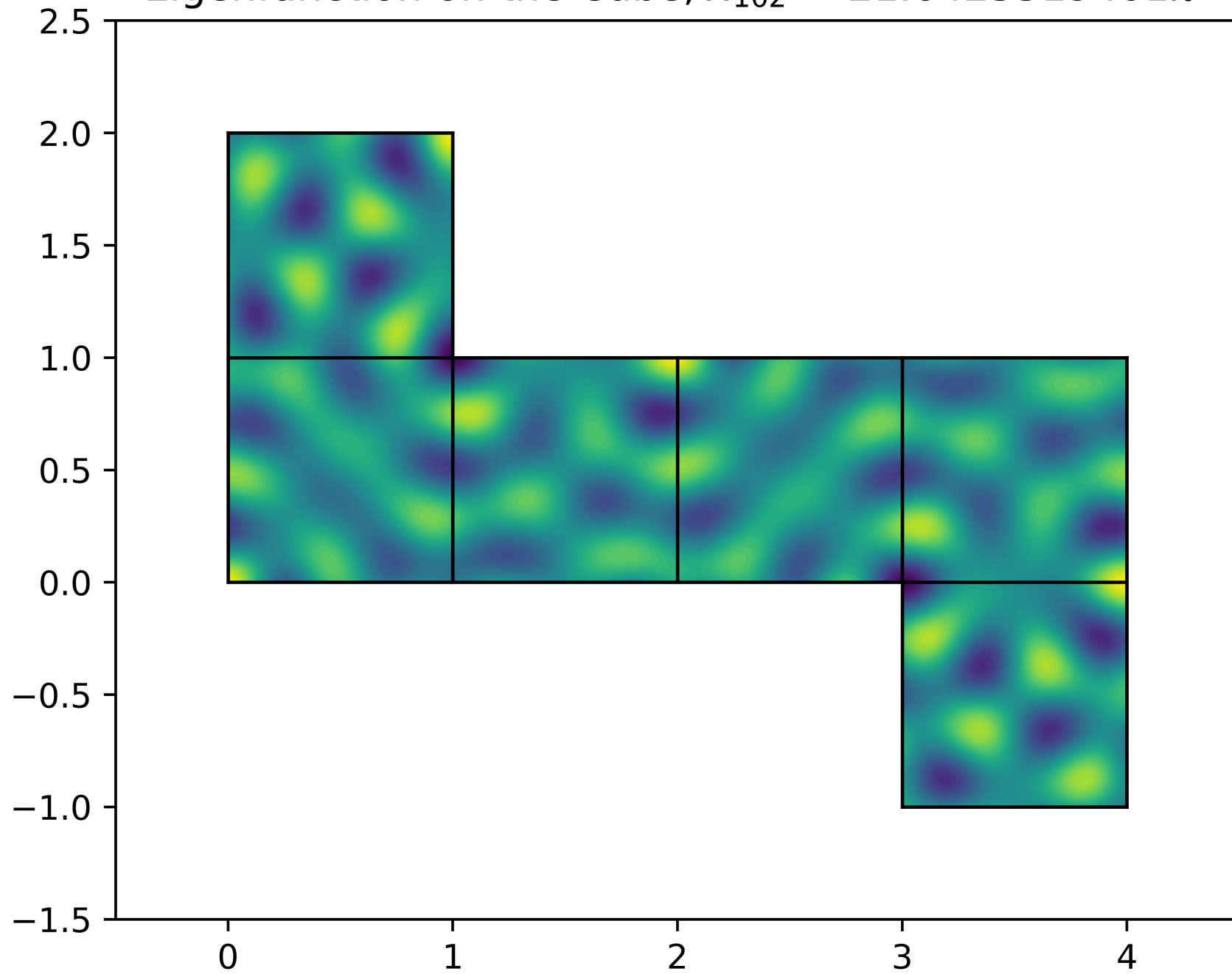
Eigenfunction on the Cube, \lambda_{102} = 21.6425519401\pi^2
