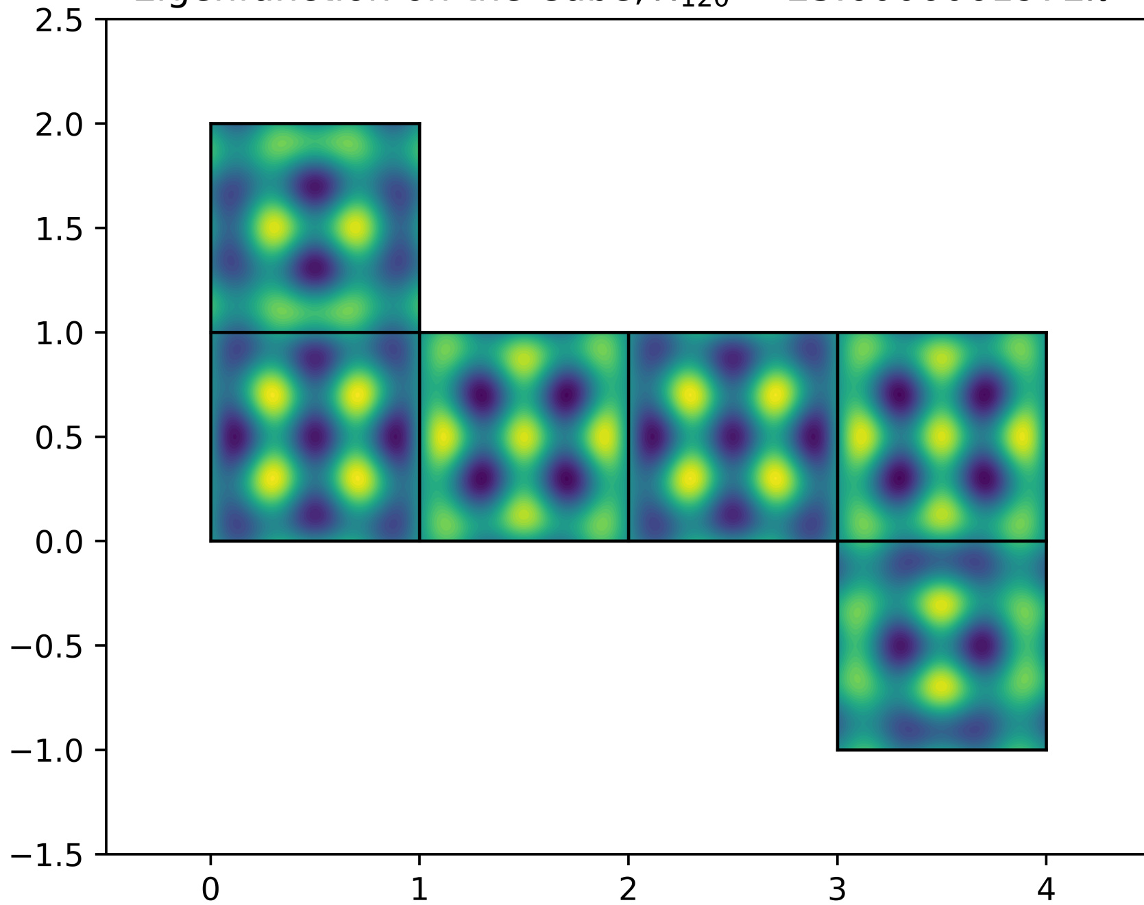
Eigenfunction on the Cube, \lambda_{120} = 25.6006061972\pi^2
