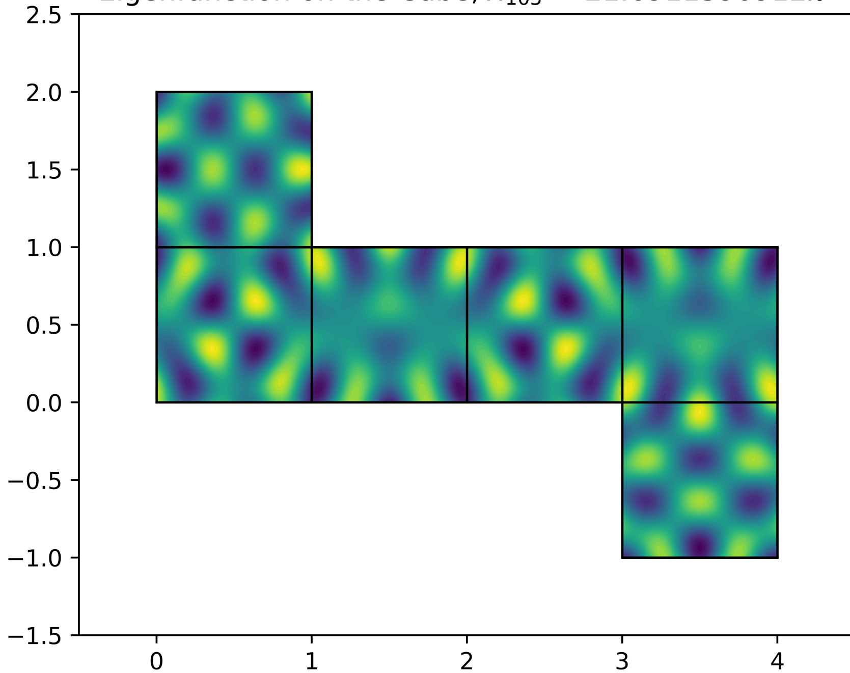
Eigenfunction on the Cube, \lambda_{105} = 21.6911590912\pi^2
