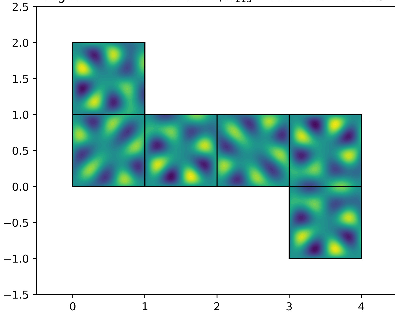
Eigenfunction on the Cube, \lambda_{113} = 24.2233737848\pi^2
