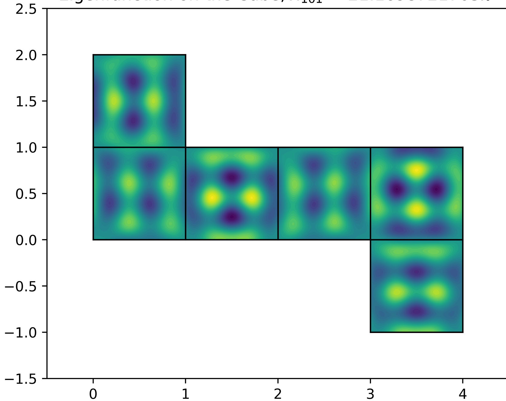
Eigenfunction on the Cube, \lambda_{101} = 21.1698721703\pi^2
