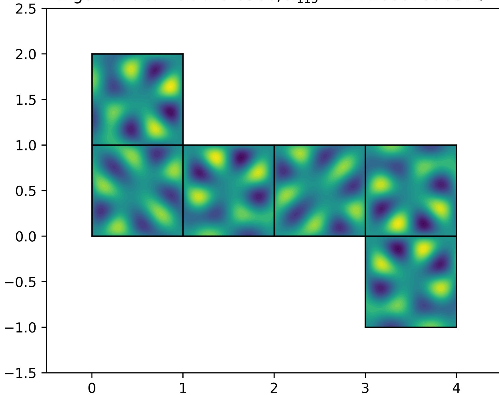
Eigenfunction on the Cube, \lambda_{115} = 24.2835733637\pi^2
