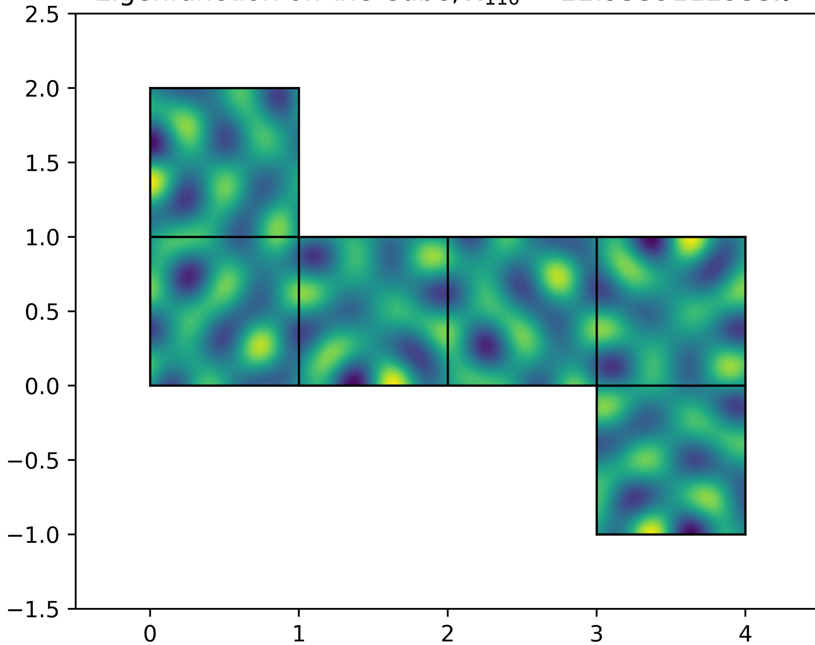
Eigenfunction on the Cube, \lambda_{110} = 22.9539112935\pi^2
