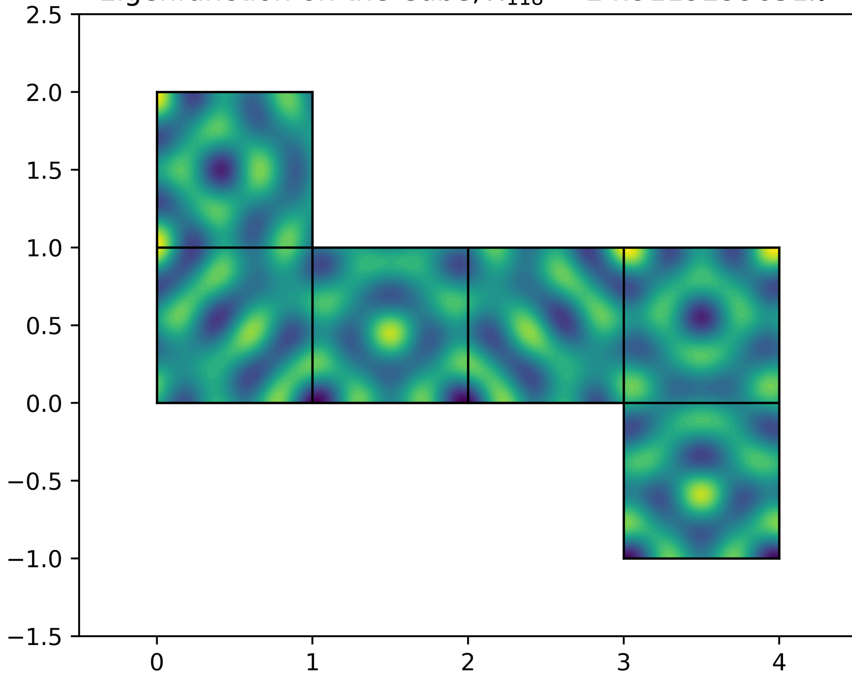
Eigenfunction on the Cube, \lambda_{118} = 24.9119299651\pi^2
