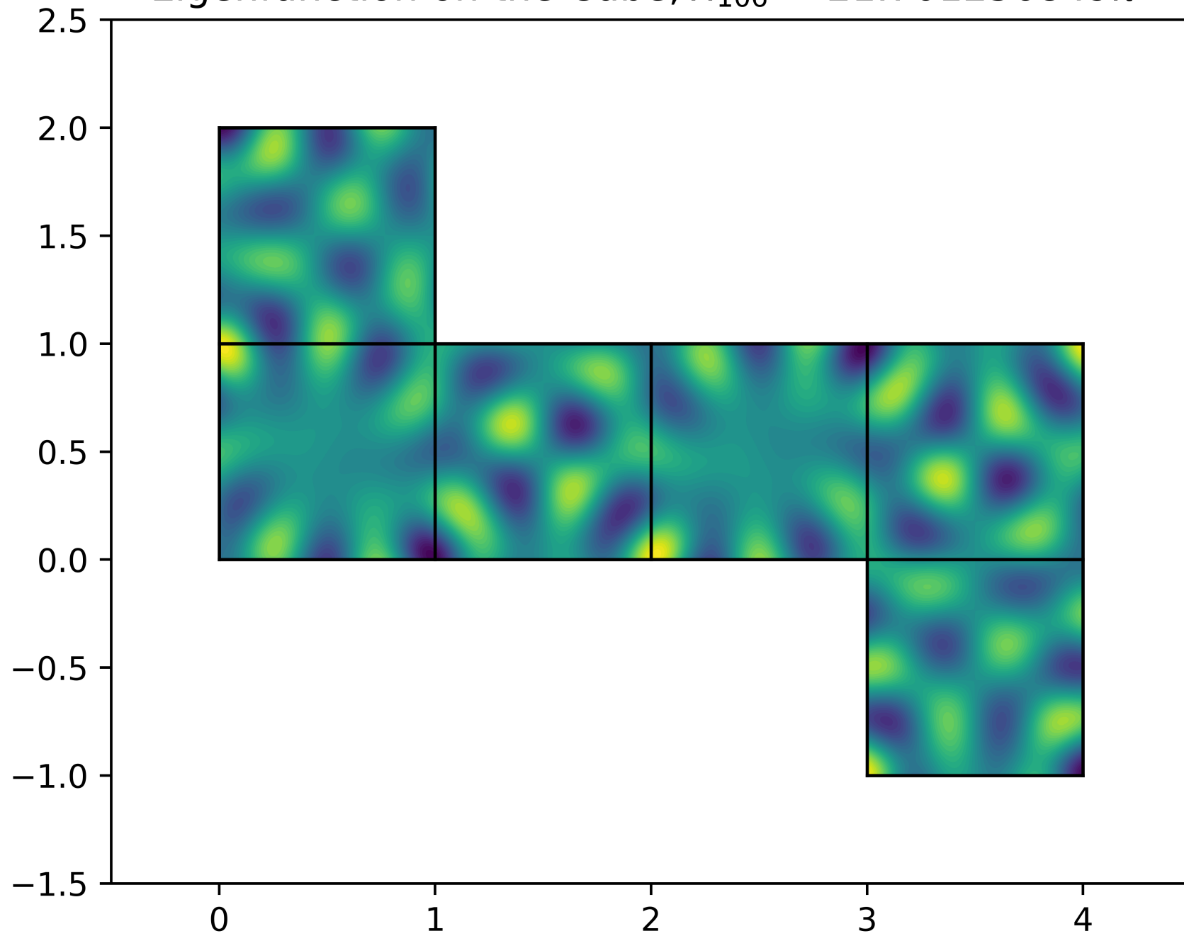
Eigenfunction on the Cube, \lambda_{106} = 21.701256849\pi^2
