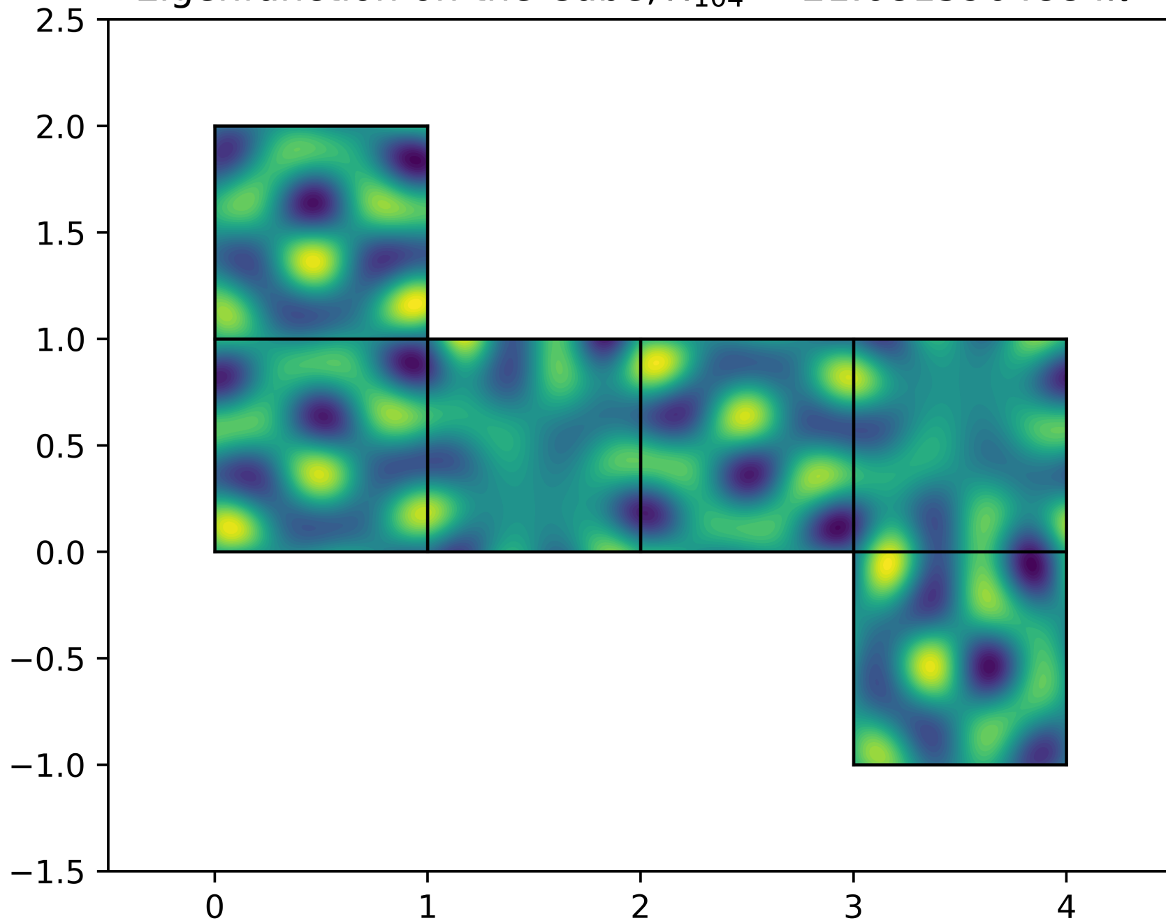
Eigenfunction on the Cube, \lambda_{104} = 21.6815964884\pi^2
