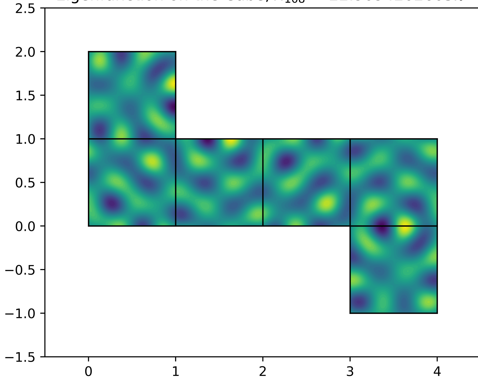
Eigenfunction on the Cube, \lambda_{108} = 22.9094202605\pi^2
