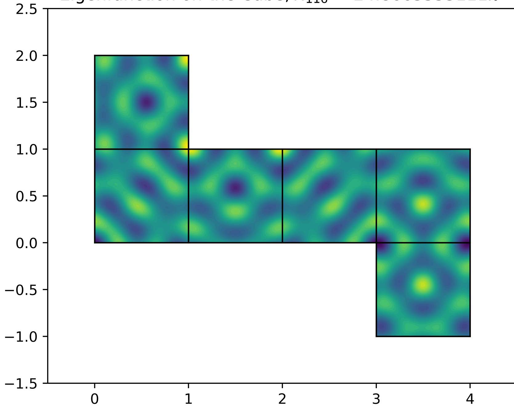
Eigenfunction on the Cube, \lambda_{116} = 24.8663553111\pi^2
