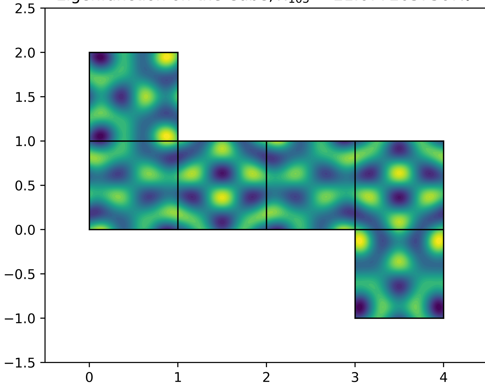
Eigenfunction on the Cube, \lambda_{103} = 21.6772037567\pi^2
