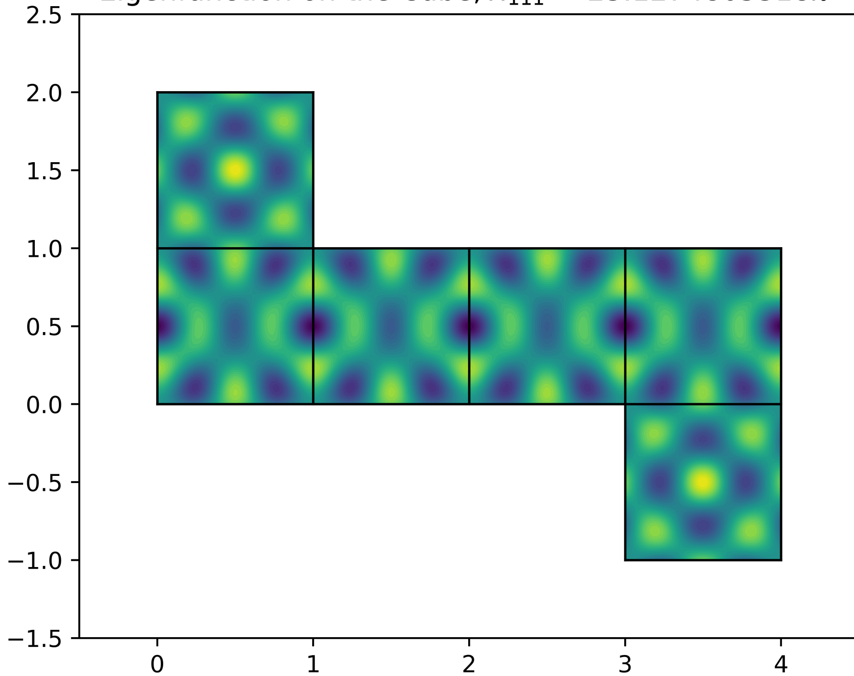
Eigenfunction on the Cube, \lambda_{111} = 23.1274805318\pi^2
