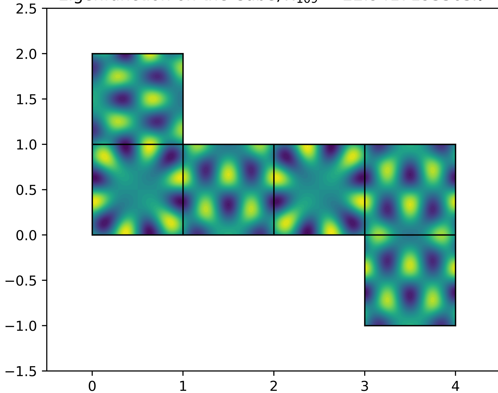
Eigenfunction on the Cube, \lambda_{109} = 22.9417193565\pi^2
