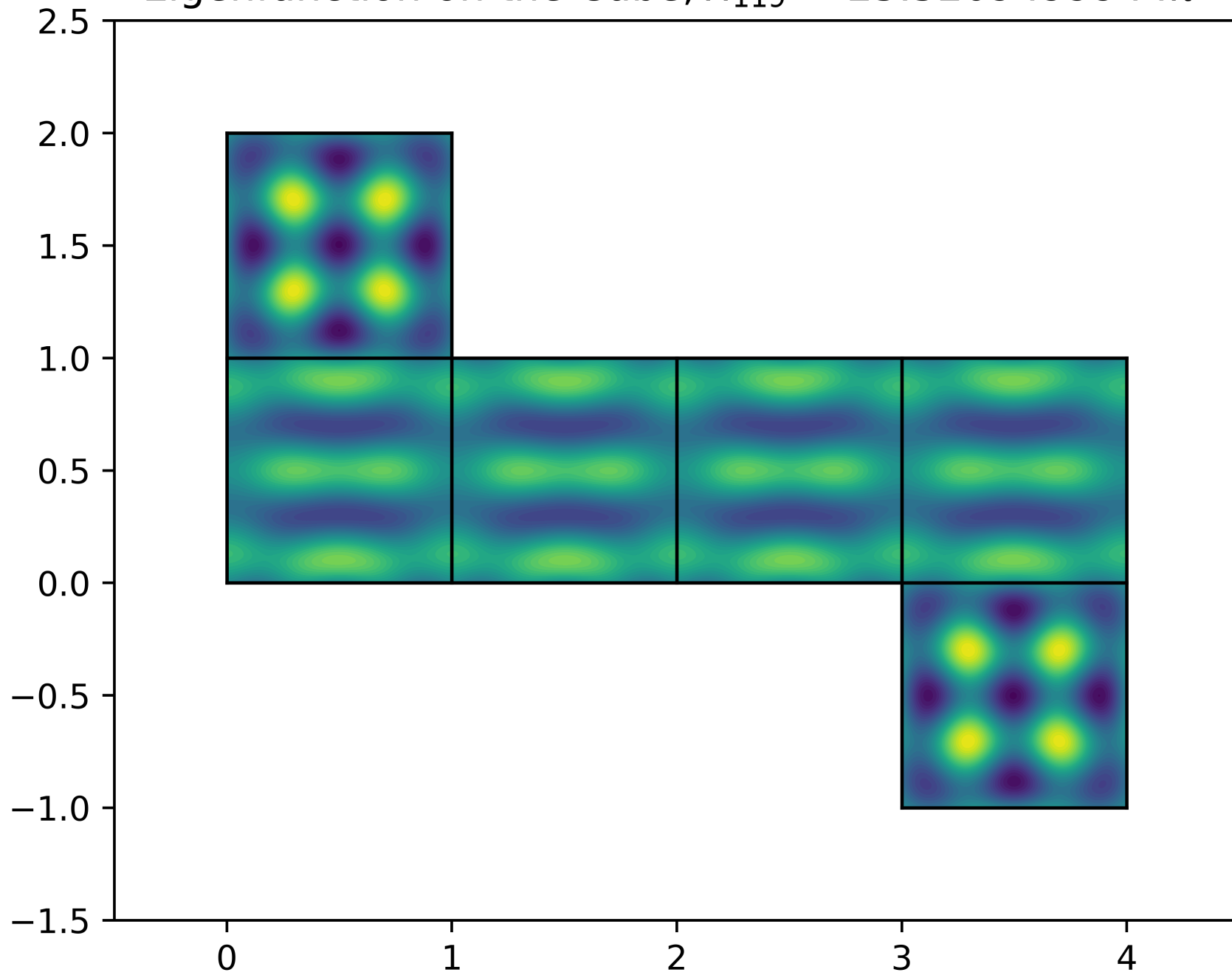
Eigenfunction on the Cube, \lambda_{119} = 25.5209499944\pi^2
