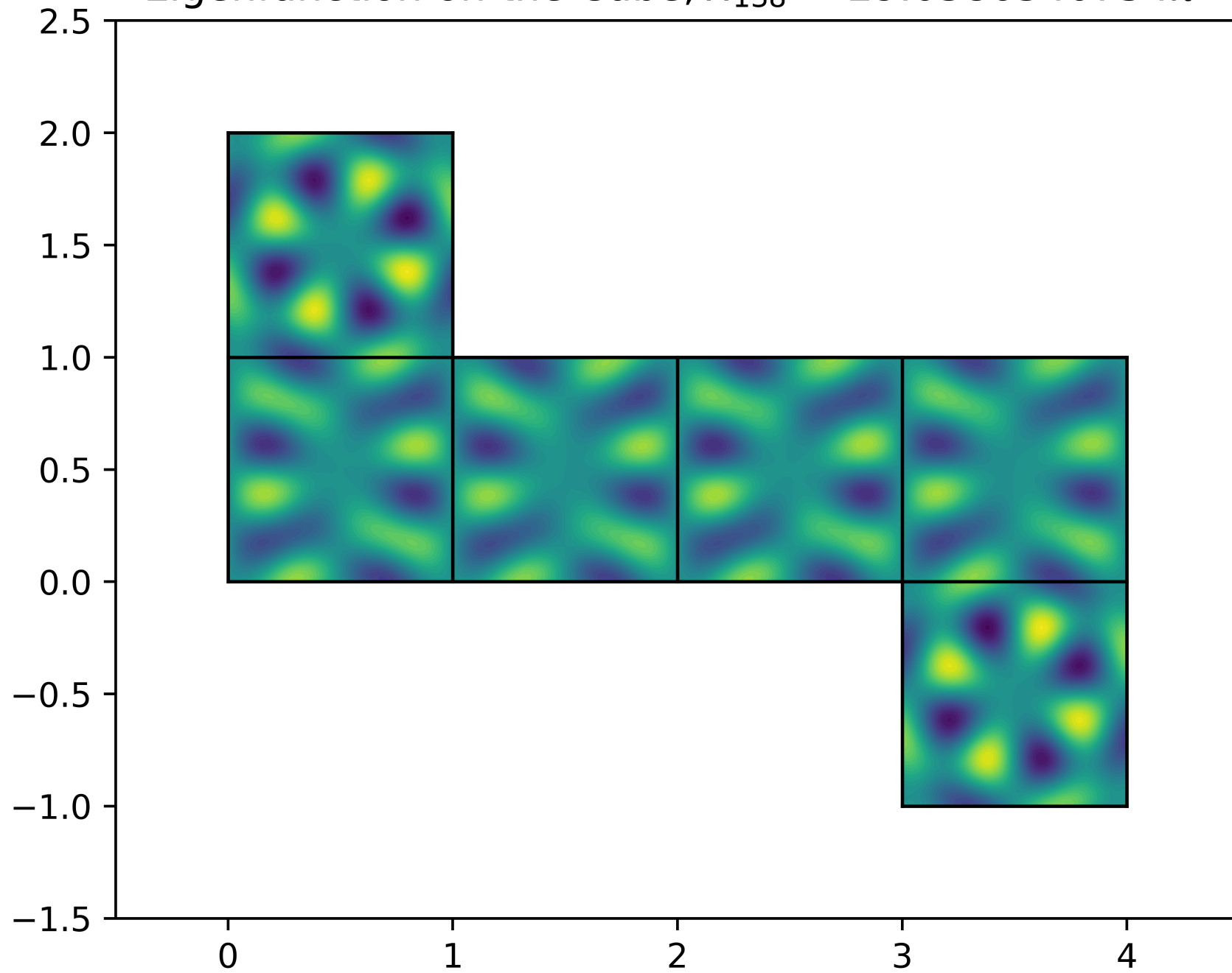
Eigenfunction on the Cube, \lambda_{138} = 29.0386340754\pi^2
