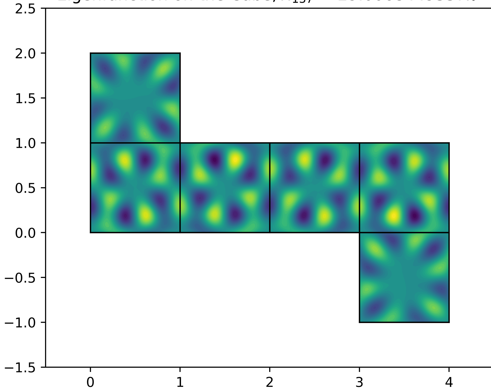
Eigenfunction on the Cube, \lambda_{137} = 29.0068449337\pi^2
