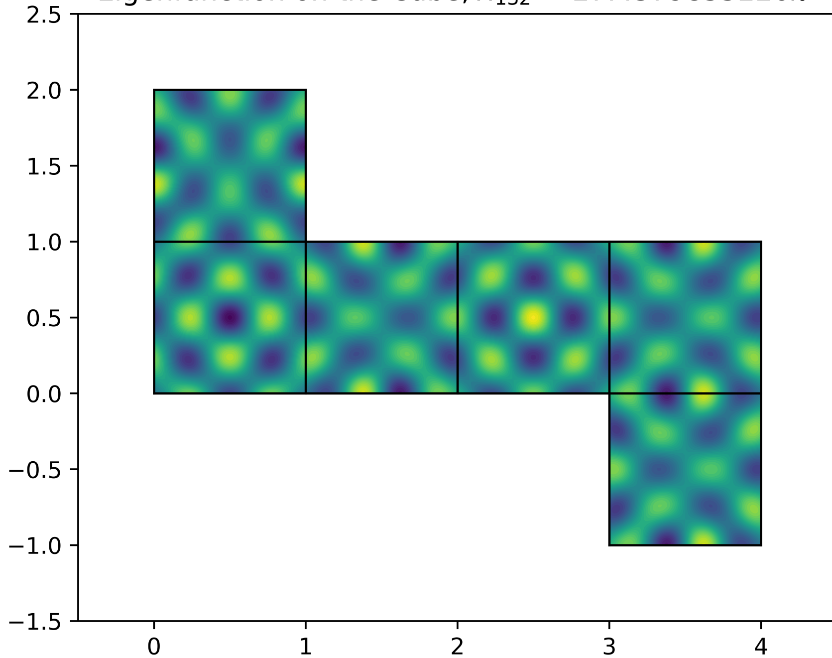
Eigenfunction on the Cube, \lambda_{132} = 27.4379855226\pi^2
