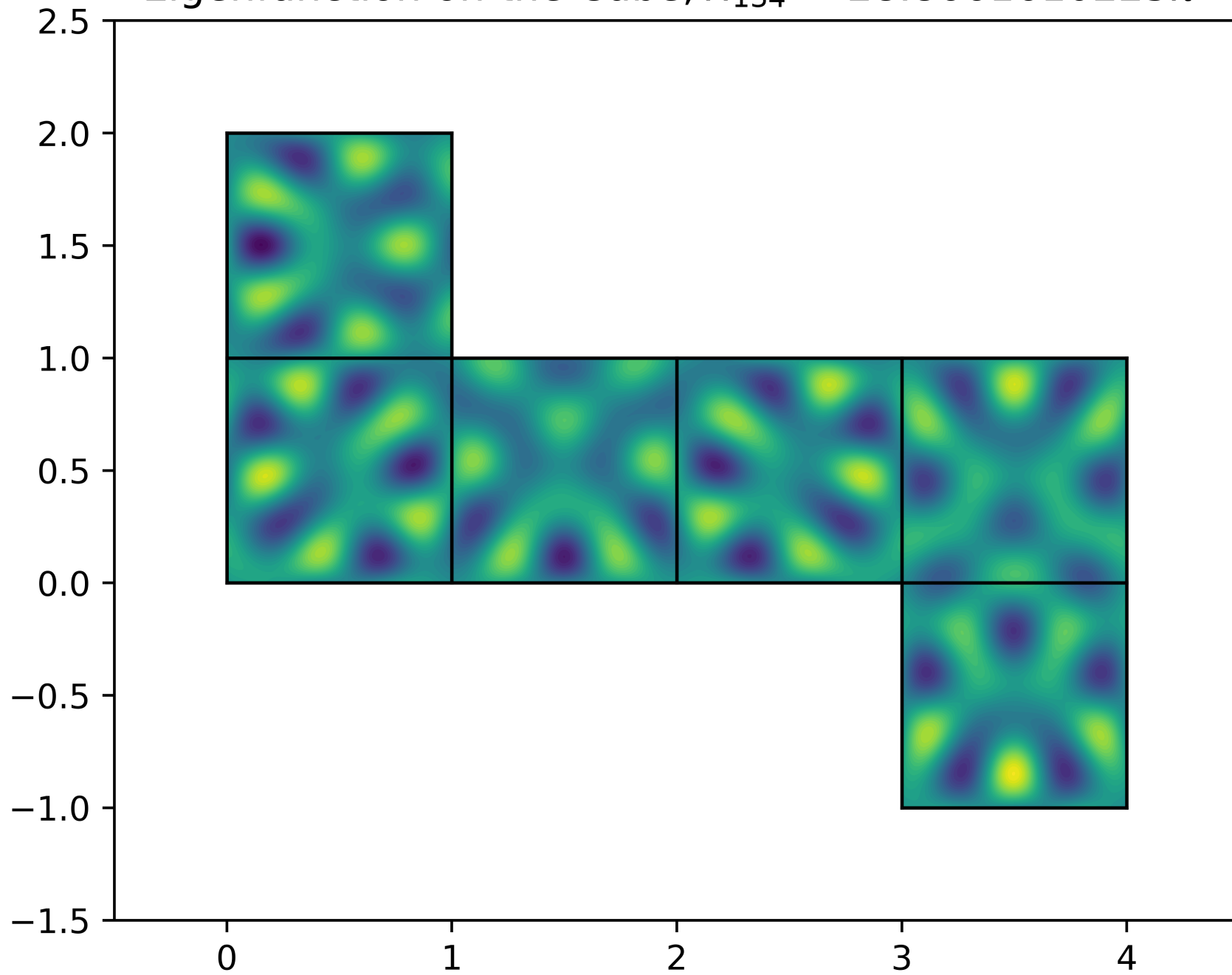
Eigenfunction on the Cube, \lambda_{134} = 28.8661610225\pi^2
