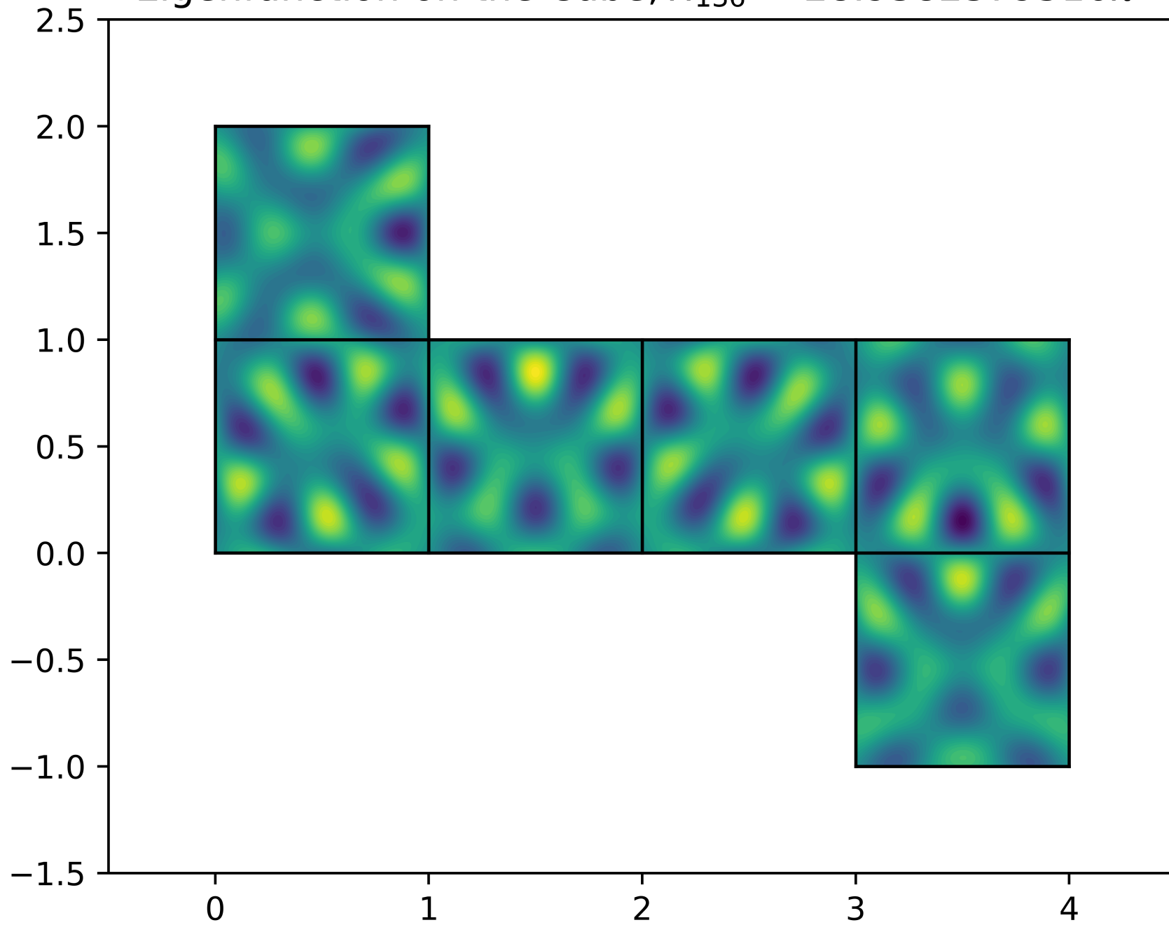
Eigenfunction on the Cube, \lambda_{136} = 28.9382379516\pi^2
