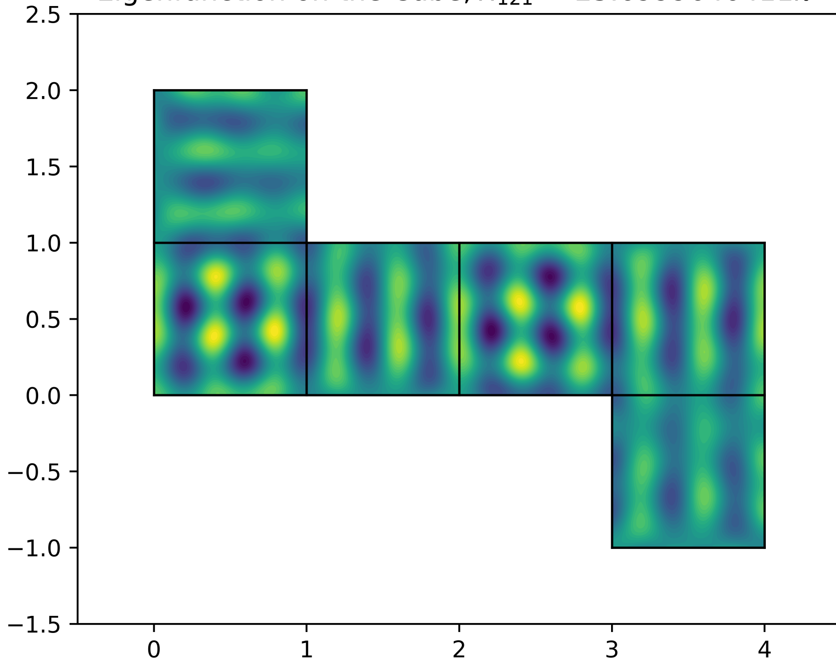
Eigenfunction on the Cube, \lambda_{121} = 25.6999646411\pi^2
