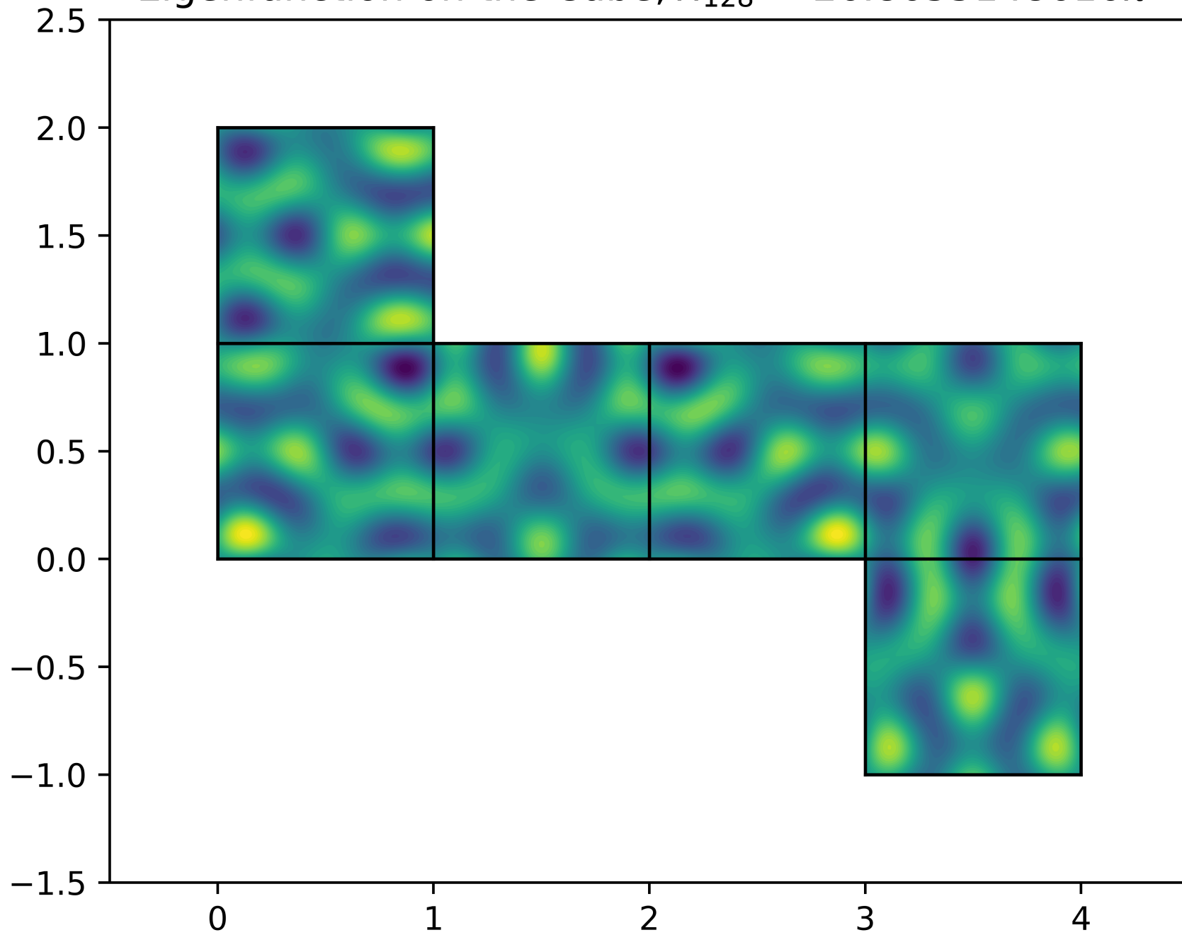
Eigenfunction on the Cube, \lambda_{128} = 26.8655148616\pi^2
