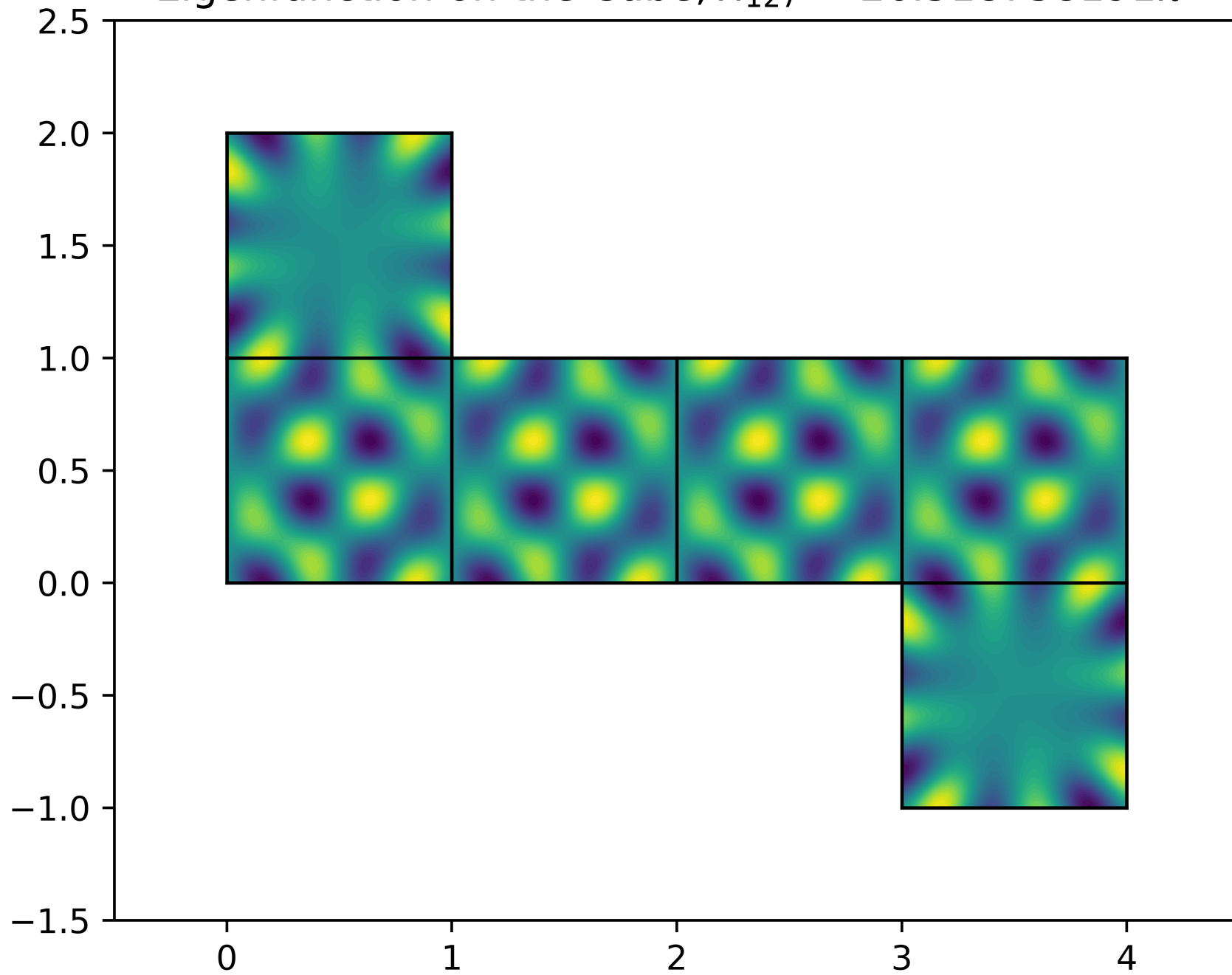
Eigenfunction on the Cube, \lambda_{127} = 26.518758191\pi^2
