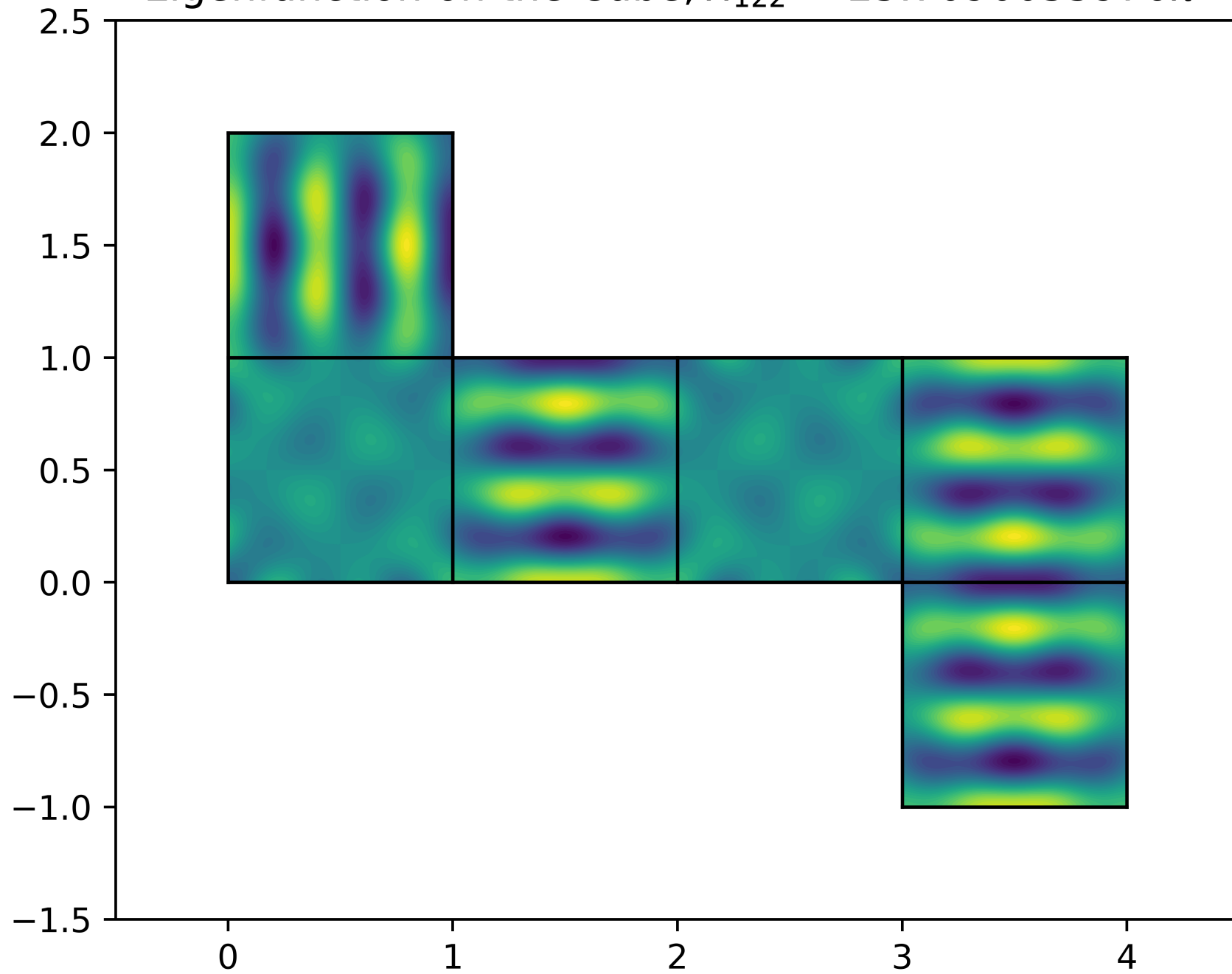
Eigenfunction on the Cube, \lambda_{122} = 25.7090055976\pi^2
