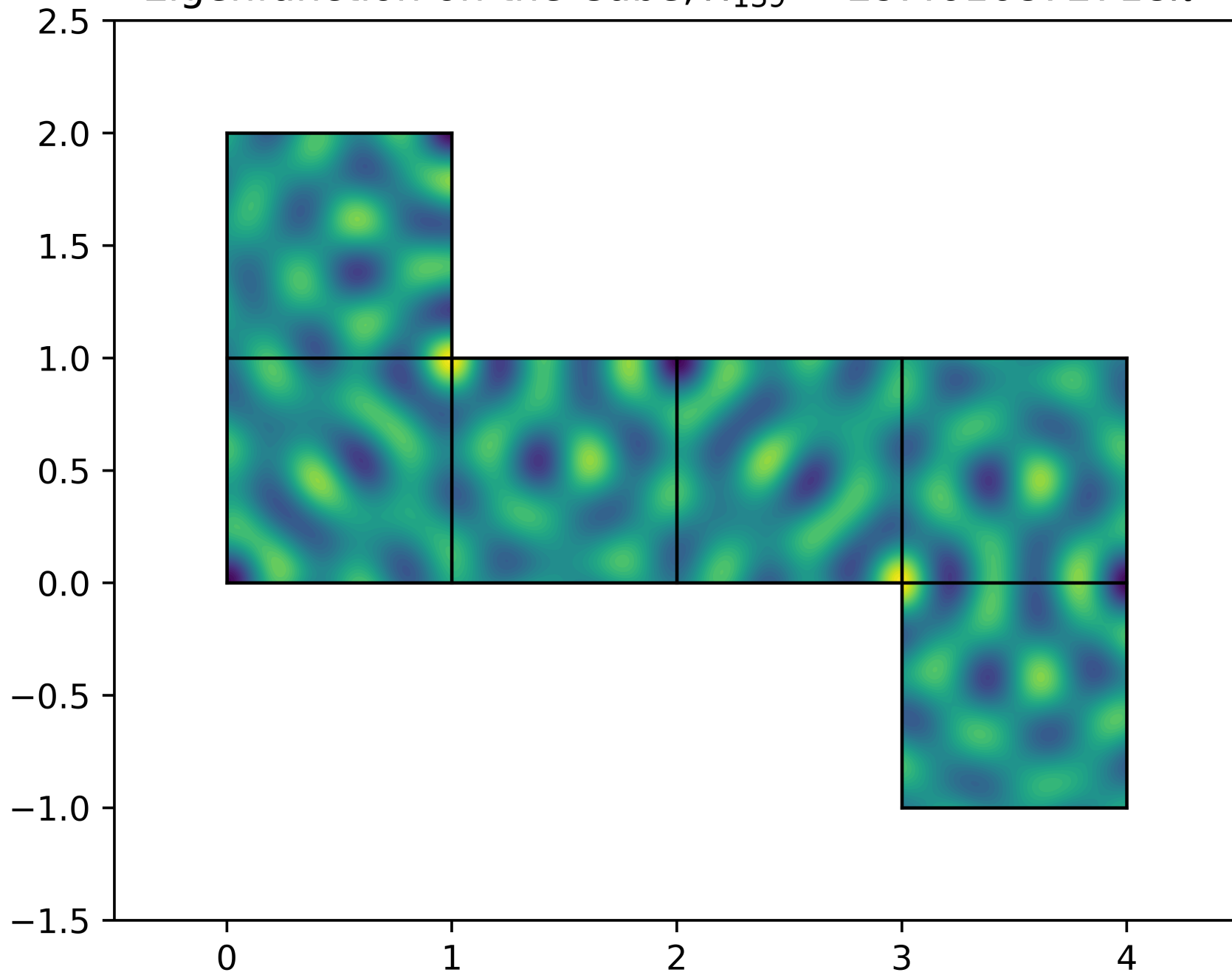
Eigenfunction on the Cube, \lambda_{139} = 29.4616872718\pi^2
