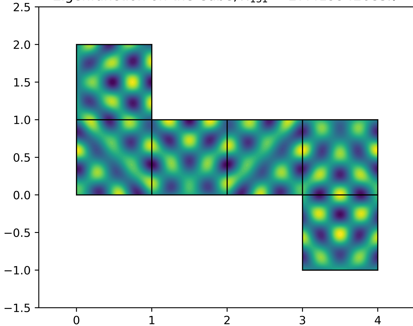
Eigenfunction on the Cube, \lambda_{131} = 27.419942685\pi^2
