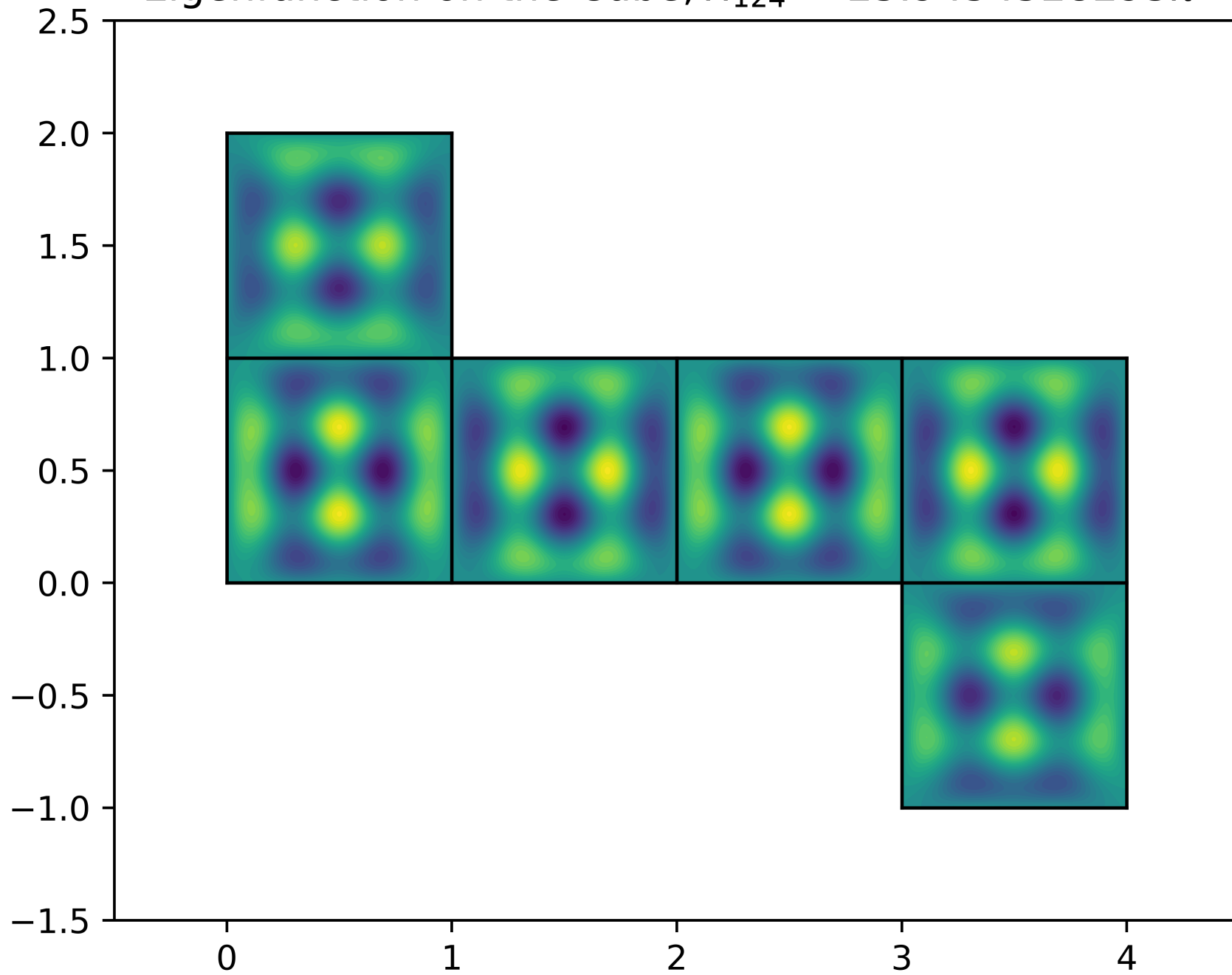
Eigenfunction on the Cube, \lambda_{124} = 25.9454528293\pi^2
