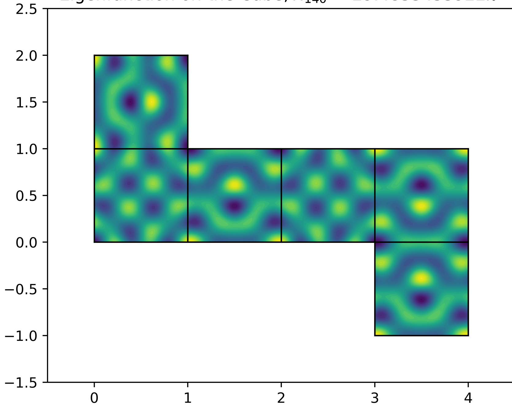
Eigenfunction on the Cube, \lambda_{140} = 29.4833433922\pi^2
