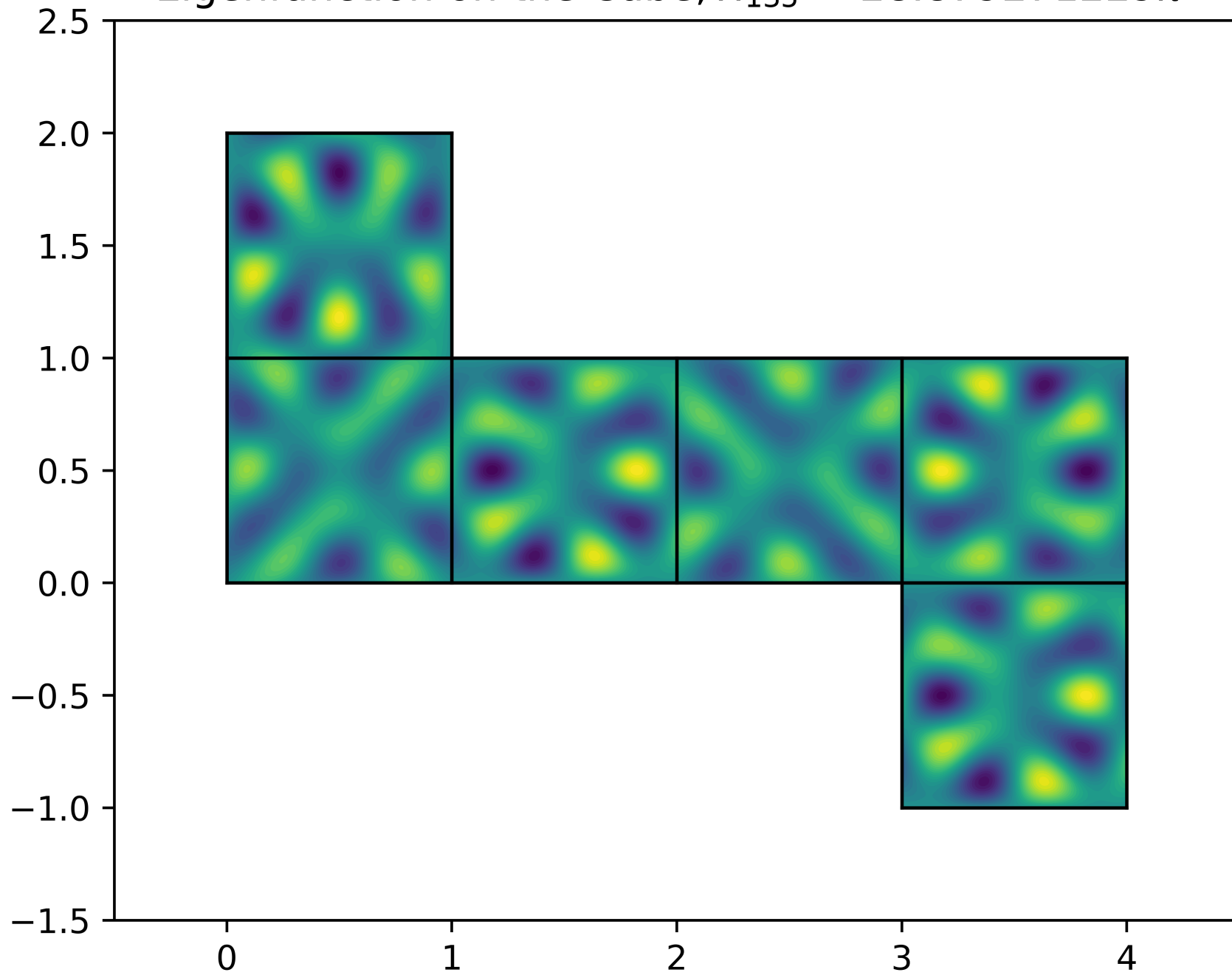
Eigenfunction on the Cube, \lambda_{135} = 28.879271229\pi^2
