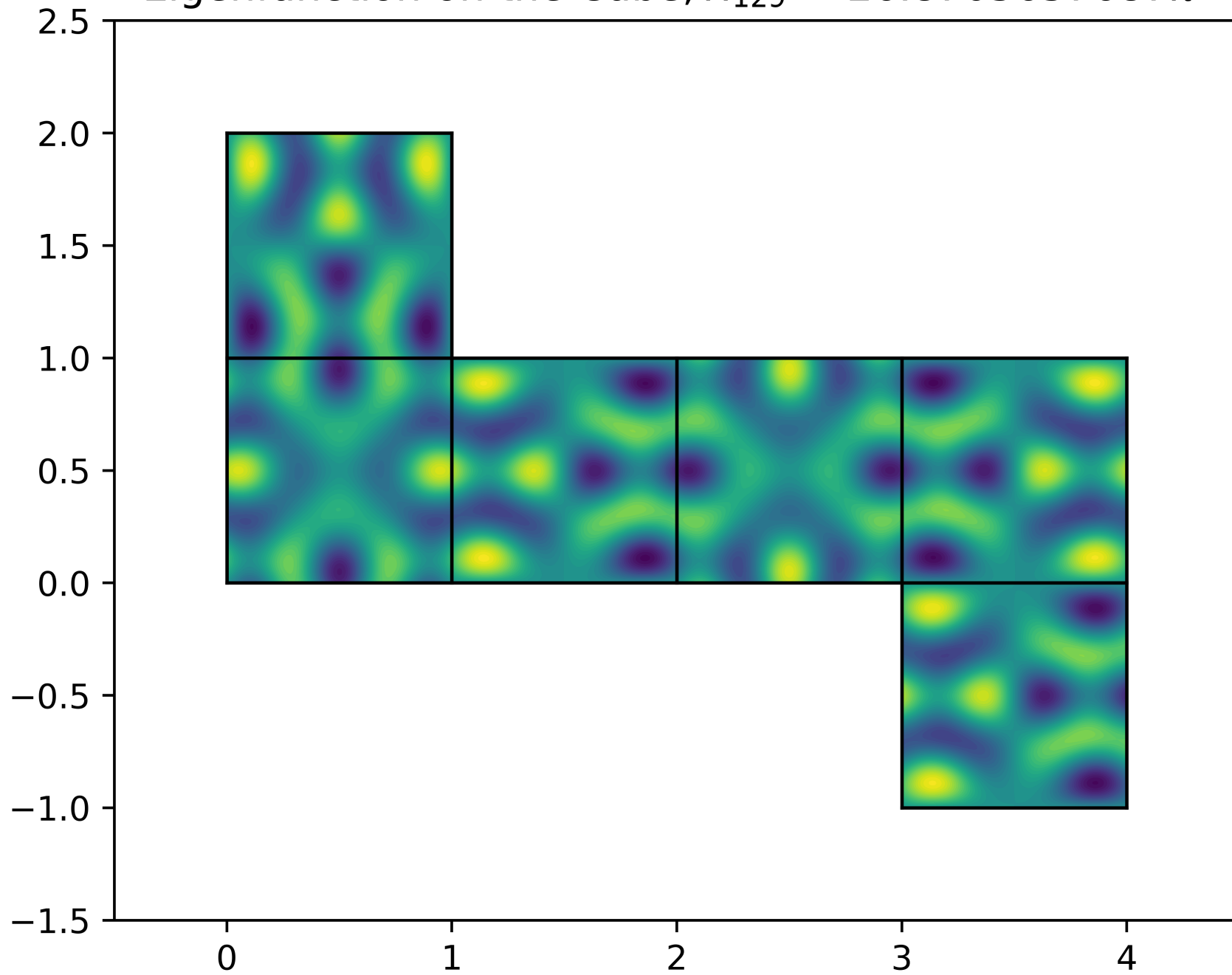
Eigenfunction on the Cube, \lambda_{129} = 26.8705657687\pi^2
