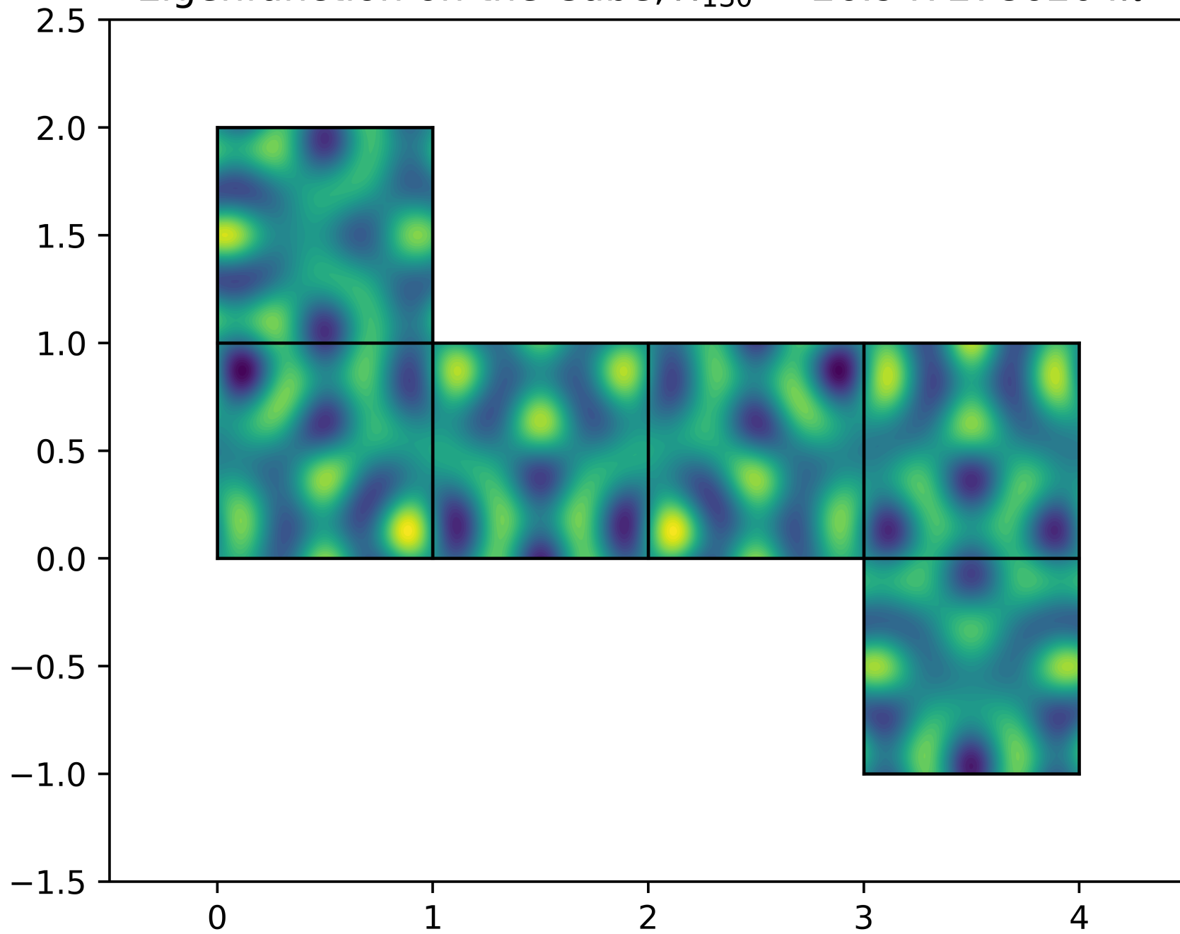
Eigenfunction on the Cube, \lambda_{130} = 26.9472786204\pi^2
