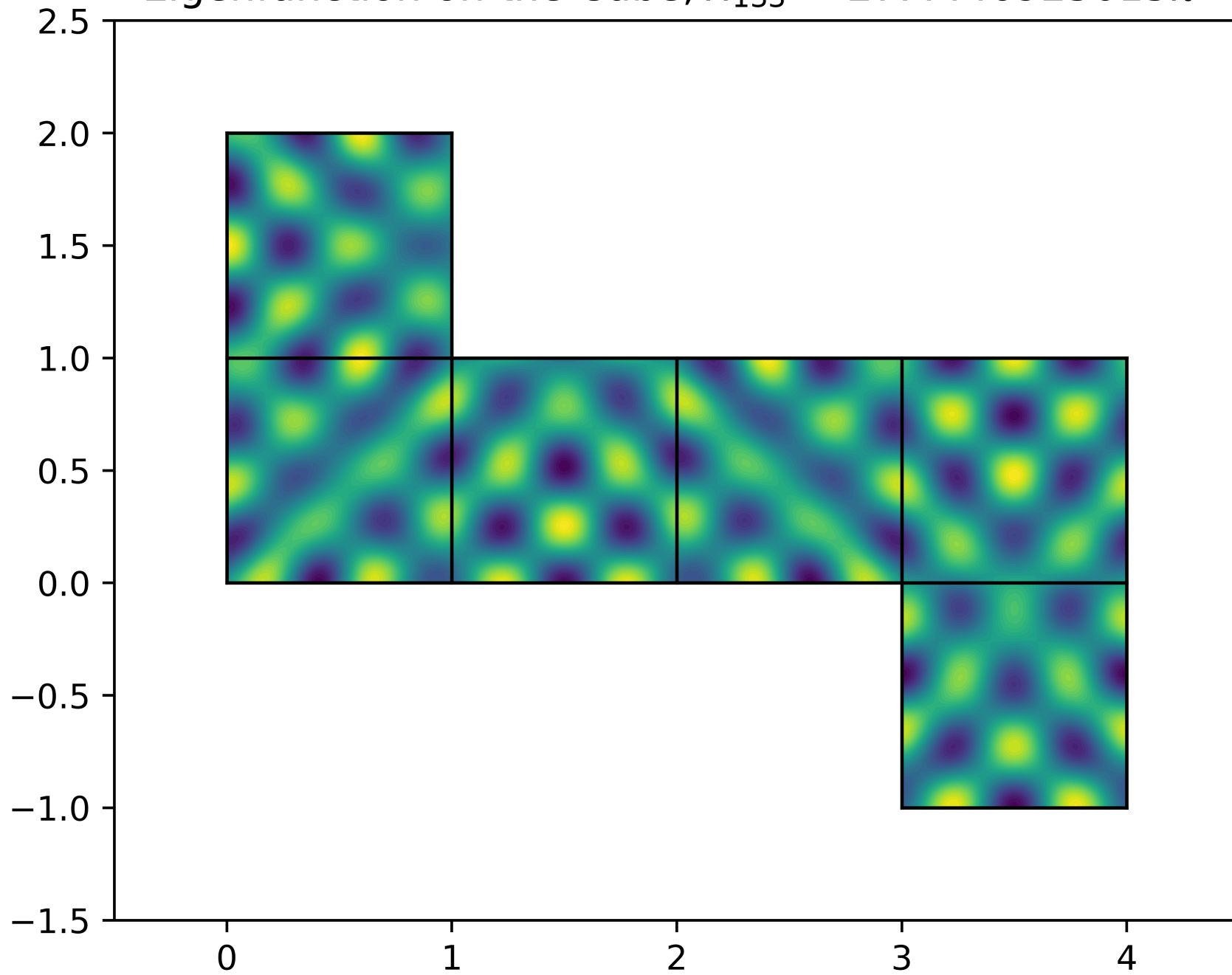
Eigenfunction on the Cube, \lambda_{133} = 27.4446925015\pi^2
