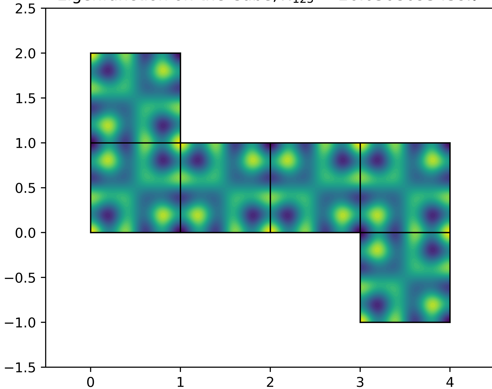
Eigenfunction on the Cube, \lambda_{125} = 26.0308093439\pi^2
