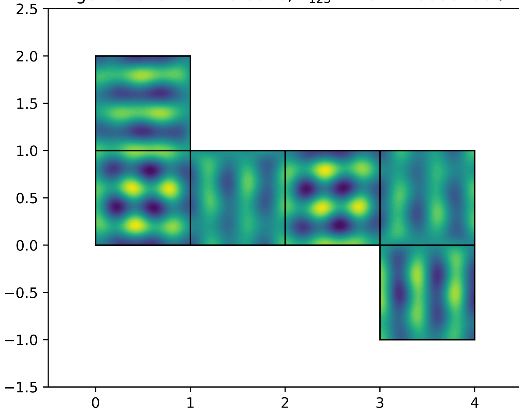
Eigenfunction on the Cube, \lambda_{123} = 25.7123355108\pi^2
