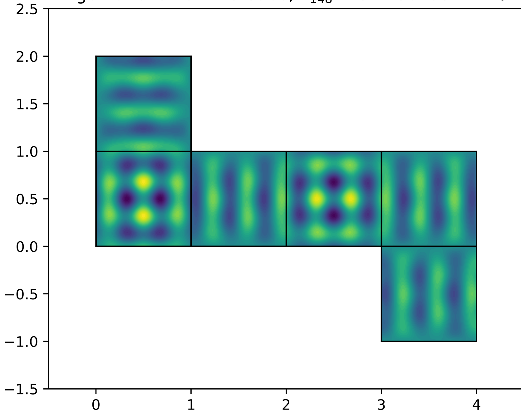
Eigenfunction on the Cube, \lambda_{148} = 31.1301954171\pi^2
