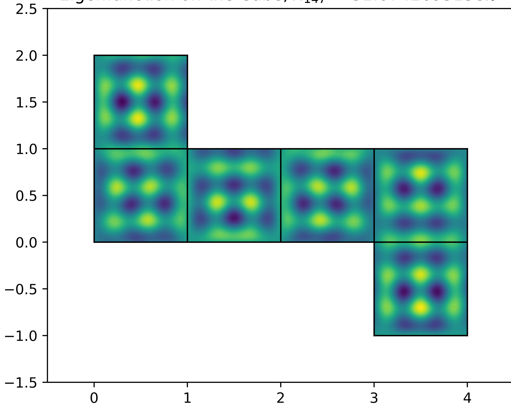
Eigenfunction on the Cube, \lambda_{147} = 31.0742695158\pi^2
