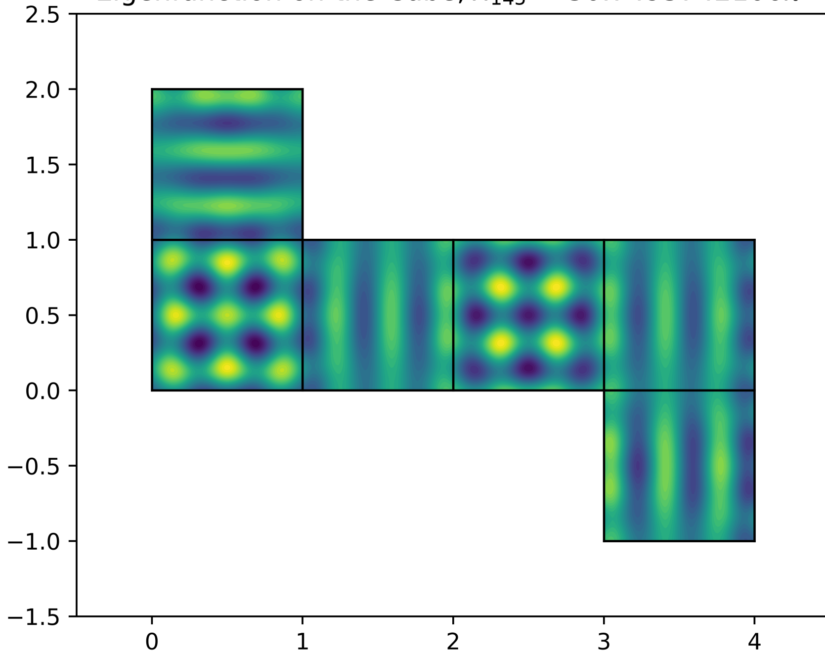
Eigenfunction on the Cube, \lambda_{145} = 30.7493742106\pi^2
