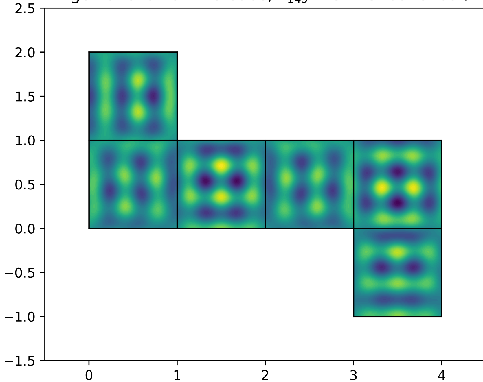
Eigenfunction on the Cube, \lambda_{149} = 31.1540378409\pi^2
