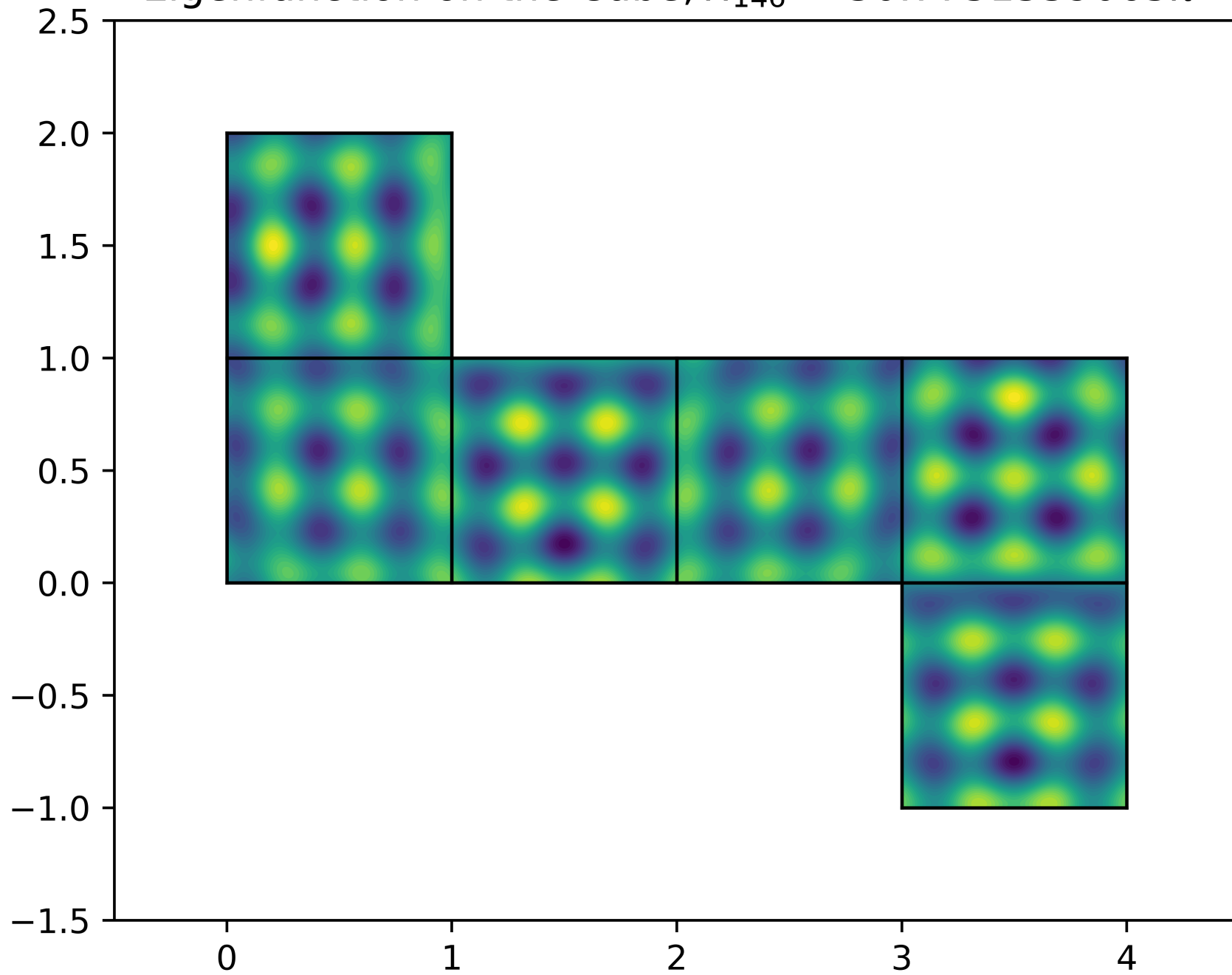
Eigenfunction on the Cube, \lambda_{146} = 30.7751339065\pi^2
