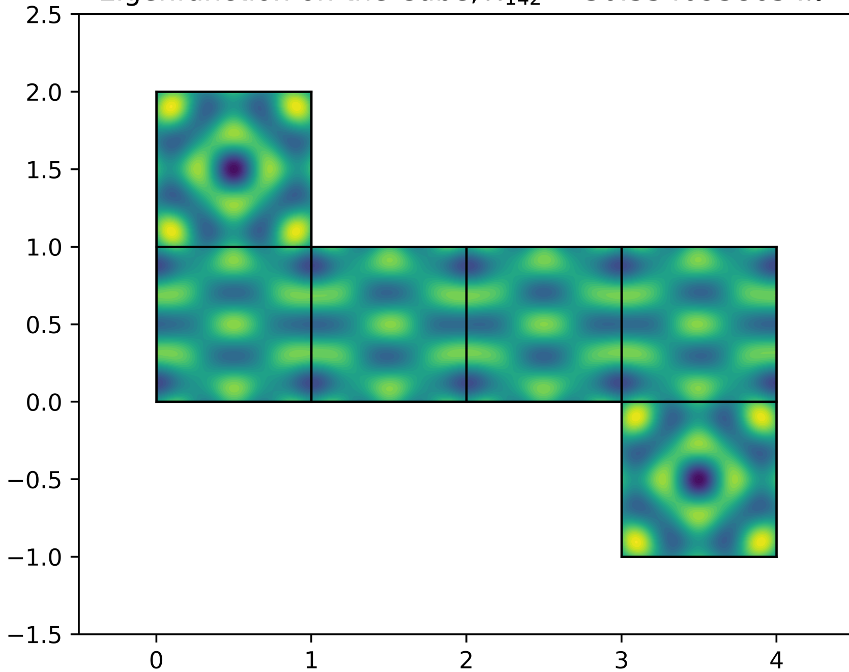
Eigenfunction on the Cube, \lambda_{142} = 30.5540938654\pi^2
