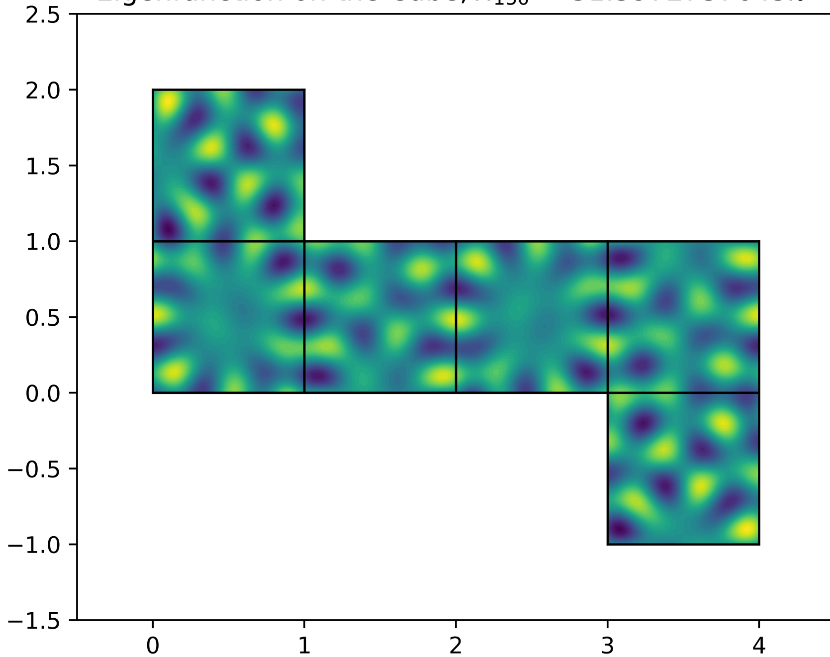
Eigenfunction on the Cube, \lambda_{150} = 31.5972737645\pi^2
