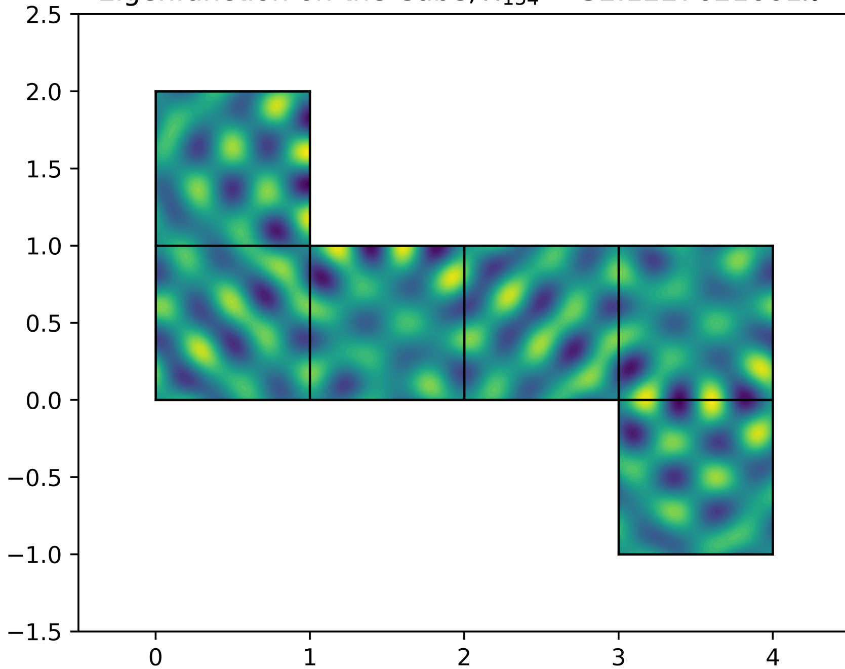
Eigenfunction on the Cube, \lambda_{154} = 32.1227621661\pi^2
