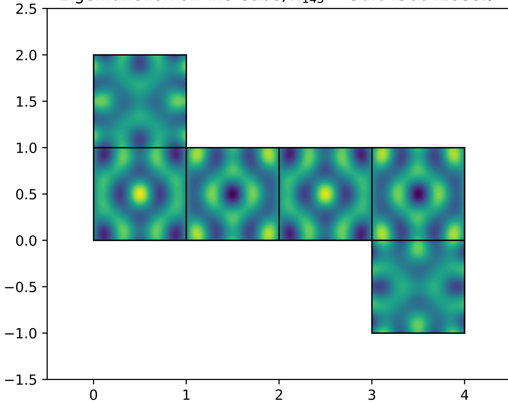
Eigenfunction on the Cube, \lambda_{143} = 30.6456642935\pi^2
