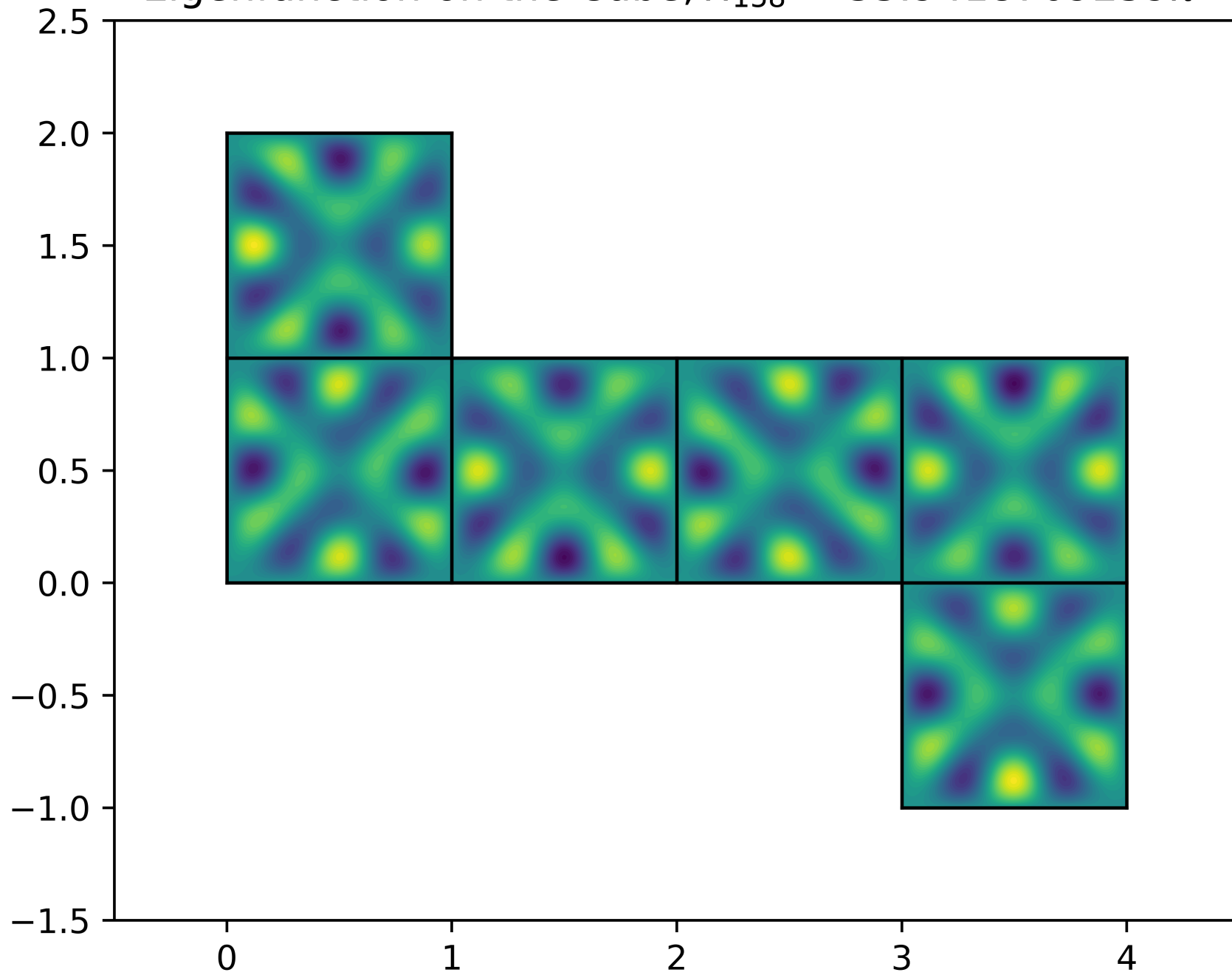
Eigenfunction on the Cube, \lambda_{158} = 33.9418709259\pi^2
