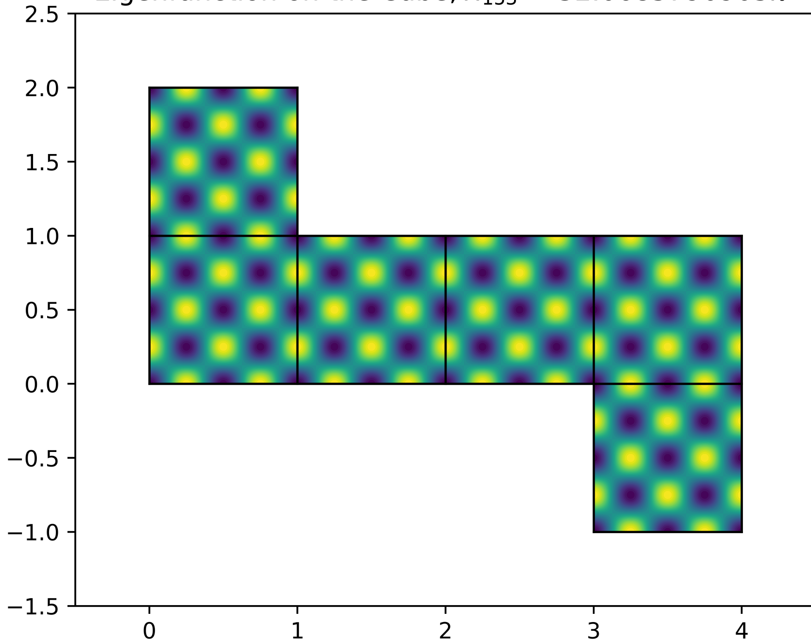
Eigenfunction on the Cube, \lambda_{153} = 32.0685790905\pi^2
