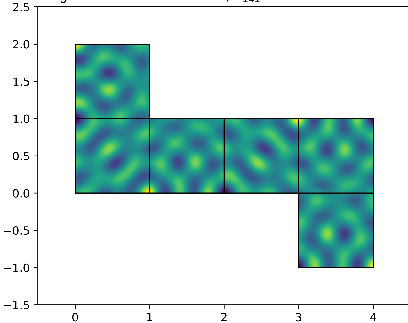
Eigenfunction on the Cube, \lambda_{141} = 29.4919153624\pi^2
