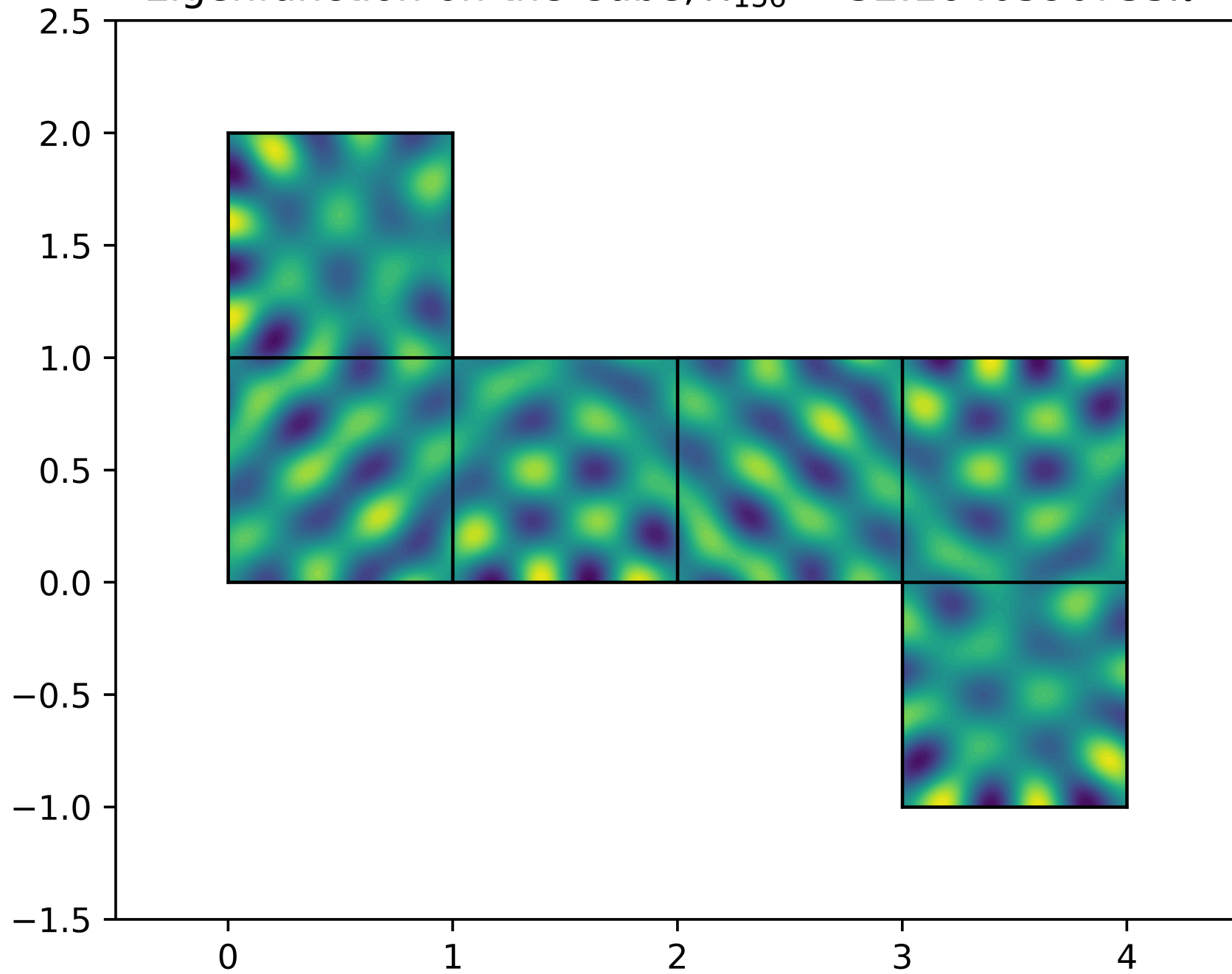
Eigenfunction on the Cube, \lambda_{156} = 32.1640590735\pi^2
