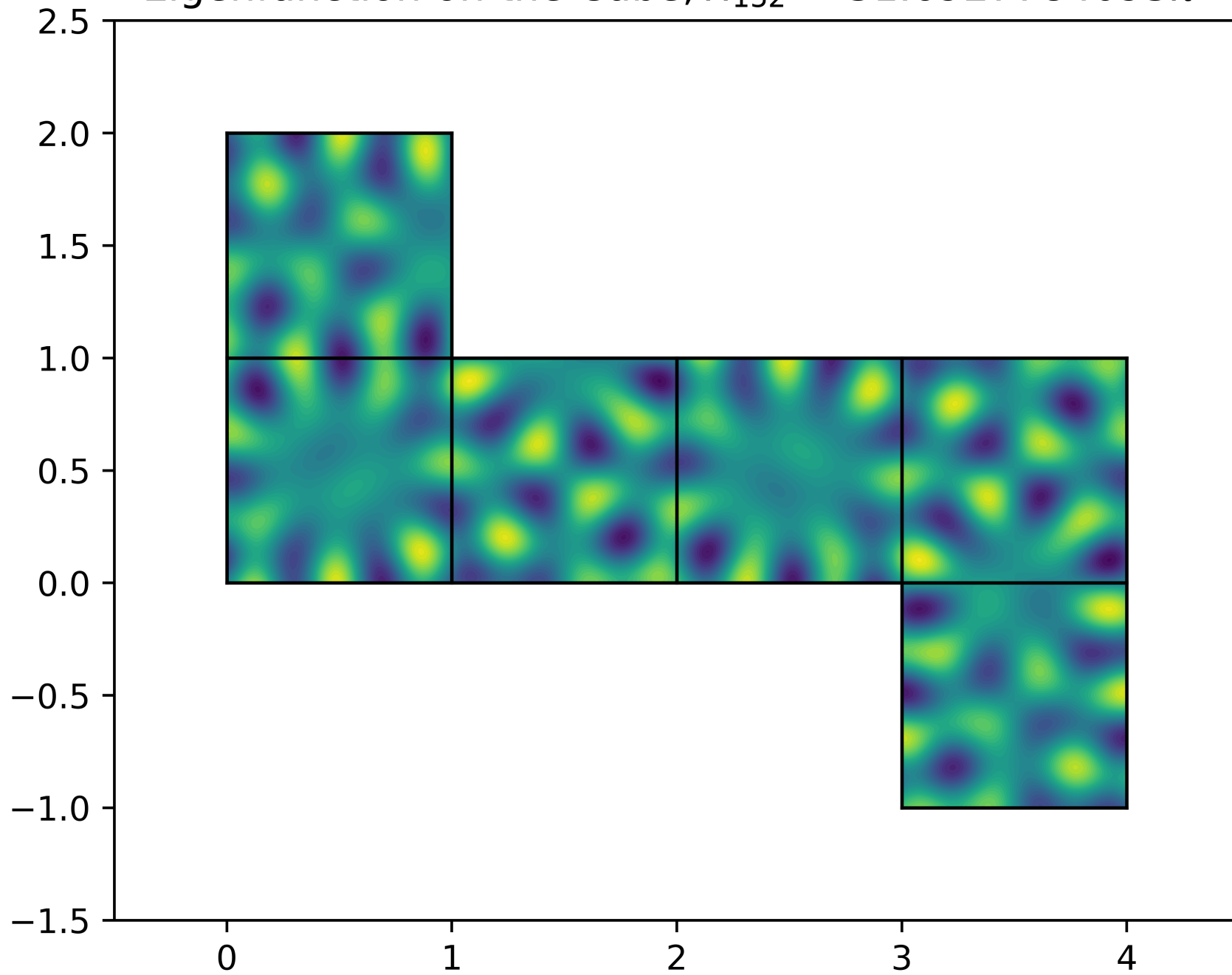
Eigenfunction on the Cube, \lambda_{152} = 31.6927784093\pi^2
