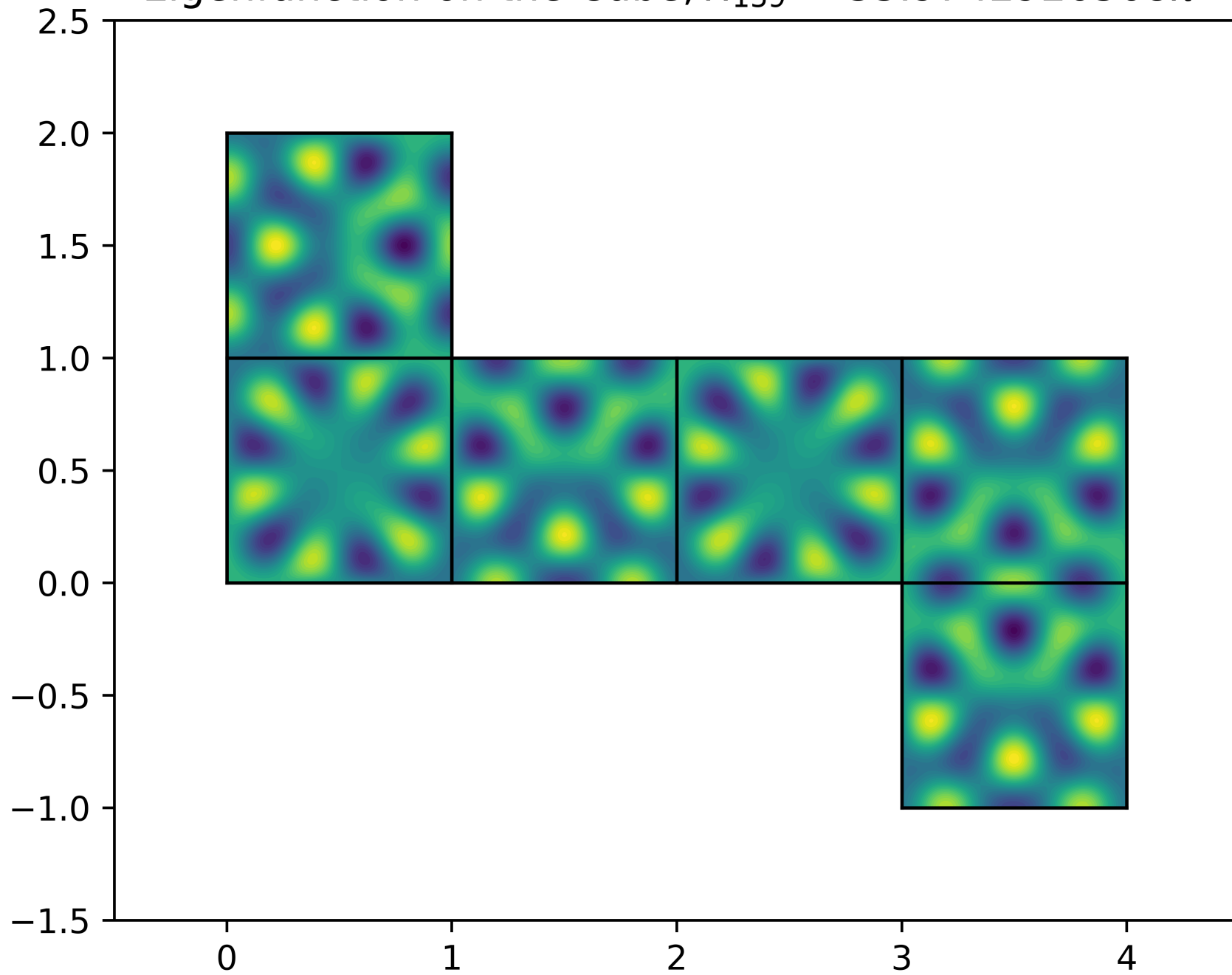
Eigenfunction on the Cube, \lambda_{159} = 33.9742926368\pi^2
