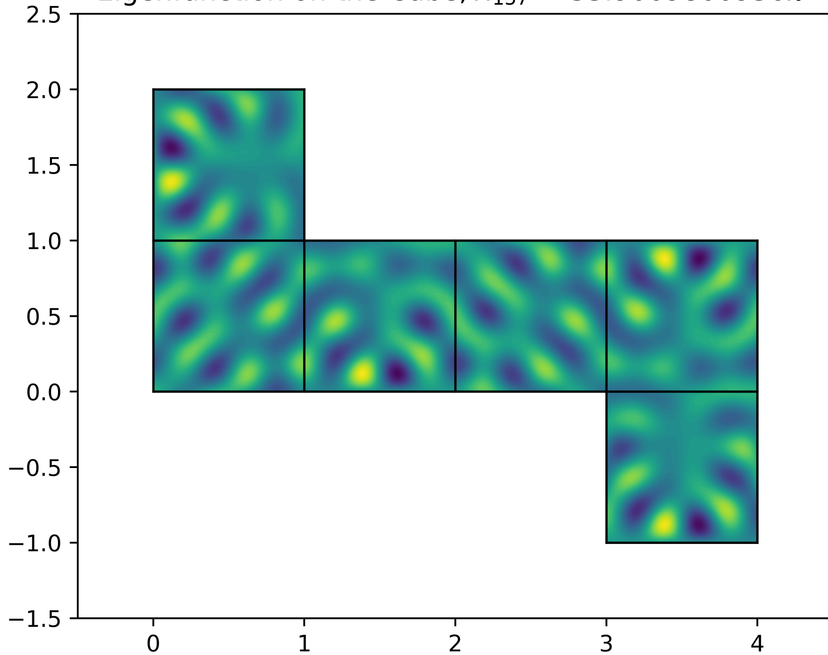
Eigenfunction on the Cube, \lambda_{157} = 33.9009800936\pi^2
