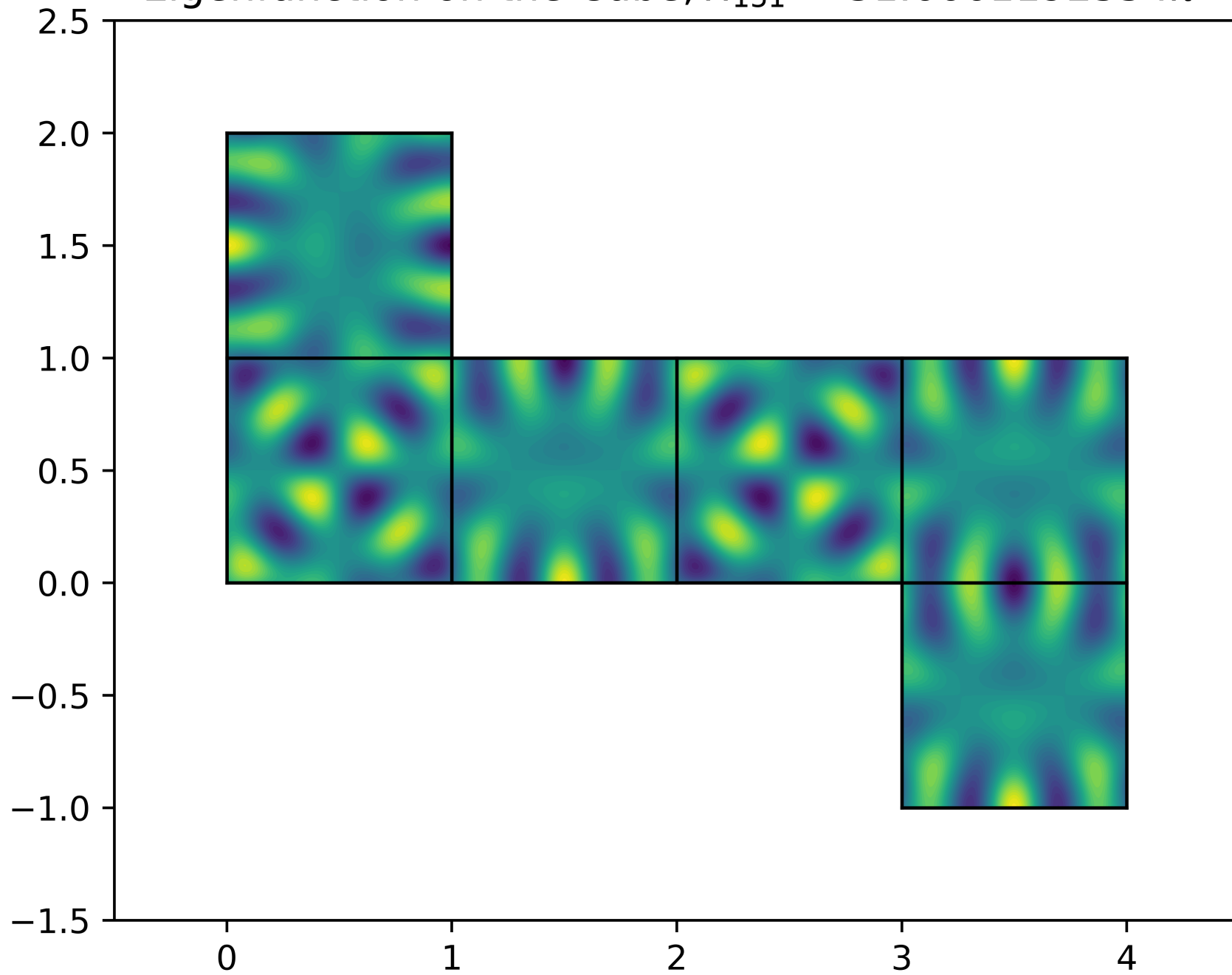
Eigenfunction on the Cube, \lambda_{151} = 31.6661192554\pi^2
