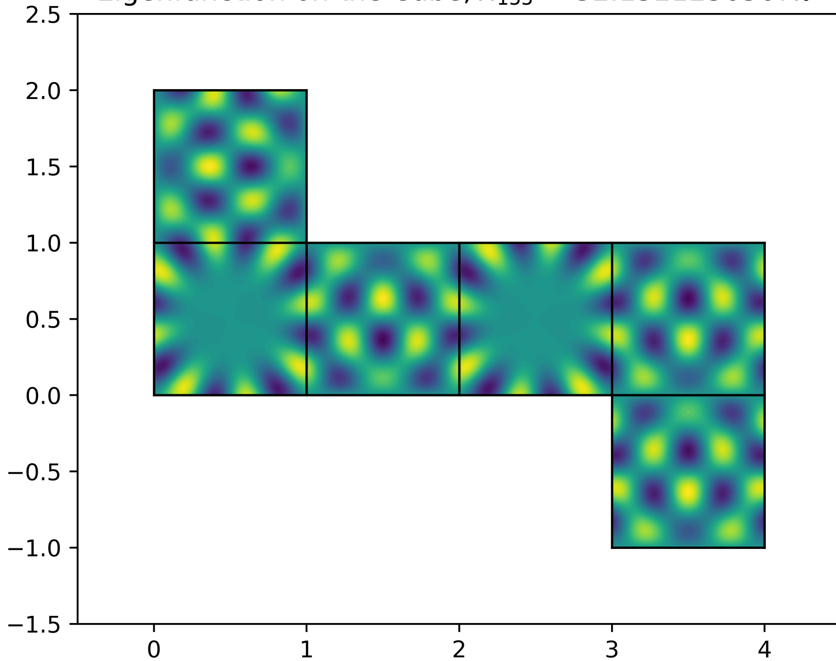
Eigenfunction on the Cube, \lambda_{155} = 32.1321236567\pi^2
