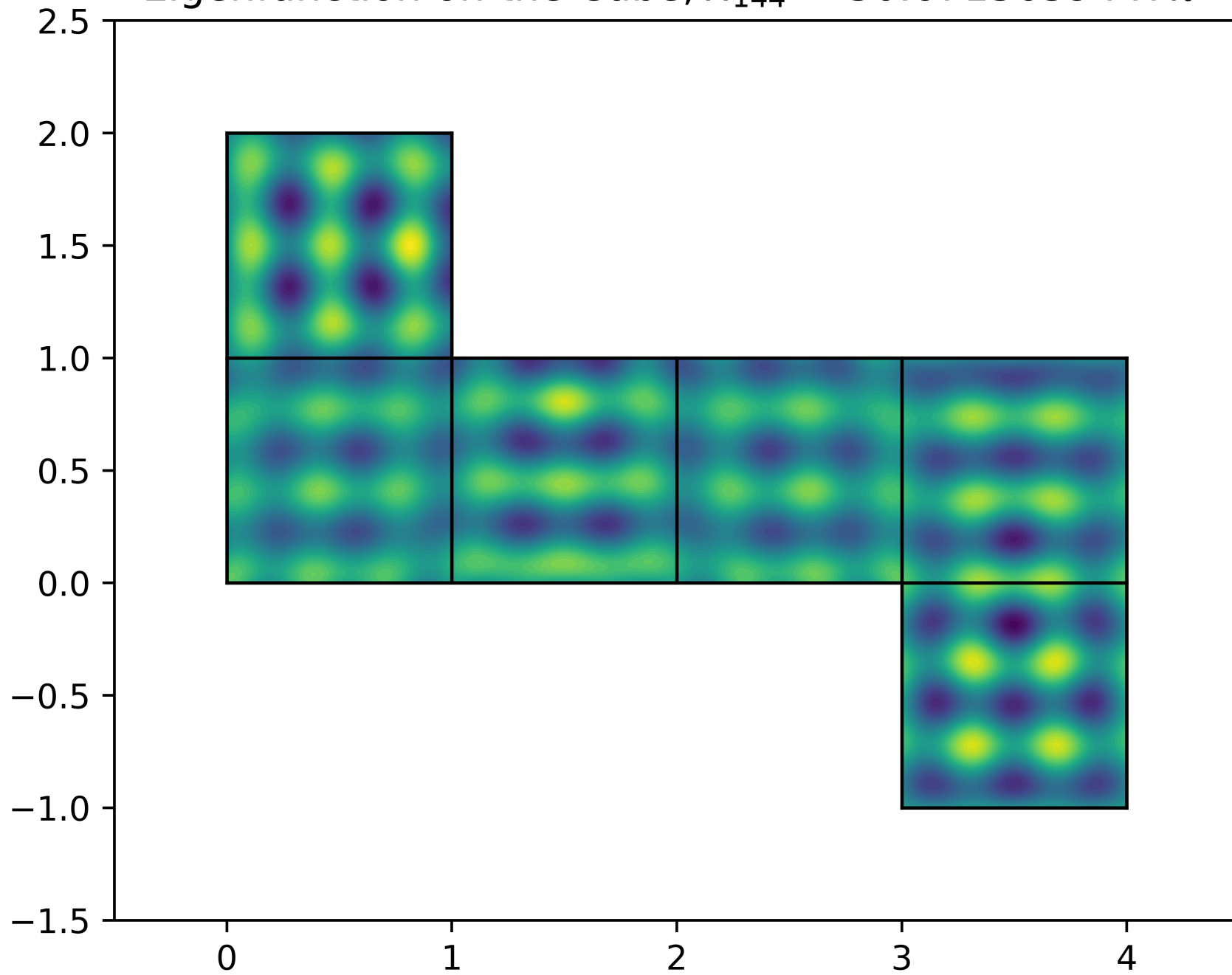
Eigenfunction on the Cube, \lambda_{144} = 30.6713639447\pi^2
