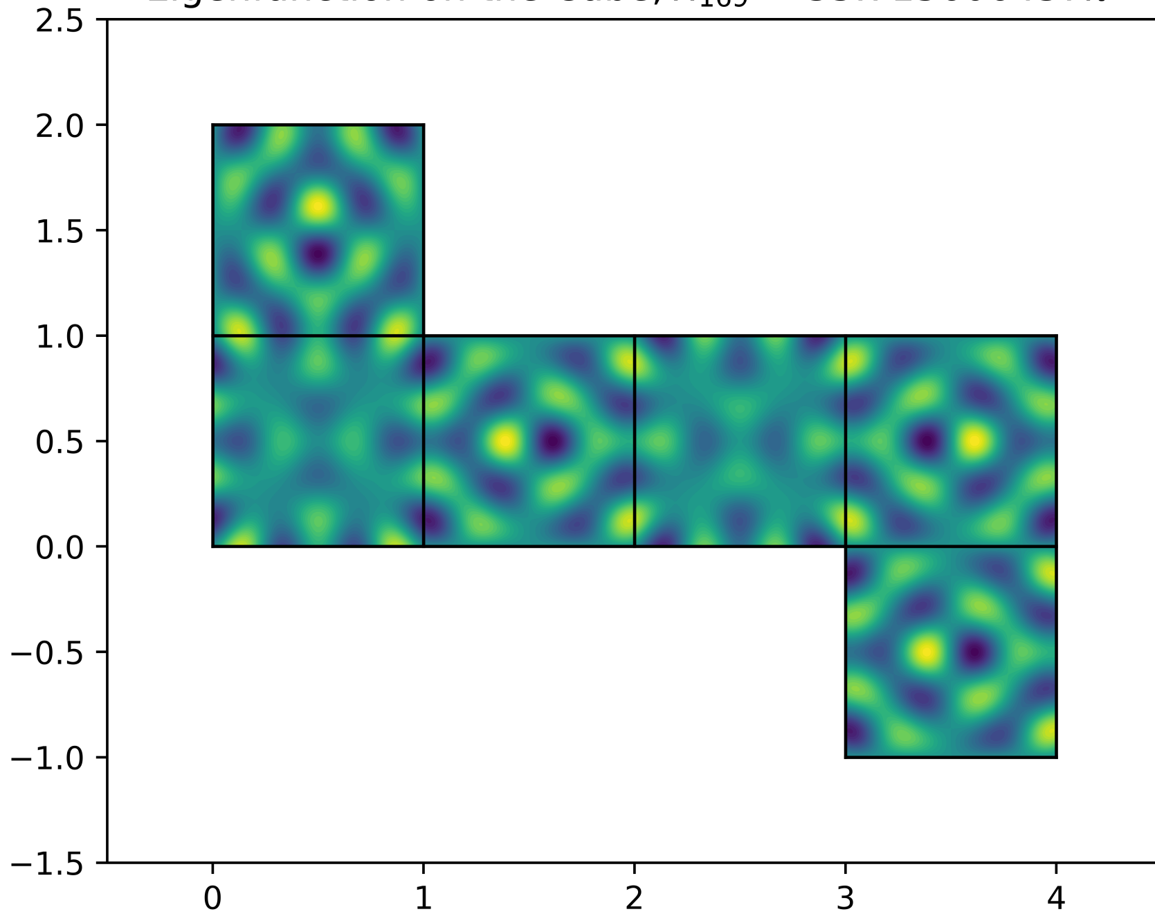
Eigenfunction on the Cube, \lambda_{169} = 35.715606437\pi^2
