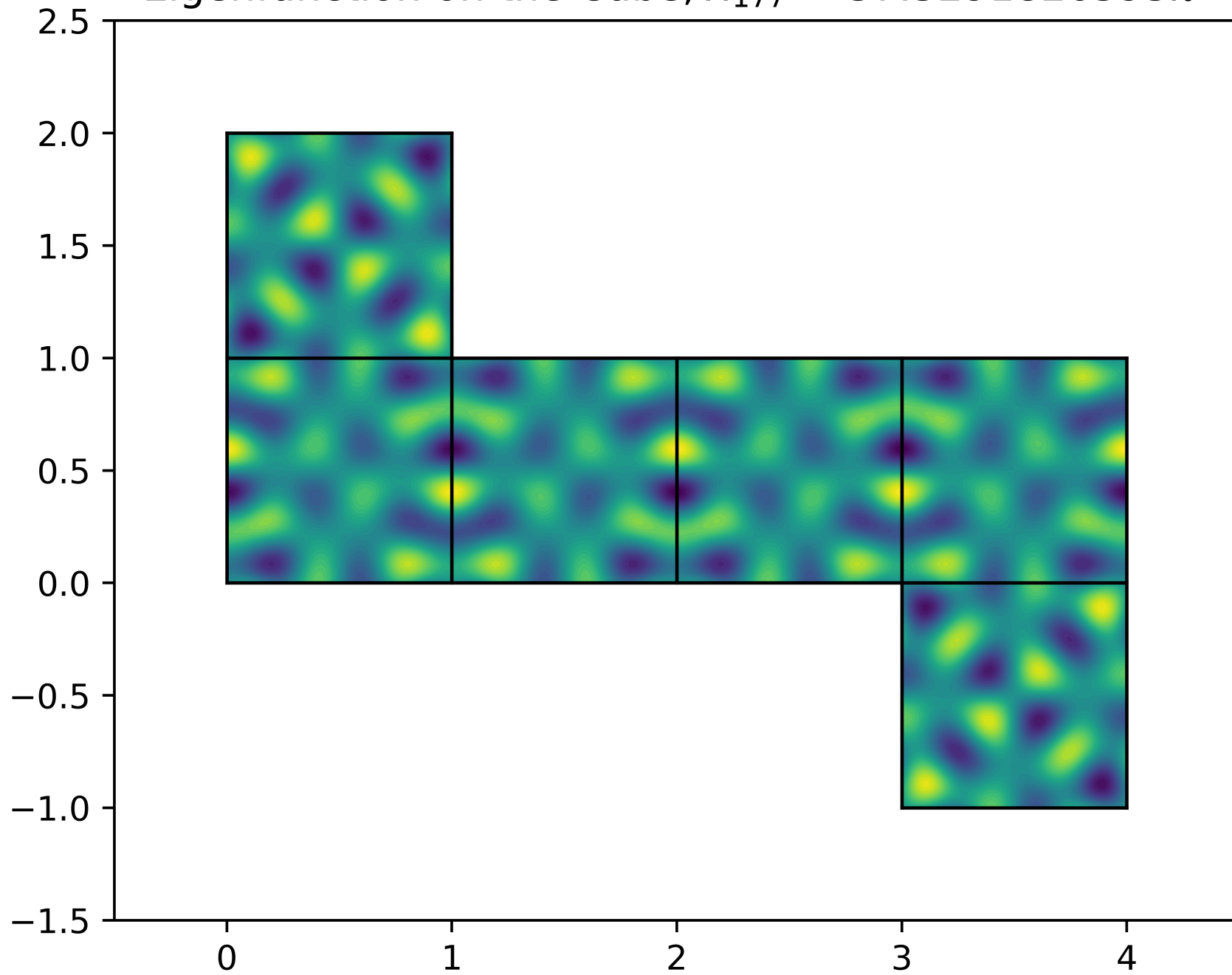
Eigenfunction on the Cube, \lambda_{177} = 37.3291826593\pi^2
