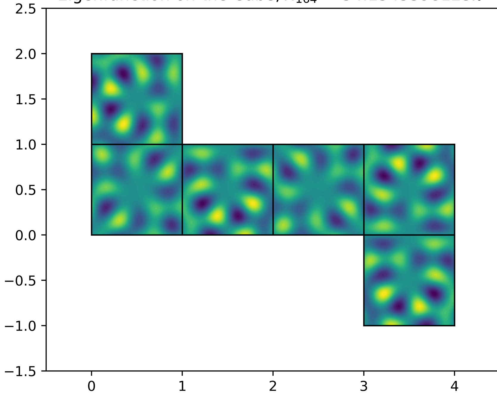
Eigenfunction on the Cube, \lambda_{164} = 34.1545398123\pi^2
