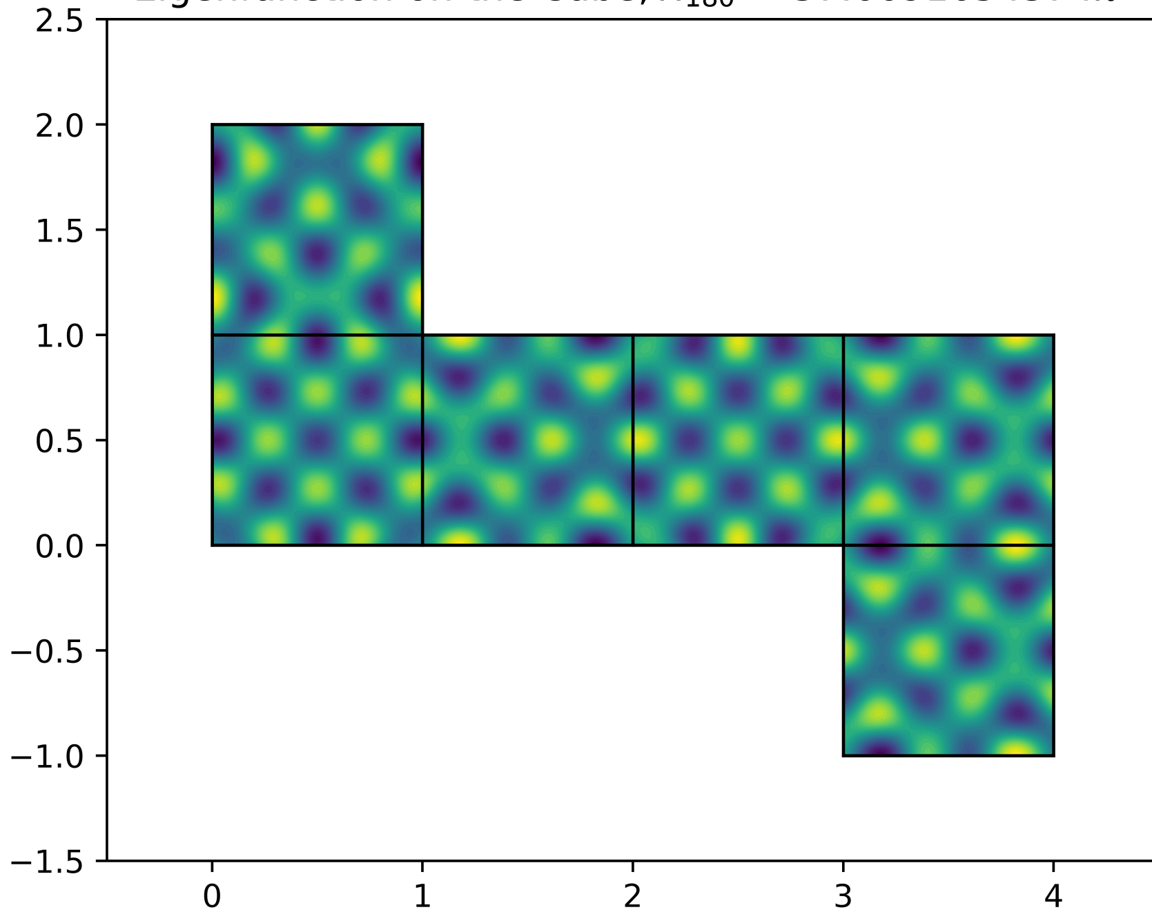
Eigenfunction on the Cube, \lambda_{180} = 37.6691654374\pi^2
