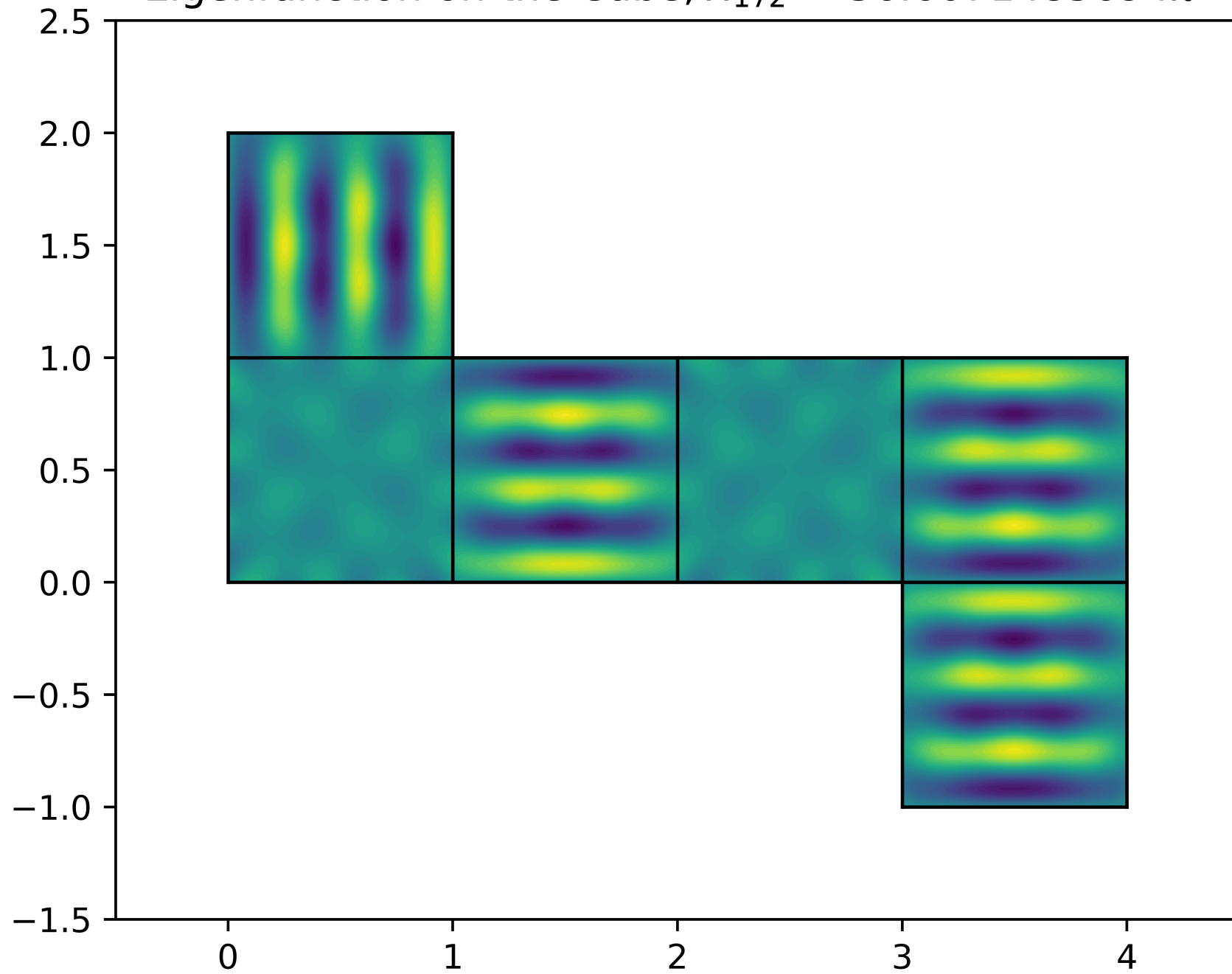
Eigenfunction on the Cube, \lambda_{172} = 36.6071485694\pi^2
