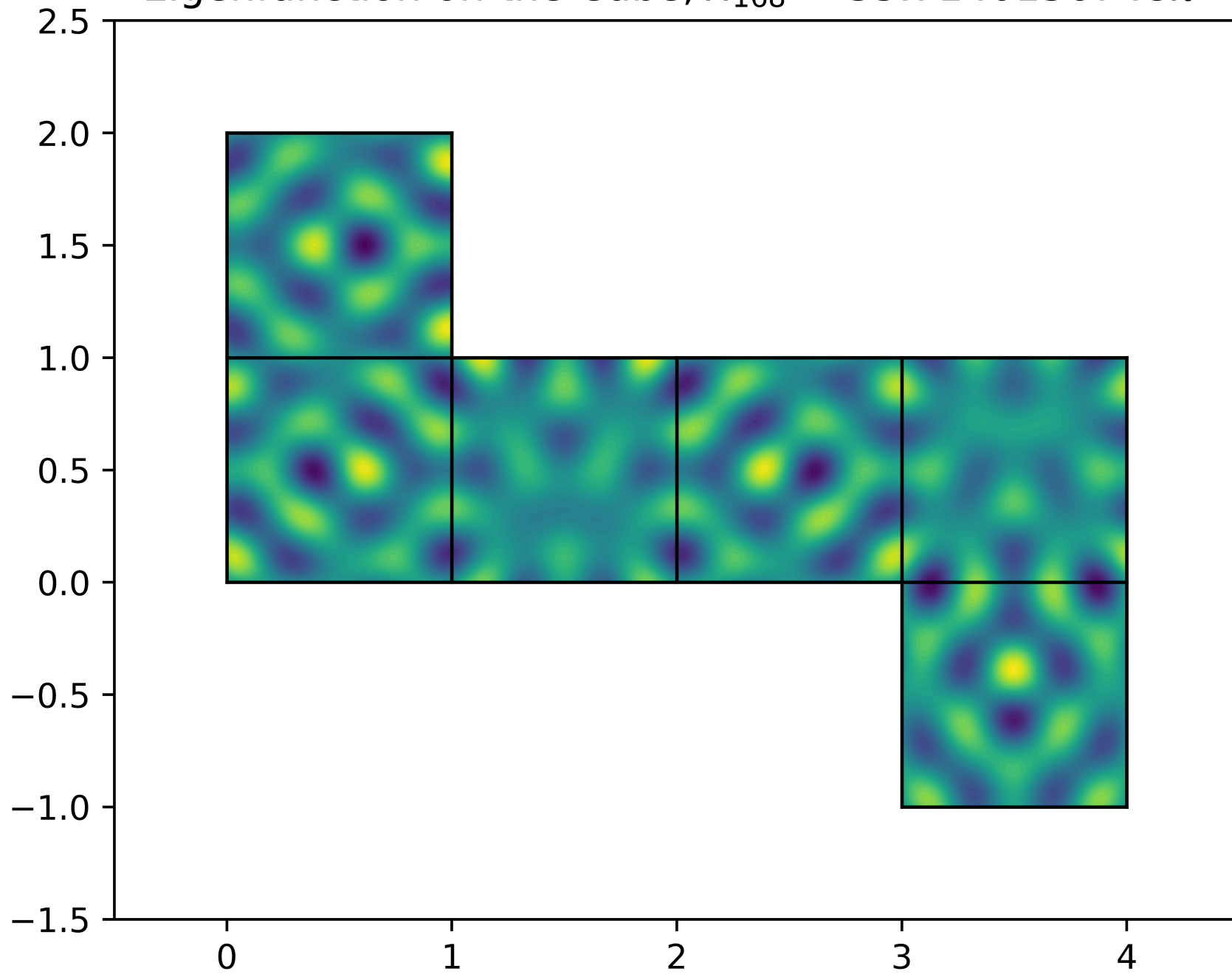
Eigenfunction on the Cube, \lambda_{168} = 35.7140156748\pi^2
