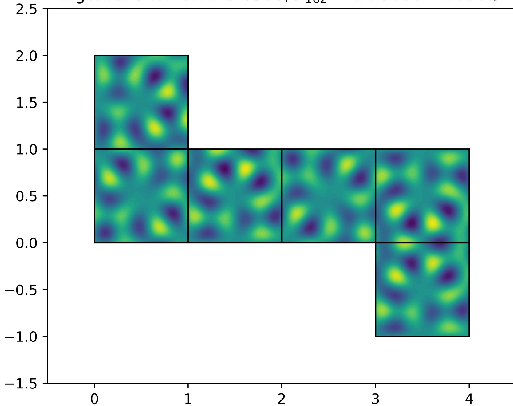
Eigenfunction on the Cube, \lambda_{162} = 34.0886742398\pi^2
