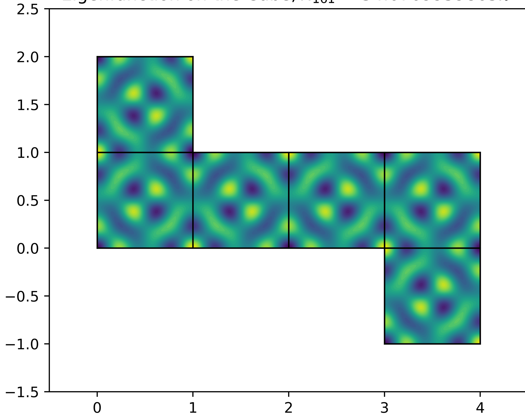
Eigenfunction on the Cube, \lambda_{161} = 34.0709959865\pi^2
