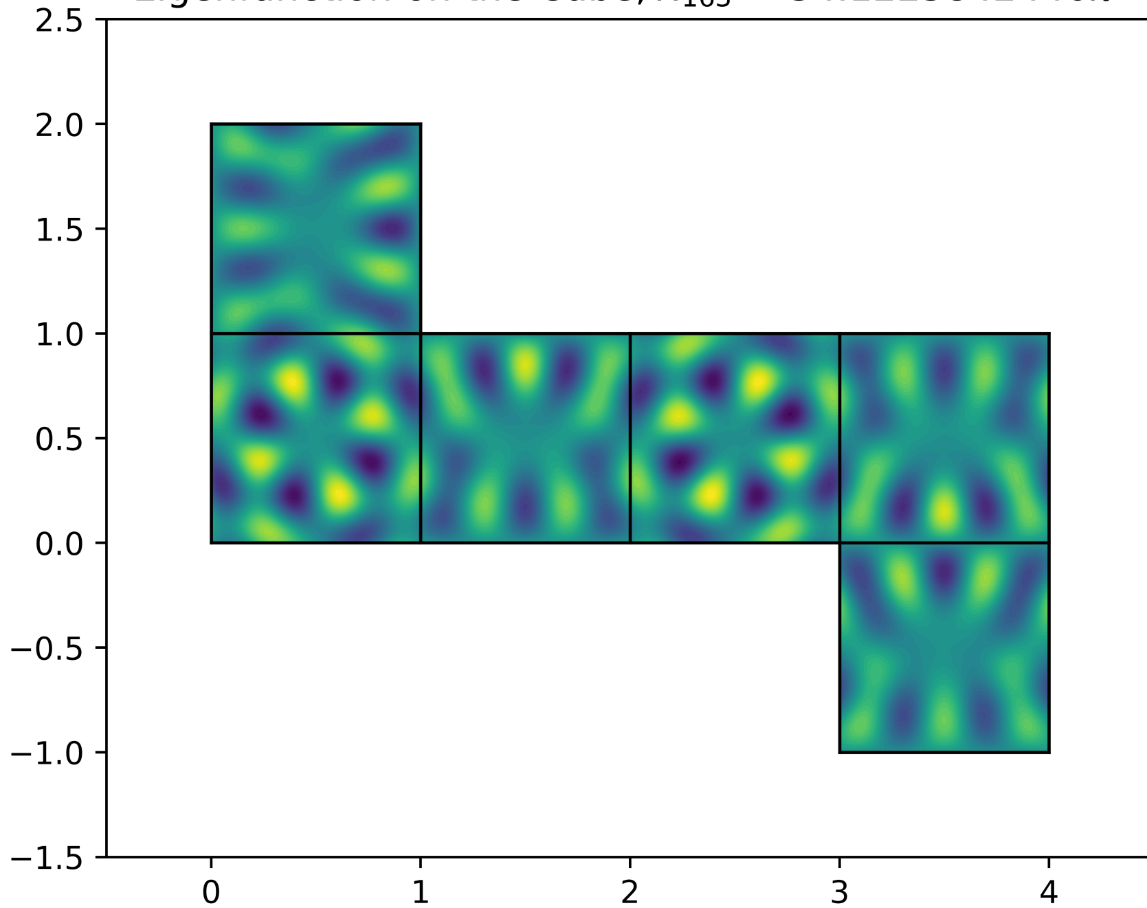
Eigenfunction on the Cube, \lambda_{163} = 34.1225842446\pi^2
