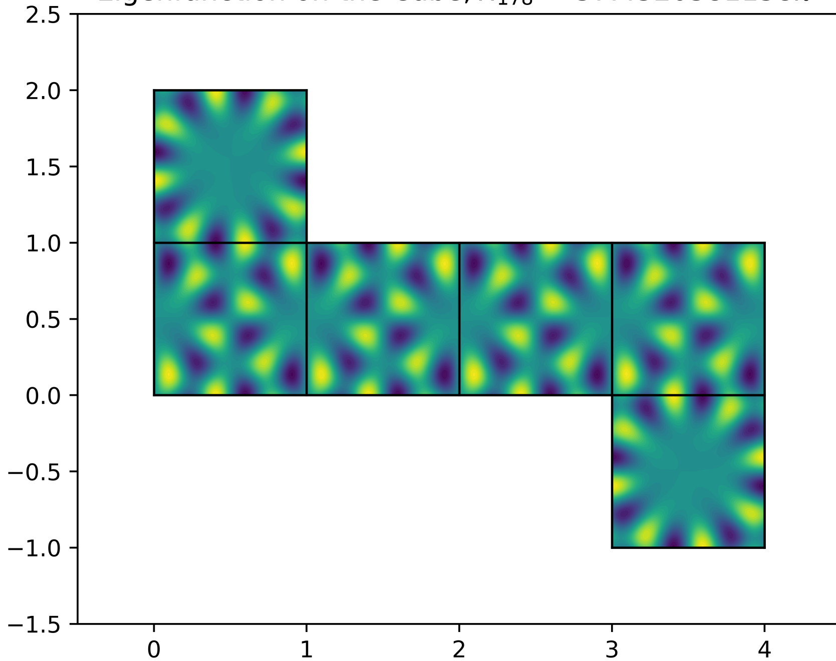
Eigenfunction on the Cube, \lambda_{178} = 37.4320381158\pi^2
