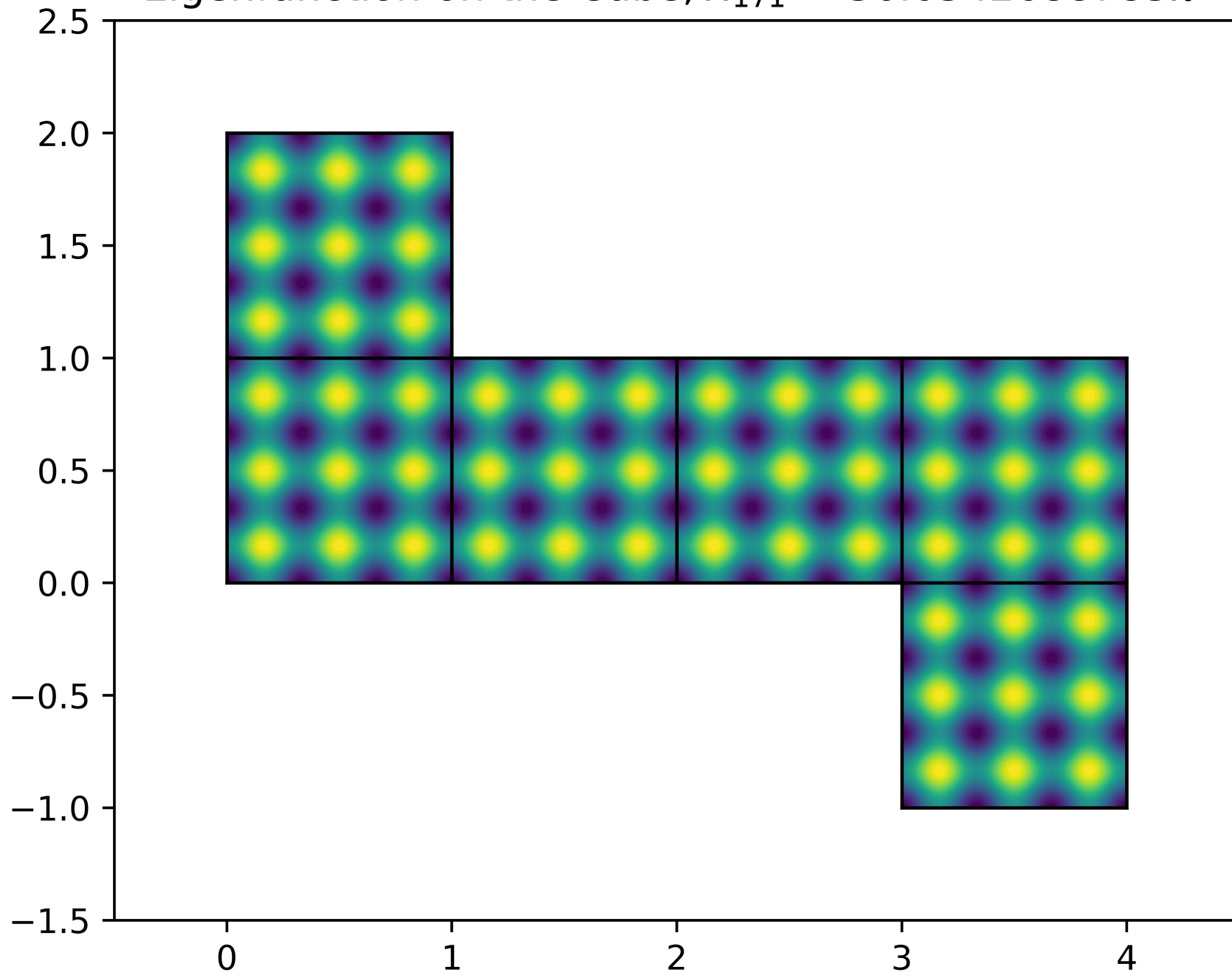
Eigenfunction on the Cube, \lambda_{171} = 36.0542688783\pi^2
