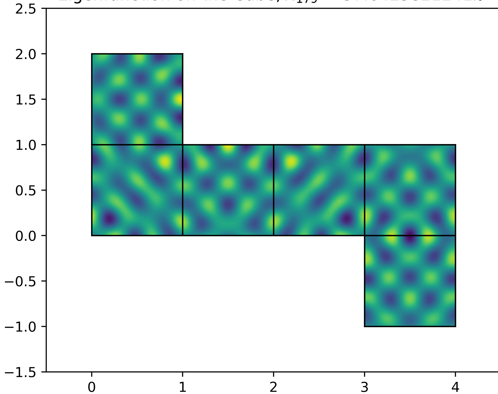
Eigenfunction on the Cube, \lambda_{179} = 37.6425821241\pi^2
