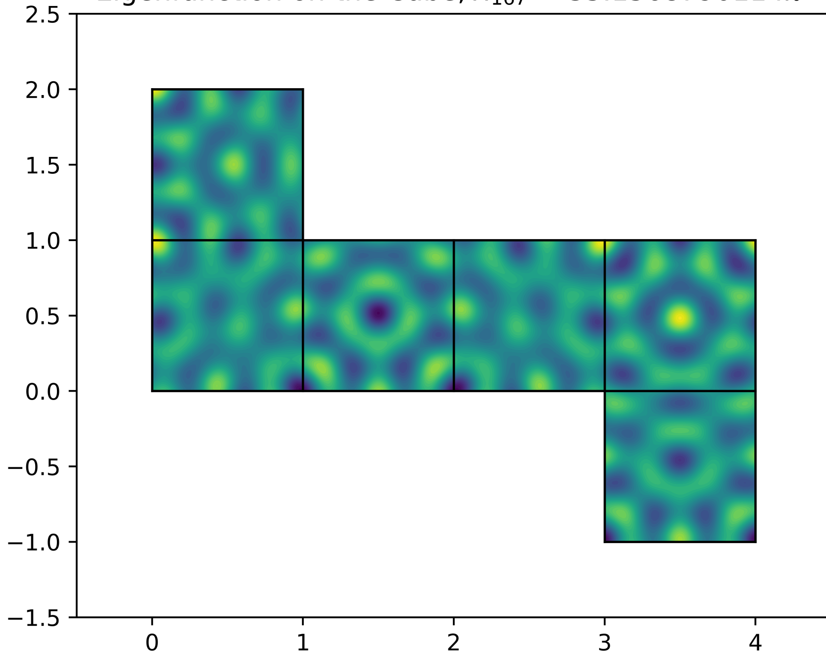
Eigenfunction on the Cube, \lambda_{167} = 35.1568790114\pi^2
