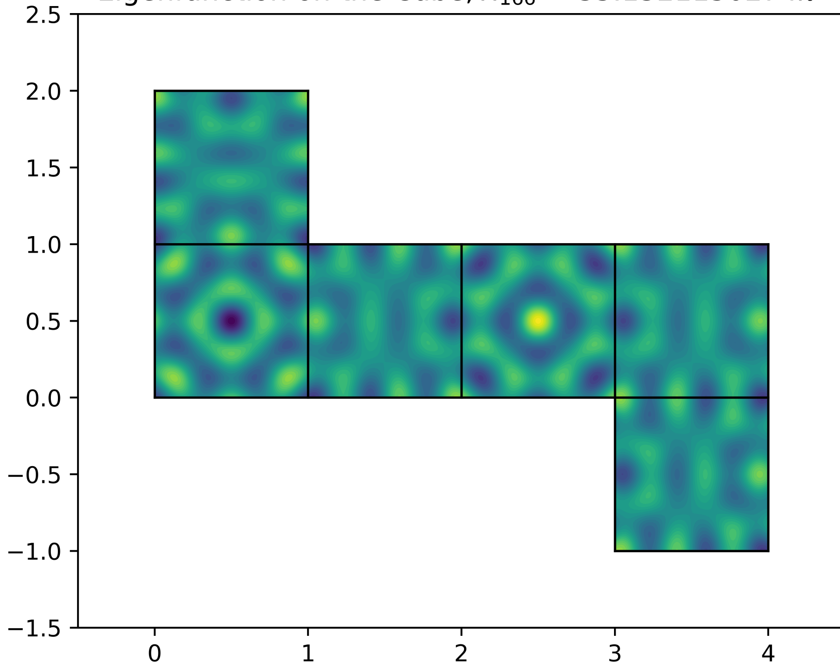
Eigenfunction on the Cube, \lambda_{166} = 35.1321150274\pi^2
