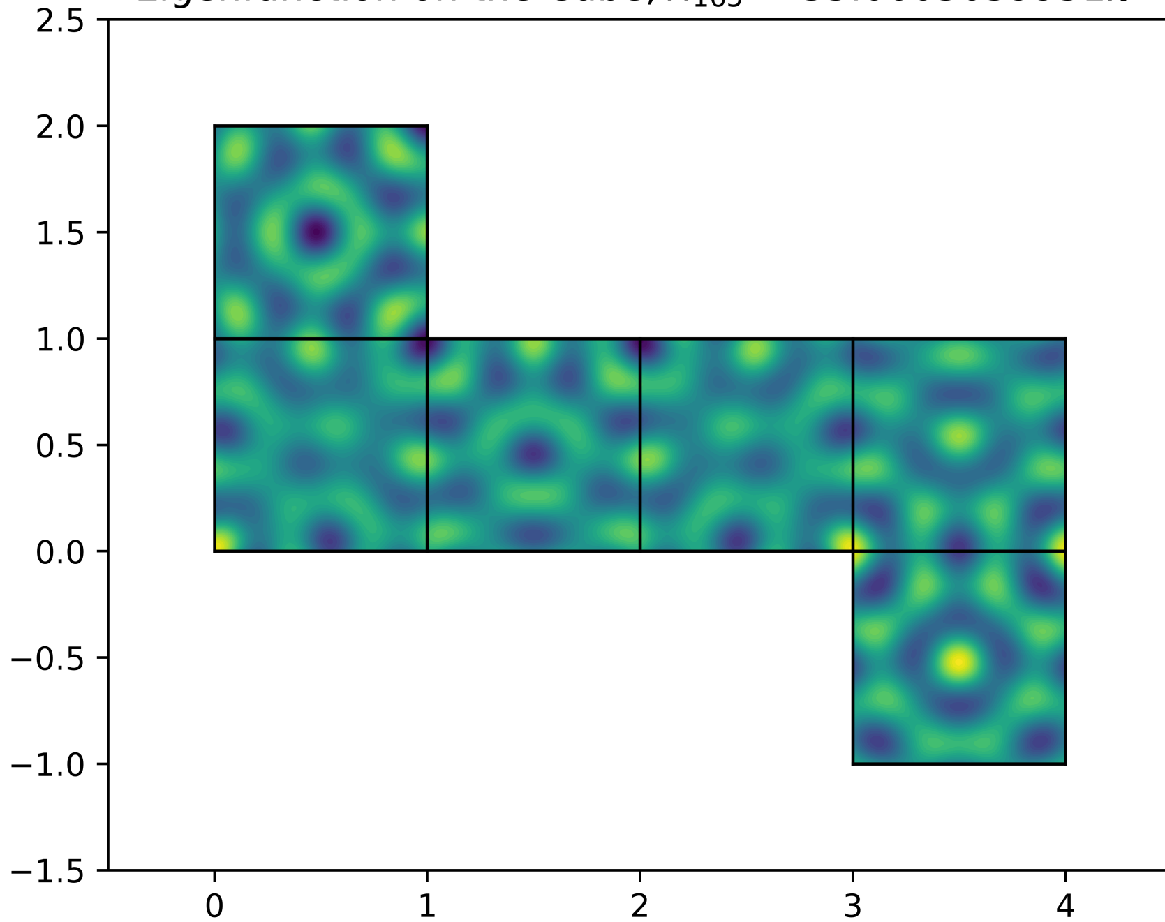
Eigenfunction on the Cube, \lambda_{165} = 35.0603059951\pi^2
