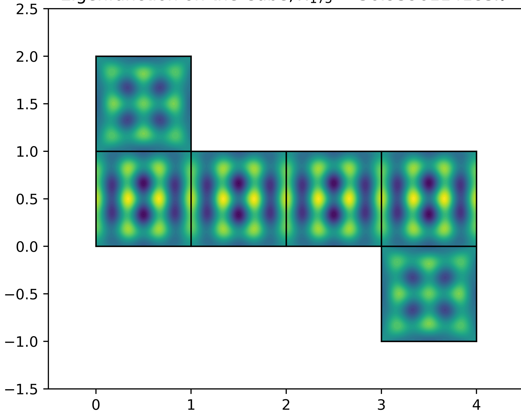
Eigenfunction on the Cube, \lambda_{175} = 36.9396114183\pi^2
