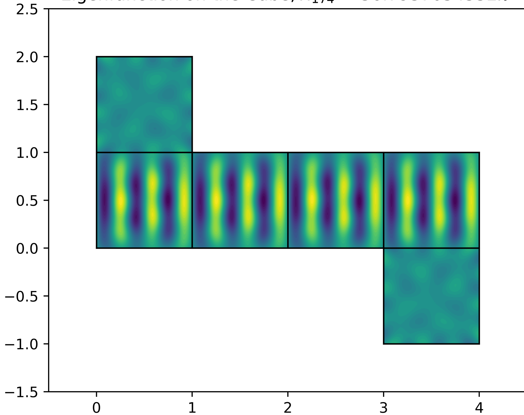
Eigenfunction on the Cube, \lambda_{174} = 36.7937054532\pi^2
