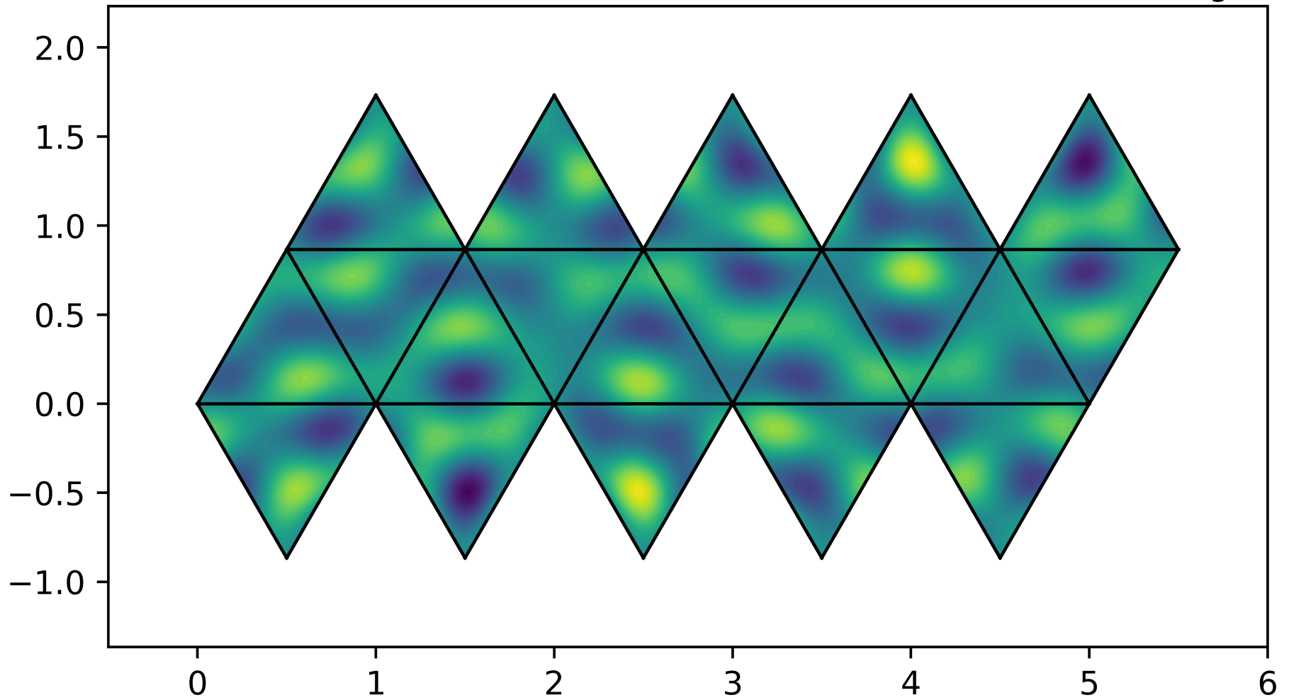
Eigenfunction on the Icosahedron, \lambda_{95} = 10.2769328408\frac{4}{3}\pi^2
