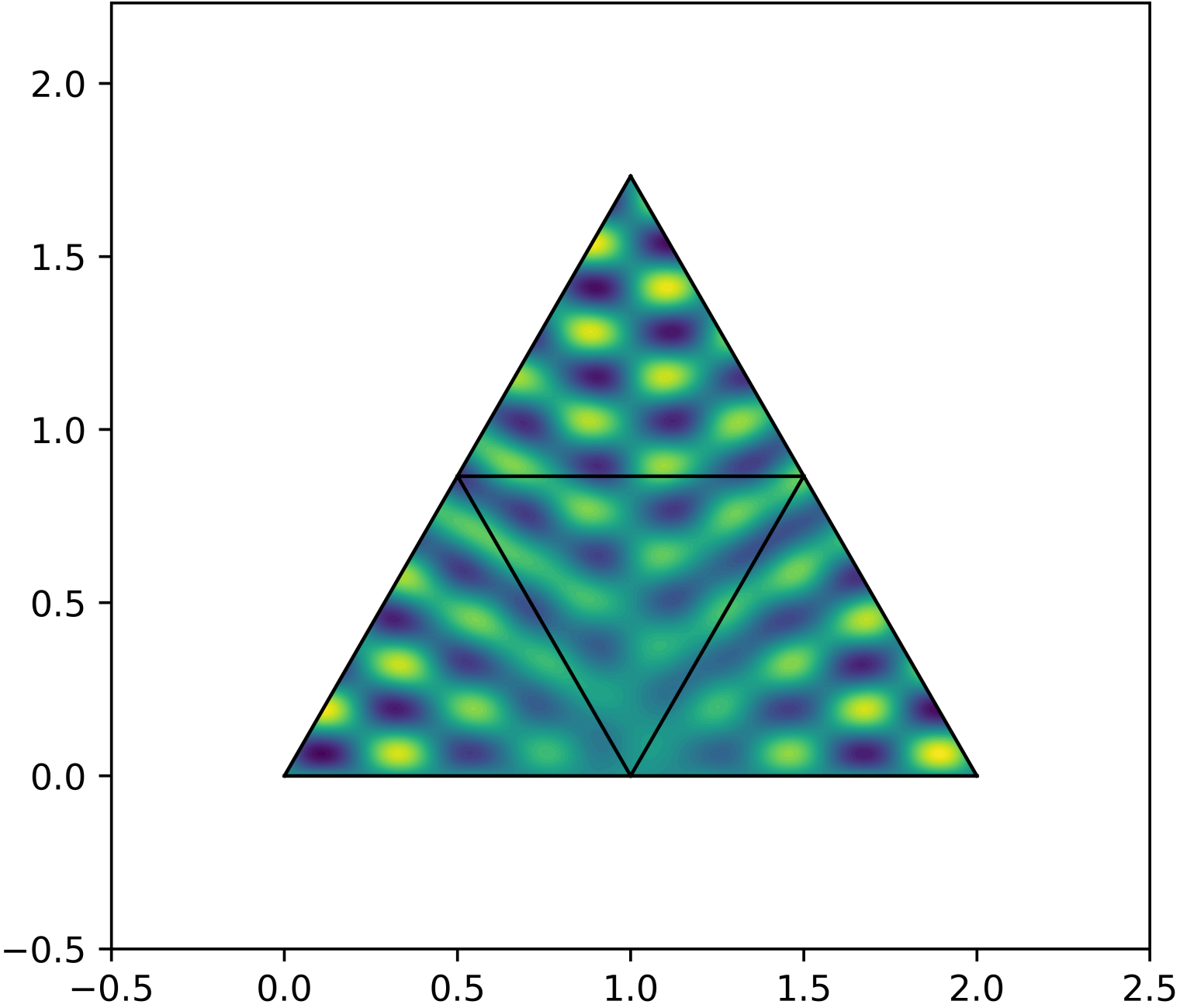
Eigenfunction on the Tetrahedron, \lambda_{107} = 61.0467147937\frac{4}{3}\pi^2
