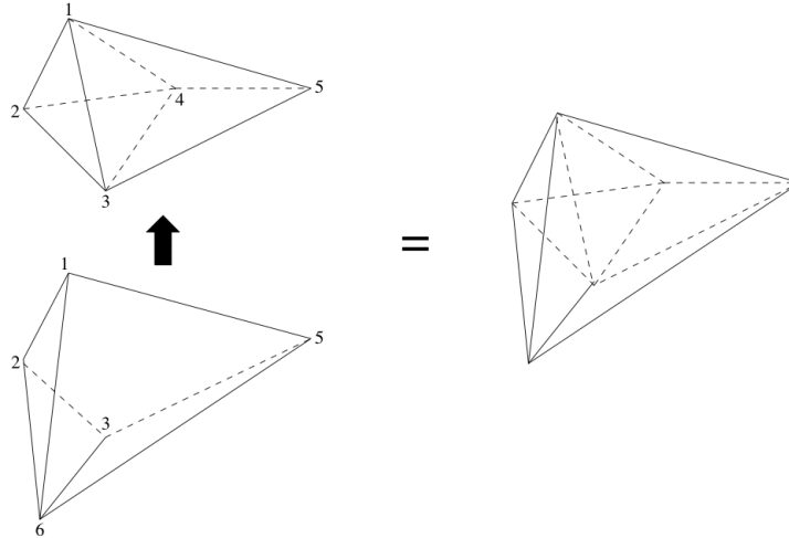
Figure 2: Attaching \Sigma_3 to \Sigma_1 \cup \Sigma_2 .
