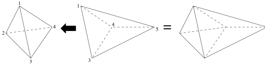
Figure 1: Attaching \Sigma_2 to \Sigma_1 .
