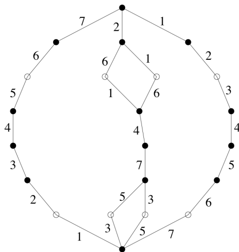
Figure 3: Maximal chains whose labels are in C(\sigma) . Elements whose ranks are in S \cup \{0, 7\} are filled in.
