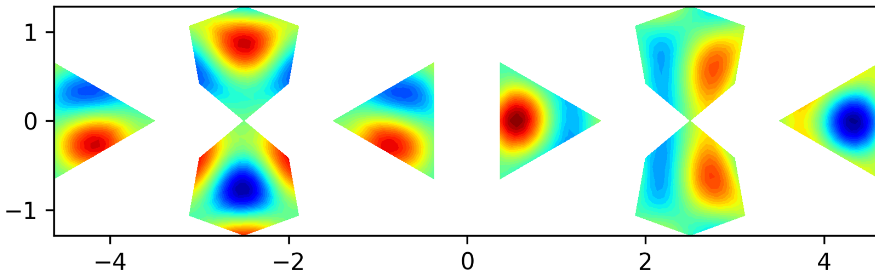
Eigenfunction 19 on the level 1 polyhedron, EV = 36.0815
