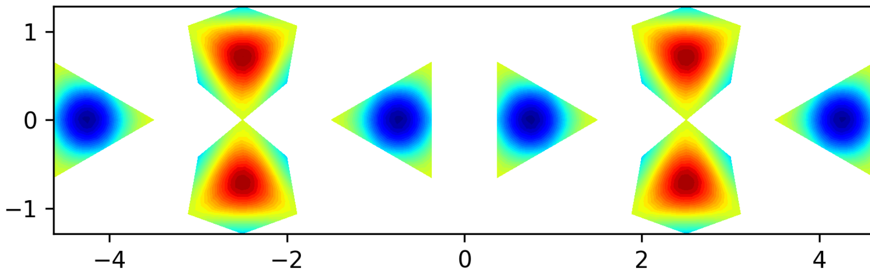
Eigenfunction 15 on the level 1 polyhedron, EV = 21.9988
