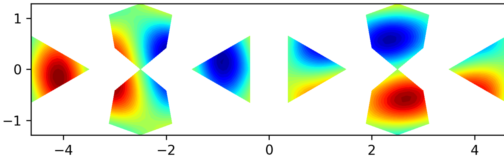
Eigenfunction 7 on the level 1 polyhedron, EV = 10.6381
