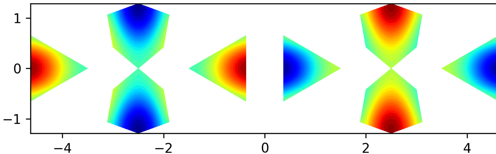
Eigenfunction 6 on the level 1 polyhedron, EV = 10.6066
