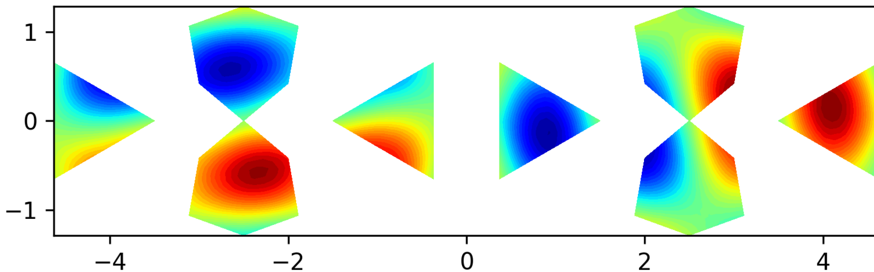
Eigenfunction 8 on the level 1 polyhedron, EV = 10.6381
