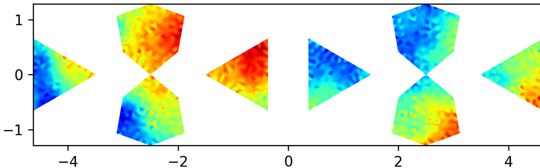
Eigenfunction 0 on the level 1 polyhedron, EV = 0.0
