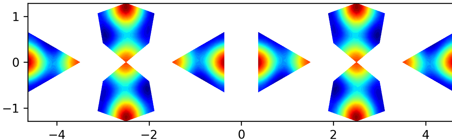
Eigenfunction 17 on the level 1 polyhedron, EV = 33.8099
