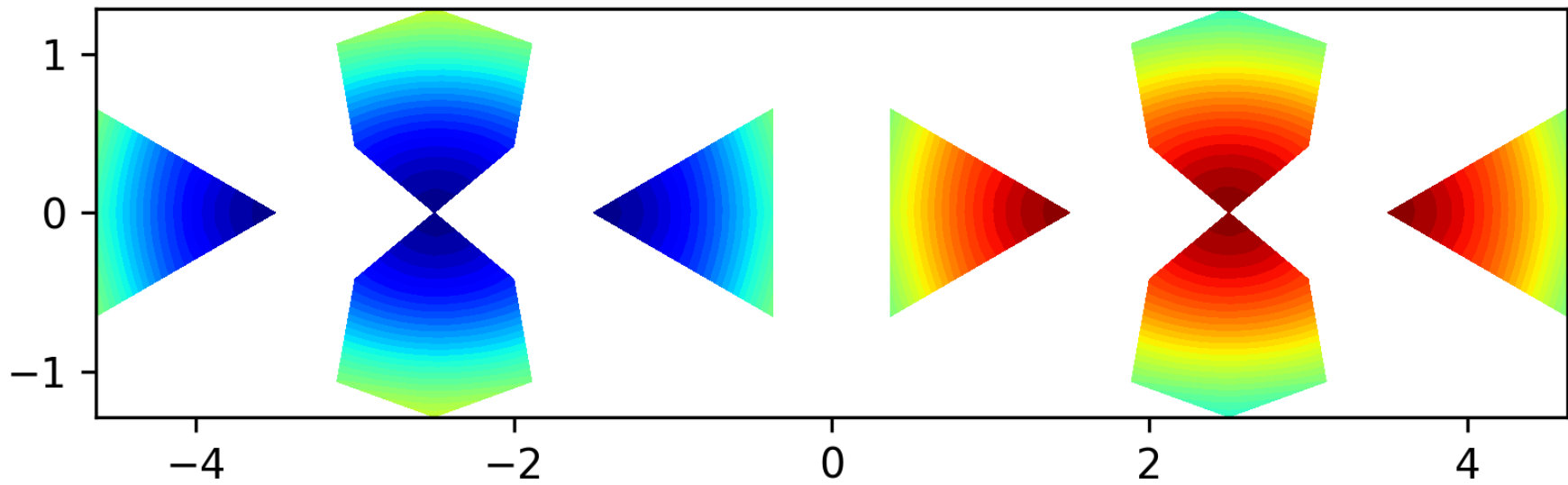
Eigenfunction 3 on the level 1 polyhedron, EV = 3.4866
