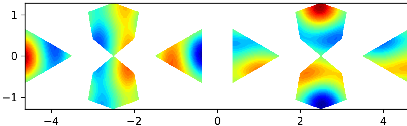
Eigenfunction 10 on the level 1 polyhedron, EV = 20.822
