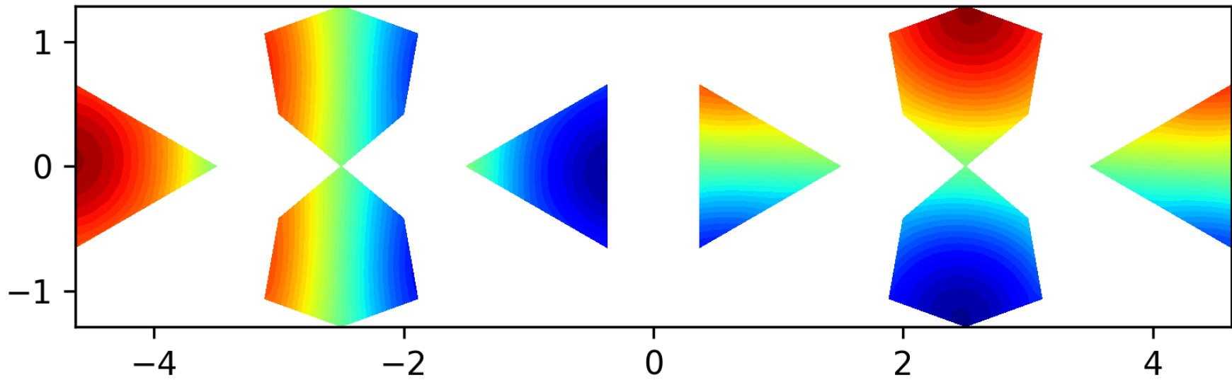
Eigenfunction 1 on the level 1 polyhedron, EV = 3.4819
