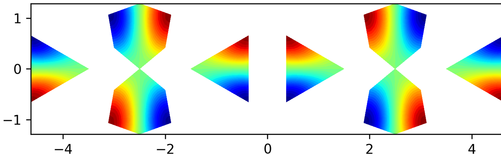
Eigenfunction 4 on the level 1 polyhedron, EV = 10.3246
