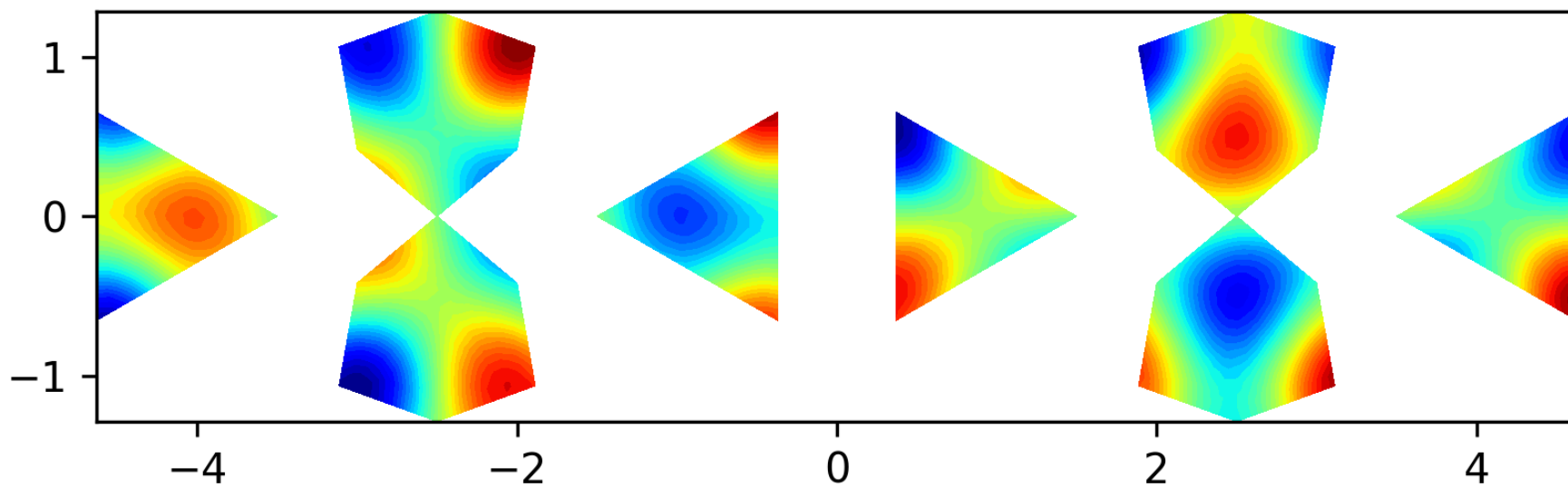
Eigenfunction 13 on the level 1 polyhedron, EV = 21.1268
