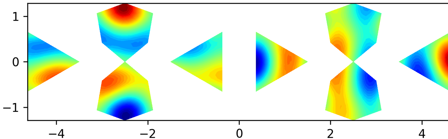
Eigenfunction 9 on the level 1 polyhedron, EV = 20.8213
