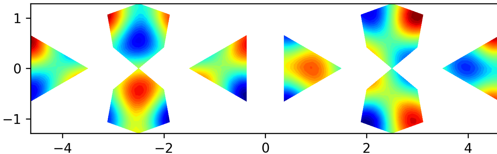
Eigenfunction 12 on the level 1 polyhedron, EV = 21.1259
