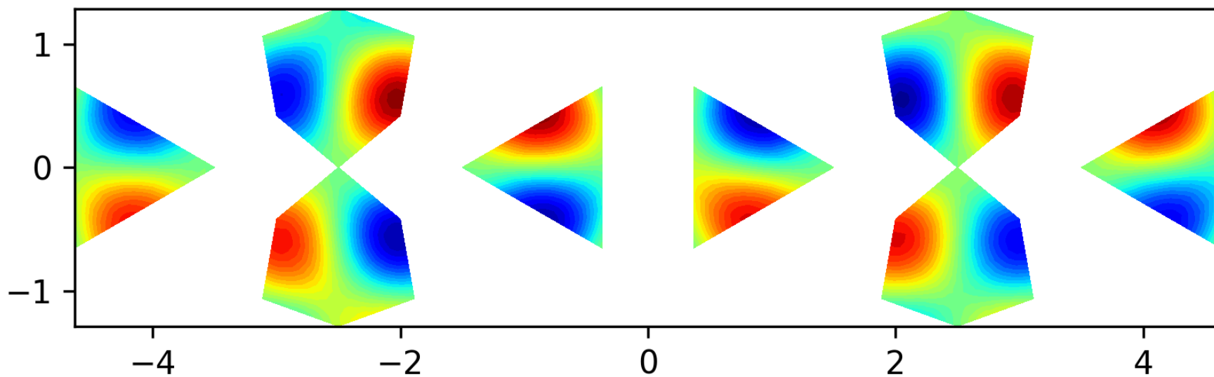
Eigenfunction 11 on the level 1 polyhedron, EV = 20.8586
