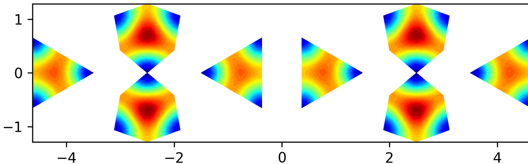
Eigenfunction 18 on the level 1 polyhedron, EV = 34.5699
