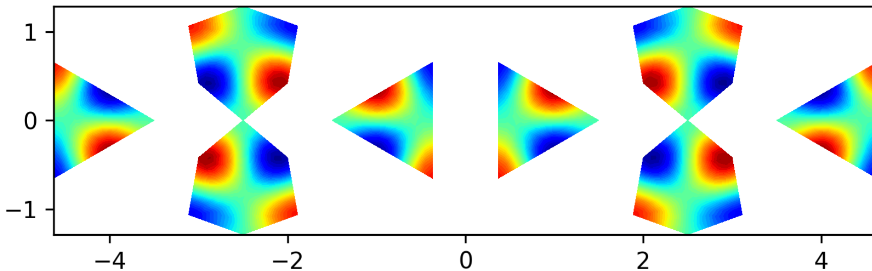
Eigenfunction 16 on the level 1 polyhedron, EV = 33.8085
