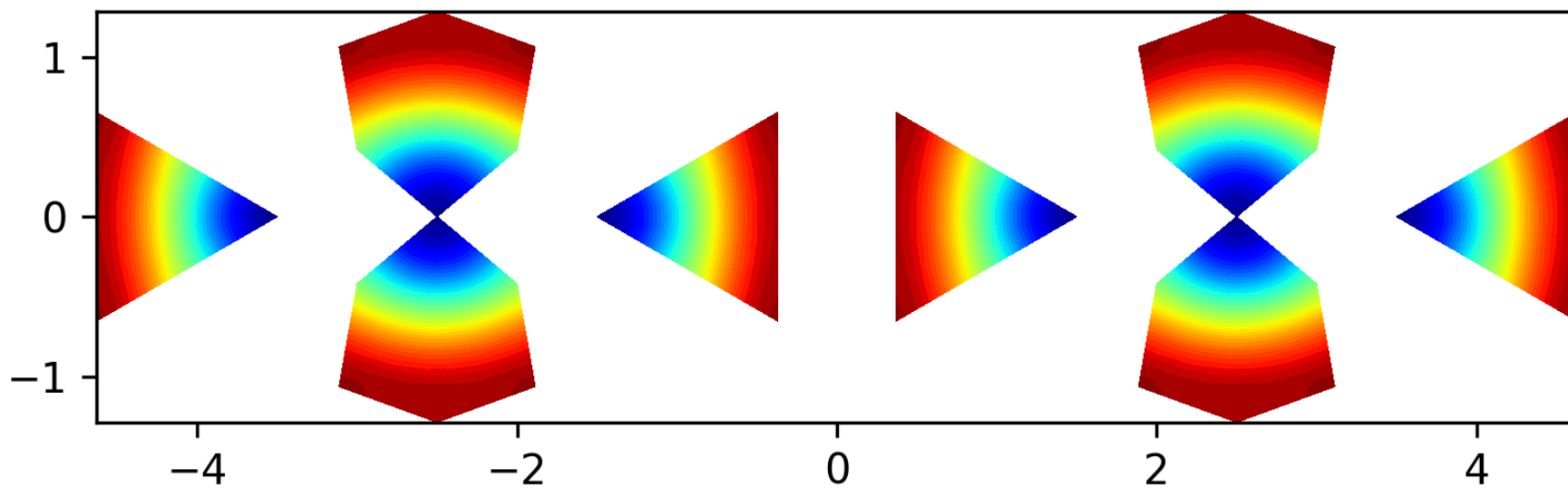
Eigenfunction 5 on the level 1 polyhedron, EV = 10.3298
