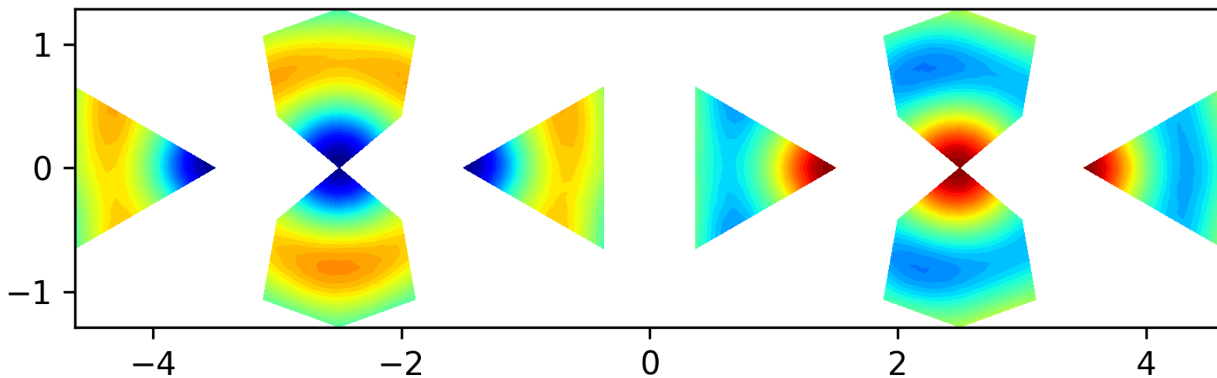
Eigenfunction 14 on the level 1 polyhedron, EV = 21.1598
