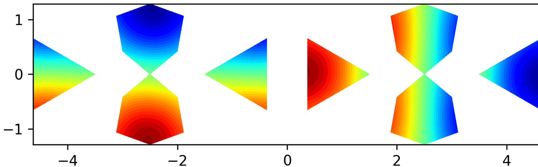
Eigenfunction 2 on the level 1 polyhedron, EV = 3.4819
