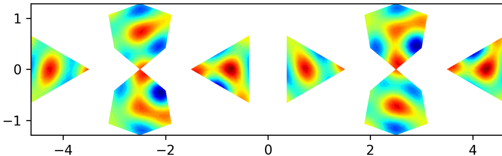
Eigenfunction 39 on the level 1 polyhedron, EV = 74.735
