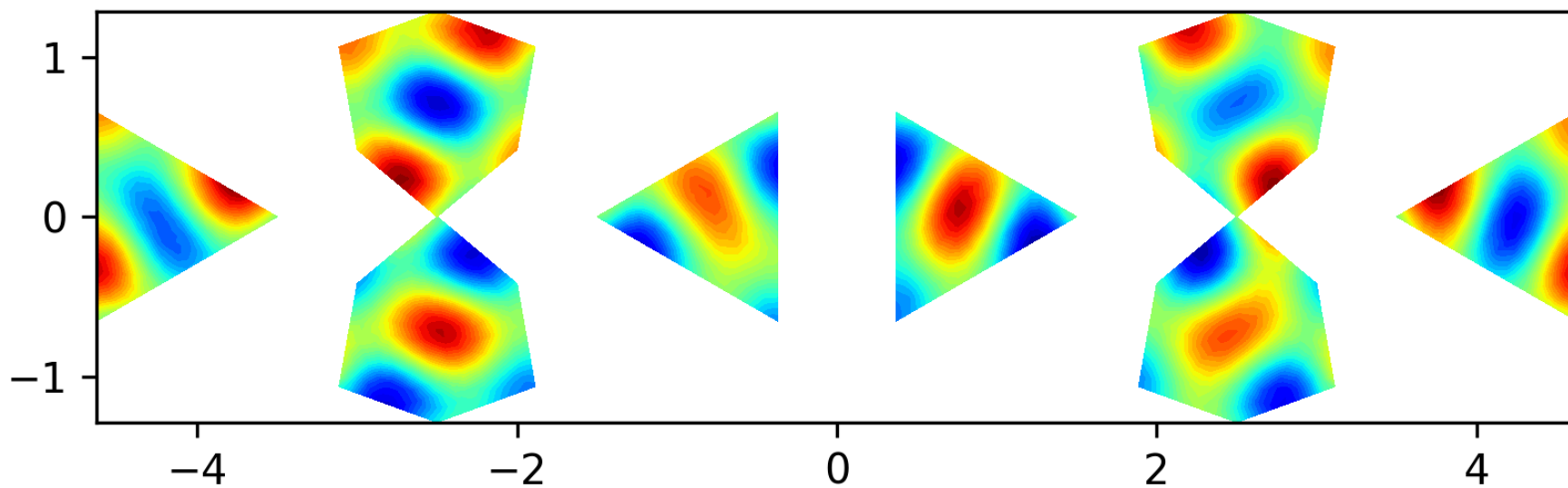
Eigenfunction 32 on the level 1 polyhedron, EV = 54.723
