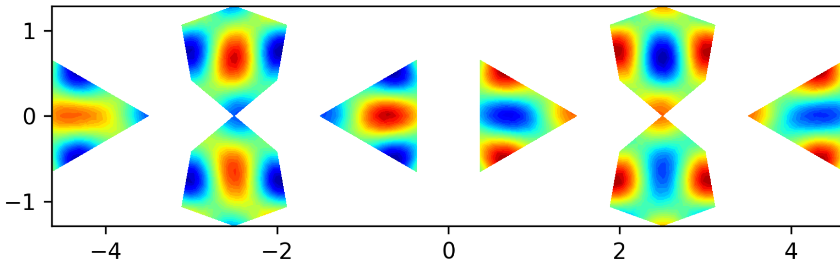
Eigenfunction 33 on the level 1 polyhedron, EV = 54.8962
