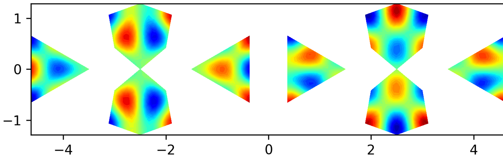
Eigenfunction 26 on the level 1 polyhedron, EV = 52.082
