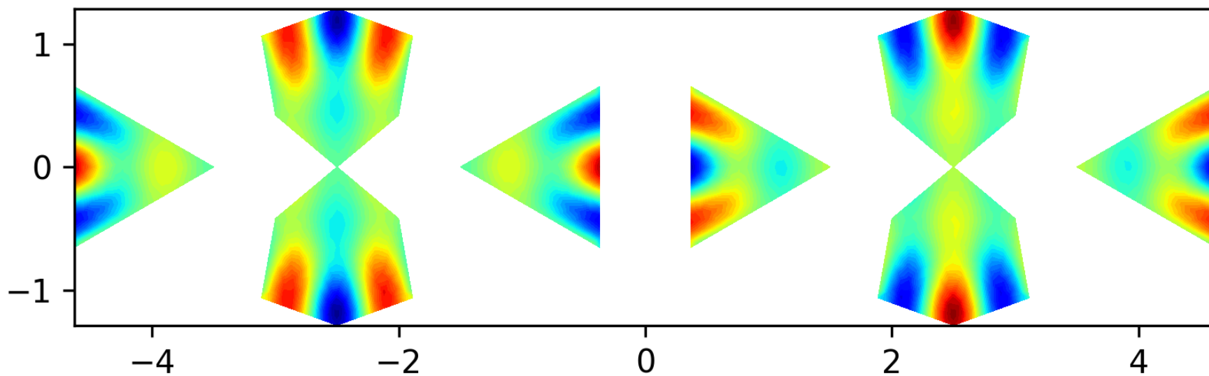
Eigenfunction 36 on the level 1 polyhedron, EV = 74.1275
