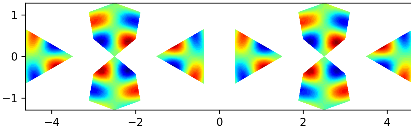
Eigenfunction 30 on the level 1 polyhedron, EV = 53.557
