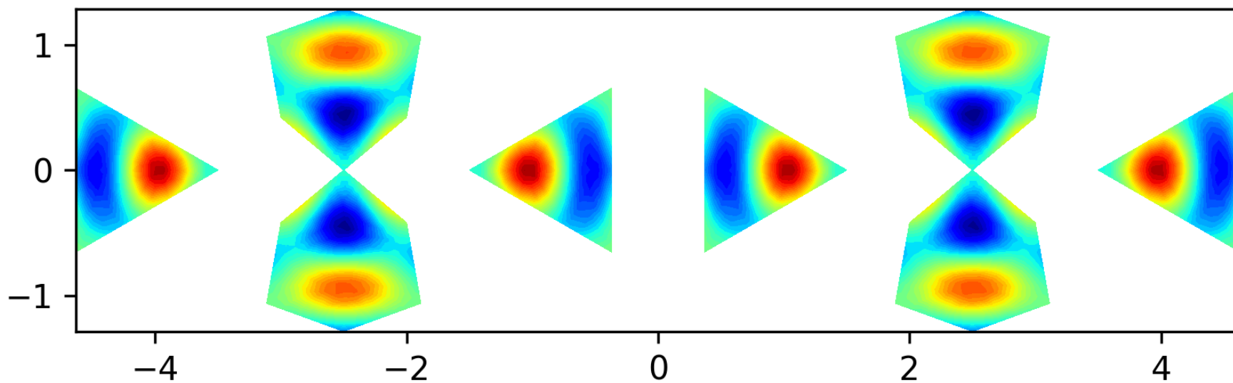
Eigenfunction 35 on the level 1 polyhedron, EV = 55.7724
