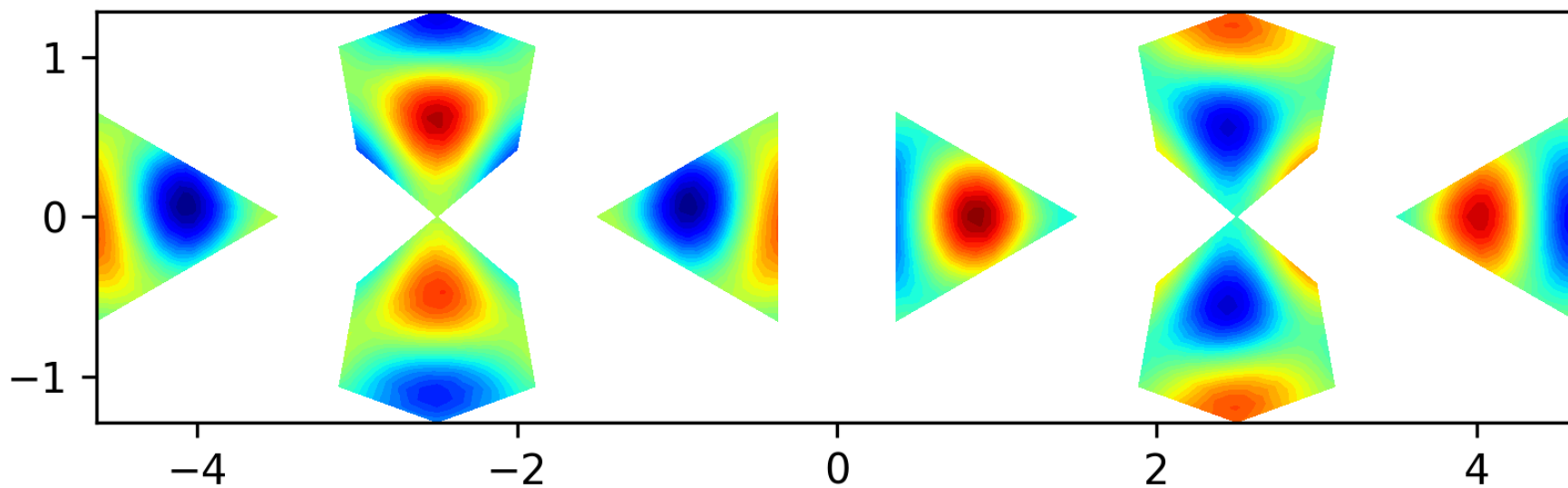
Eigenfunction 21 on the level 1 polyhedron, EV = 36.1097
