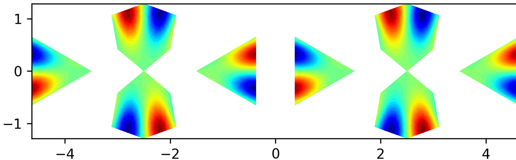
Eigenfunction 22 on the level 1 polyhedron, EV = 36.2352
