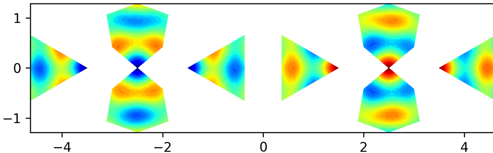
Eigenfunction 27 on the level 1 polyhedron, EV = 52.2478
