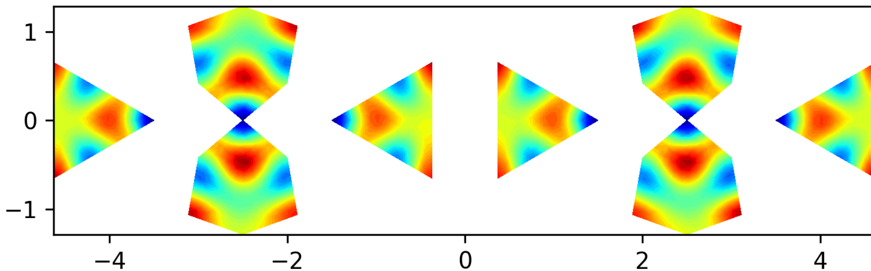
Eigenfunction 38 on the level 1 polyhedron, EV = 74.2037
