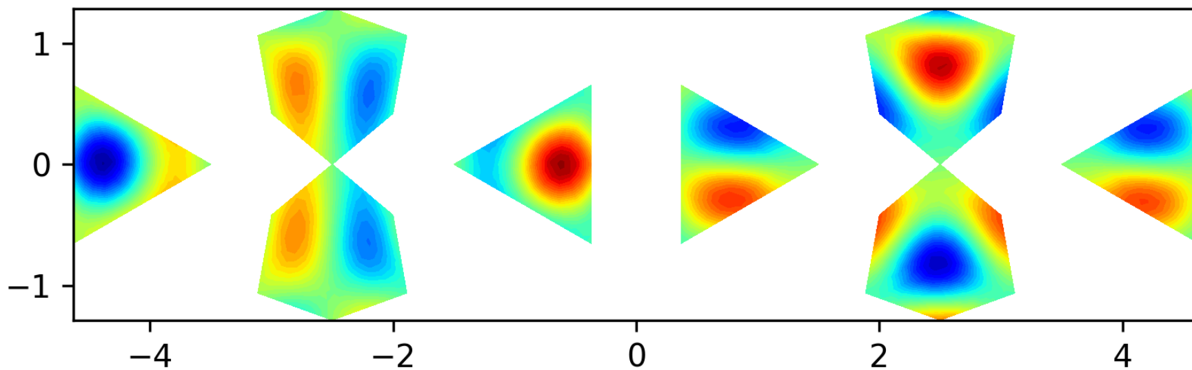
Eigenfunction 20 on the level 1 polyhedron, EV = 36.0838
