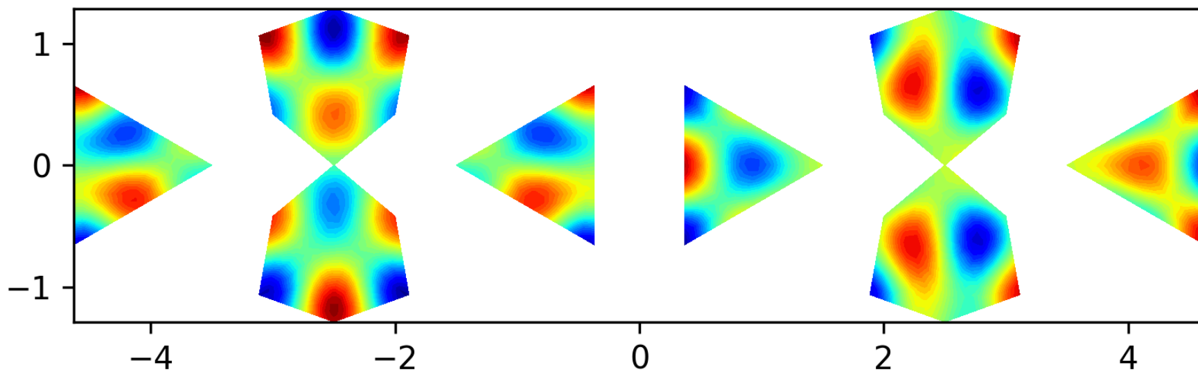
Eigenfunction 25 on the level 1 polyhedron, EV = 52.0811
