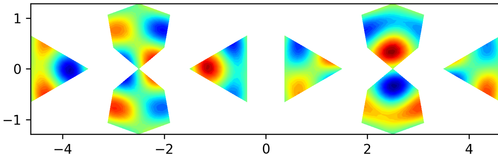
Eigenfunction 23 on the level 1 polyhedron, EV = 36.4358
