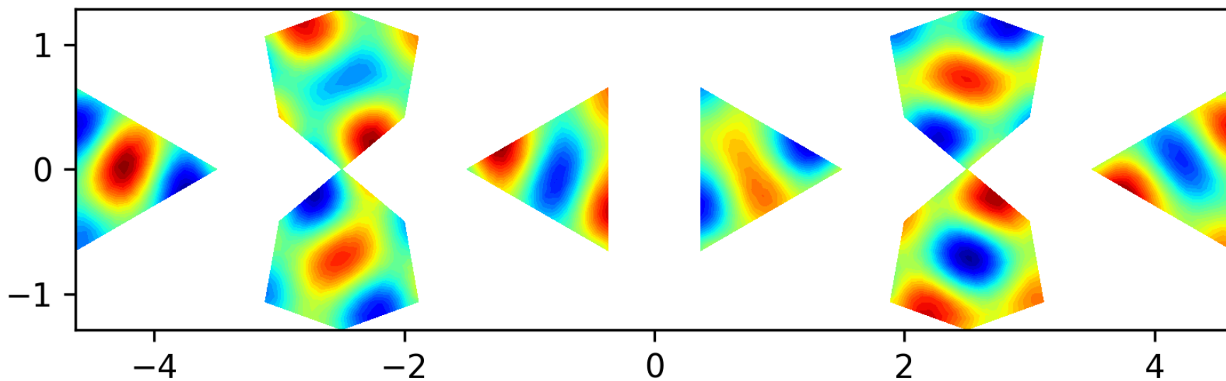
Eigenfunction 31 on the level 1 polyhedron, EV = 54.7186
