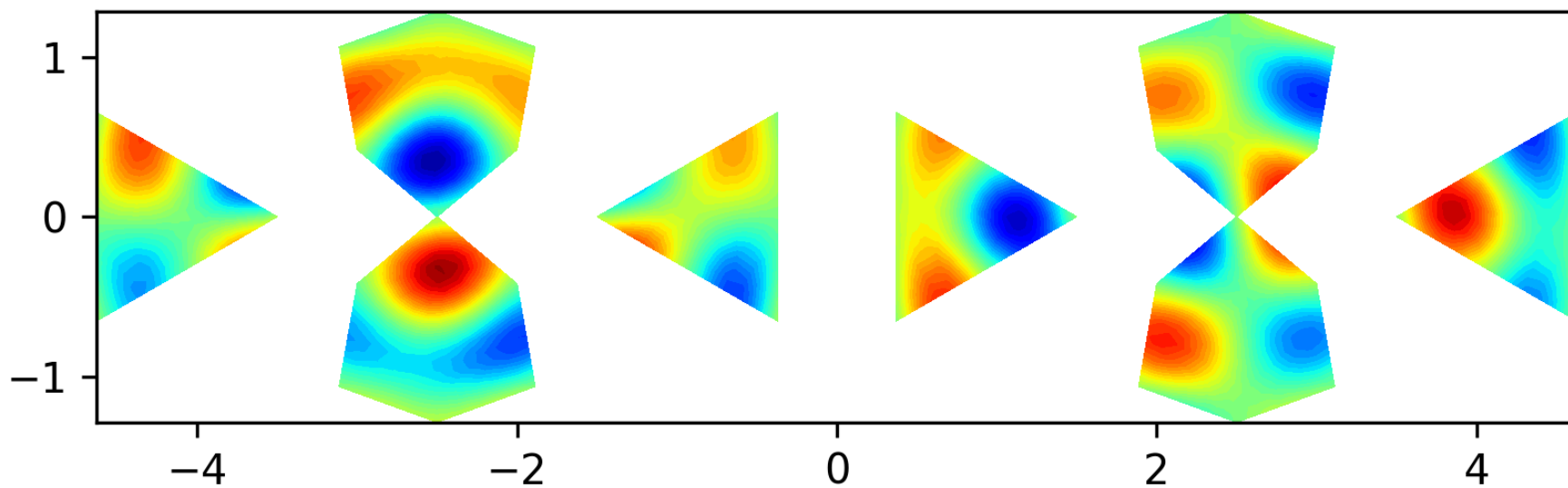
Eigenfunction 24 on the level 1 polyhedron, EV = 36.4366
