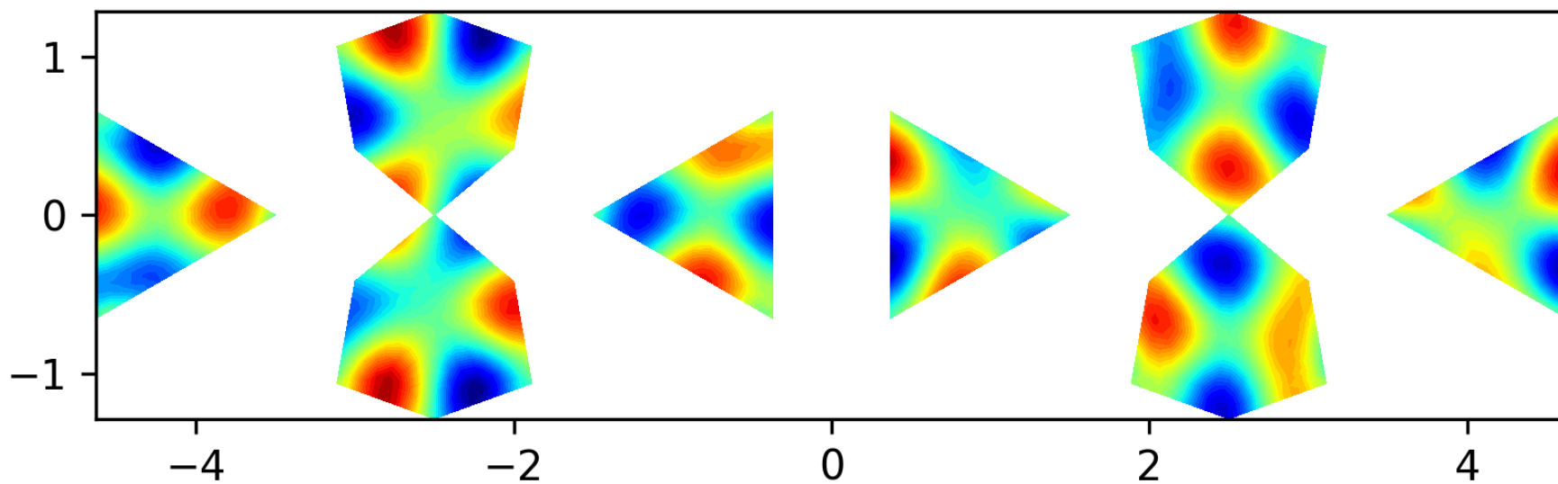
Eigenfunction 28 on the level 1 polyhedron, EV = 53.3419
