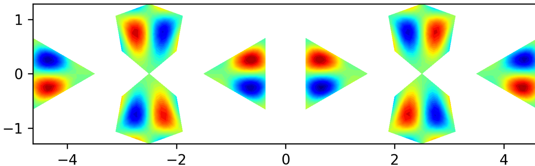
Eigenfunction 34 on the level 1 polyhedron, EV = 55.6
