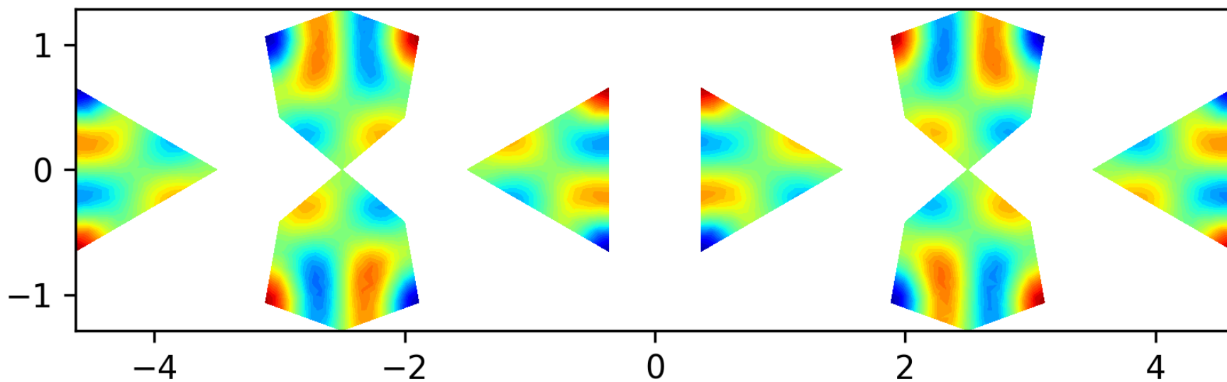
Eigenfunction 37 on the level 1 polyhedron, EV = 74.1801
