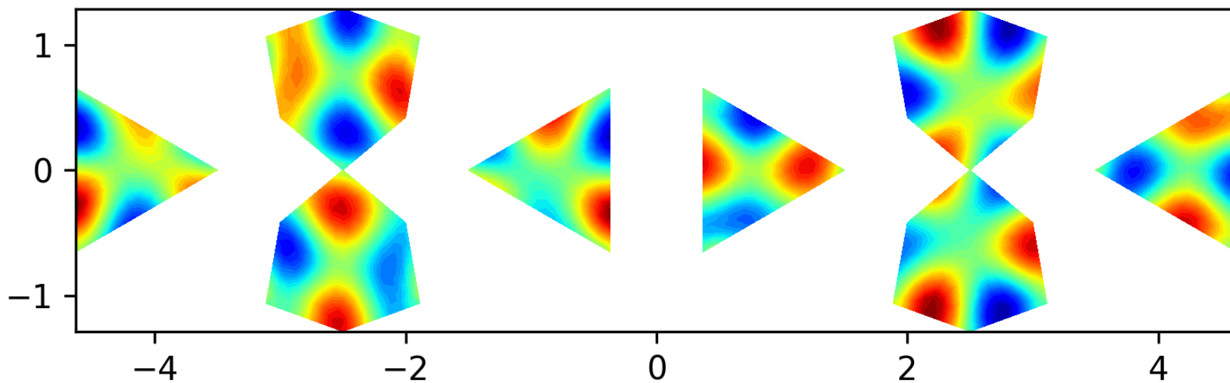
Eigenfunction 29 on the level 1 polyhedron, EV = 53.3429
