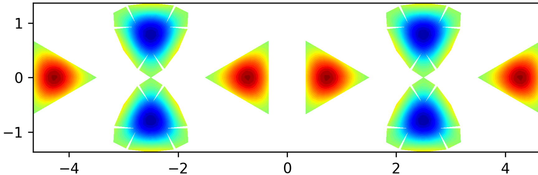
Eigenfunction 15 on the level 2 polyhedron, EV = 19.8077
