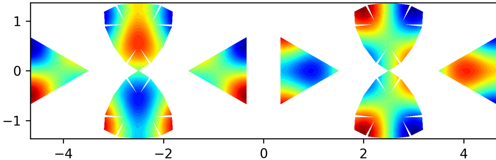
Eigenfunction 9 on the level 2 polyhedron, EV = 18.2078
