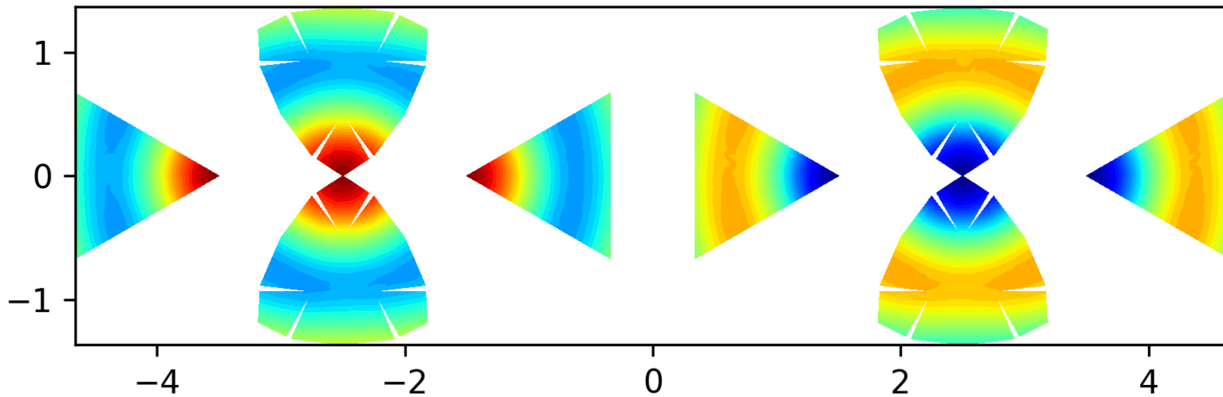
Eigenfunction 11 on the level 2 polyhedron, EV = 18.2201
