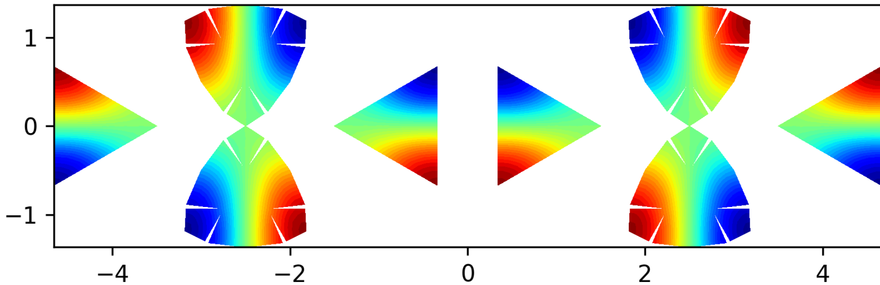
Eigenfunction 4 on the level 2 polyhedron, EV = 8.9231
