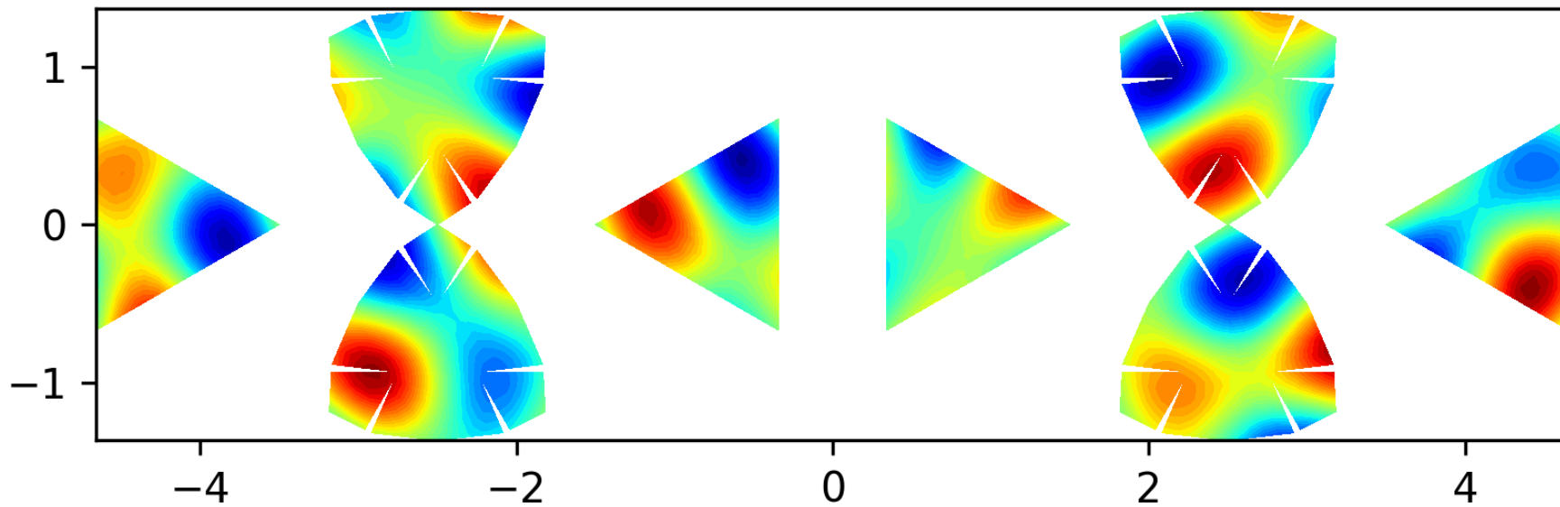
Eigenfunction 17 on the level 2 polyhedron, EV = 30.9367
