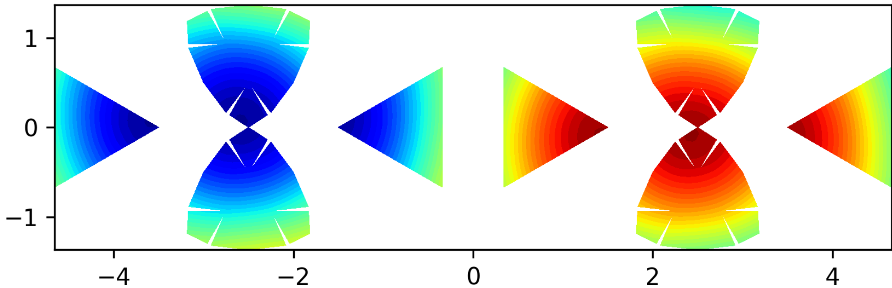
Eigenfunction 3 on the level 2 polyhedron, EV = 3.0989
