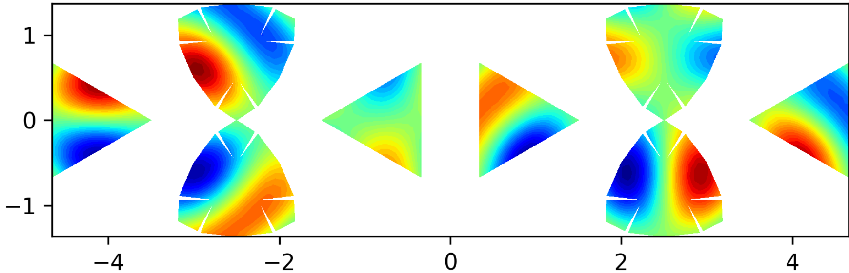
Eigenfunction 14 on the level 2 polyhedron, EV = 18.9604
