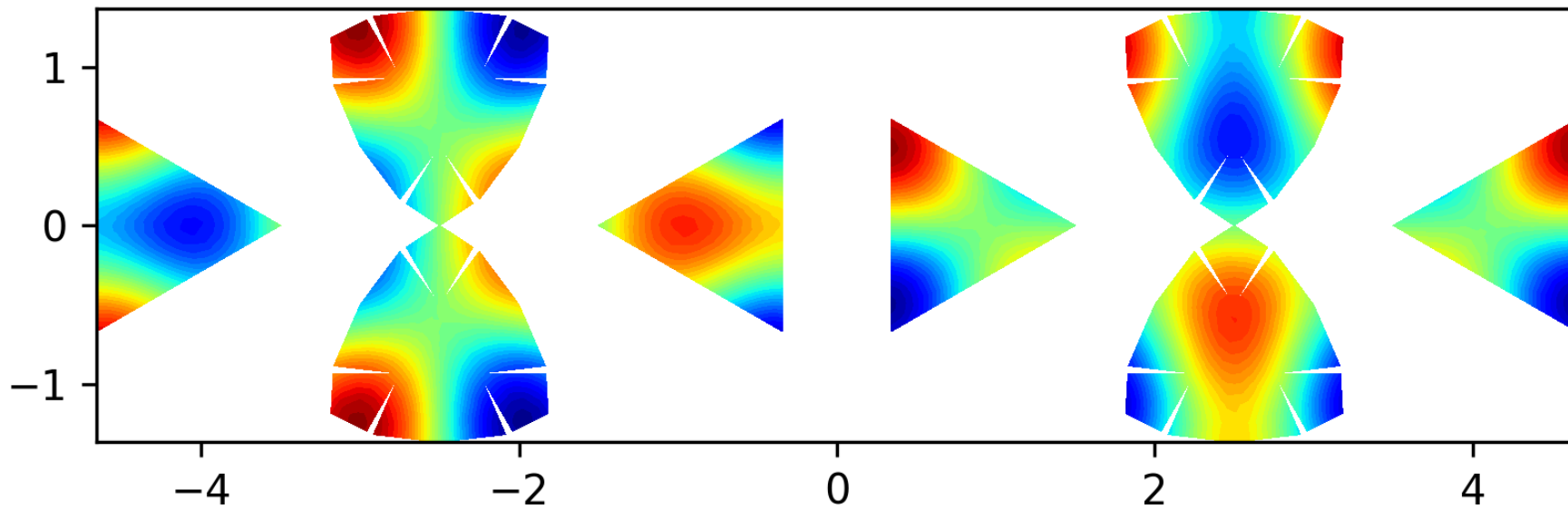
Eigenfunction 10 on the level 2 polyhedron, EV = 18.2079
