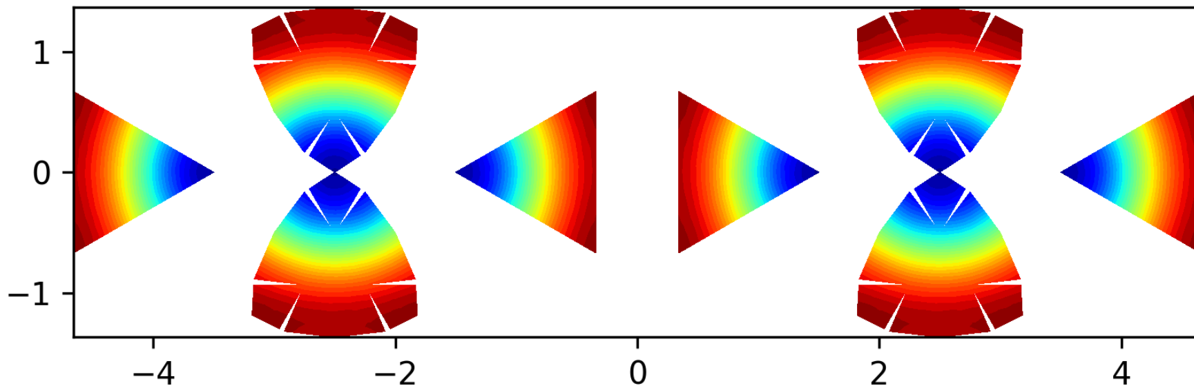
Eigenfunction 5 on the level 2 polyhedron, EV = 8.925
