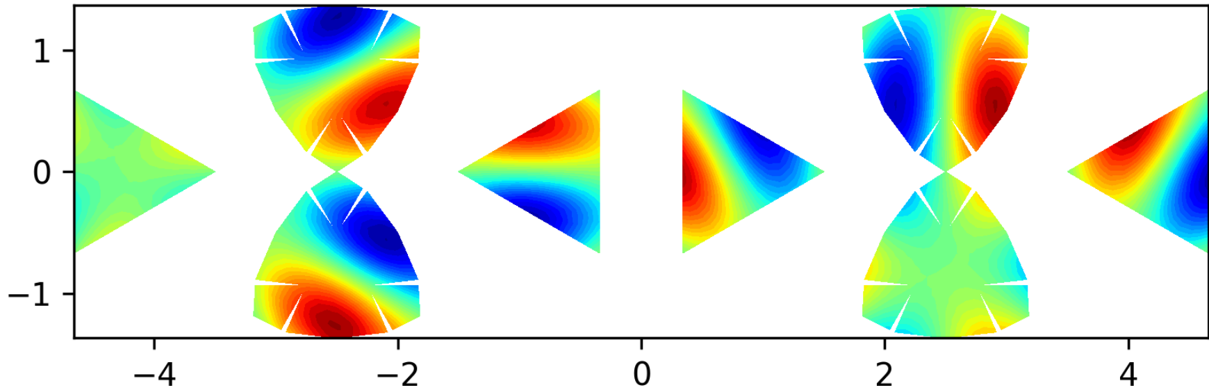
Eigenfunction 12 on the level 2 polyhedron, EV = 18.9518
