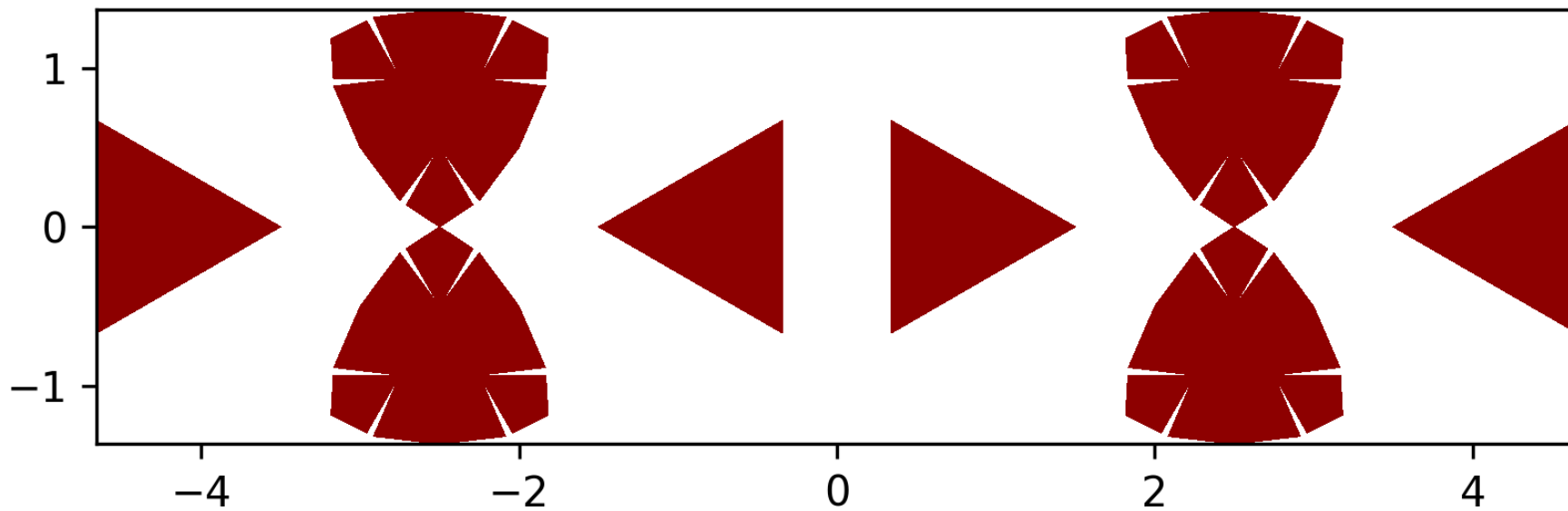
Eigenfunction 0 on the level 2 polyhedron, EV = 0.0
