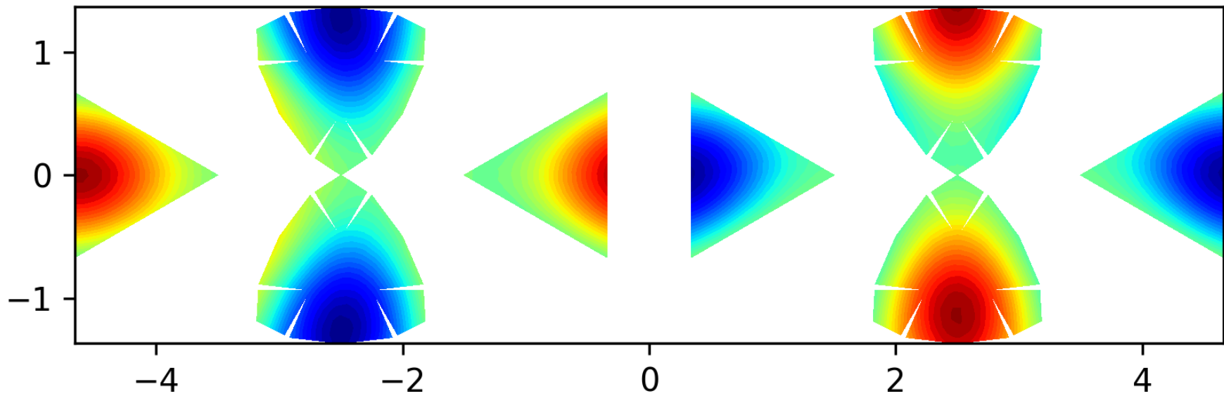
Eigenfunction 8 on the level 2 polyhedron, EV = 9.6111
