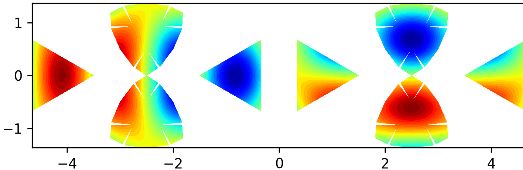
Eigenfunction 6 on the level 2 polyhedron, EV = 9.605
