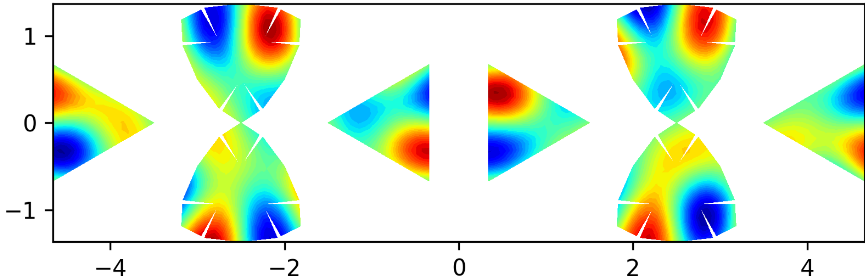
Eigenfunction 19 on the level 2 polyhedron, EV = 30.9494
