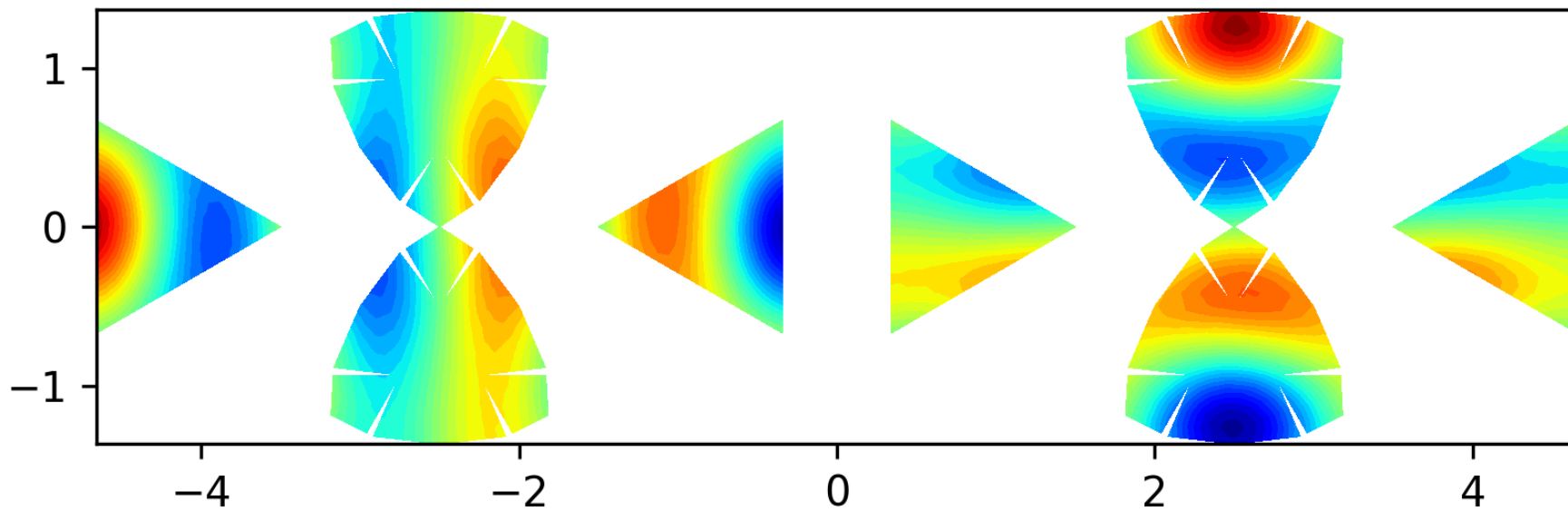
Eigenfunction 13 on the level 2 polyhedron, EV = 18.9548
