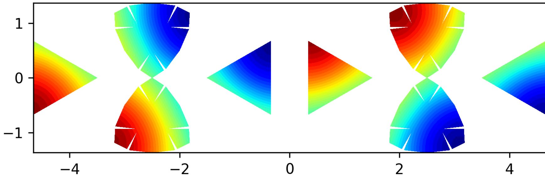
Eigenfunction 2 on the level 2 polyhedron, EV = 3.0981
