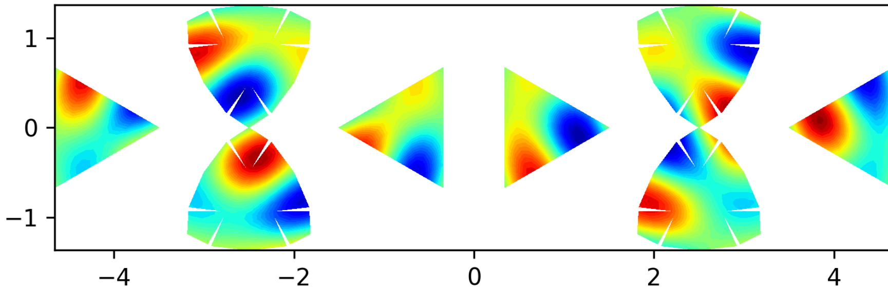
Eigenfunction 18 on the level 2 polyhedron, EV = 30.9388
