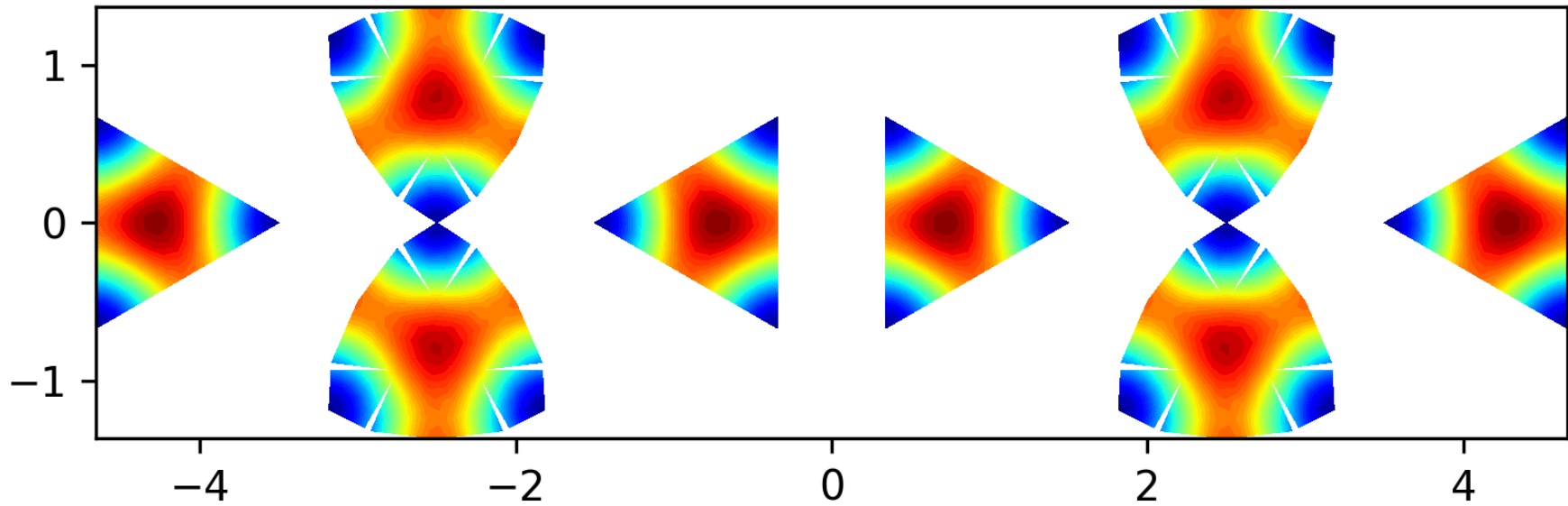
Eigenfunction 16 on the level 2 polyhedron, EV = 29.9466
