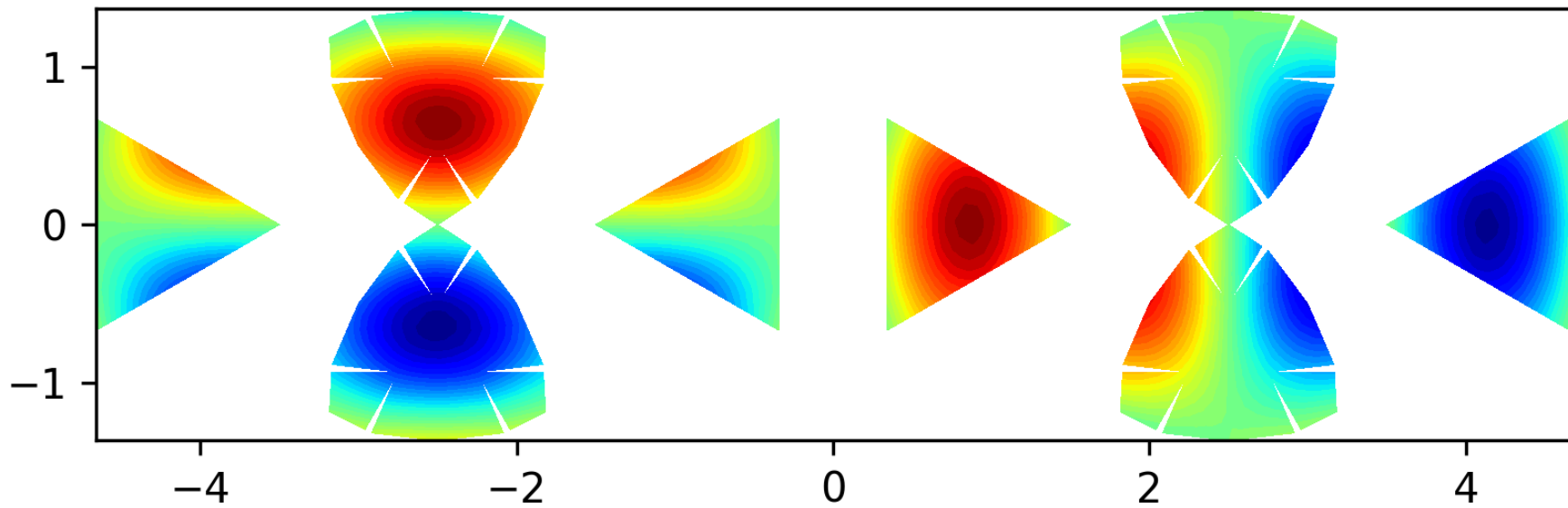
Eigenfunction 7 on the level 2 polyhedron, EV = 9.6055
