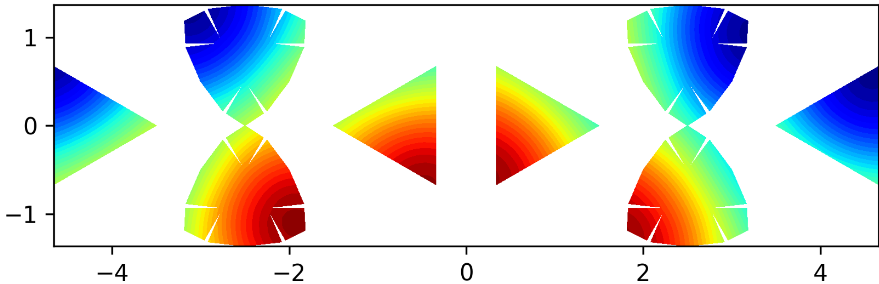
Eigenfunction 1 on the level 2 polyhedron, EV = 3.0981
