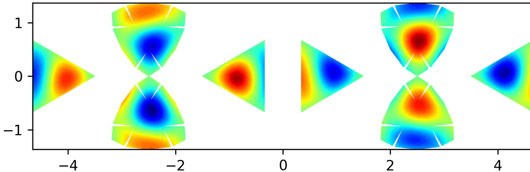
Eigenfunction 22 on the level 2 polyhedron, EV = 32.6037
