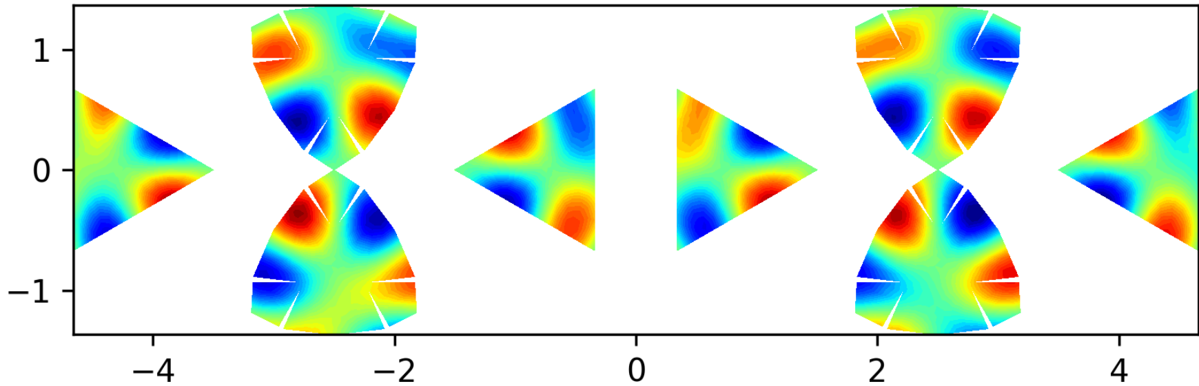
Eigenfunction 30 on the level 2 polyhedron, EV = 46.9678
