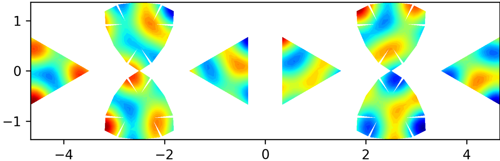
Eigenfunction 25 on the level 2 polyhedron, EV = 45.7702
