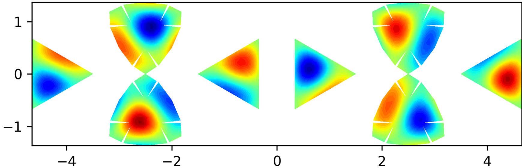
Eigenfunction 23 on the level 2 polyhedron, EV = 32.6364
