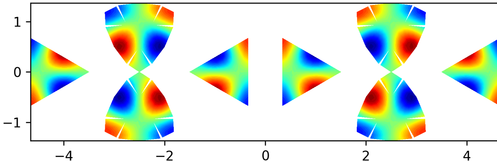
Eigenfunction 21 on the level 2 polyhedron, EV = 31.2361
