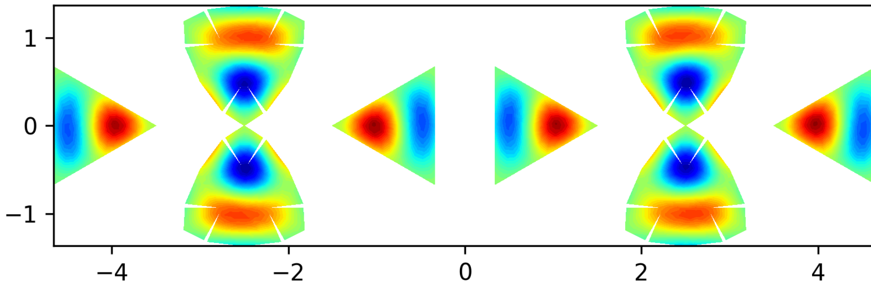
Eigenfunction 32 on the level 2 polyhedron, EV = 48.7193
