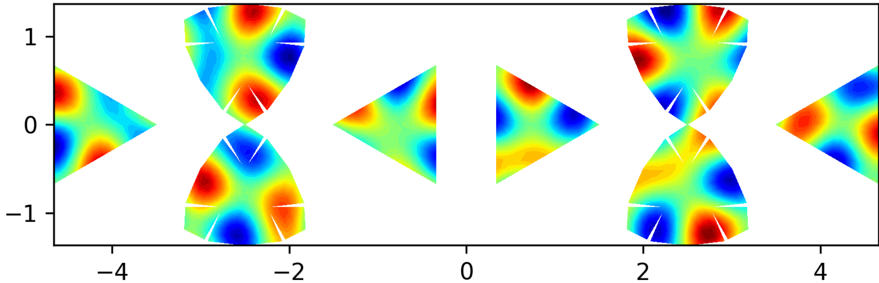
Eigenfunction 28 on the level 2 polyhedron, EV = 46.931
