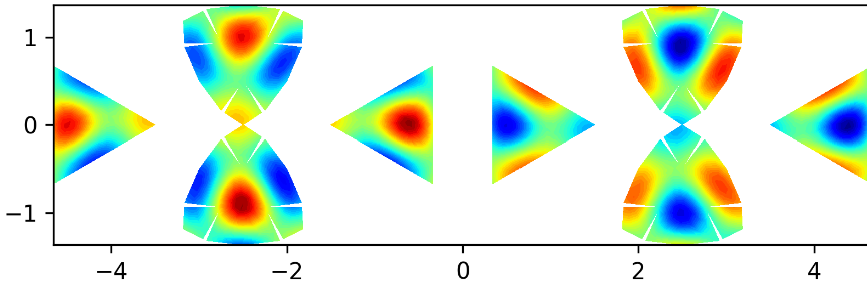
Eigenfunction 33 on the level 2 polyhedron, EV = 49.0925
