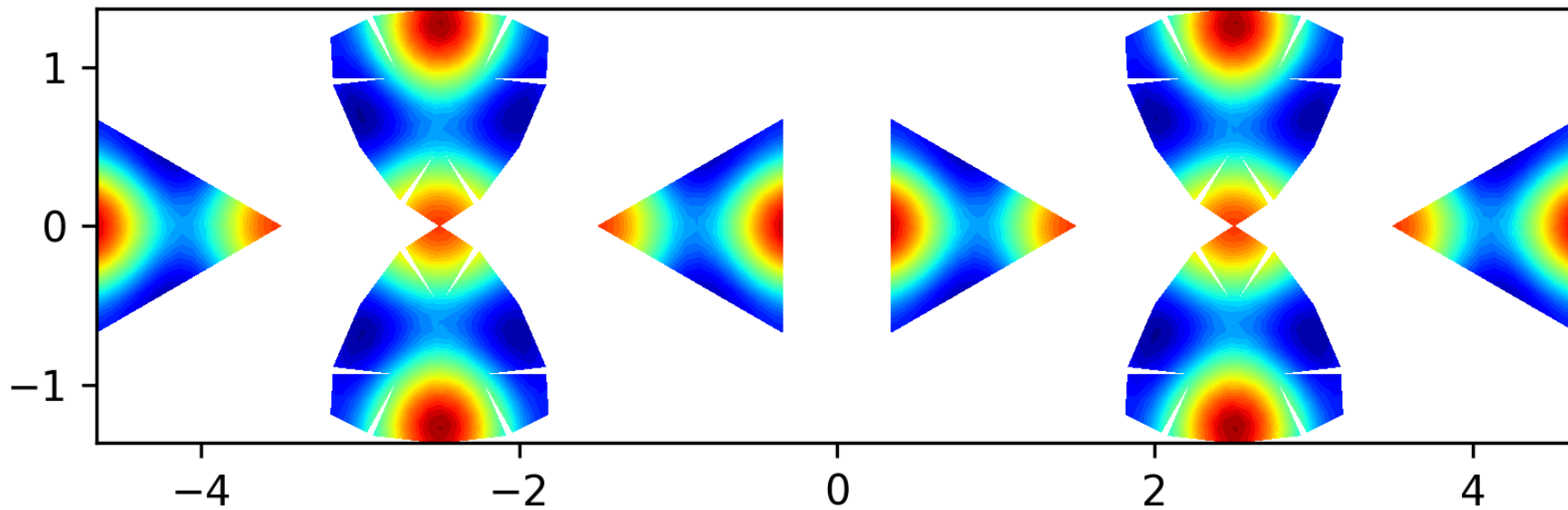
Eigenfunction 20 on the level 2 polyhedron, EV = 31.2229
