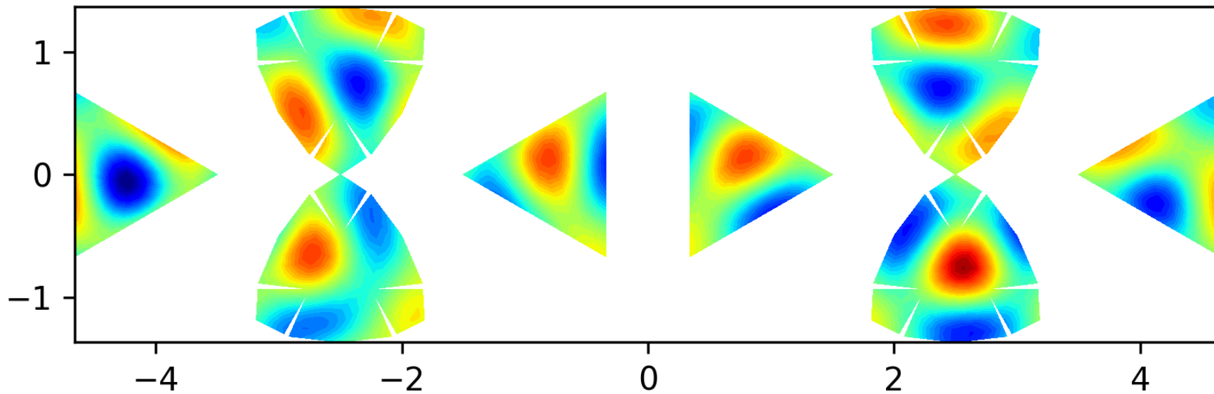
Eigenfunction 35 on the level 2 polyhedron, EV = 49.1335
