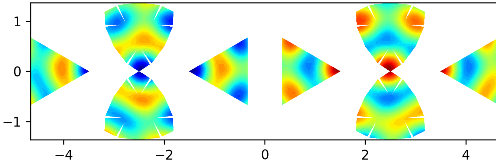
Eigenfunction 27 on the level 2 polyhedron, EV = 45.8008
