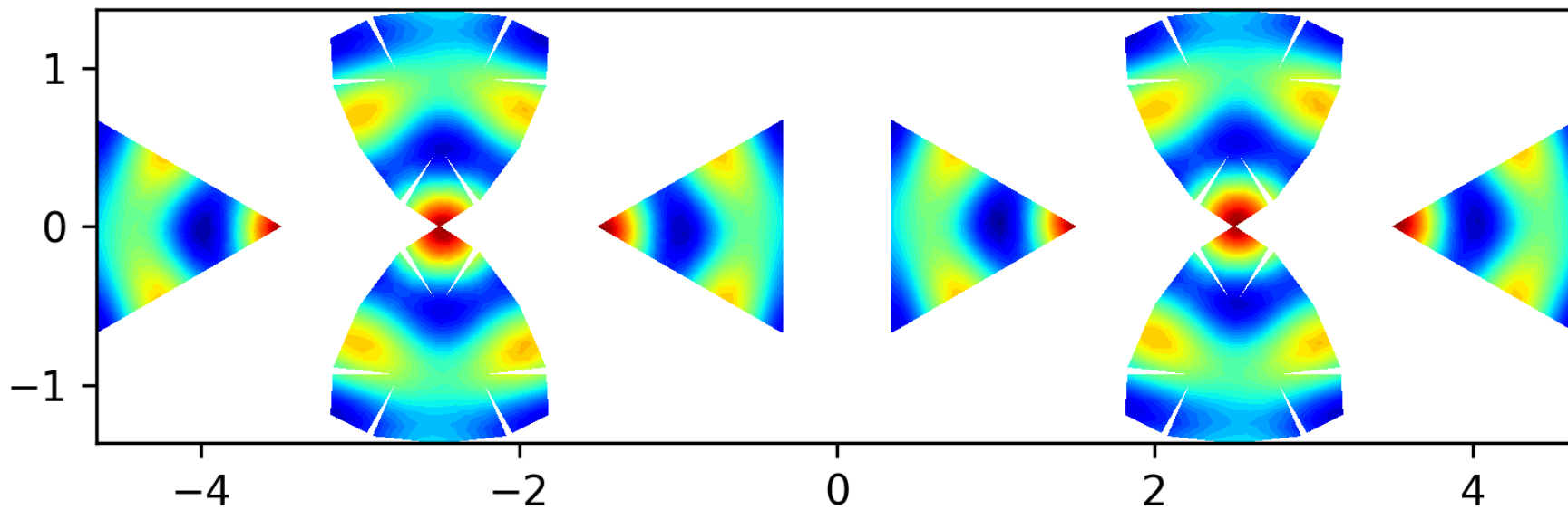
Eigenfunction 37 on the level 2 polyhedron, EV = 64.7738
