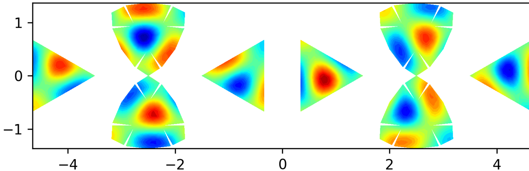
Eigenfunction 34 on the level 2 polyhedron, EV = 49.1303
