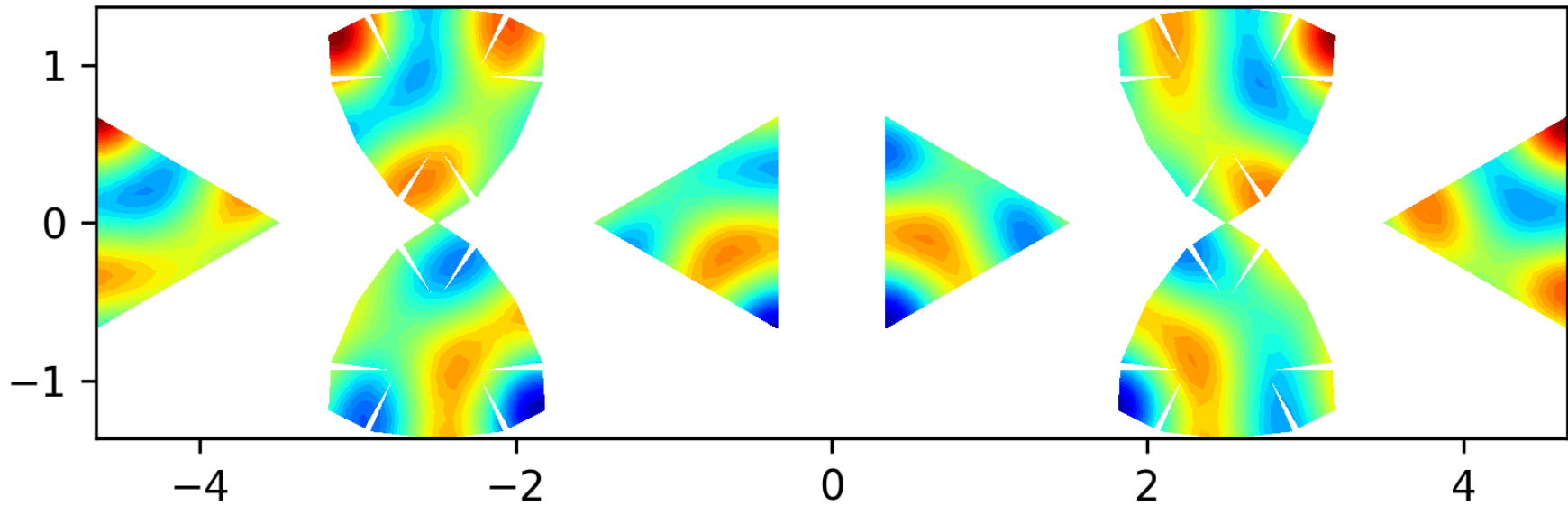
Eigenfunction 26 on the level 2 polyhedron, EV = 45.7753
