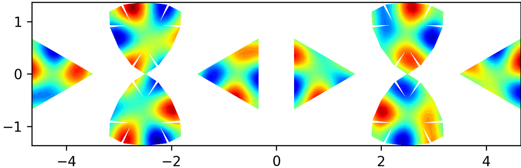
Eigenfunction 29 on the level 2 polyhedron, EV = 46.9344
