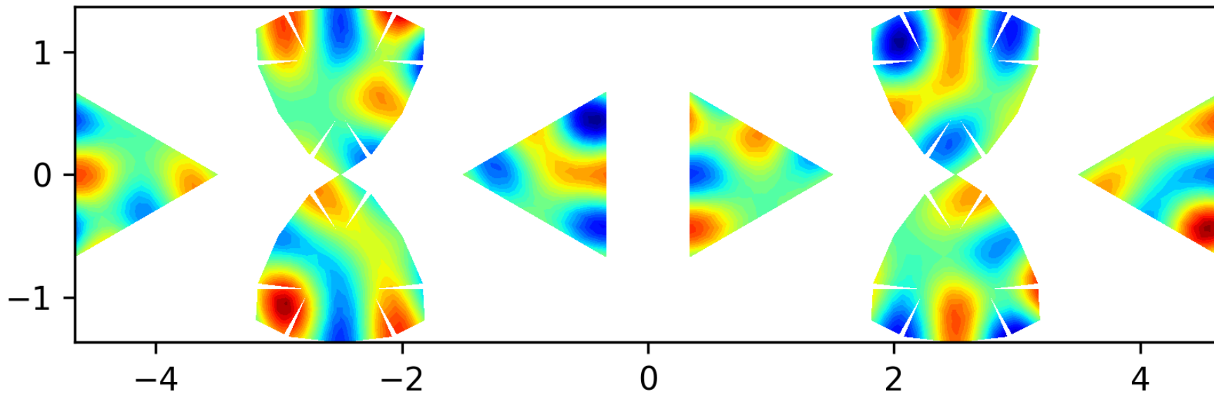
Eigenfunction 38 on the level 2 polyhedron, EV = 64.8737
