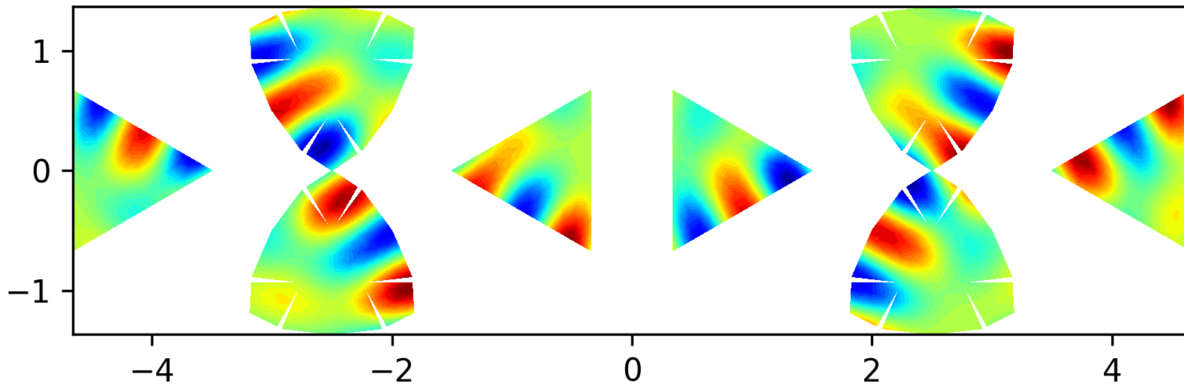
Eigenfunction 39 on the level 2 polyhedron, EV = 64.9292
