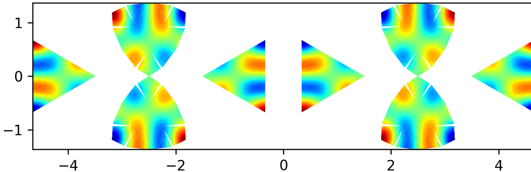
Eigenfunction 36 on the level 2 polyhedron, EV = 64.7025
