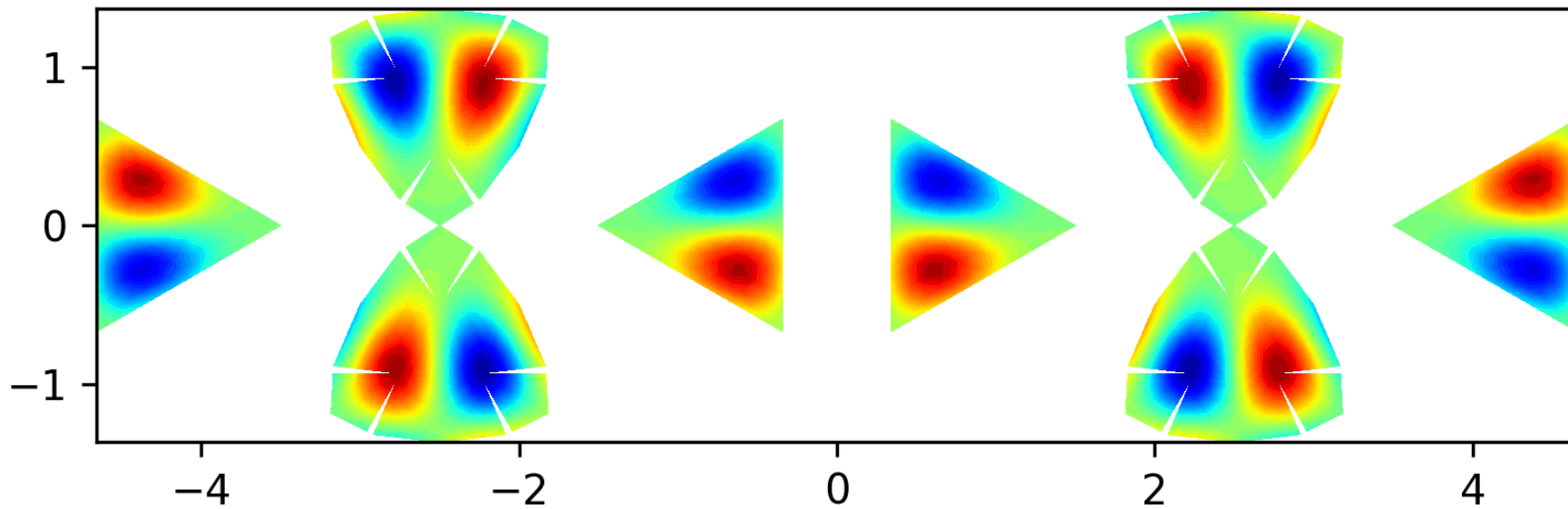
Eigenfunction 31 on the level 2 polyhedron, EV = 48.7177
