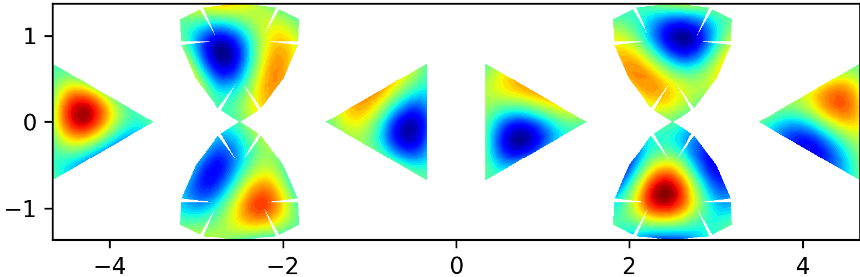
Eigenfunction 24 on the level 2 polyhedron, EV = 32.641
