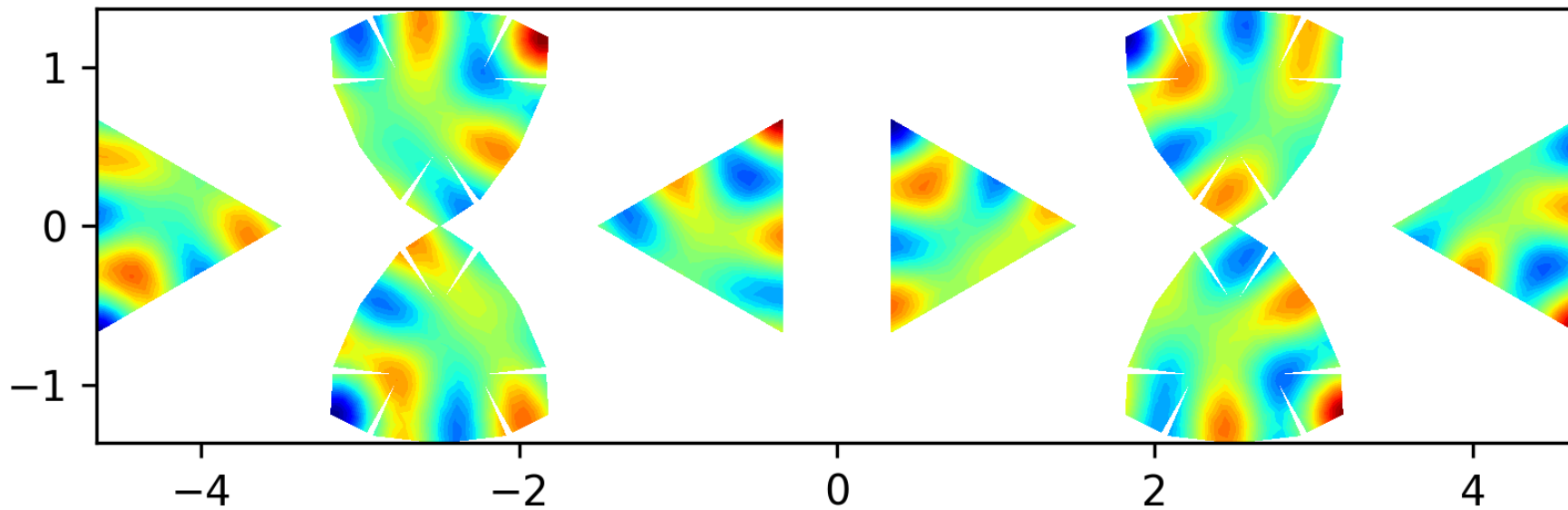
Eigenfunction 50 on the level 2 polyhedron, EV = 86.7712
