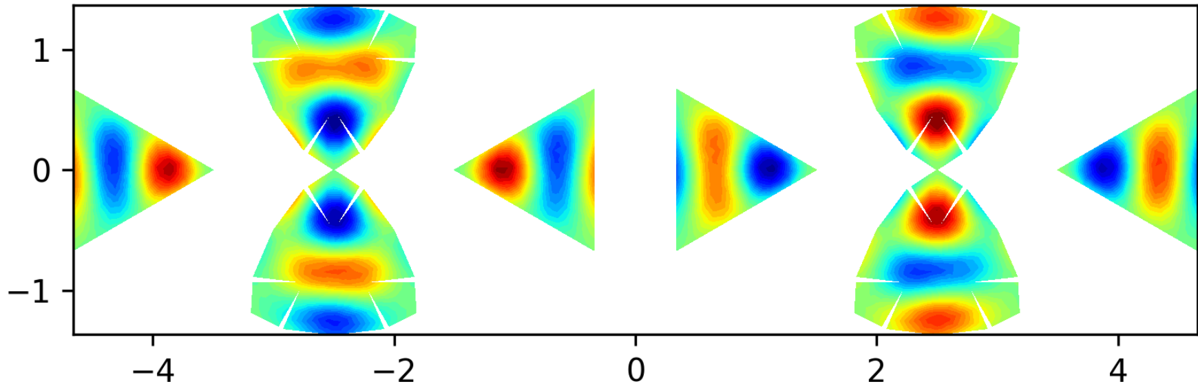
Eigenfunction 44 on the level 2 polyhedron, EV = 68.5638
