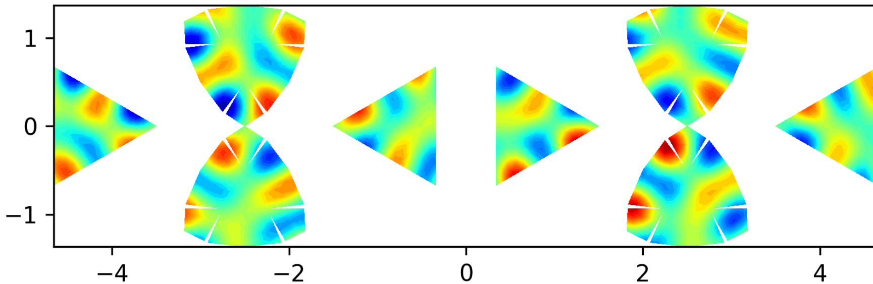
Eigenfunction 54 on the level 2 polyhedron, EV = 87.871
