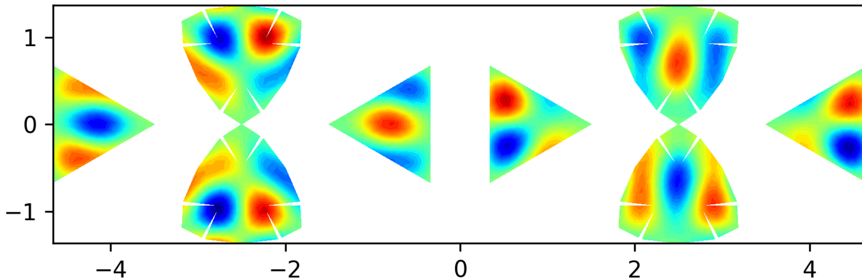
Eigenfunction 43 on the level 2 polyhedron, EV = 68.4946
