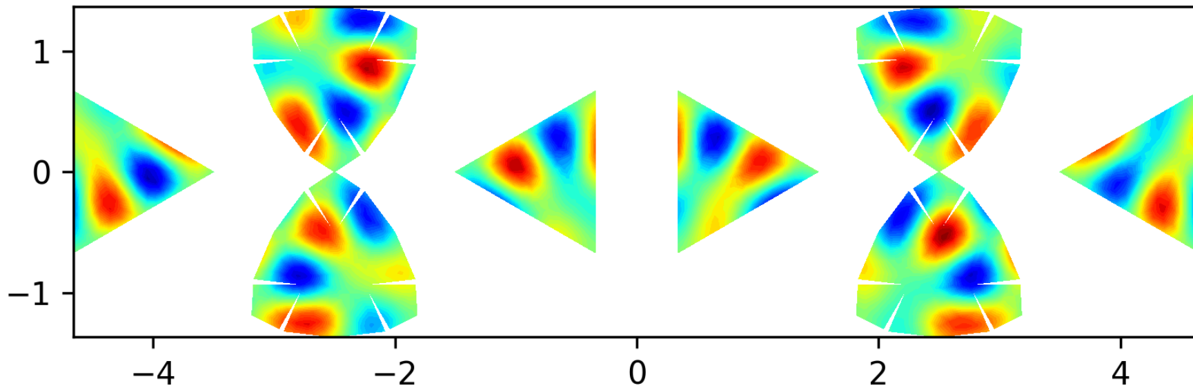
Eigenfunction 57 on the level 2 polyhedron, EV = 92.3012
