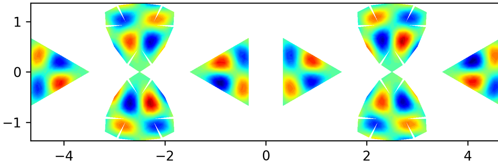
Eigenfunction 59 on the level 2 polyhedron, EV = 92.9028
