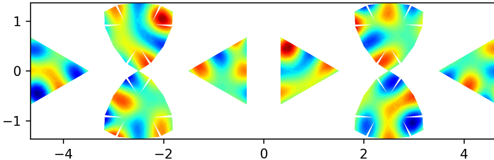
Eigenfunction 40 on the level 2 polyhedron, EV = 64.9482
