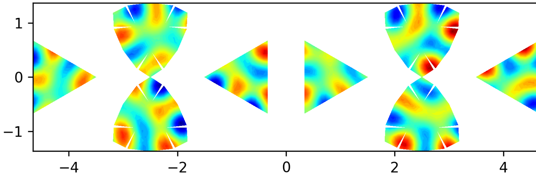
Eigenfunction 52 on the level 2 polyhedron, EV = 87.6103
