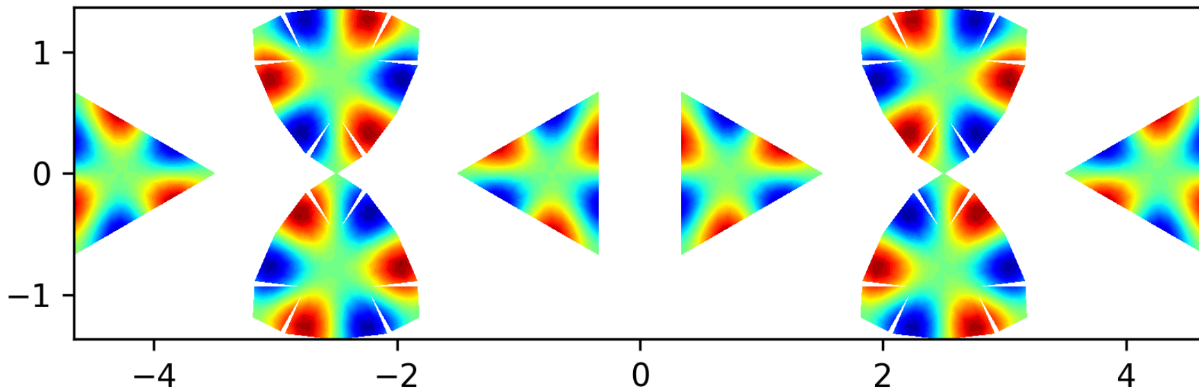
Eigenfunction 41 on the level 2 polyhedron, EV = 66.6785
