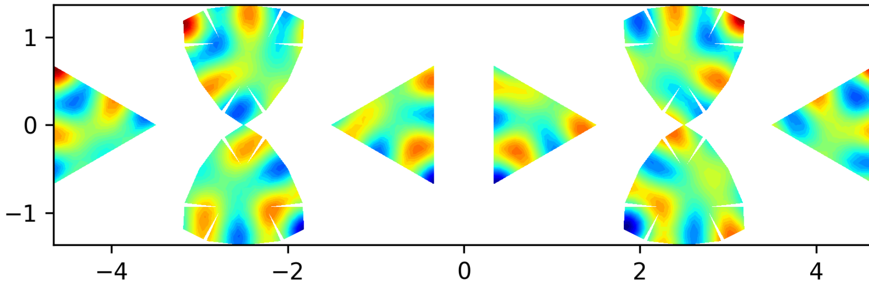
Eigenfunction 49 on the level 2 polyhedron, EV = 86.7519
