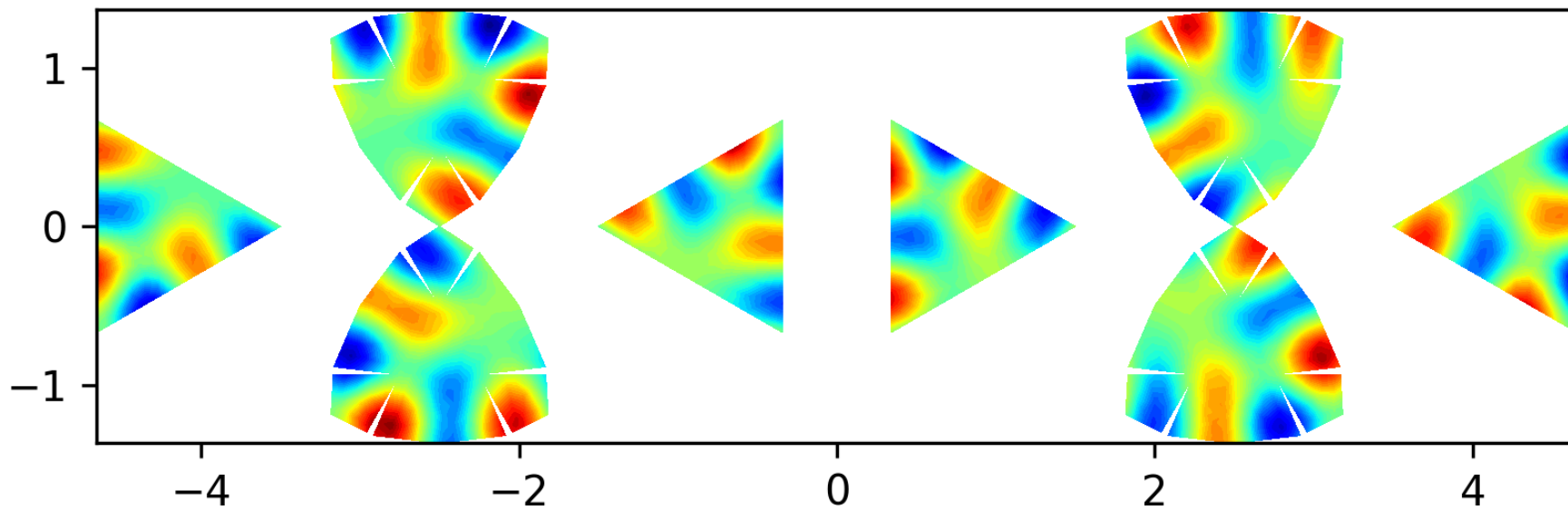
Eigenfunction 53 on the level 2 polyhedron, EV = 87.6643
