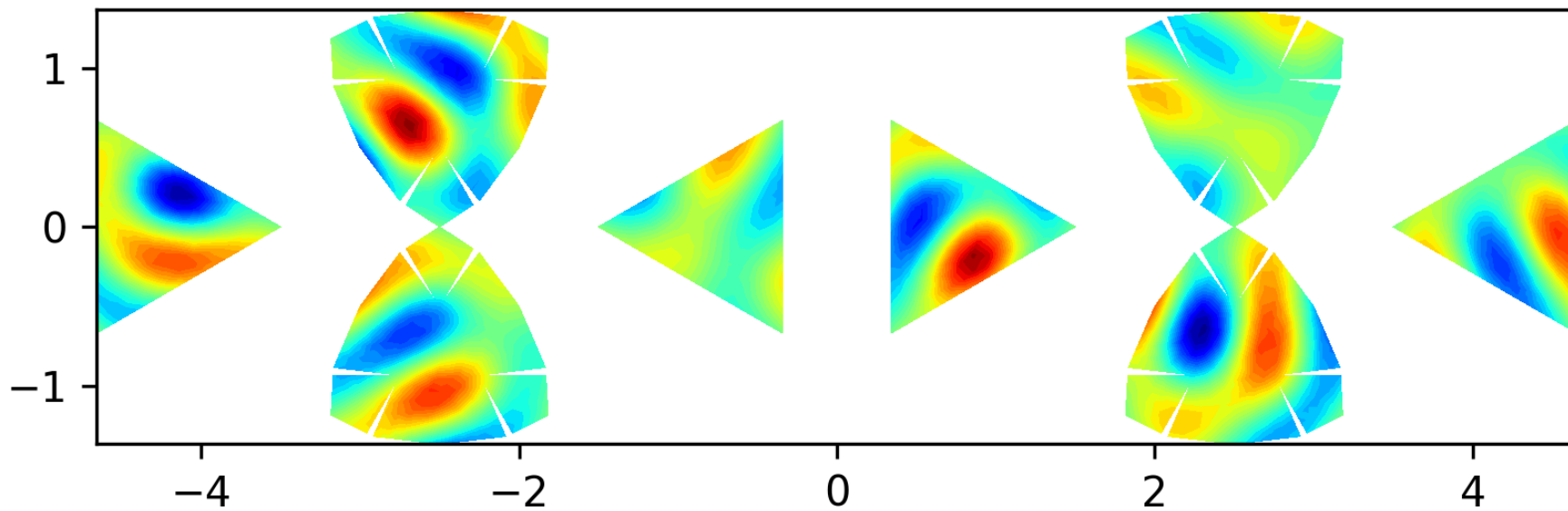
Eigenfunction 47 on the level 2 polyhedron, EV = 69.2121
