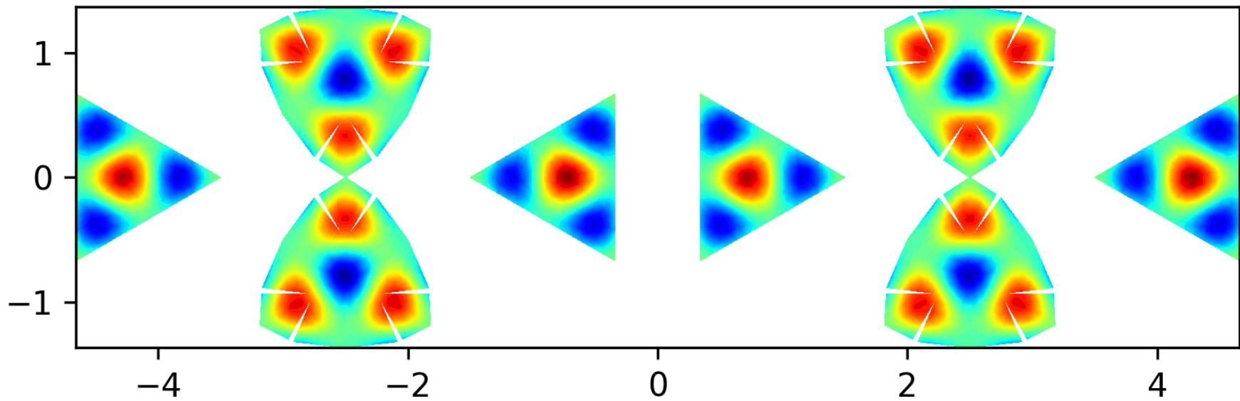
Eigenfunction 55 on the level 2 polyhedron, EV = 91.165
