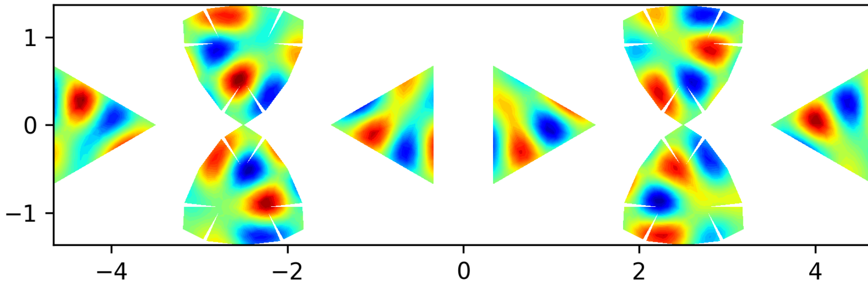
Eigenfunction 58 on the level 2 polyhedron, EV = 92.3087
