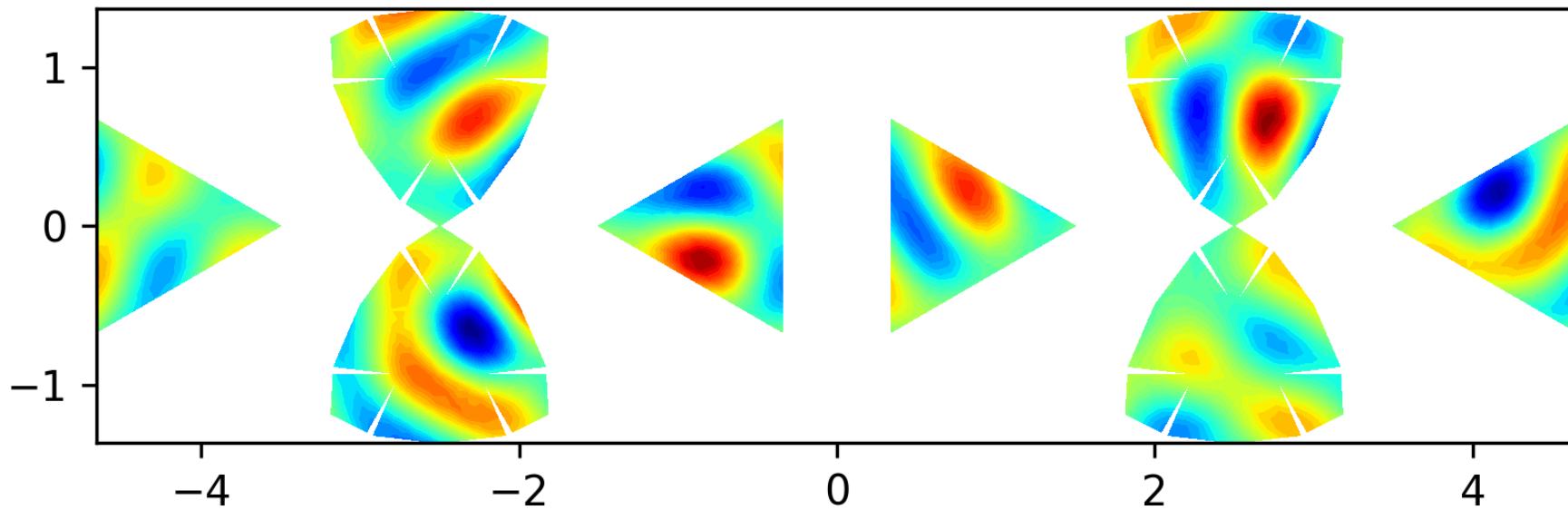
Eigenfunction 45 on the level 2 polyhedron, EV = 69.0875
