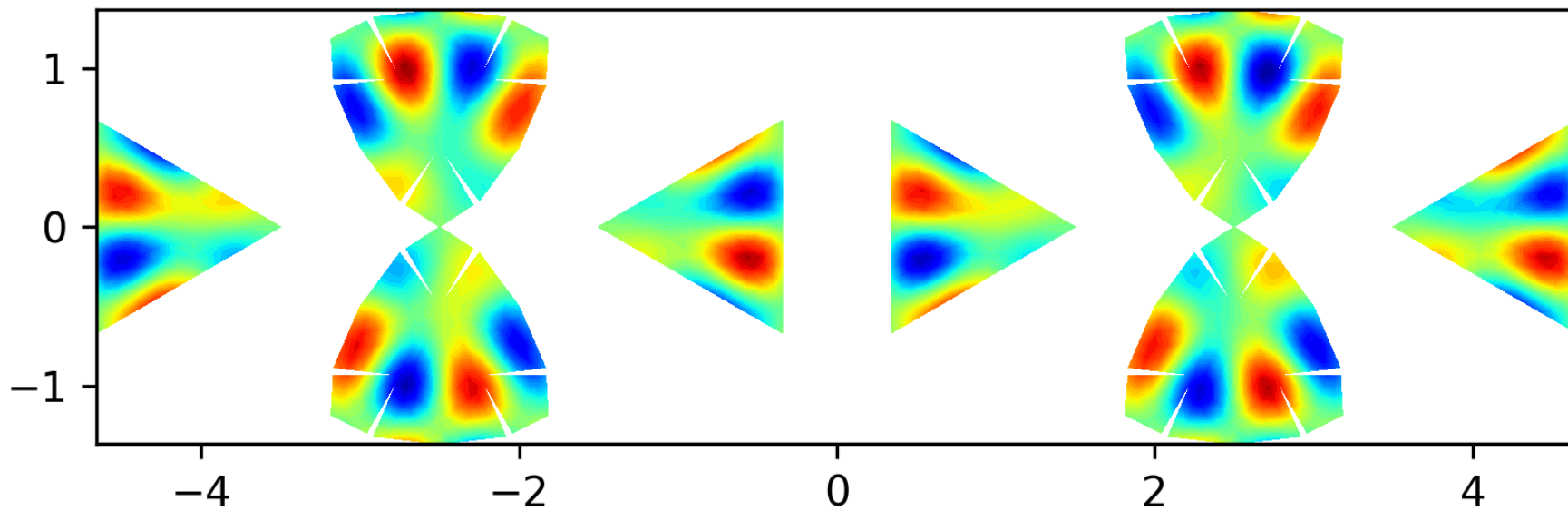
Eigenfunction 56 on the level 2 polyhedron, EV = 91.972
