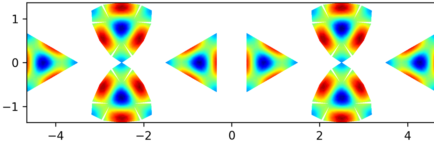
Eigenfunction 48 on the level 2 polyhedron, EV = 69.5676
