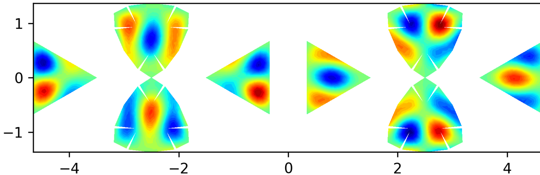
Eigenfunction 42 on the level 2 polyhedron, EV = 68.4914
