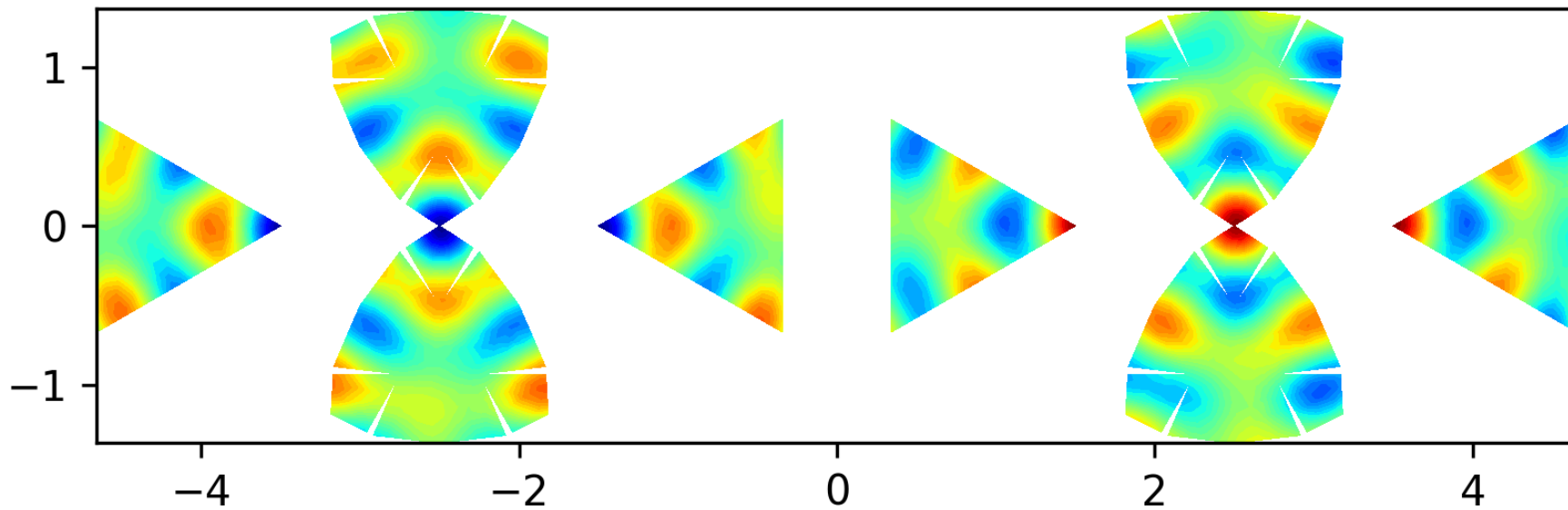
Eigenfunction 51 on the level 2 polyhedron, EV = 87.0479
