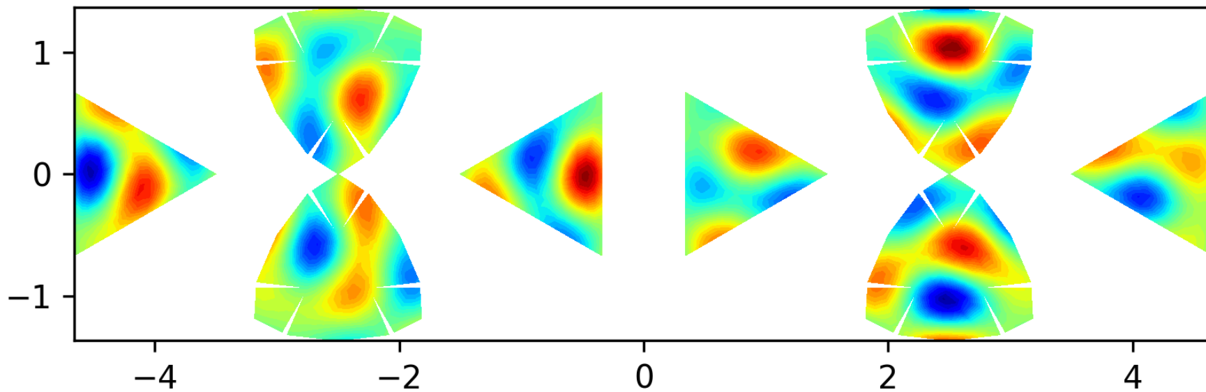
Eigenfunction 46 on the level 2 polyhedron, EV = 69.1653
