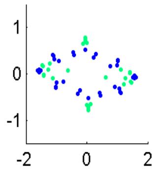
Eigval2235.779
