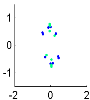
Eigval8097.449
