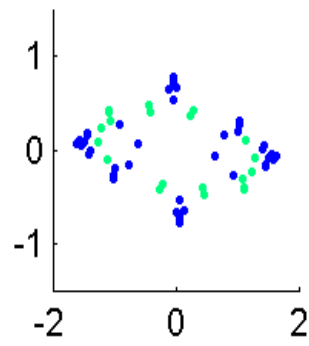
Eigval2223.1736
