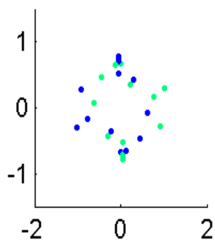
Eigval9091.0596
