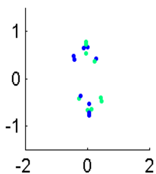
Eigval9091.0512
