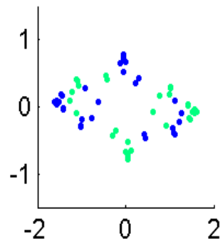
Eigval1760.5646
