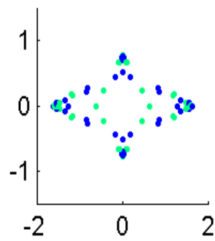
Eigval6594.2549
