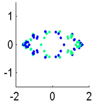
Eigval5557.3573
