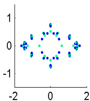
Eigval24616.5127
