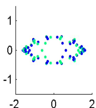
Eigval16938.5596
