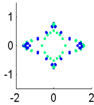
Eigval5515.3198
