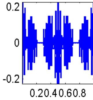
Num112
