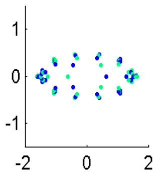
Eigval24616.9923
