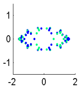
Eigval16625.7202
