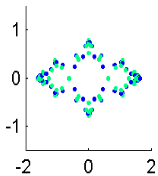
Eigval18867.721
