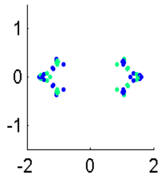
Eigval6594.8703
