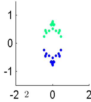
Eigval195.808
