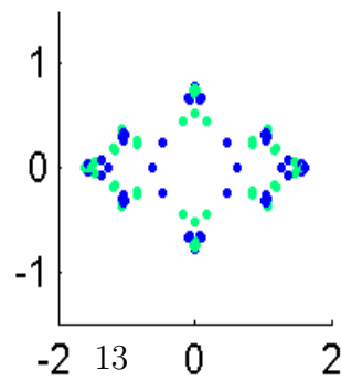
Eigval6594.8703
