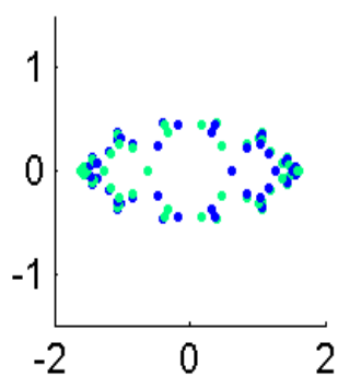
Eigval17377.8563
