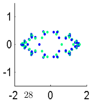
Eigval32826.3716
