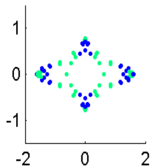
Eigval2294.1548
