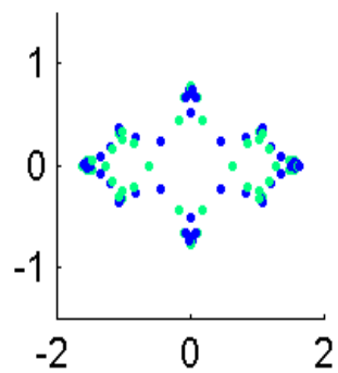
Eigval16870.6618
