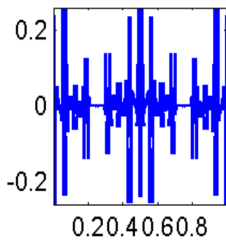
Num120
