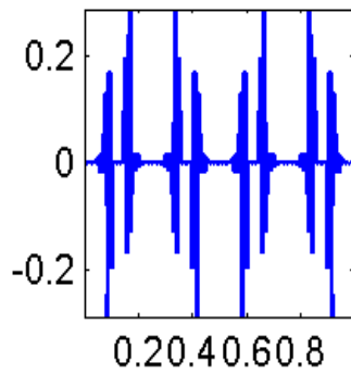
Num88
