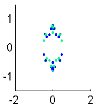
Eigval34240.3306
