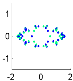
Eigval34331.2981
