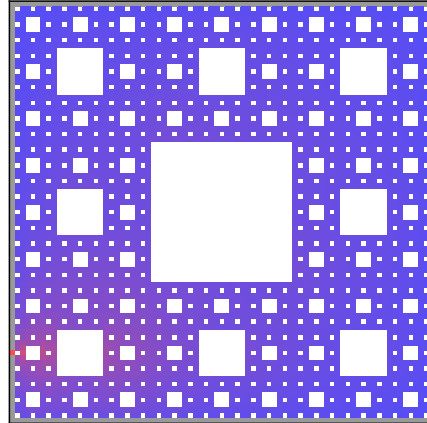
Torus Harmonic Function 13 on M = 4
