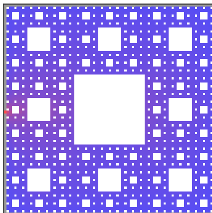
Torus Harmonic Function 39 on M = 4
