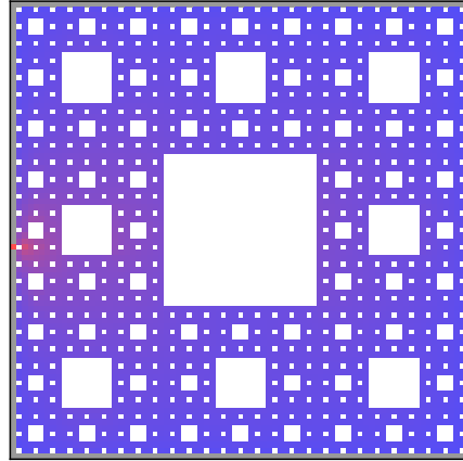
Torus Harmonic Function 37 on M = 4
