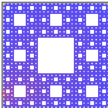
Torus Harmonic Function 11 on M = 4
