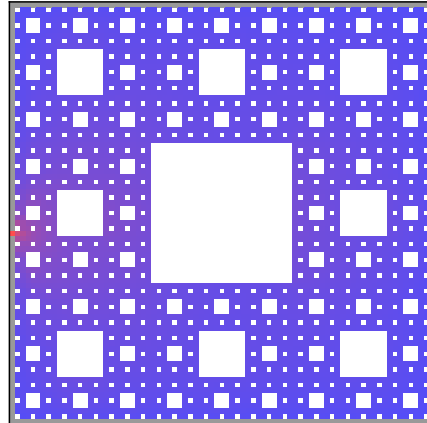
Torus Harmonic Function 36 on M = 4
