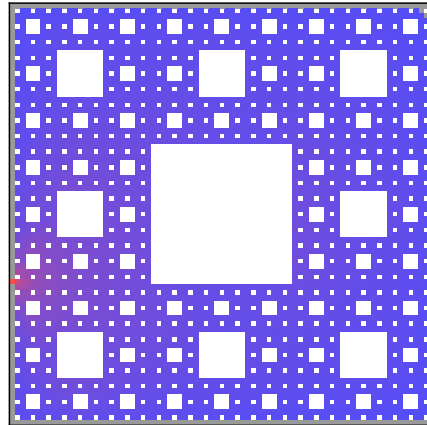
Torus Harmonic Function 27 on M = 4
