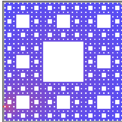
Torus Harmonic Function 10 on M = 4
