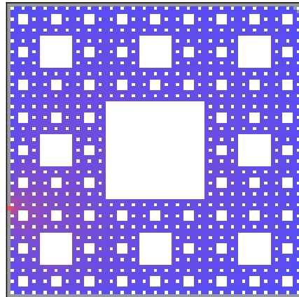
Torus Harmonic Function 24 on M = 4
