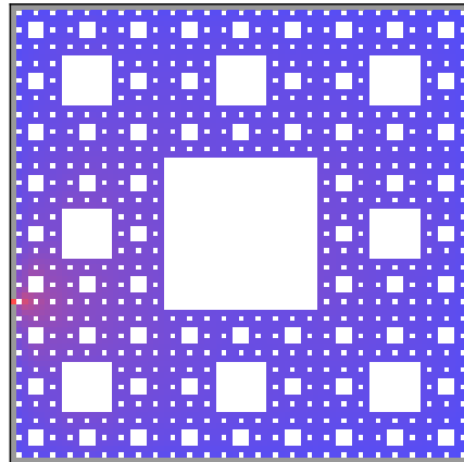
Torus Harmonic Function 28 on M = 4
