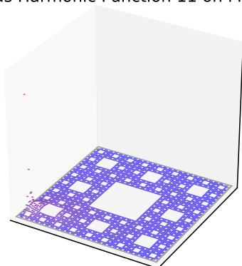
Torus Harmonic Function 11 on M = 4
