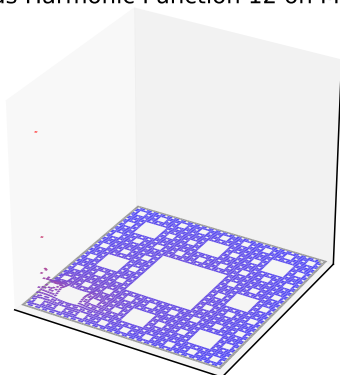
Torus Harmonic Function 12 on M = 4
