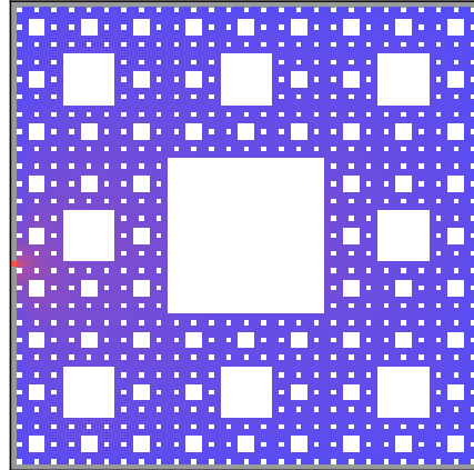
Torus Harmonic Function 35 on M = 4
