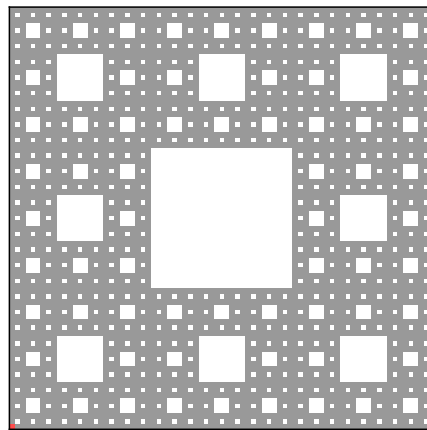
Torus Harmonic Function 0 on M = 4
