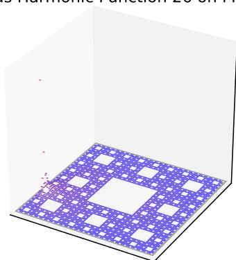
Torus Harmonic Function 26 on M = 4
