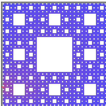
Torus Harmonic Function 15 on M = 4
