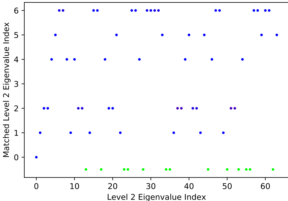
Torus Glued Comparison of Level 2 and 1 Eigenvalue Indices (Dot 0=Blue, 1=Red, 2=Green, 3=Cyan)
