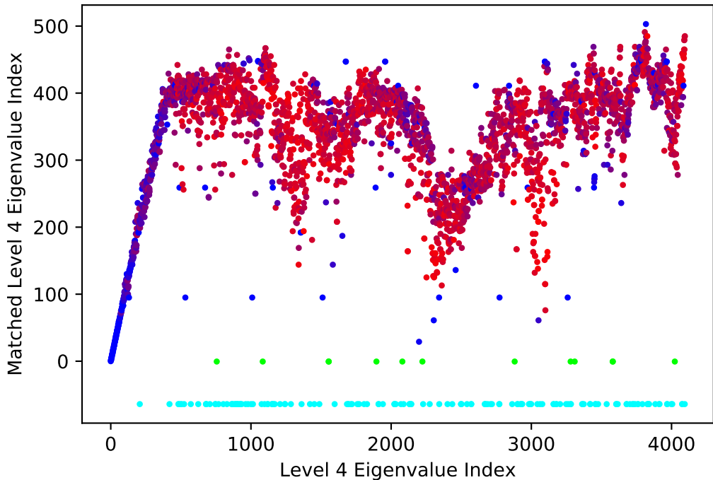
Torus Glued Comparison of Level 4 and 3 Eigenvalue Indices (Dot 0=Blue, 1=Red, 2=Green, 3=Cyan)
