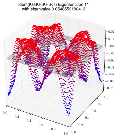
Eigenfunction 11 with eigenvalue 0.0548552180413
