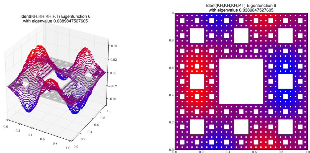
Eigenfunction 6 with eigenvalue 0.0389847527605
