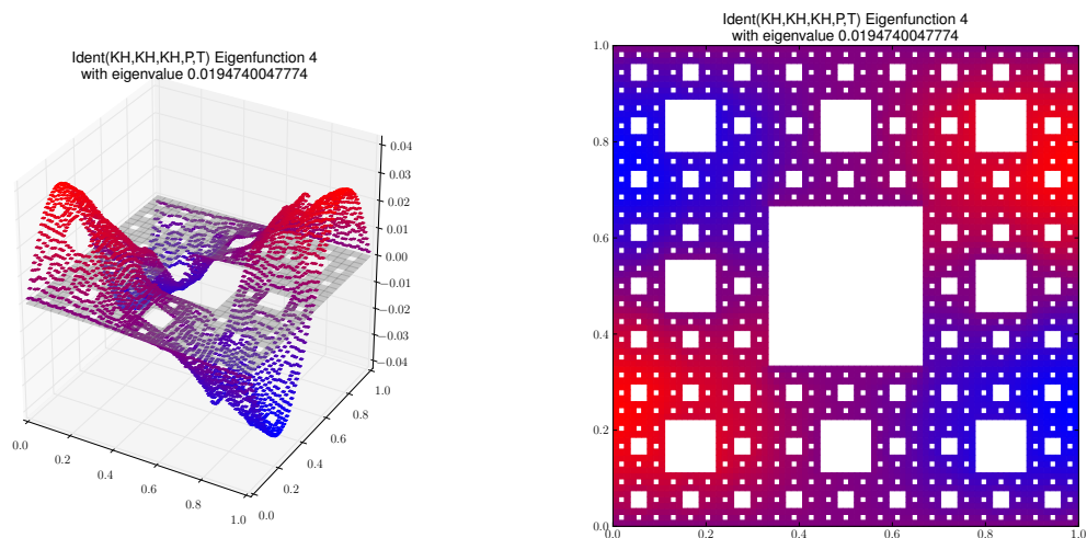
Eigenfunction 4 with eigenvalue 0.0194740047774
