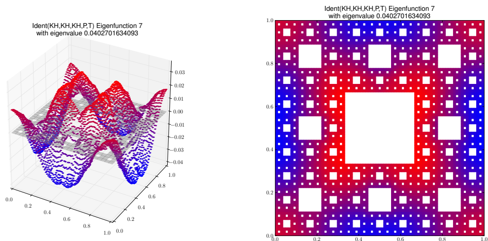
Eigenfunction 7 with eigenvalue 0.0402701634093
