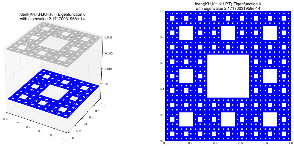
Eigenfunction 0 with eigenvalue 2.17170031958e-14
