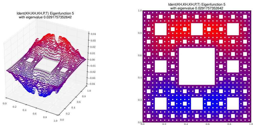
Eigenfunction 5 with eigenvalue 0.0291757352642
