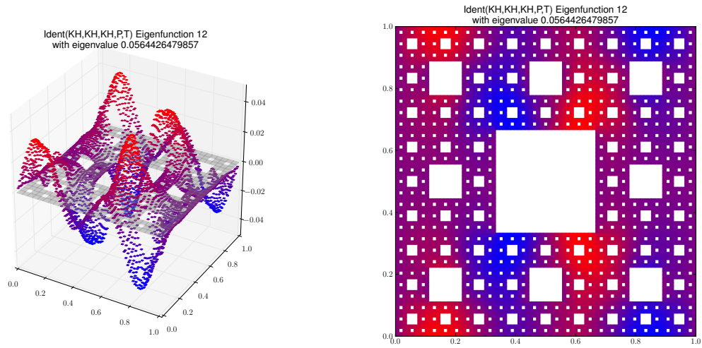
Eigenfunction 12 with eigenvalue 0.0564426479857
