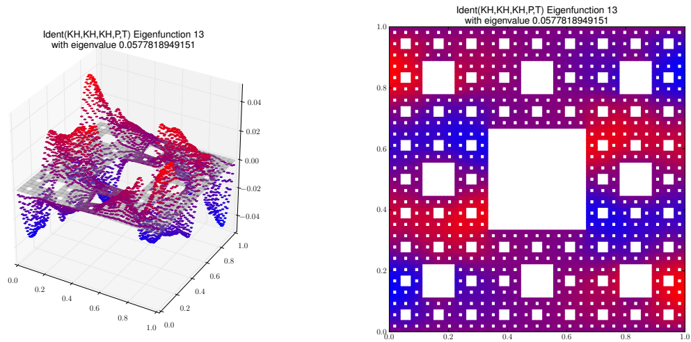
Eigenfunction 13 with eigenvalue 0.0577818949151
