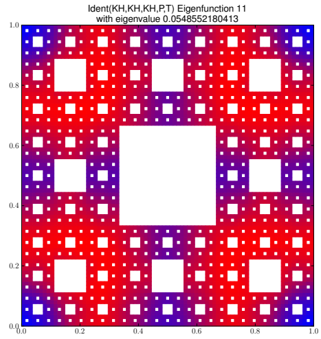
Eigenfunction 11 with eigenvalue 0.0548552180413
