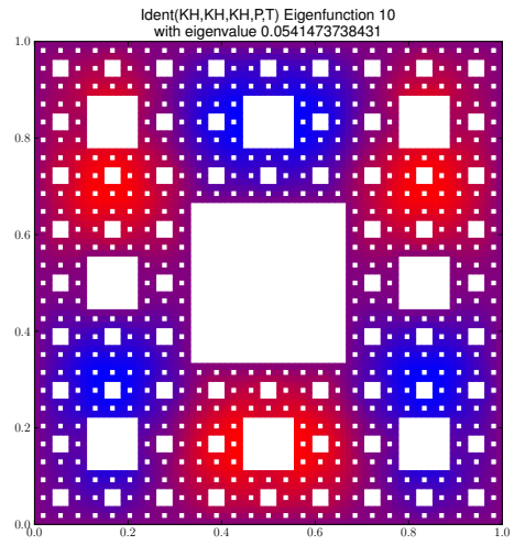
Eigenfunction 10 with eigenvalue 0.0541473738431
