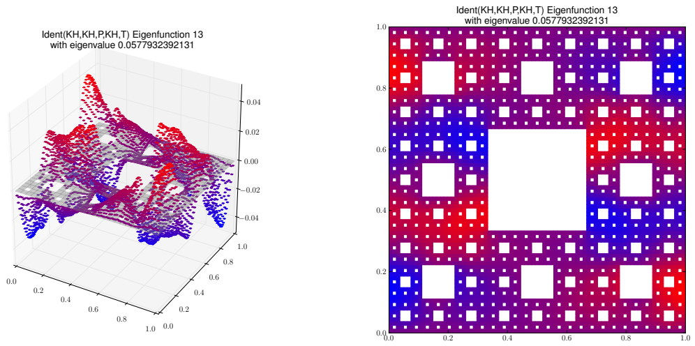
Eigenfunction 13 with eigenvalue 0.0577932392131
