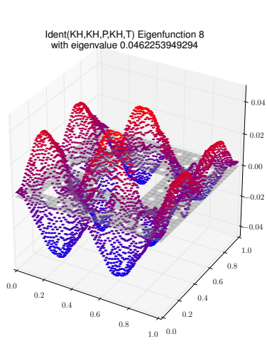
Eigenfunction 8 with eigenvalue 0.0462253949294
