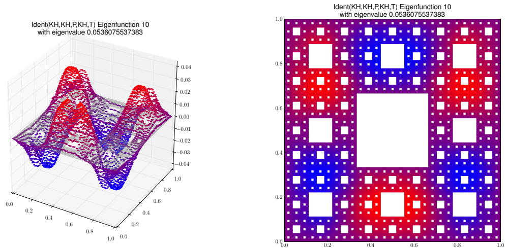
Eigenfunction 10 with eigenvalue 0.0536075537383
