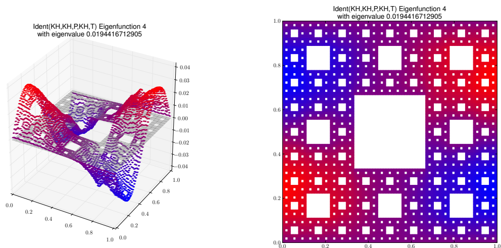
Eigenfunction 4 with eigenvalue 0.0194416712905
