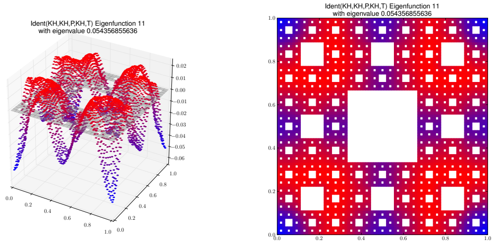
Eigenfunction 11 with eigenvalue 0.054356855636
