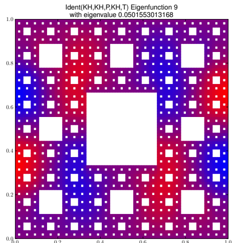
Eigenfunction 9 with eigenvalue 0.0501553013168
