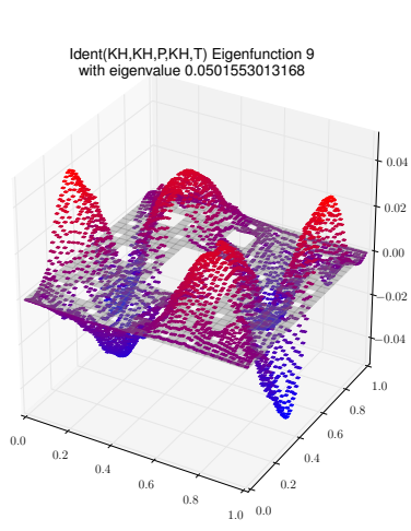
Eigenfunction 9 with eigenvalue 0.0501553013168
