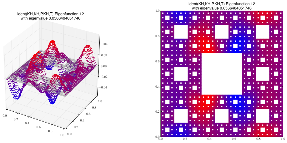
Eigenfunction 12 with eigenvalue 0.0566404051746
