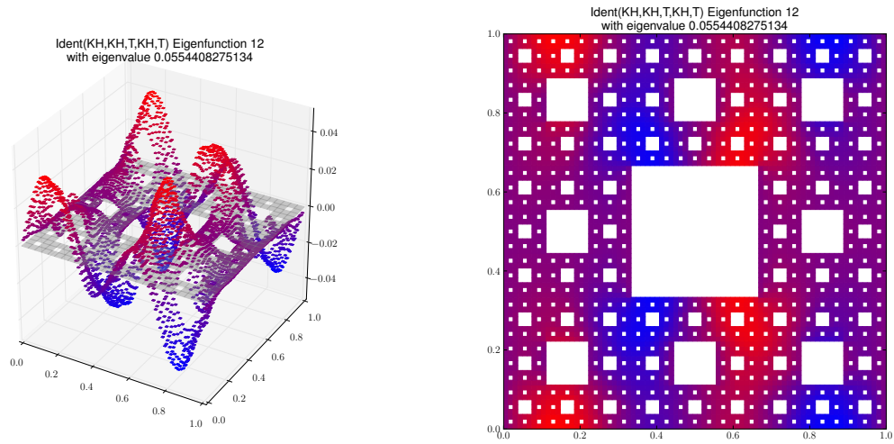
Eigenfunction 12 with eigenvalue 0.0554408275134
