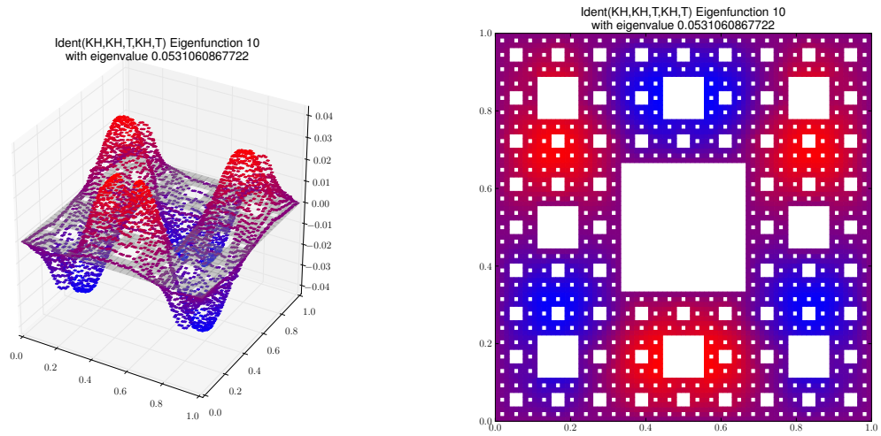
Eigenfunction 10 with eigenvalue 0.0531060867722
