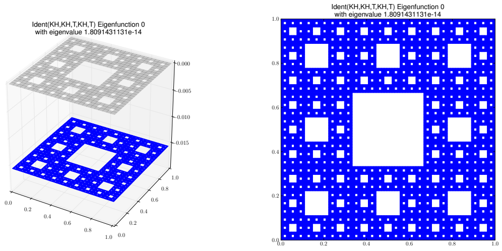
Eigenfunction 0 with eigenvalue 1.8091431131e-14
