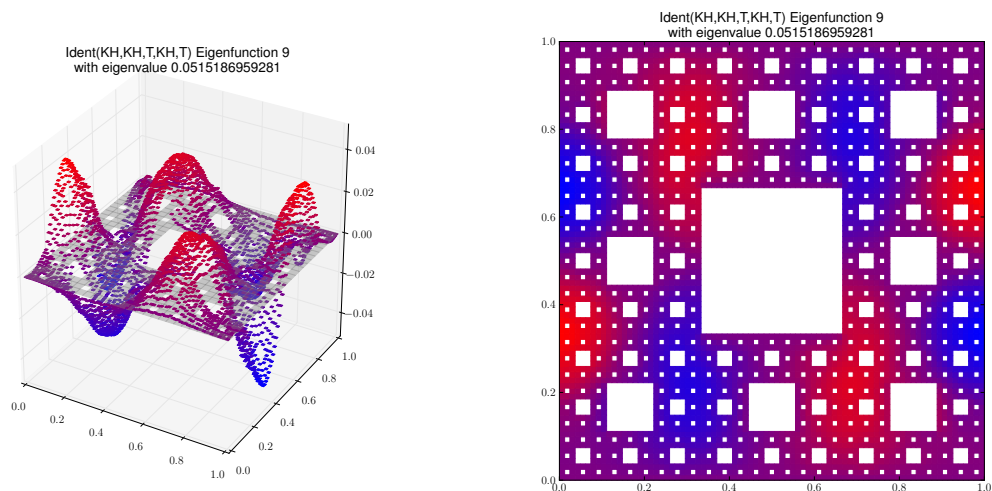
Eigenfunction 9 with eigenvalue 0.0515186959281
