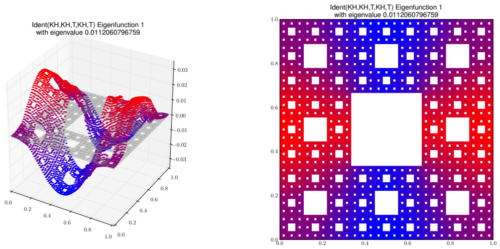
Eigenfunction 1 with eigenvalue 0.0112060796759
