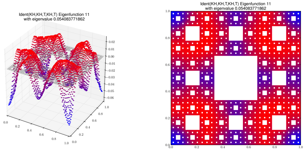
Eigenfunction 11 with eigenvalue 0.054083771862
