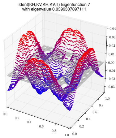
Eigenfunction 7 with eigenvalue 0.0399307897111
