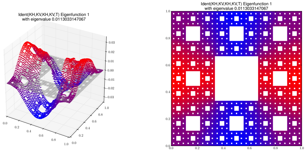
Eigenfunction 1 with eigenvalue 0.0113033147067
