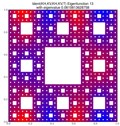
Eigenfunction 13 with eigenvalue 0.0610813628758
