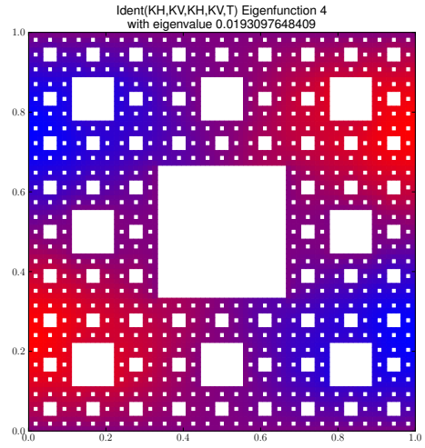
Eigenfunction 4 with eigenvalue 0.0193097648409
