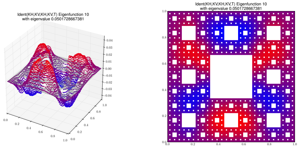
Eigenfunction 10 with eigenvalue 0.0501728667381
