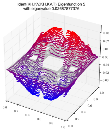
Eigenfunction 5 with eigenvalue 0.02687877376
