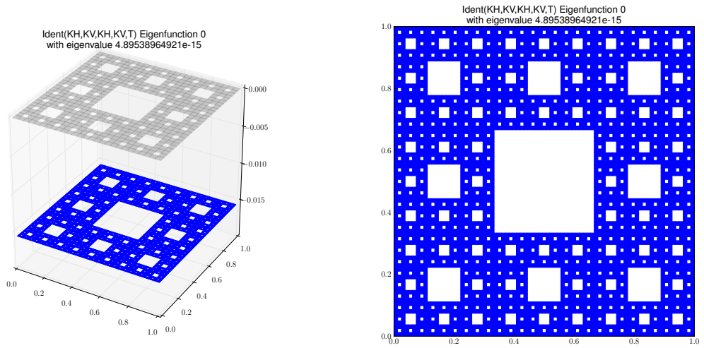
Eigenfunction 0 with eigenvalue 4.89538964921e-15
