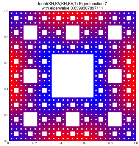
Eigenfunction 7 with eigenvalue 0.0399307897111
