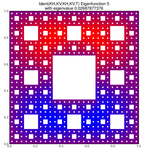
Eigenfunction 5 with eigenvalue 0.02687877376
