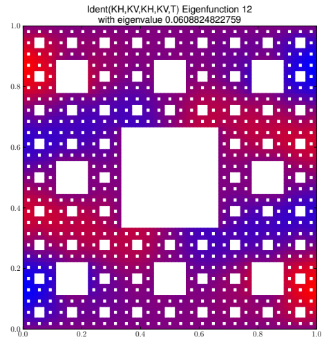
Eigenfunction 12 with eigenvalue 0.0608824822759
