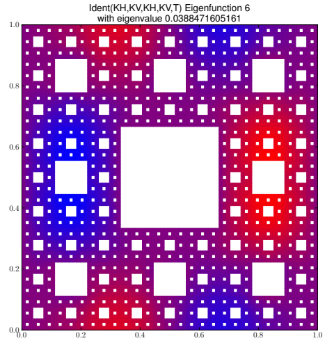
Eigenfunction 6 with eigenvalue 0.0388471605161
