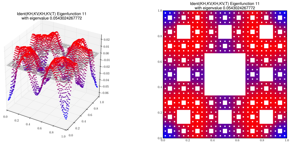
Eigenfunction 11 with eigenvalue 0.0543024267772
