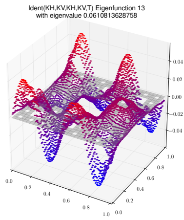
Eigenfunction 13 with eigenvalue 0.0610813628758
