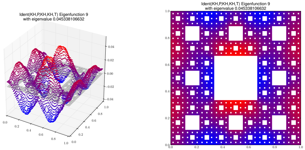
Eigenfunction 9 with eigenvalue 0.045338106632
