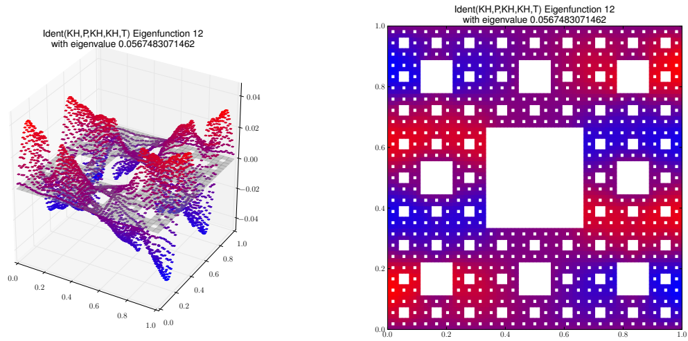
Eigenfunction 12 with eigenvalue 0.0567483071462
