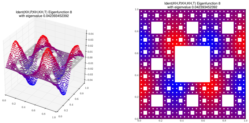
Eigenfunction 8 with eigenvalue 0.042393452392
