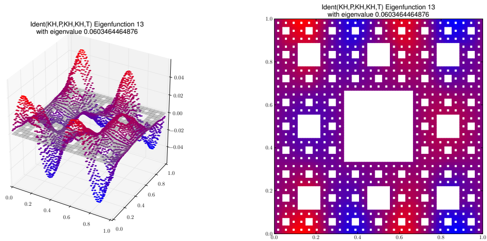
Eigenfunction 13 with eigenvalue 0.0603464464876
