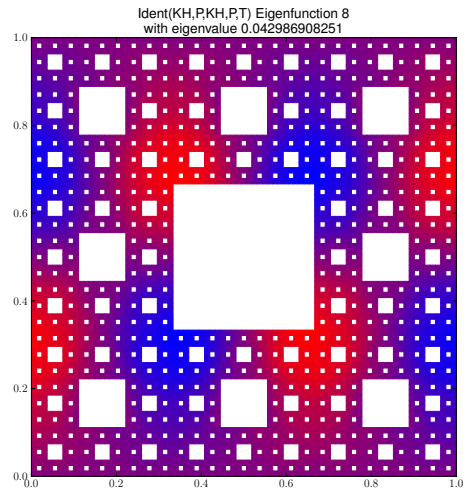
Eigenfunction 8 with eigenvalue 0.042986908251
