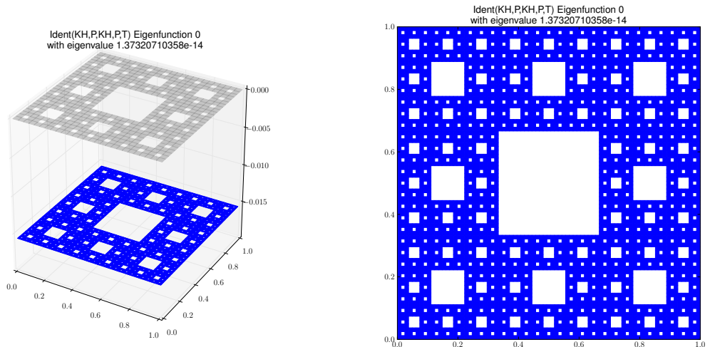
Eigenfunction 0 with eigenvalue 1.37320710358e-14
