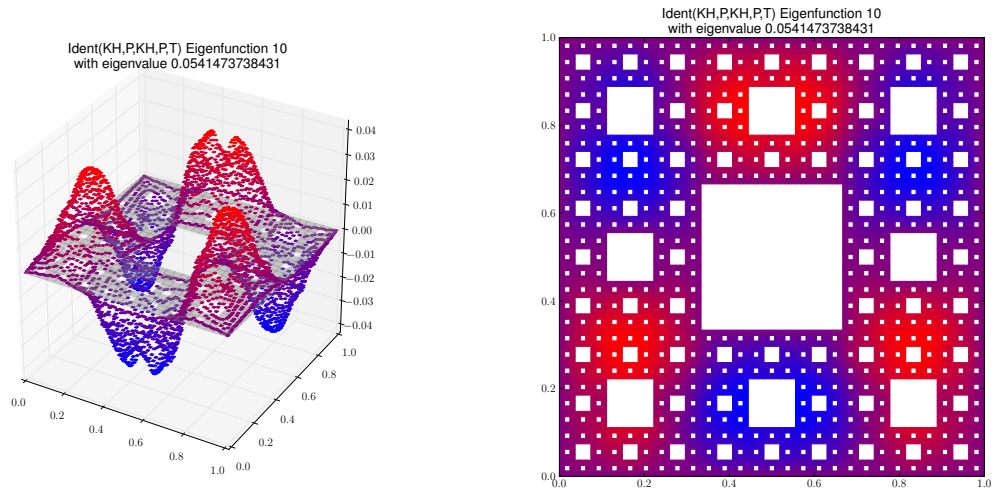
Eigenfunction 10 with eigenvalue 0.0541473738431
