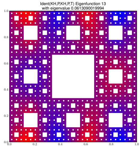
Eigenfunction 13 with eigenvalue 0.0613090019994
