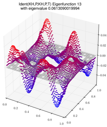
Eigenfunction 13 with eigenvalue 0.0613090019994
