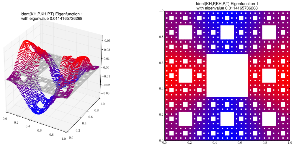
Eigenfunction 1 with eigenvalue 0.0114165736268
