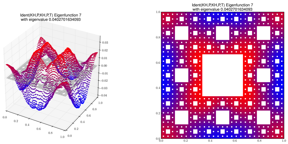
Eigenfunction 7 with eigenvalue 0.0402701634093
