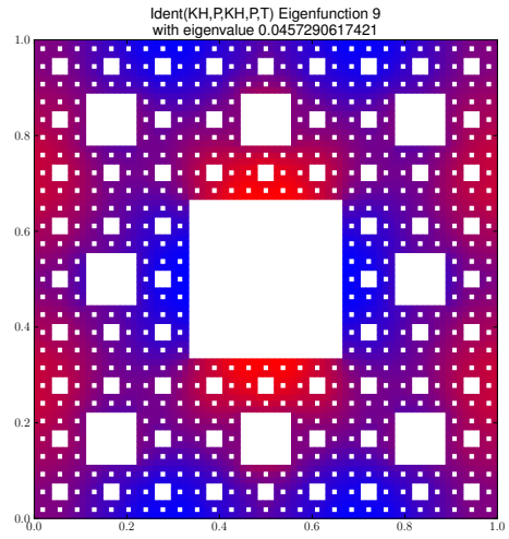
Eigenfunction 9 with eigenvalue 0.0457290617421
