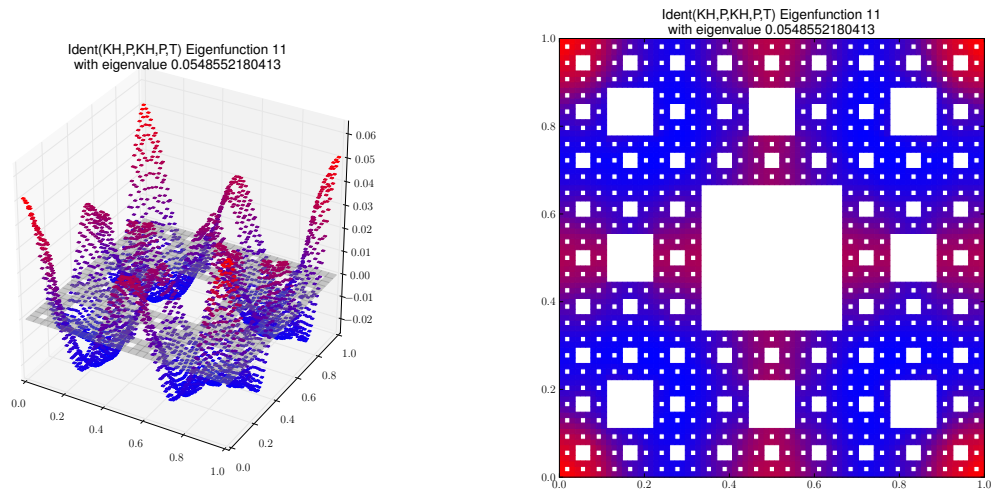
Eigenfunction 11 with eigenvalue 0.0548552180413
