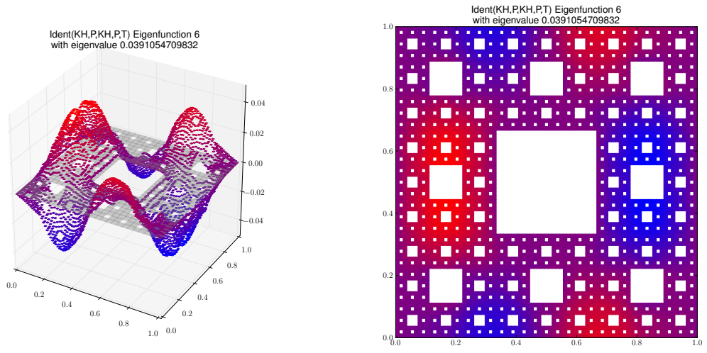
Eigenfunction 6 with eigenvalue 0.0391054709832
