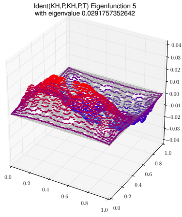
Eigenfunction 5 with eigenvalue 0.0291757352642
