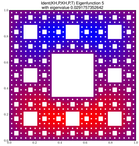
Eigenfunction 5 with eigenvalue 0.0291757352642
