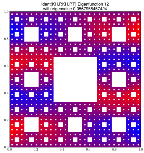
Eigenfunction 12 with eigenvalue 0.0567958457424
