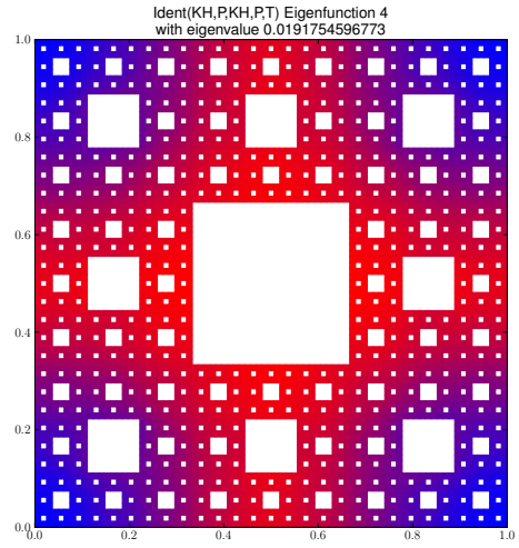
Eigenfunction 4 with eigenvalue 0.0191754596773
