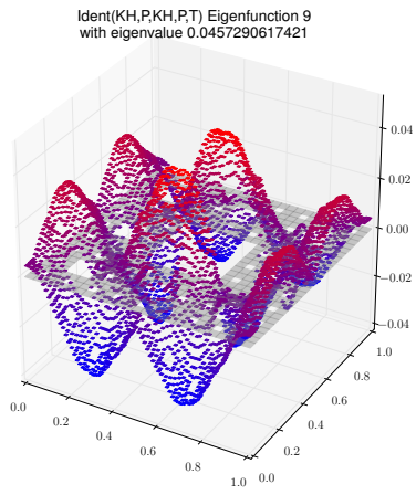
Eigenfunction 9 with eigenvalue 0.0457290617421
