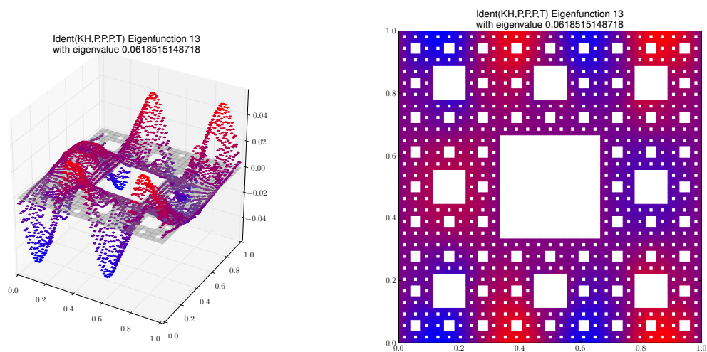
Eigenfunction 13 with eigenvalue 0.0618515148718
