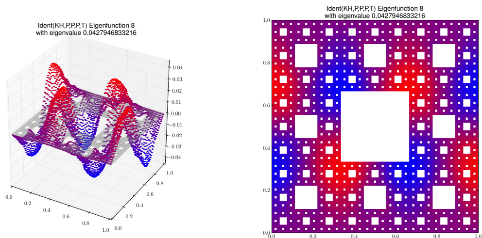
Eigenfunction 8 with eigenvalue 0.0427946833216
