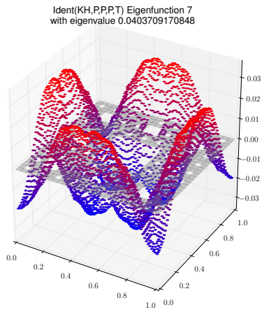
Eigenfunction 7 with eigenvalue 0.0403709170848
