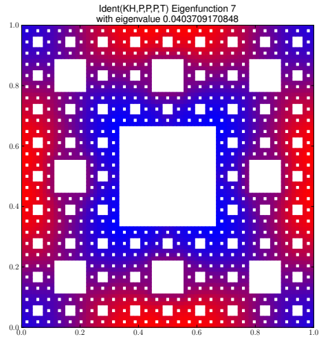
Eigenfunction 7 with eigenvalue 0.0403709170848
