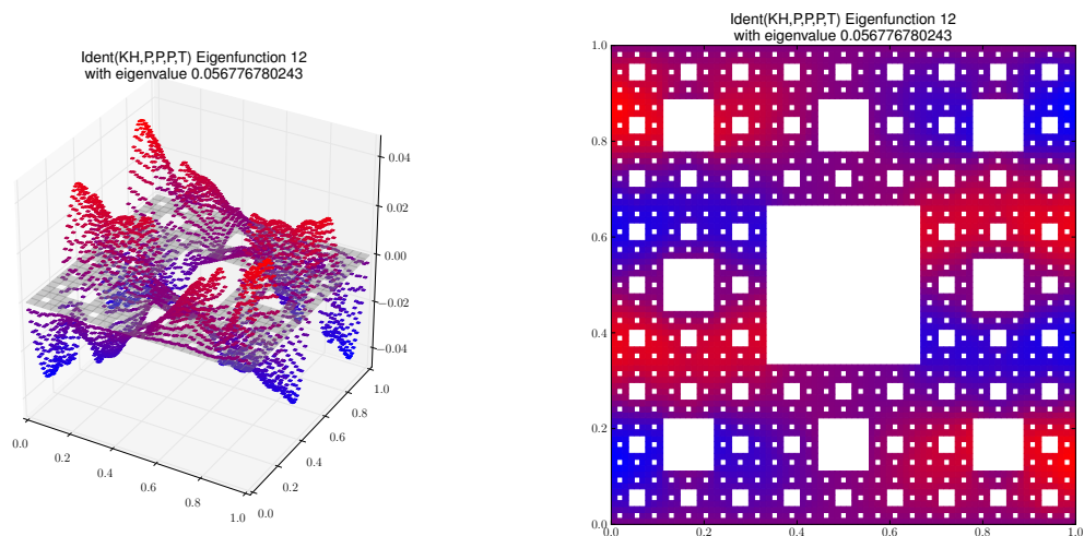
Eigenfunction 12 with eigenvalue 0.056776780243
