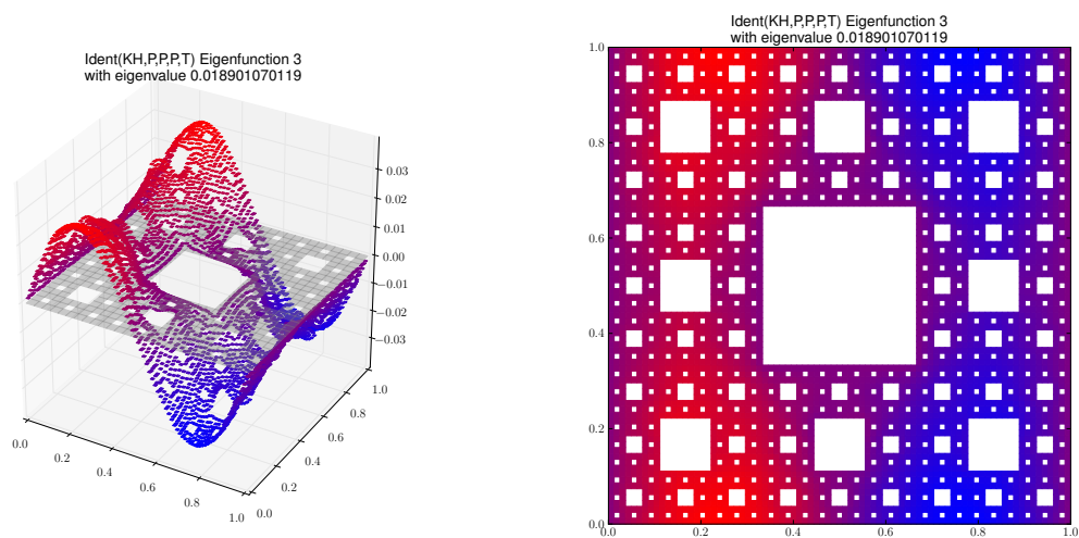
Eigenfunction 3 with eigenvalue 0.018901070119
