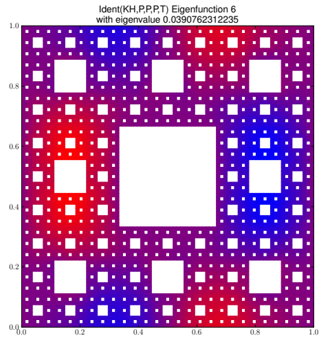
Eigenfunction 6 with eigenvalue 0.0390762312235
