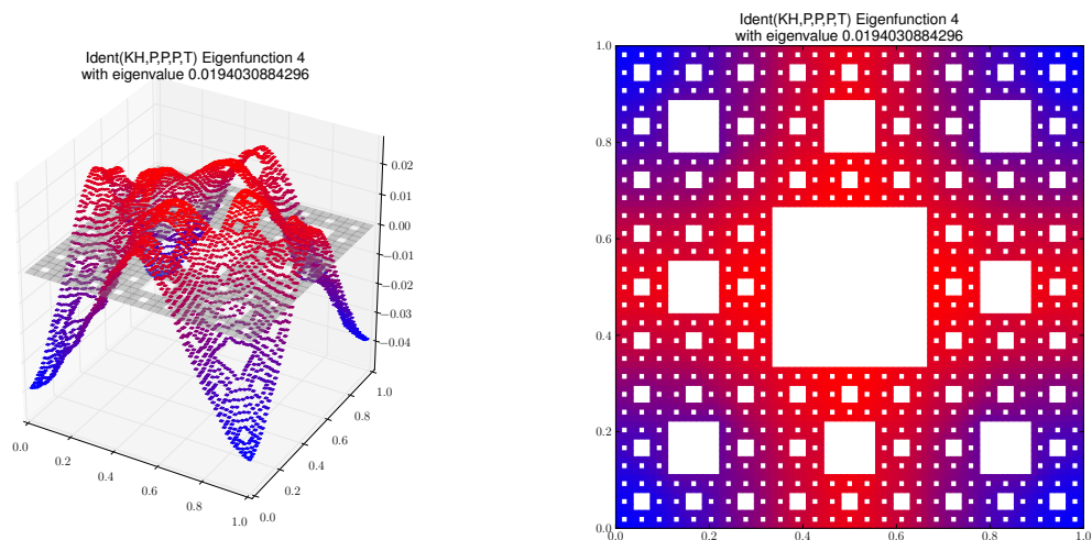
Eigenfunction 4 with eigenvalue 0.0194030884296
