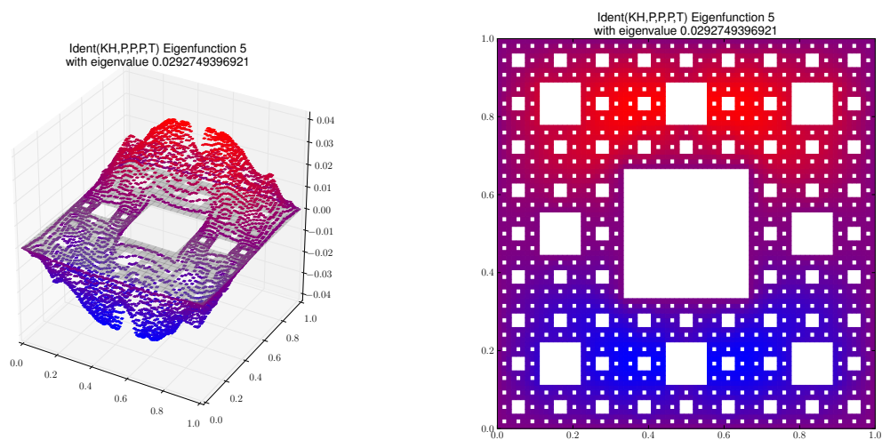
Eigenfunction 5 with eigenvalue 0.0292749396921
