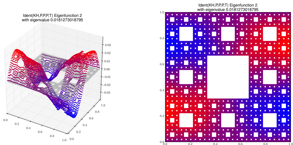
Eigenfunction 2 with eigenvalue 0.0181273018795
