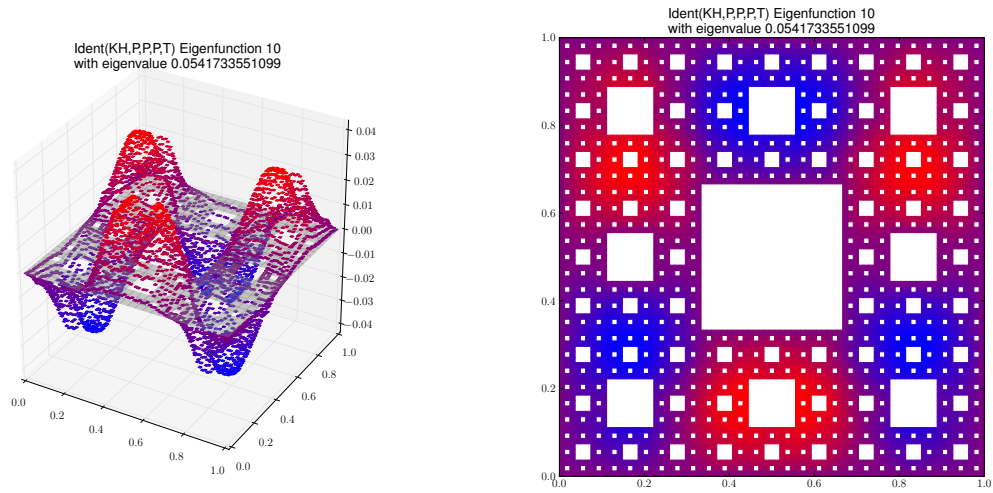
Eigenfunction 10 with eigenvalue 0.0541733551099
