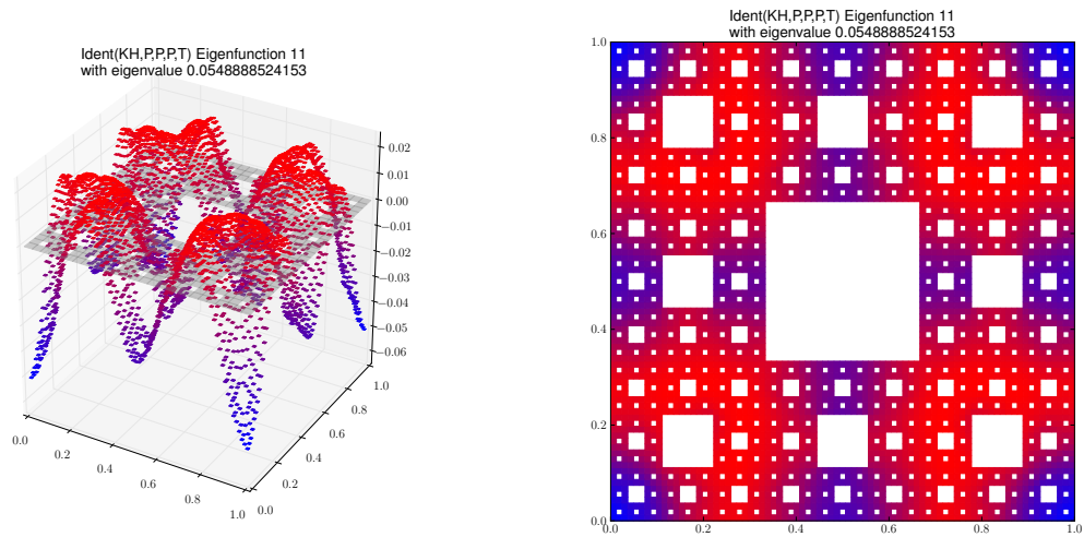
Eigenfunction 11 with eigenvalue 0.0548888524153
