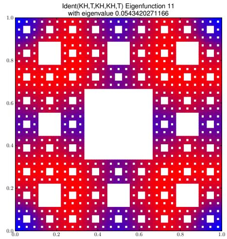
Eigenfunction 11 with eigenvalue 0.0543420271166
