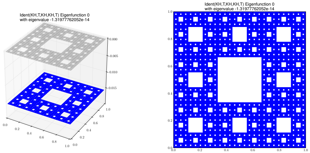
Eigenfunction 0 with eigenvalue -1.31977762052e-14
