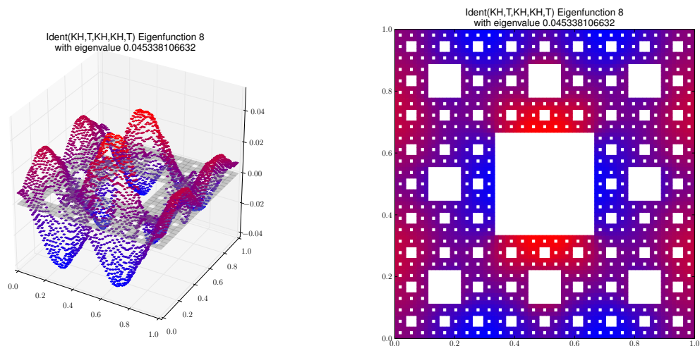
Eigenfunction 8 with eigenvalue 0.045338106632
