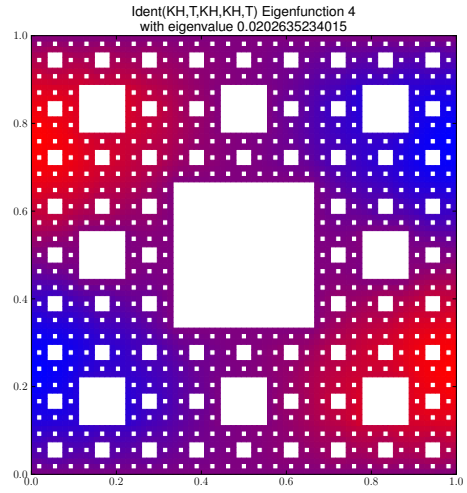
Eigenfunction 4 with eigenvalue 0.0202635234015
