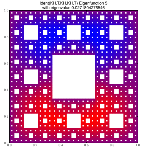
Eigenfunction 5 with eigenvalue 0.0271804276546
