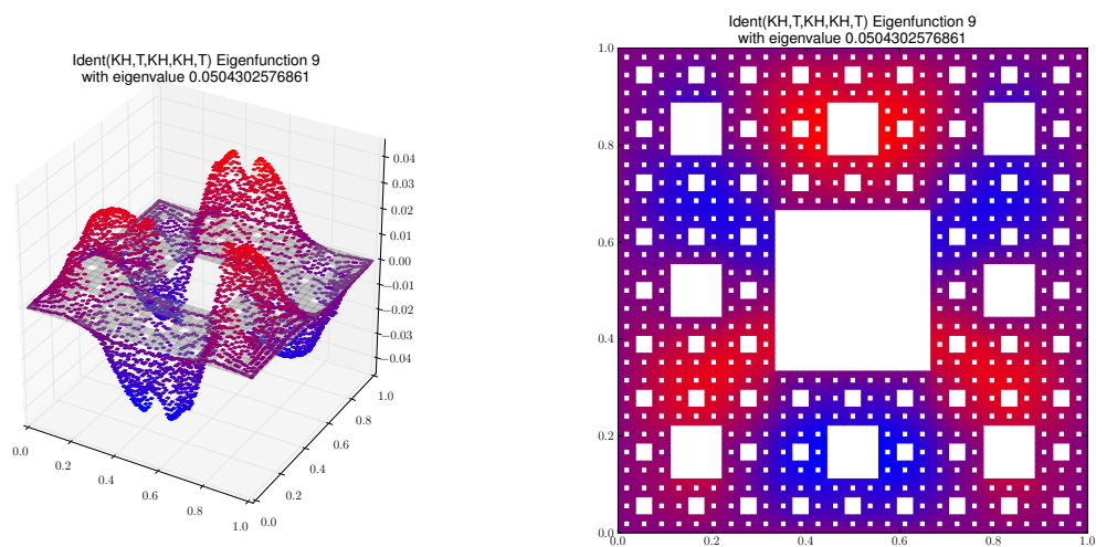
Eigenfunction 9 with eigenvalue 0.0504302576861
