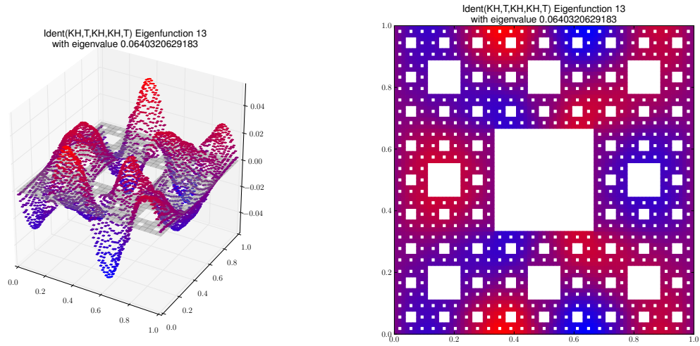
Eigenfunction 13 with eigenvalue 0.0640320629183
