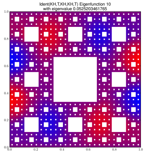
Eigenfunction 10 with eigenvalue 0.0525203461765
