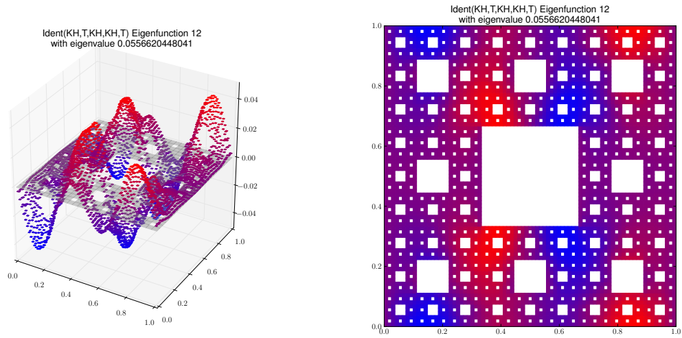
Eigenfunction 12 with eigenvalue 0.0556620448041
