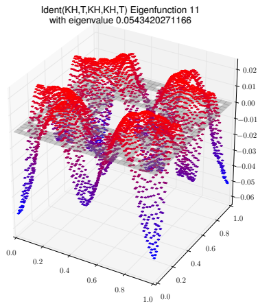
Eigenfunction 11 with eigenvalue 0.0543420271166
