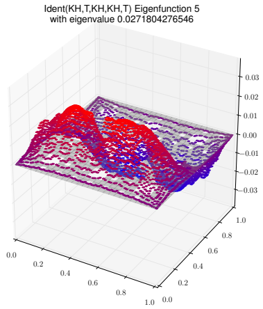
Eigenfunction 5 with eigenvalue 0.0271804276546
