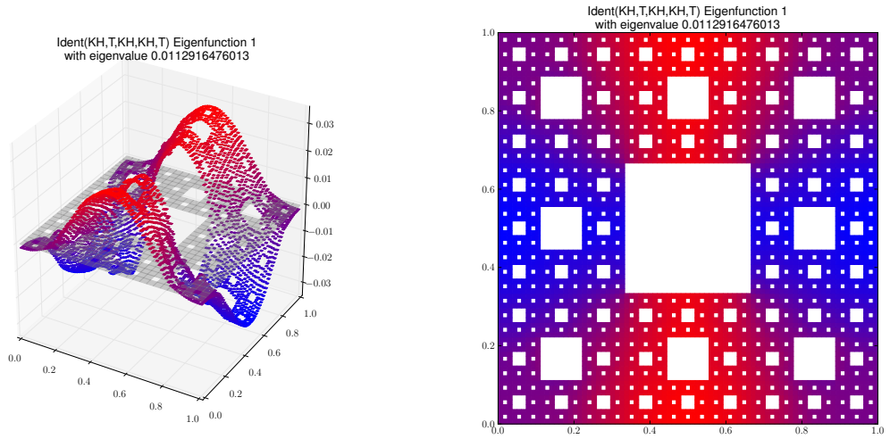
Eigenfunction 1 with eigenvalue 0.0112916476013
