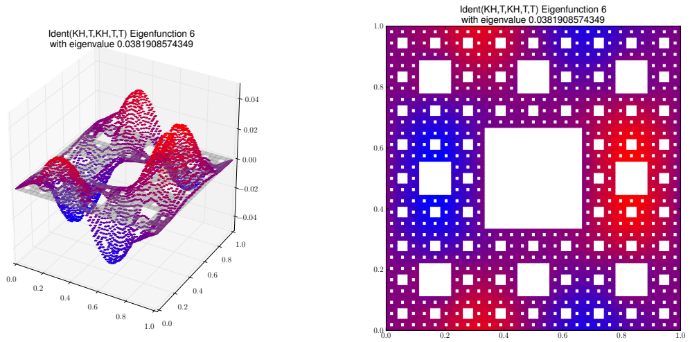
Eigenfunction 6 with eigenvalue 0.0381908574349
