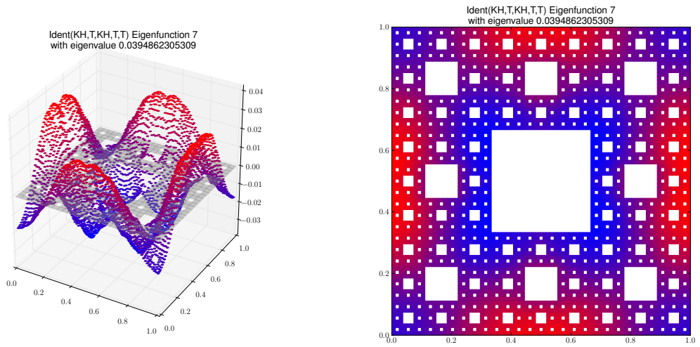
Eigenfunction 7 with eigenvalue 0.0394862305309
