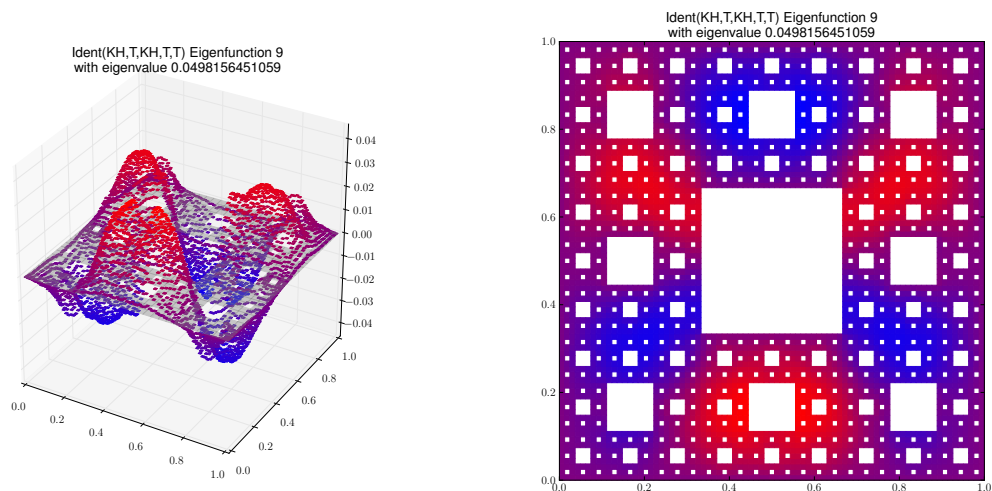
Eigenfunction 9 with eigenvalue 0.0498156451059
