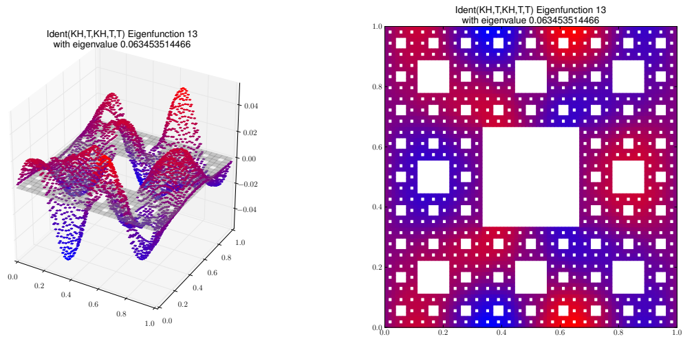
Eigenfunction 13 with eigenvalue 0.063453514466
