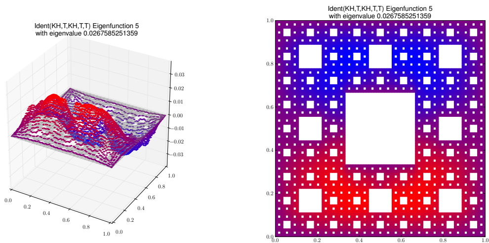
Eigenfunction 5 with eigenvalue 0.0267585251359
