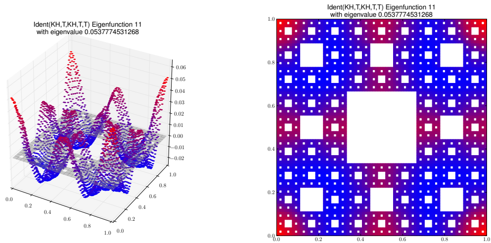
Eigenfunction 11 with eigenvalue 0.0537774531268
