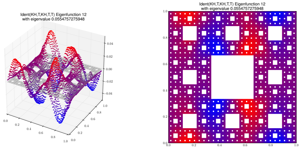
Eigenfunction 12 with eigenvalue 0.0554757275948
