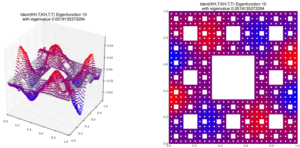
Eigenfunction 10 with eigenvalue 0.0519135373294
