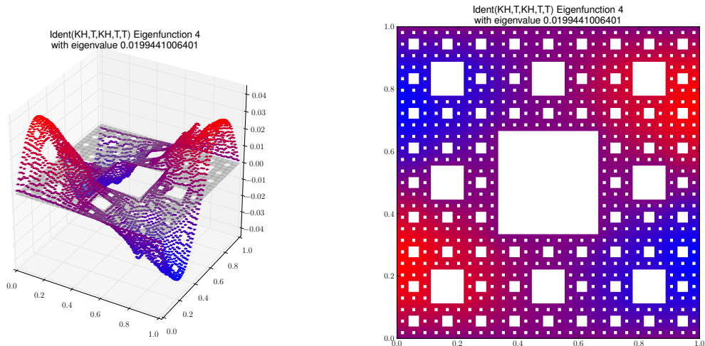
Eigenfunction 4 with eigenvalue 0.0199441006401
