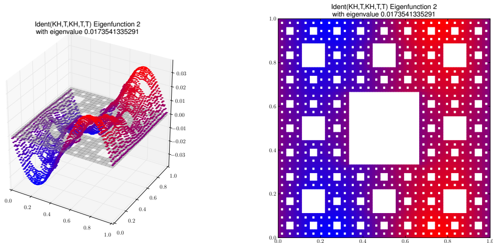
Eigenfunction 2 with eigenvalue 0.0173541335291
