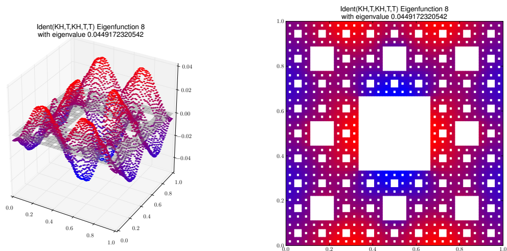
Eigenfunction 8 with eigenvalue 0.0449172320542
