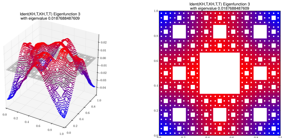
Eigenfunction 3 with eigenvalue 0.0187688487609
