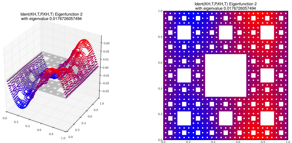
Eigenfunction 2 with eigenvalue 0.0176726057494
