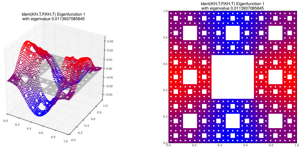
Eigenfunction 1 with eigenvalue 0.0113937085845
