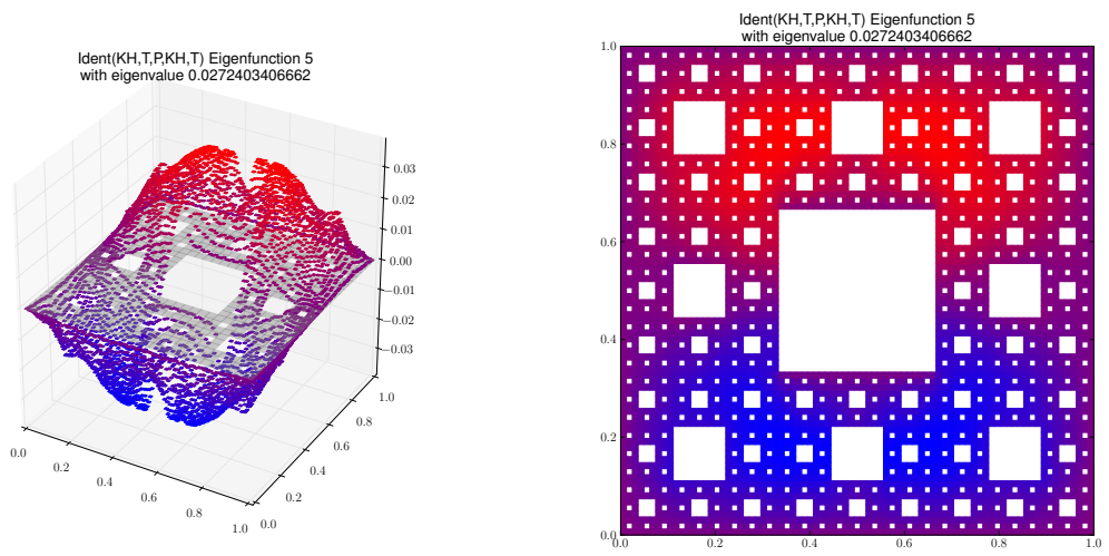
Eigenfunction 5 with eigenvalue 0.0272403406662
