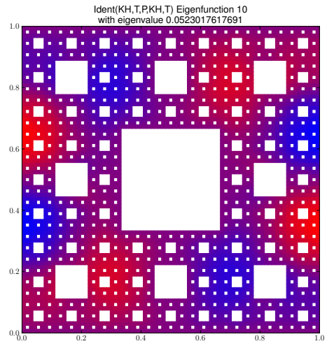
Eigenfunction 10 with eigenvalue 0.0523017617691
