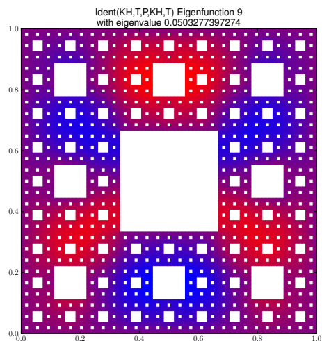
Eigenfunction 9 with eigenvalue 0.0503277397274
