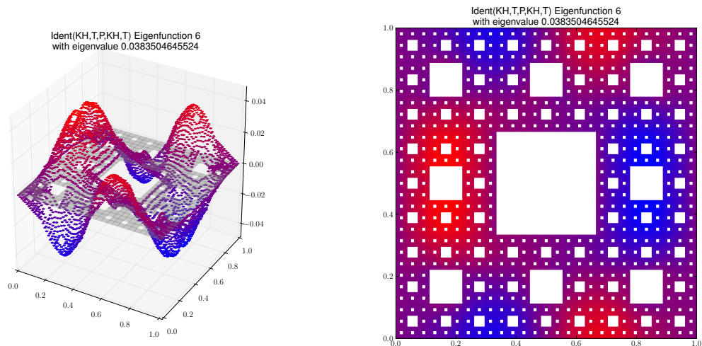
Eigenfunction 6 with eigenvalue 0.0383504645524
