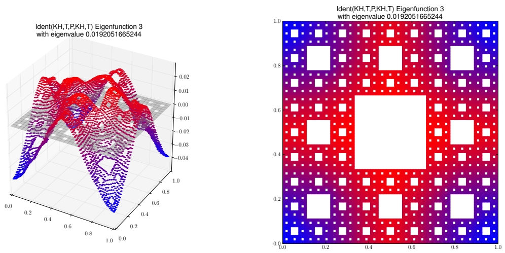
Eigenfunction 3 with eigenvalue 0.0192051665244
