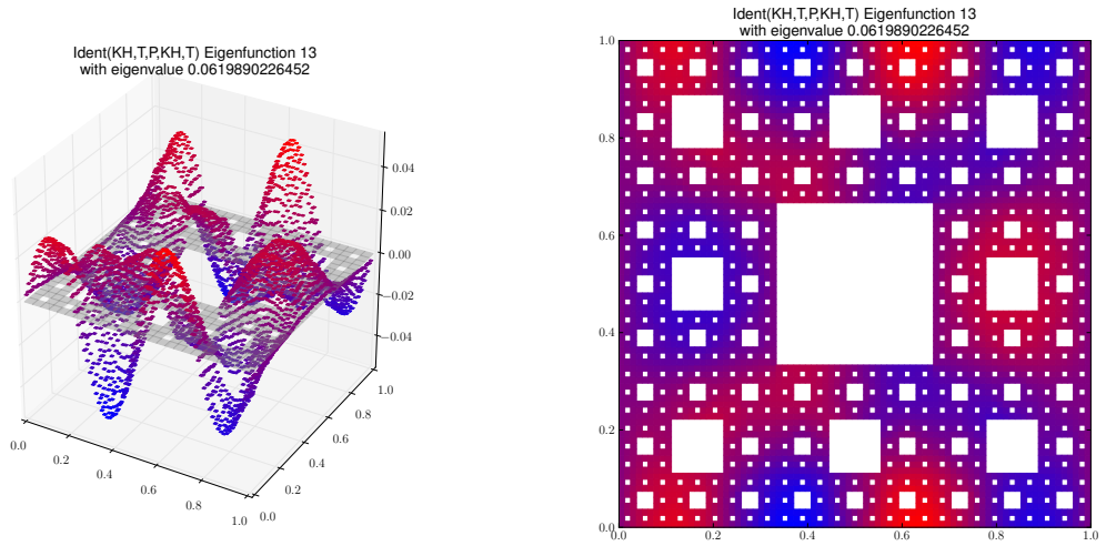
Eigenfunction 13 with eigenvalue 0.0619890226452
