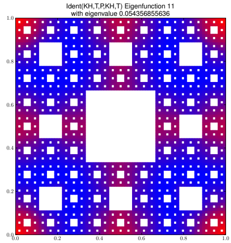
Eigenfunction 11 with eigenvalue 0.054356855636
