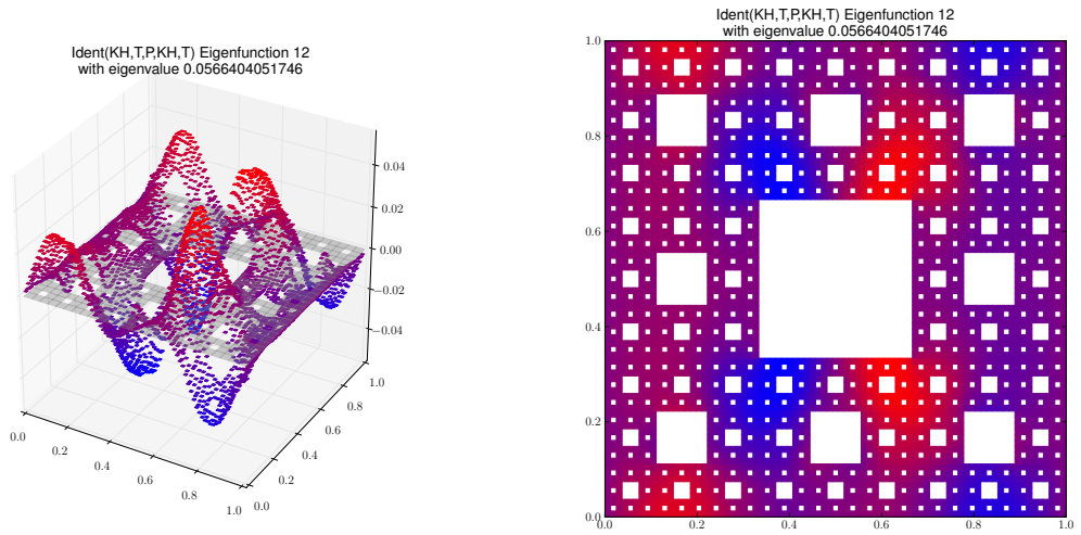
Eigenfunction 12 with eigenvalue 0.0566404051746
