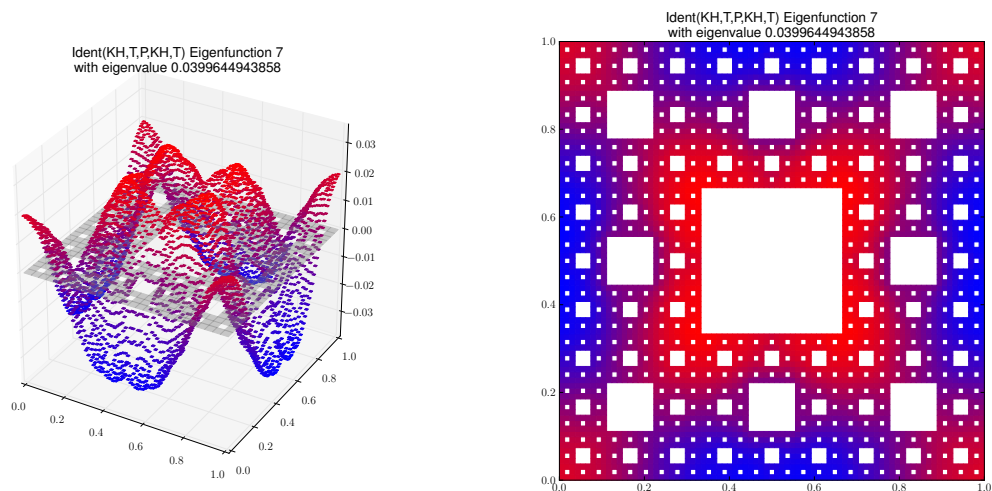
Eigenfunction 7 with eigenvalue 0.0399644943858
