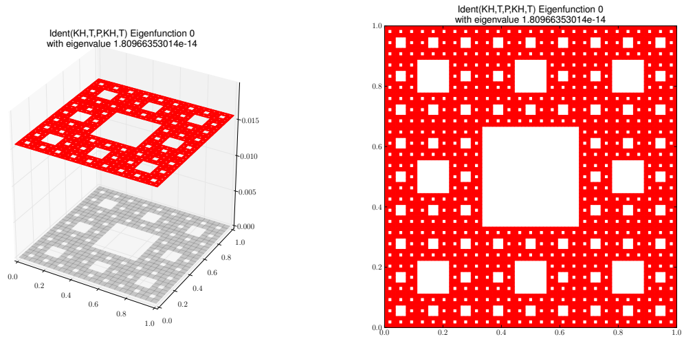
Eigenfunction 0 with eigenvalue 1.80966353014 \times 10^{-14}
