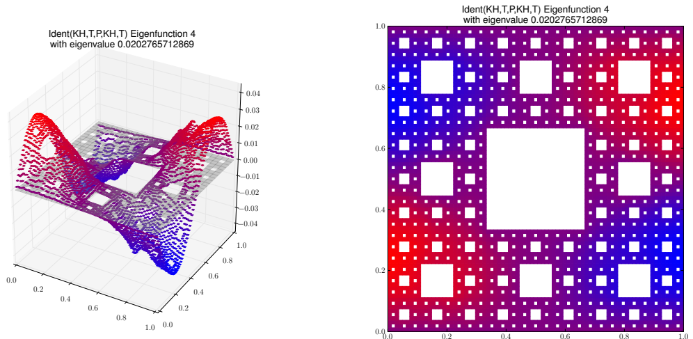
Eigenfunction 4 with eigenvalue 0.0202765712869
