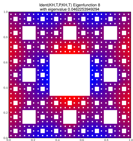
Eigenfunction 8 with eigenvalue 0.0462253949294
