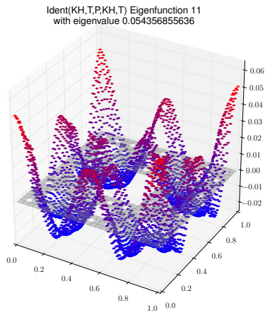
Eigenfunction 11 with eigenvalue 0.054356855636
