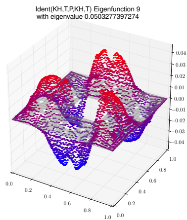
Eigenfunction 9 with eigenvalue 0.0503277397274
