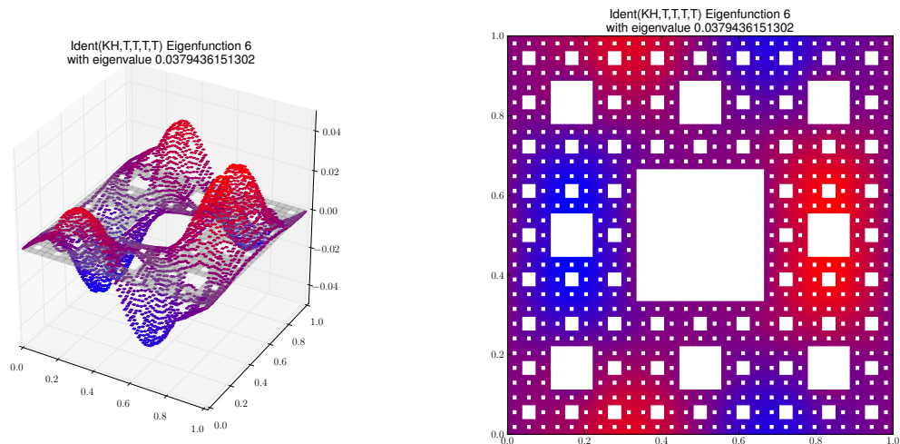
Eigenfunction 6 with eigenvalue 0.0379436151302
