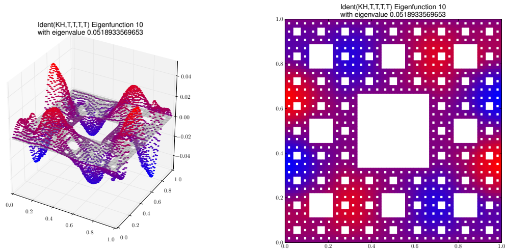
Eigenfunction 10 with eigenvalue 0.0518933569653
