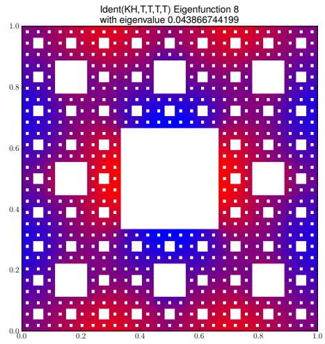
Eigenfunction 8 with eigenvalue 0.043866744199
