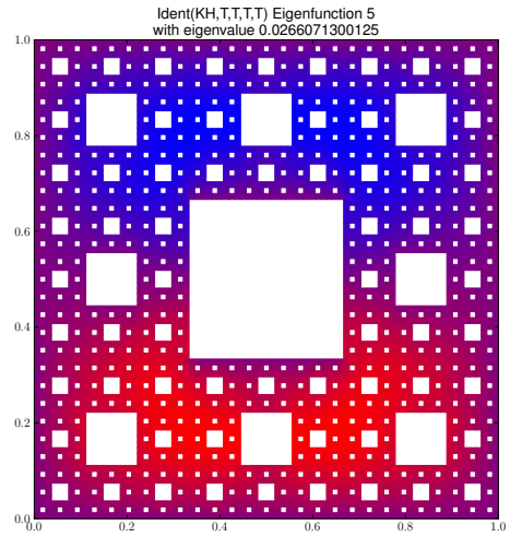
Eigenfunction 5 with eigenvalue 0.0266071300125
