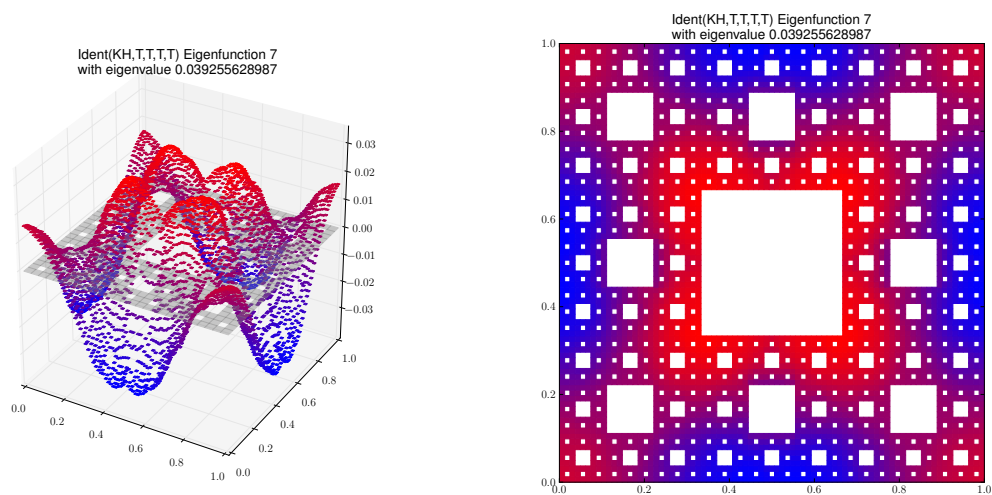
Eigenfunction 7 with eigenvalue 0.039255628987
