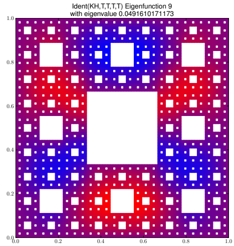
Eigenfunction 9 with eigenvalue 0.0491610171173
