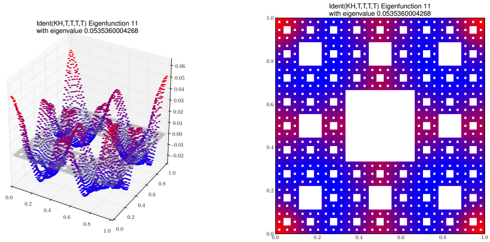
Eigenfunction 11 with eigenvalue 0.0535360004268
