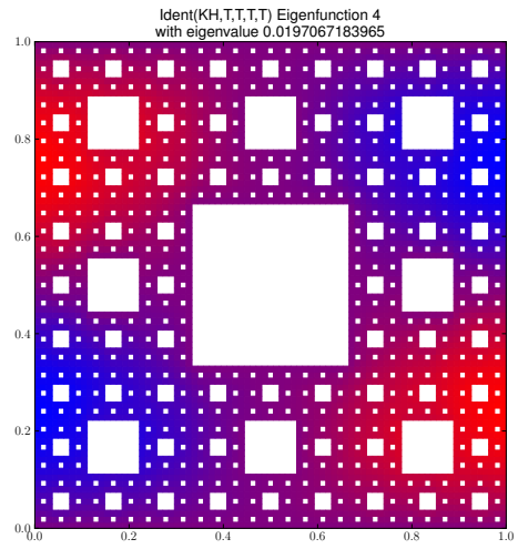
Eigenfunction 4 with eigenvalue 0.0197067183965
