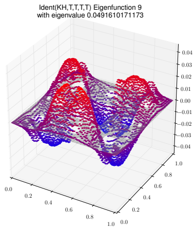
Eigenfunction 9 with eigenvalue 0.0491610171173
