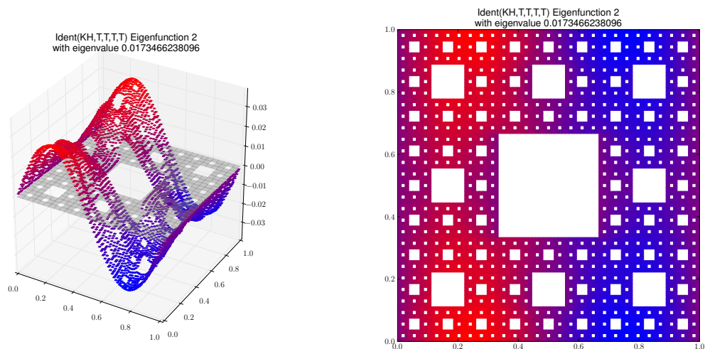
Eigenfunction 2 with eigenvalue 0.0173466238096
