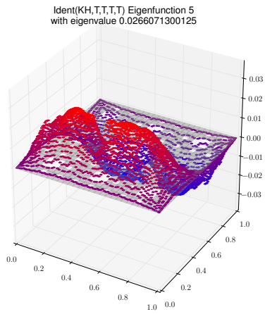
Eigenfunction 5 with eigenvalue 0.0266071300125
