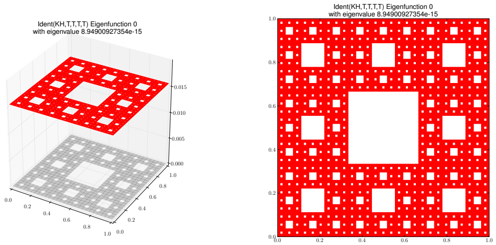
Eigenfunction 0 with eigenvalue 8.94900927354e-15
