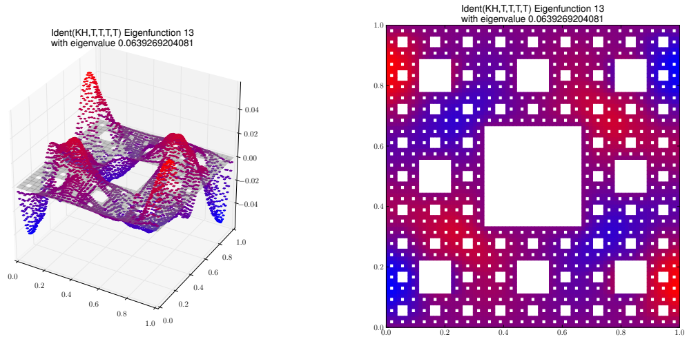
Eigenfunction 13 with eigenvalue 0.0639269204081
