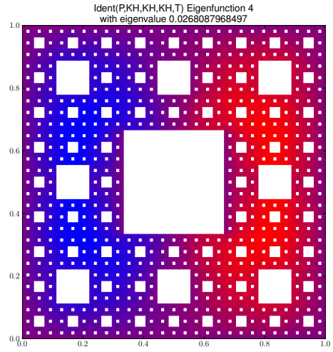
Eigenfunction 4 with eigenvalue 0.0268087968497
