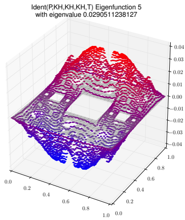
Eigenfunction 5 with eigenvalue 0.0290511238127
