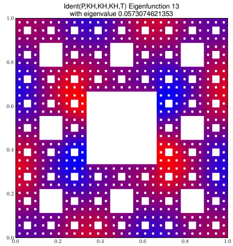
Eigenfunction 13 with eigenvalue 0.0573074621353
