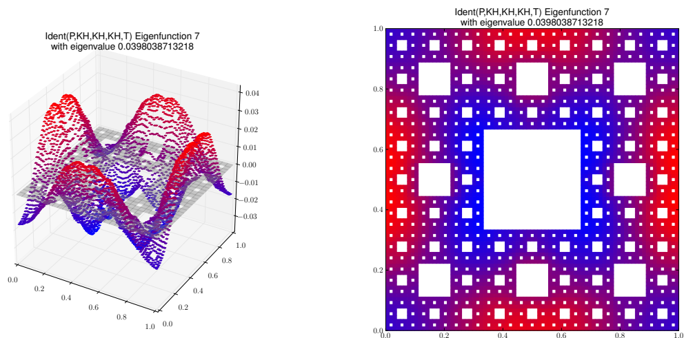
Eigenfunction 7 with eigenvalue 0.0398038713218
