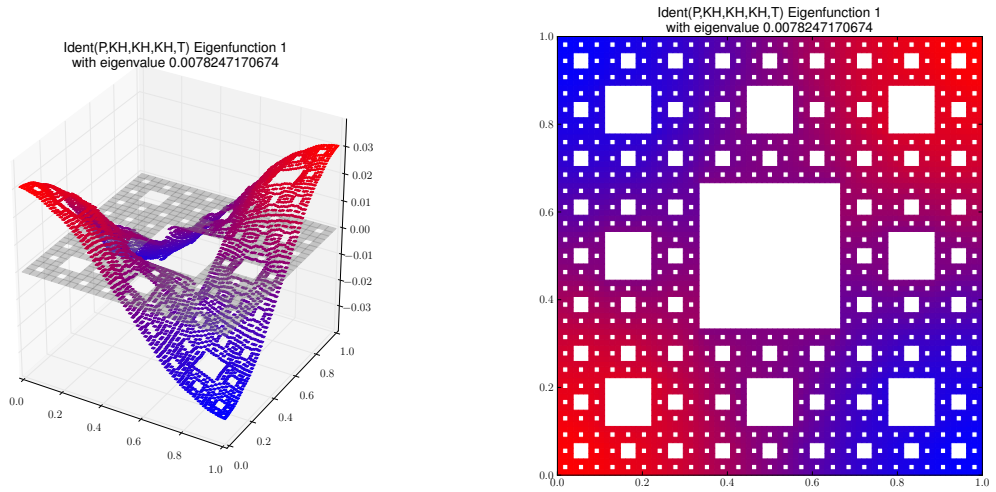
Eigenfunction 1 with eigenvalue 0.0078247170674
