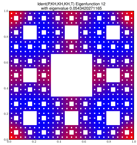
Eigenfunction 12 with eigenvalue 0.0543420271165
