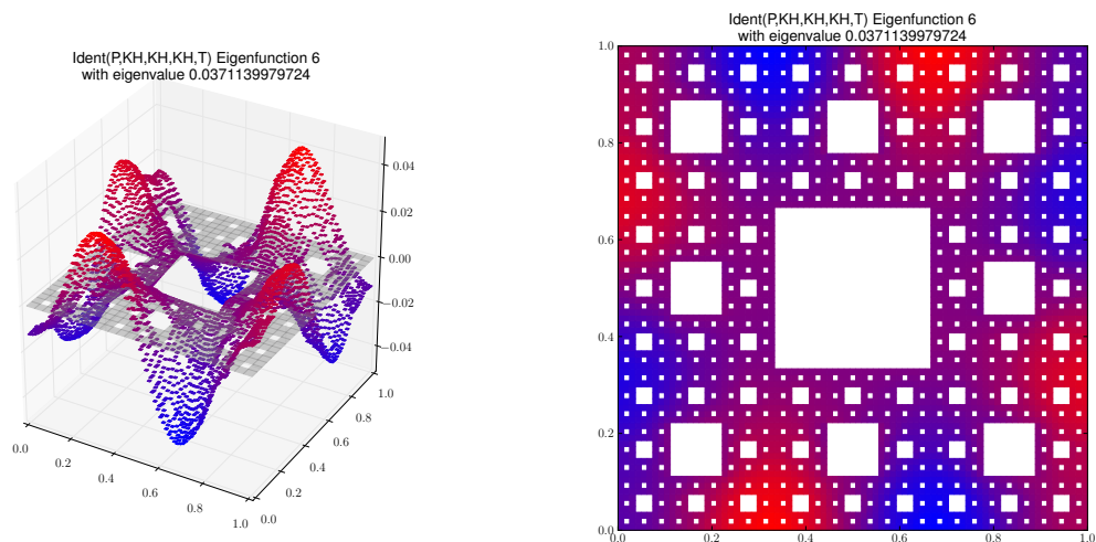
Eigenfunction 6 with eigenvalue 0.0371139979724
