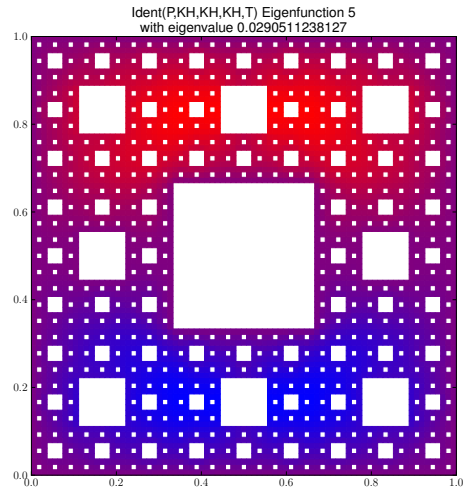
Eigenfunction 5 with eigenvalue 0.0290511238127
