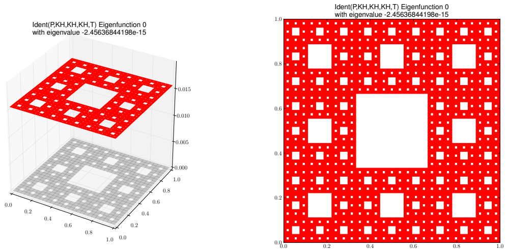
Eigenfunction 0 with eigenvalue -2.45636844198e-15
