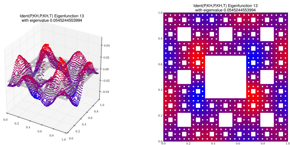
Eigenfunction 13 with eigenvalue 0.0545244553994
