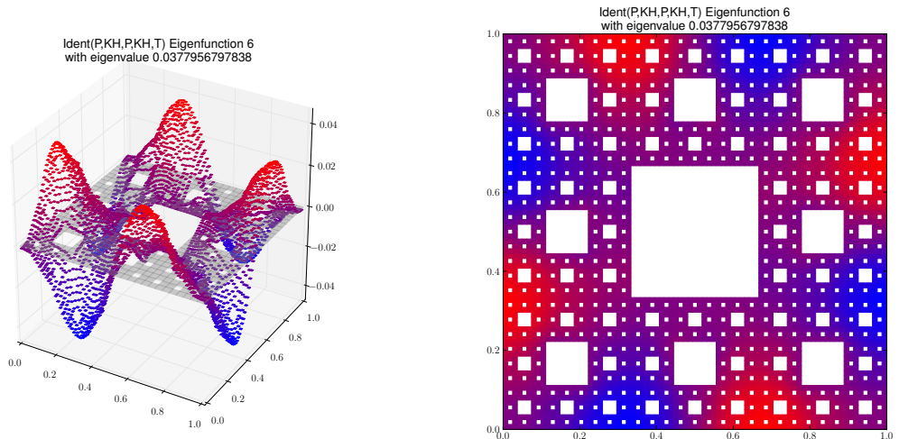
Eigenfunction 6 with eigenvalue 0.0377956797838
