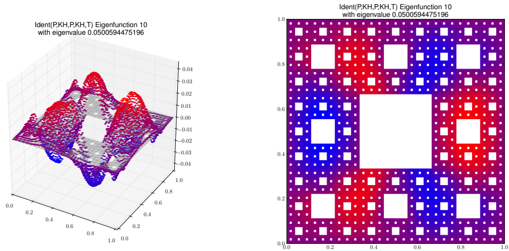
Eigenfunction 10 with eigenvalue 0.0500594475196
