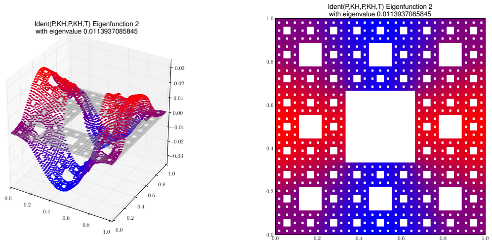
Eigenfunction 2 with eigenvalue 0.0113937085845
