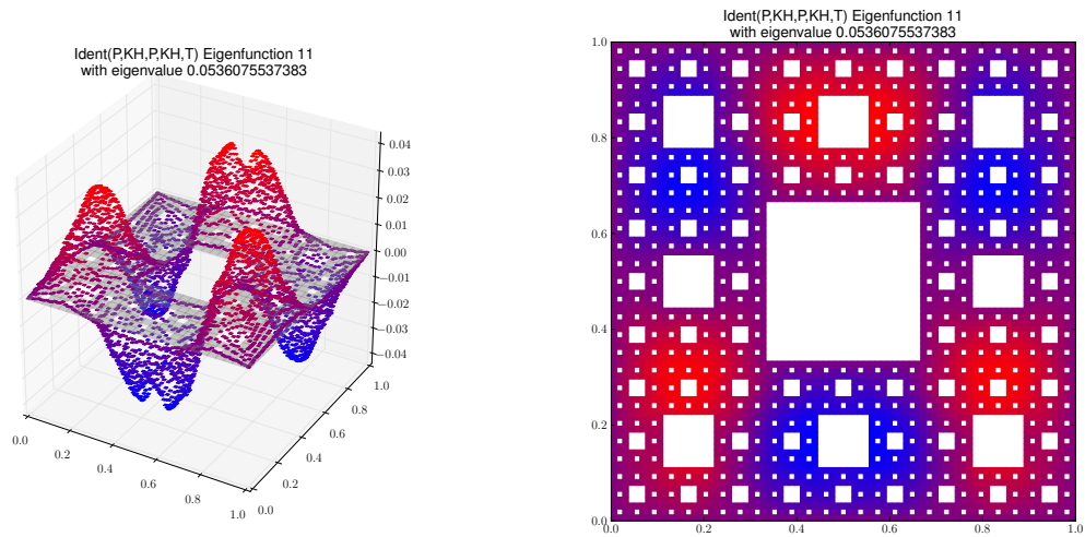
Eigenfunction 11 with eigenvalue 0.0536075537383
