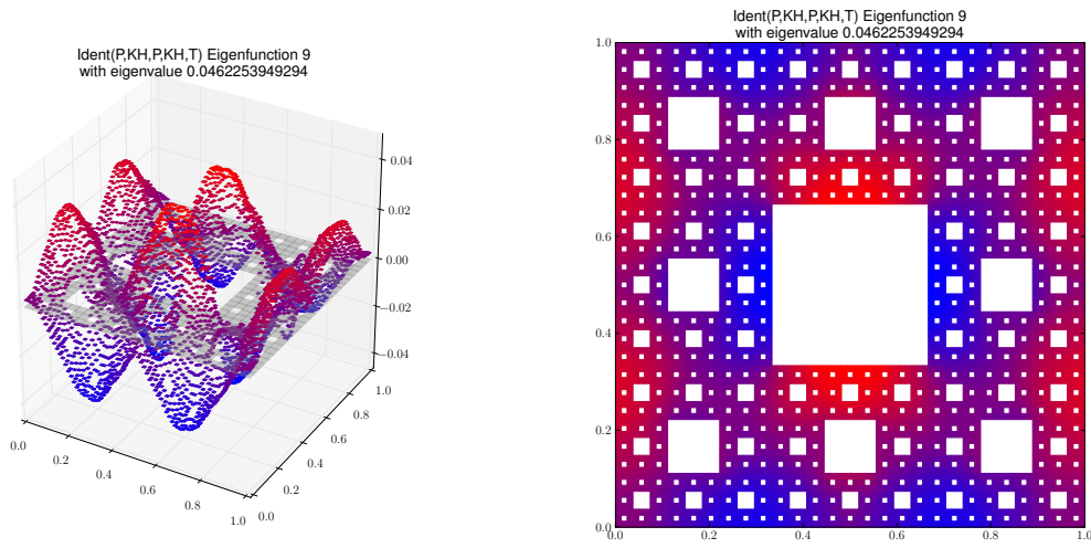
Eigenfunction 9 with eigenvalue 0.0462253949294
