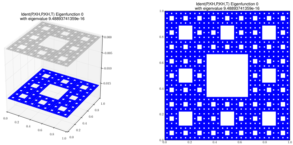
Eigenfunction 0 with eigenvalue 9.48893741359e-16
