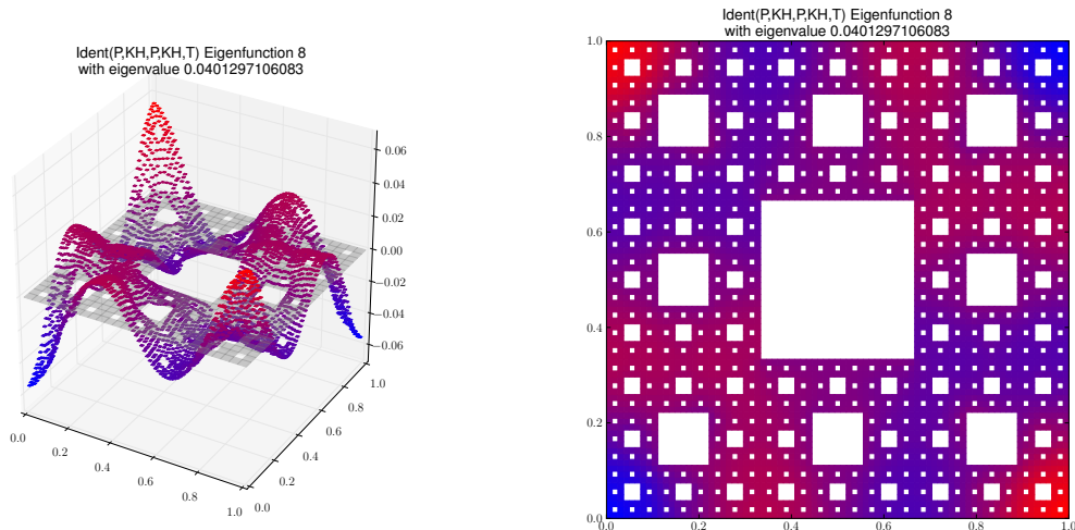
Eigenfunction 8 with eigenvalue 0.0401297106083
