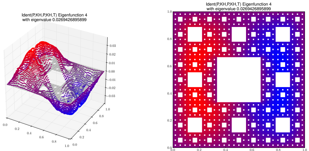
Eigenfunction 4 with eigenvalue 0.0269426895899
