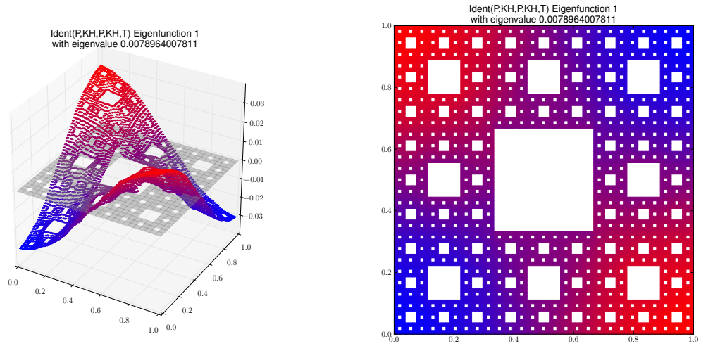
Eigenfunction 1 with eigenvalue 0.0078964007811
