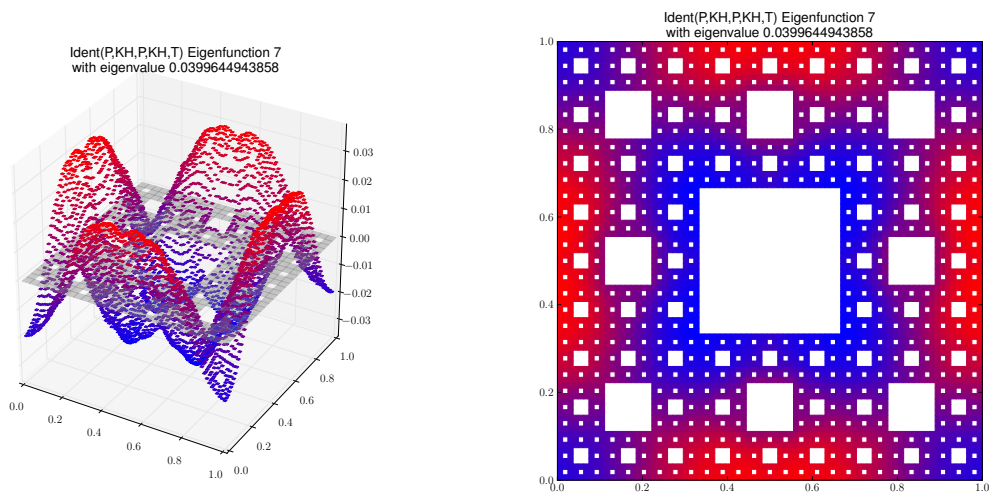
Eigenfunction 7 with eigenvalue 0.0399644943858
