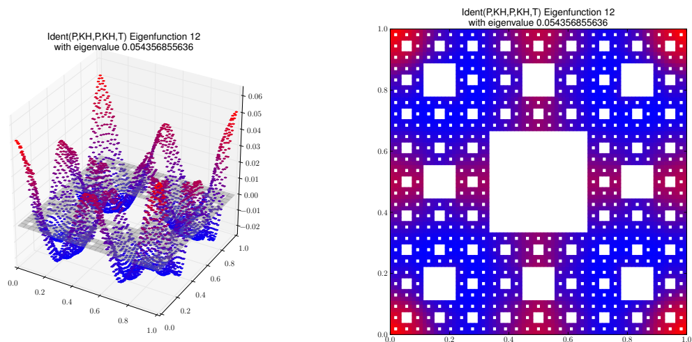
Eigenfunction 12 with eigenvalue 0.054356855636
