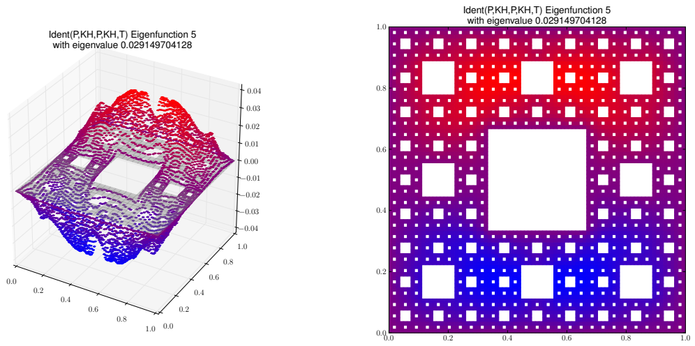
Eigenfunction 5 with eigenvalue 0.029149704128
