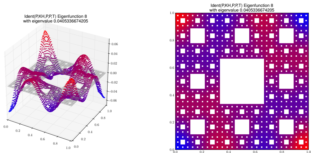
Eigenfunction 8 with eigenvalue 0.0405336674205
