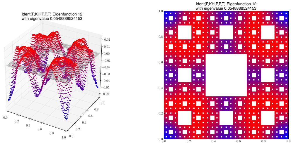
Eigenfunction 12 with eigenvalue 0.0548888524153
