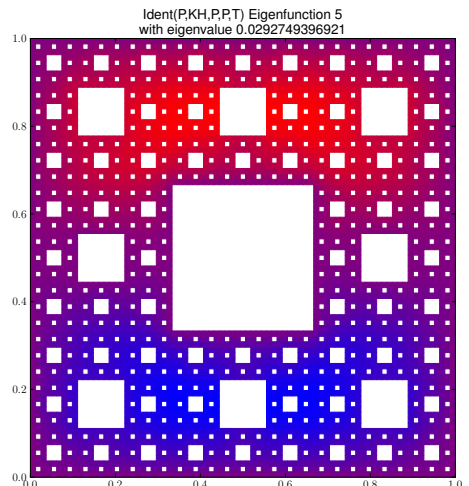
Eigenfunction 5 with eigenvalue 0.0292749396921
