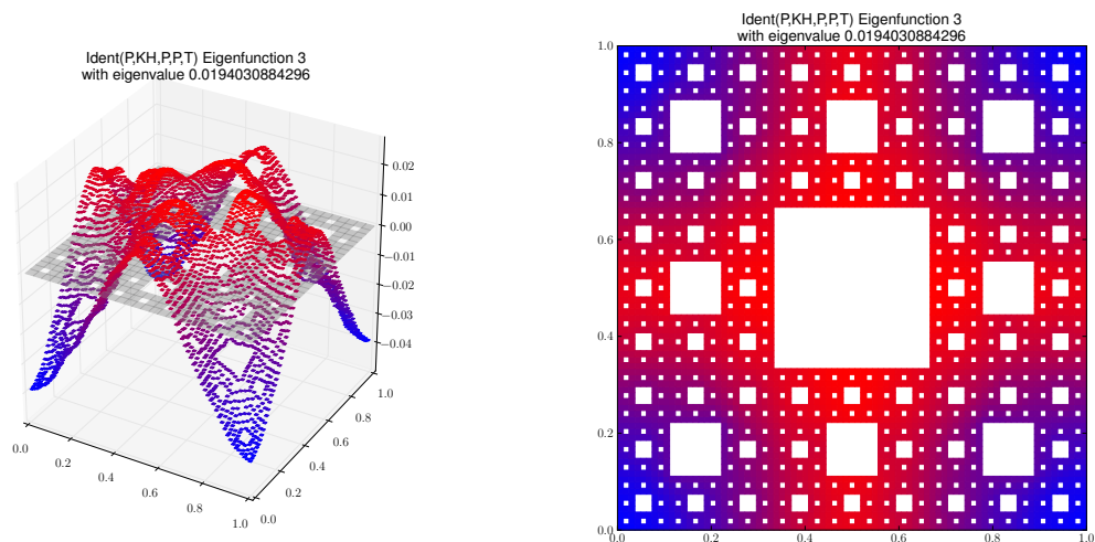
Eigenfunction 3 with eigenvalue 0.0194030884296
