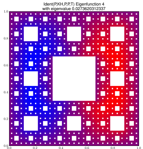
Eigenfunction 4 with eigenvalue 0.0273620312337
