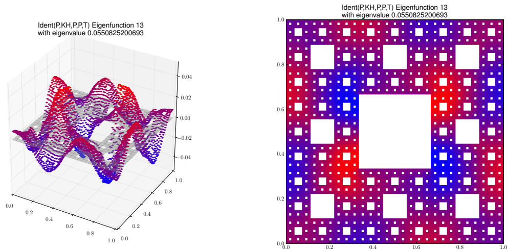
Eigenfunction 13 with eigenvalue 0.0550825200693
