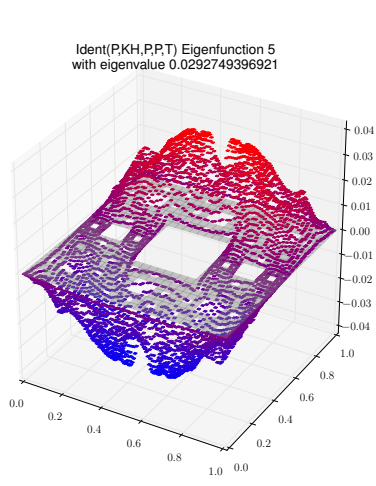
Eigenfunction 5 with eigenvalue 0.0292749396921
