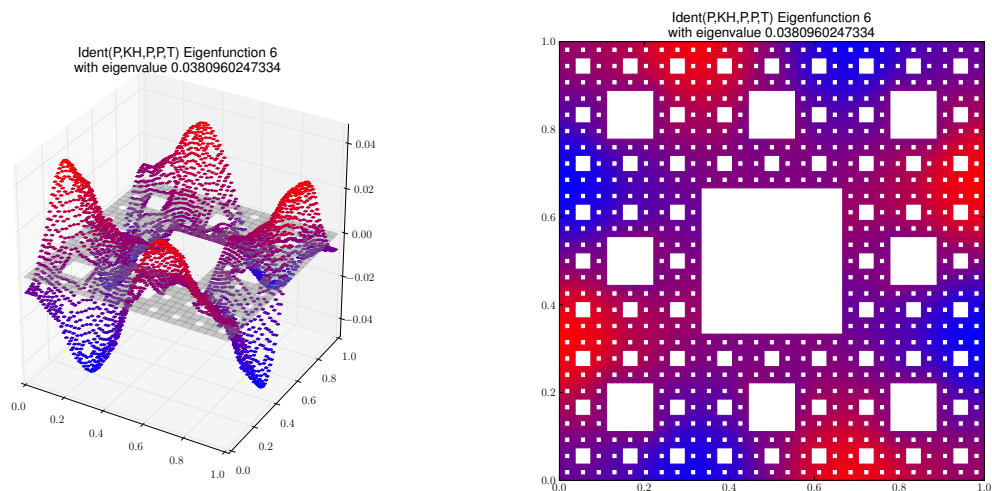
Eigenfunction 6 with eigenvalue 0.0380960247334
