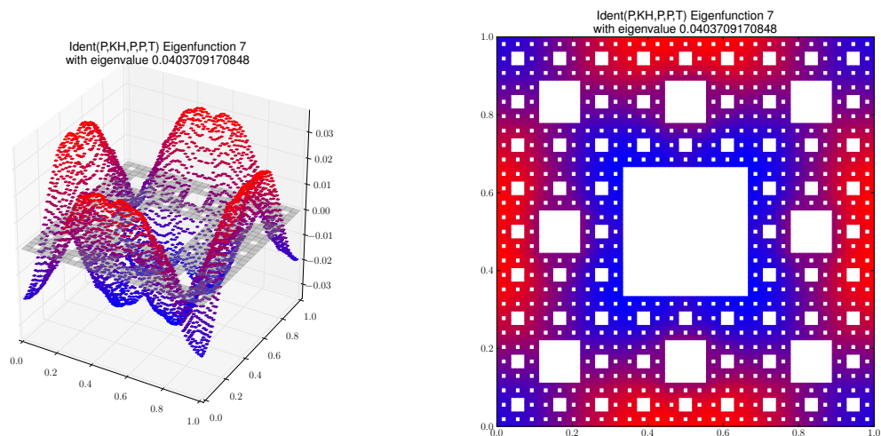
Eigenfunction 7 with eigenvalue 0.0403709170848
