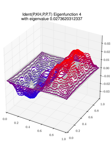
Eigenfunction 4 with eigenvalue 0.0273620312337
