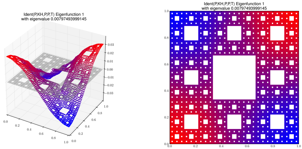
Eigenfunction 1 with eigenvalue 0.00797493999145
