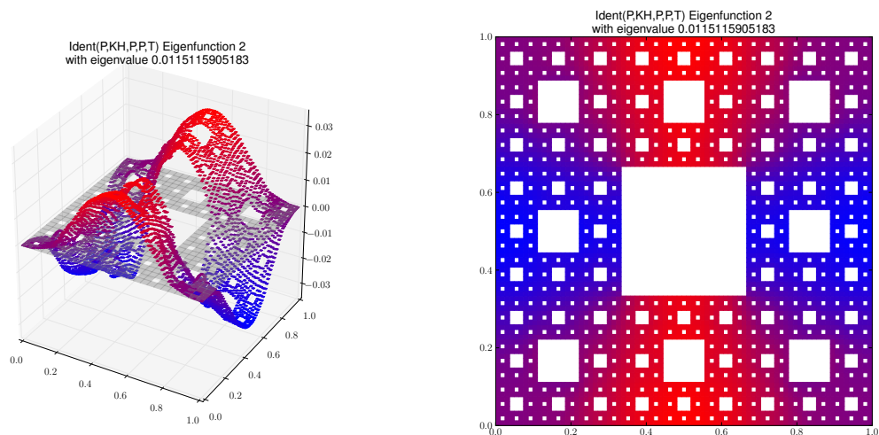
Eigenfunction 2 with eigenvalue 0.0115115905183
