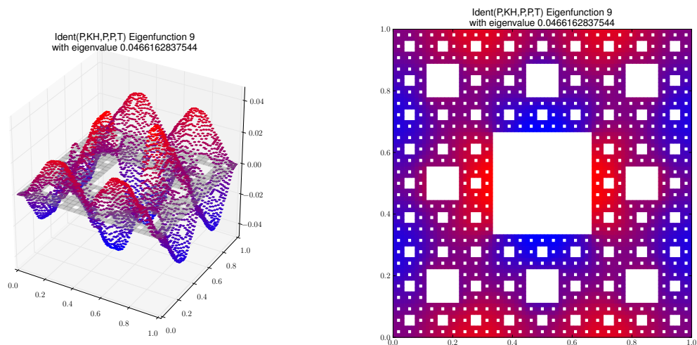
Eigenfunction 9 with eigenvalue 0.0466162837544
