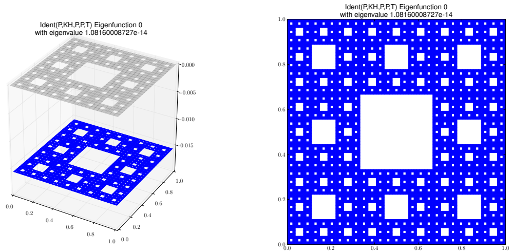
Eigenfunction 0 with eigenvalue 1.08160008727e-14
