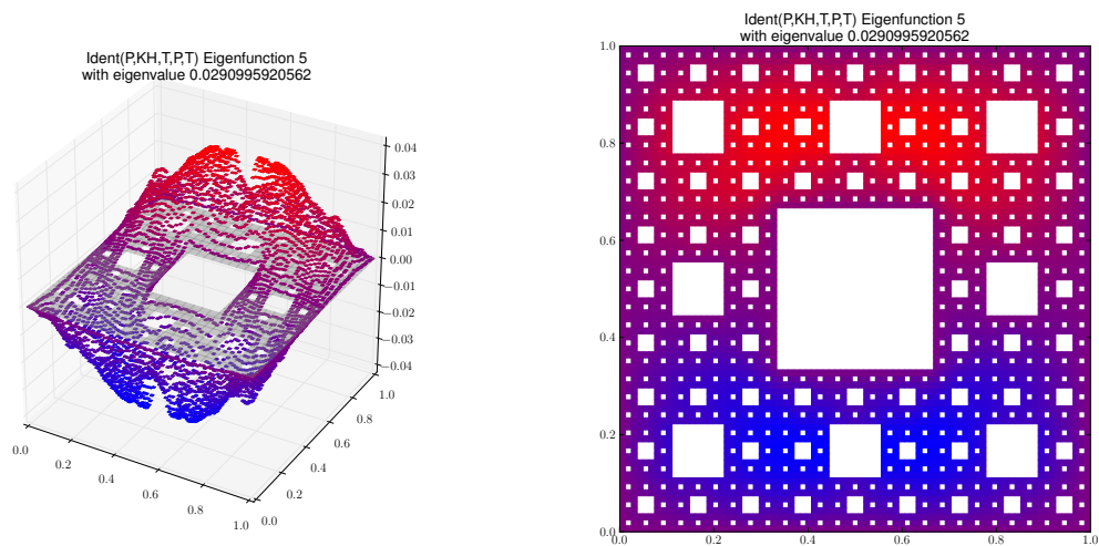
Eigenfunction 5 with eigenvalue 0.0290995920562
