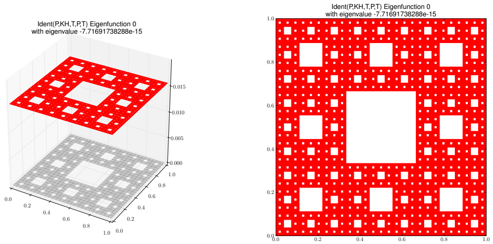
Eigenfunction 0 with eigenvalue -7.71691738288e-15
