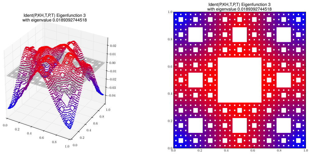
Eigenfunction 3 with eigenvalue 0.0189392744518
