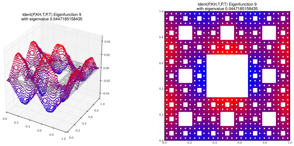
Eigenfunction 9 with eigenvalue 0.0447185158435
