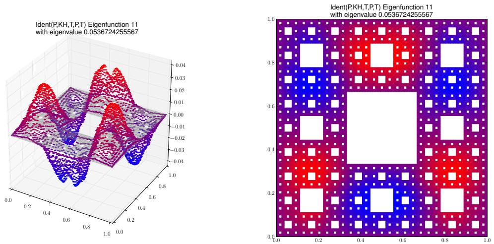
Eigenfunction 11 with eigenvalue 0.0536724255567
