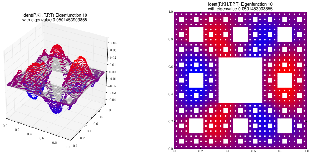
Eigenfunction 10 with eigenvalue 0.0501453903855
