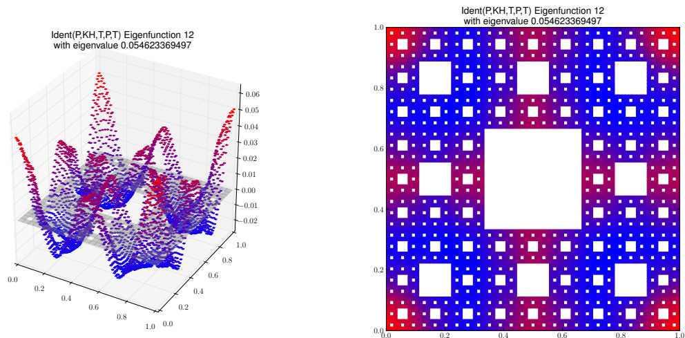
Eigenfunction 12 with eigenvalue 0.054623369497
