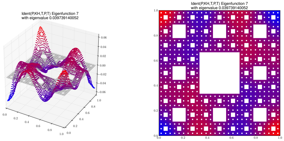
Eigenfunction 7 with eigenvalue 0.039739140052
