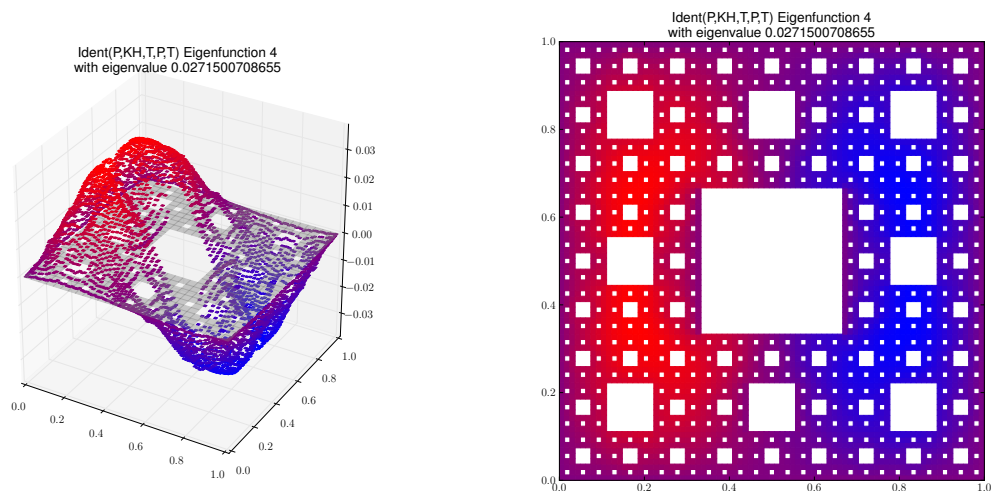
Eigenfunction 4 with eigenvalue 0.0271500708655
