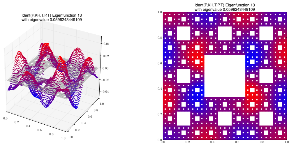
Eigenfunction 13 with eigenvalue 0.0596243449109
