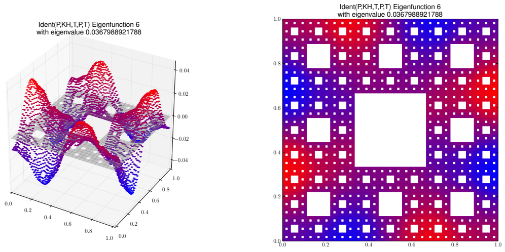
Eigenfunction 6 with eigenvalue 0.0367988921788
