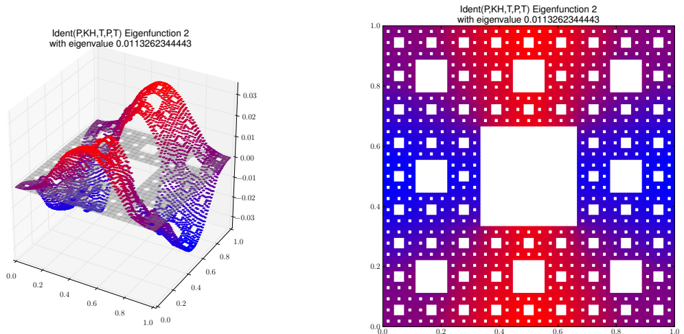
Eigenfunction 2 with eigenvalue 0.0113262344443
