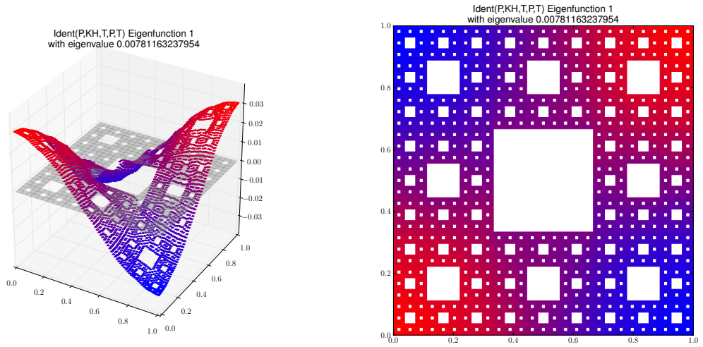
Eigenfunction 1 with eigenvalue 0.00781163237954
