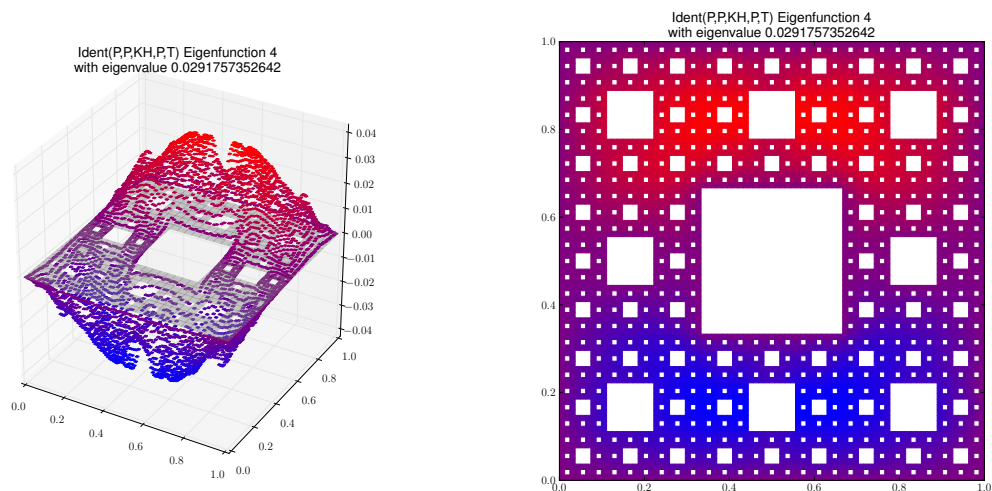
Eigenfunction 4 with eigenvalue 0.0291757352642
