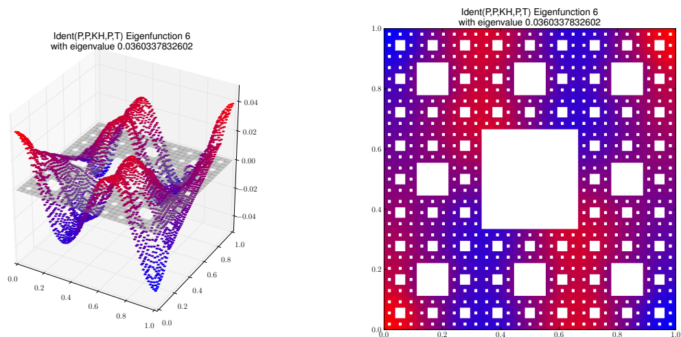
Eigenfunction 6 with eigenvalue 0.0360337832602
