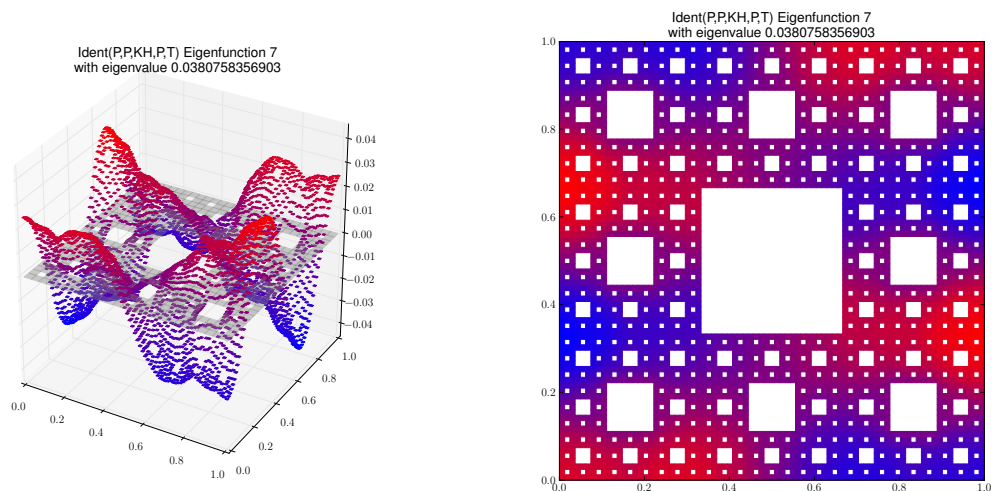
Eigenfunction 7 with eigenvalue 0.0380758356903
