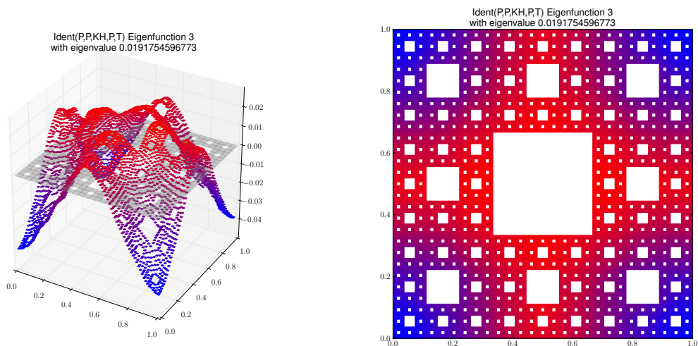
Eigenfunction 3 with eigenvalue 0.0191754596773
