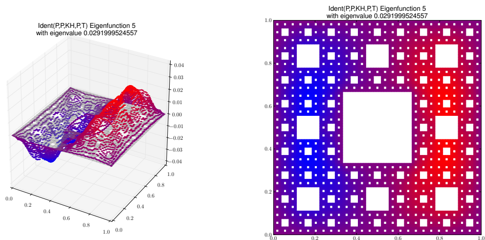
Eigenfunction 5 with eigenvalue 0.0291999524557
