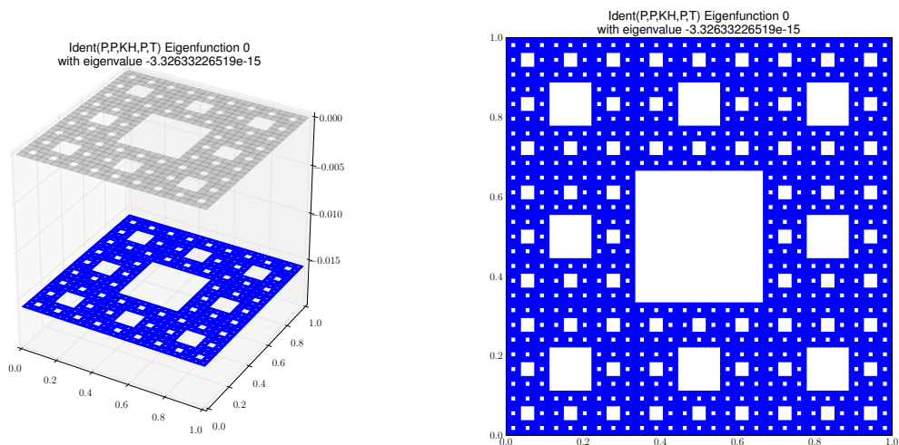
Eigenfunction 0 with eigenvalue -3.32633226519 \times 10^{-15}
