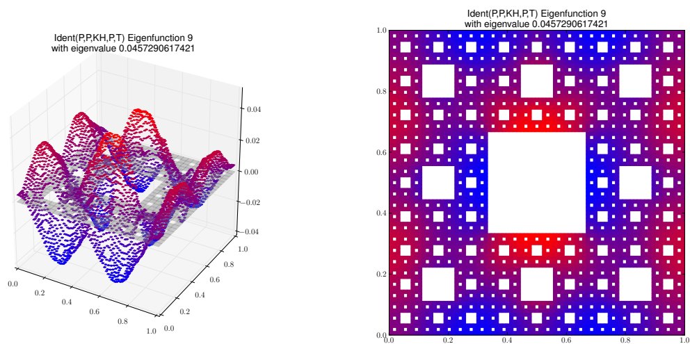
Eigenfunction 9 with eigenvalue 0.0457290617421
