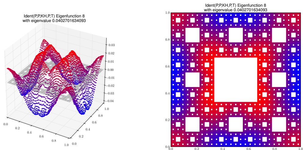
Eigenfunction 8 with eigenvalue 0.0402701634093
