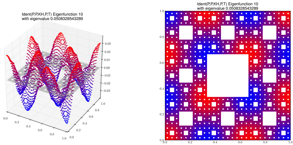
Eigenfunction 10 with eigenvalue 0.0508328543289
