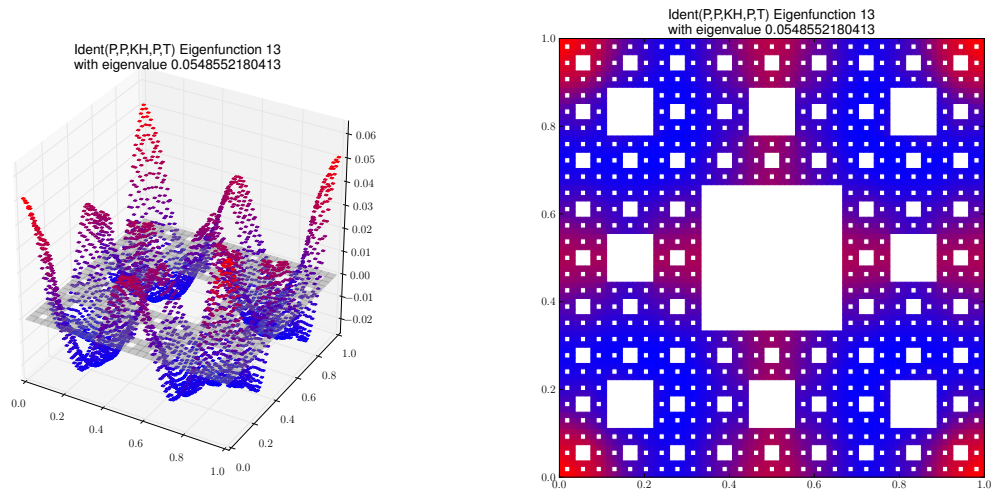
Eigenfunction 13 with eigenvalue 0.0548552180413
