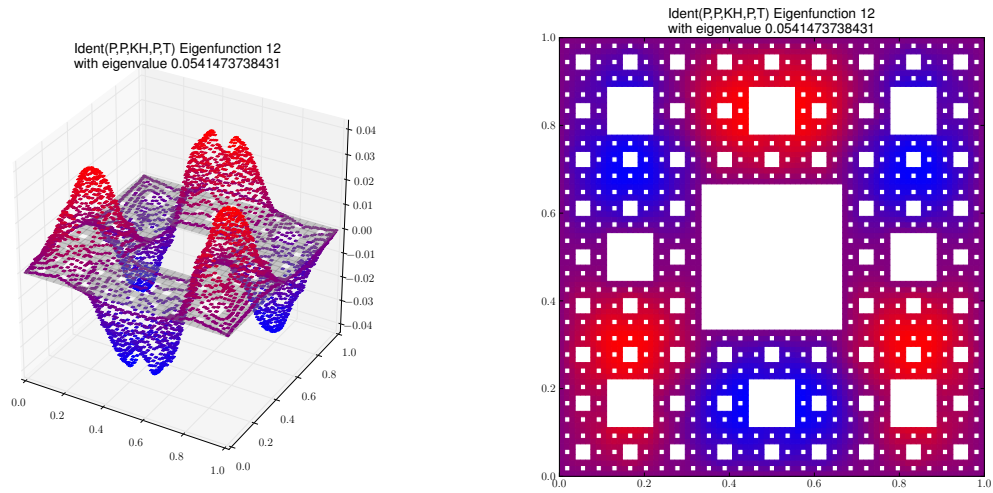
Eigenfunction 12 with eigenvalue 0.0541473738431
