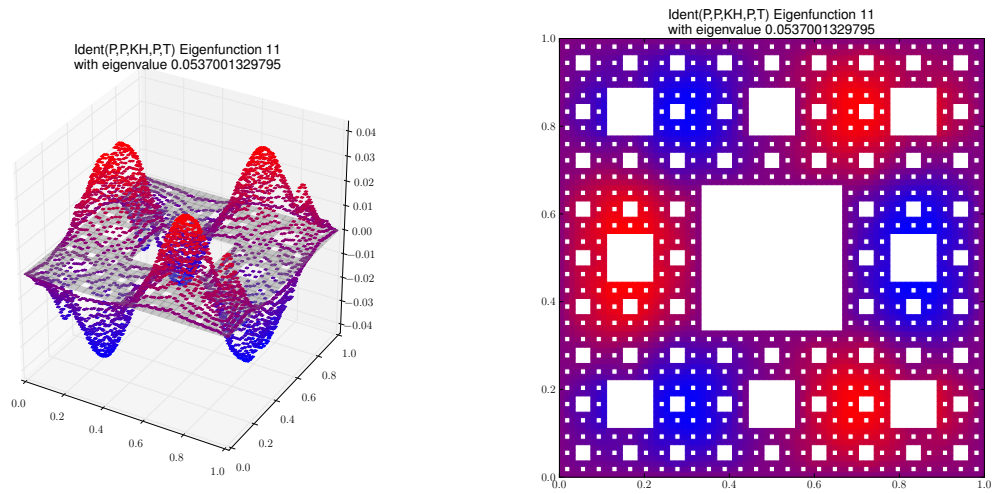
Eigenfunction 11 with eigenvalue 0.0537001329795
