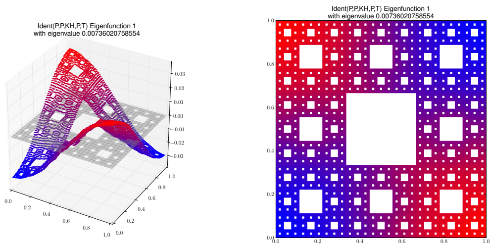
Eigenfunction 1 with eigenvalue 0.00736020758554
