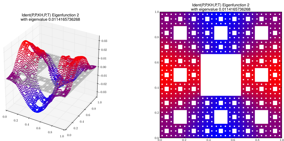
Eigenfunction 2 with eigenvalue 0.0114165736268
