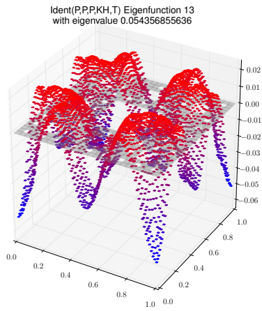
Eigenfunction 13 with eigenvalue 0.054356855636
