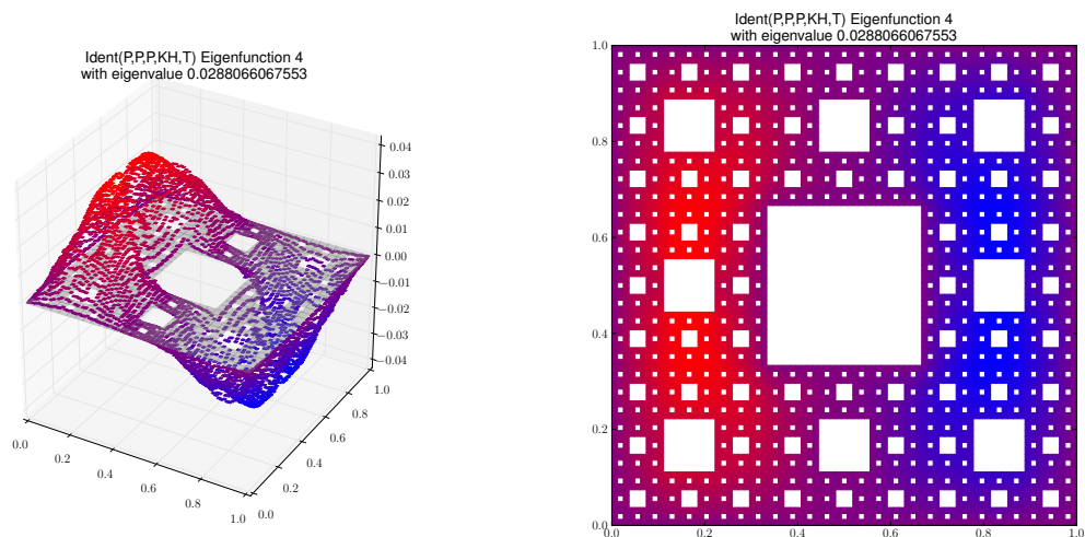
Eigenfunction 4 with eigenvalue 0.0288066067553
