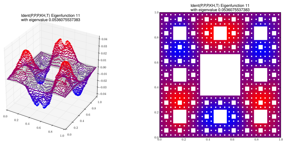
Eigenfunction 11 with eigenvalue 0.0536075537383
