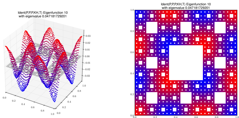
Eigenfunction 10 with eigenvalue 0.047181729201
