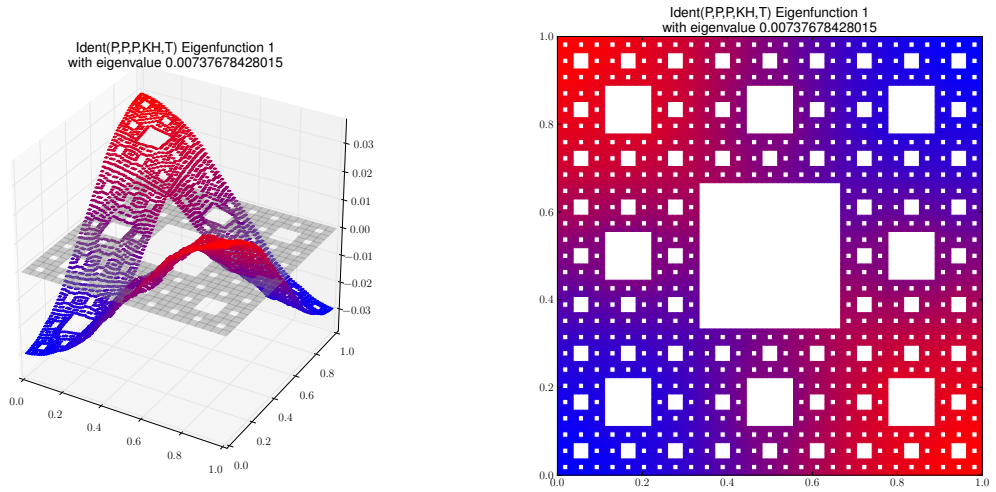
Eigenfunction 1 with eigenvalue 0.00737678428015
