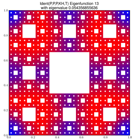
Eigenfunction 13 with eigenvalue 0.054356855636
