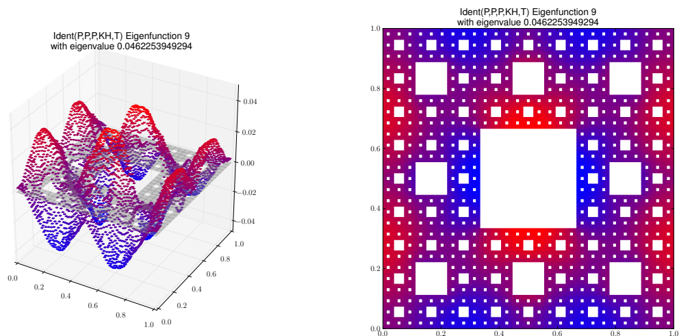
Eigenfunction 9 with eigenvalue 0.0462253949294
