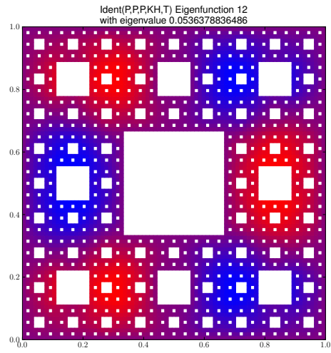
Eigenfunction 12 with eigenvalue 0.0536378836486
