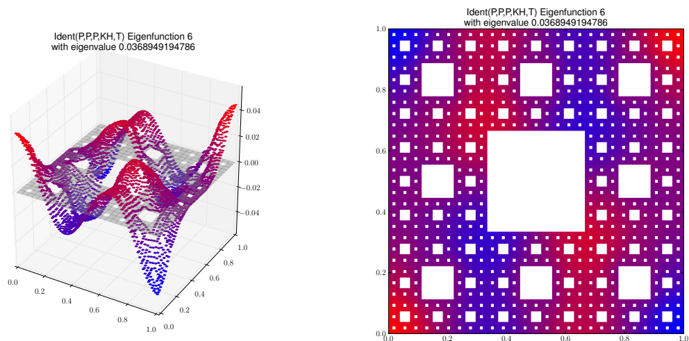
Eigenfunction 6 with eigenvalue 0.0368949194786
