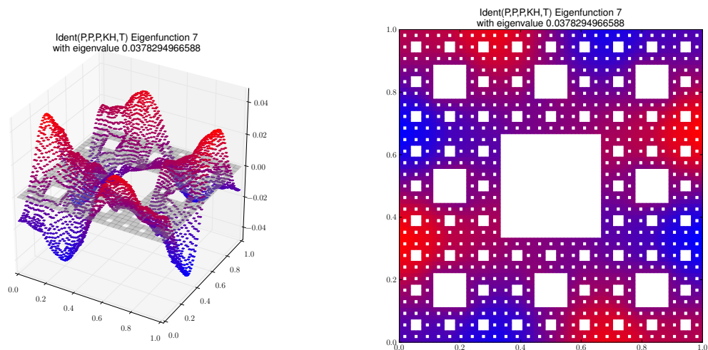
Eigenfunction 7 with eigenvalue 0.0378294966588
