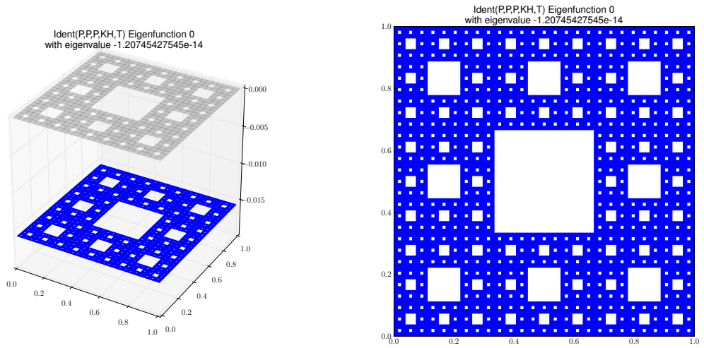
Eigenfunction 0 with eigenvalue -1.20745427545e-14
