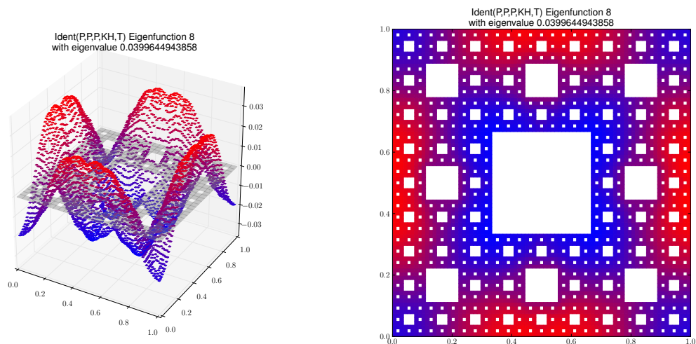
Eigenfunction 8 with eigenvalue 0.0399644943858
