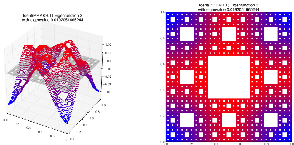
Eigenfunction 3 with eigenvalue 0.0192051665244
