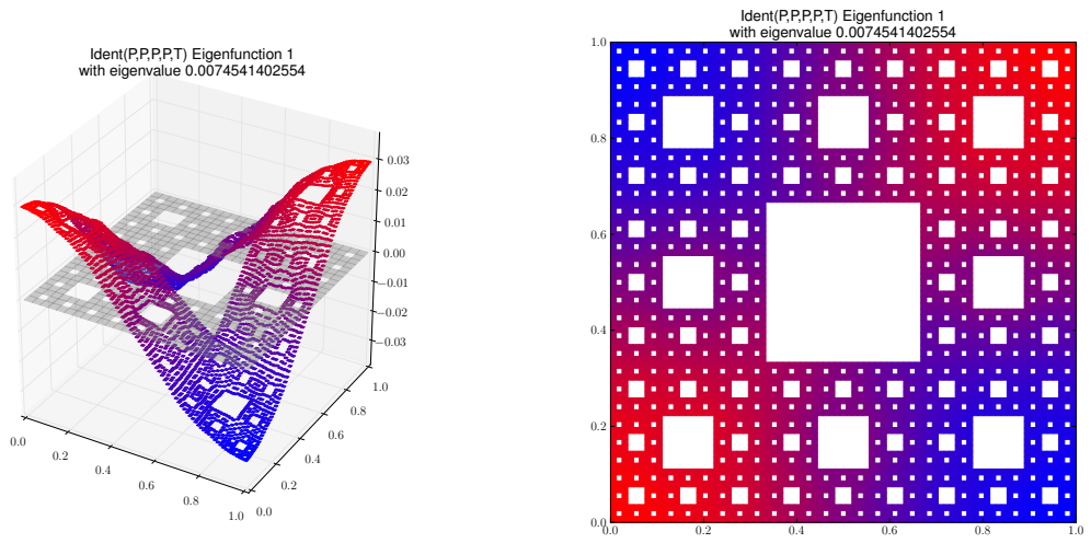
Eigenfunction 1 with eigenvalue 0.0074541402554
