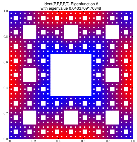
Eigenfunction 8 with eigenvalue 0.0403709170848
