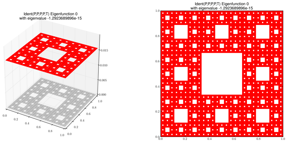
Eigenfunction 0 with eigenvalue -1.2923689896 \times 10^{-15}
