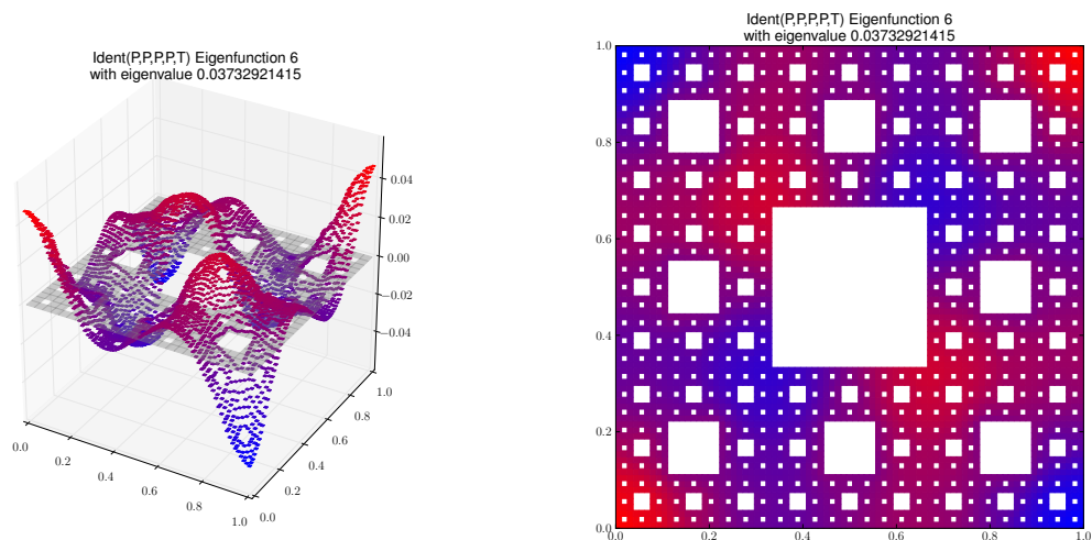
Eigenfunction 6 with eigenvalue 0.03732921415
