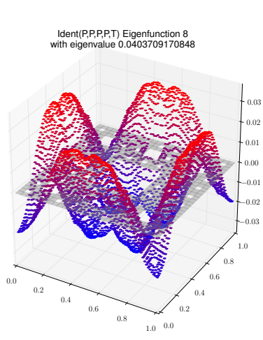
Eigenfunction 8 with eigenvalue 0.0403709170848
