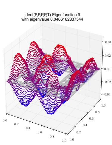
Eigenfunction 9 with eigenvalue 0.0466162837544
