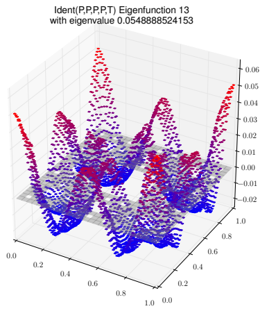
Eigenfunction 13 with eigenvalue 0.0548888524153
