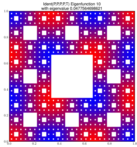
Eigenfunction 10 with eigenvalue 0.0477564698621
