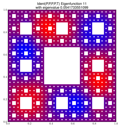
Eigenfunction 11 with eigenvalue 0.0541733551099
