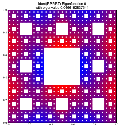
Eigenfunction 9 with eigenvalue 0.0466162837544
