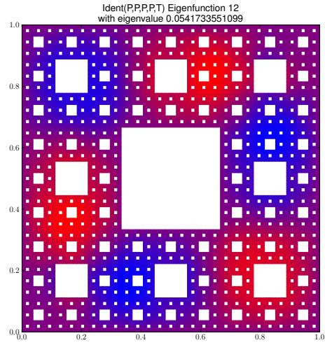
Eigenfunction 12 with eigenvalue 0.0541733551099
