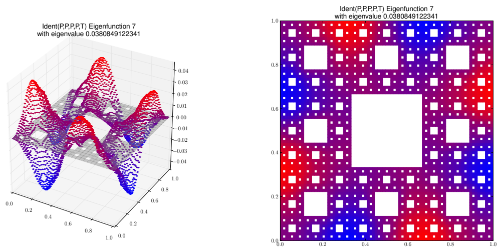
Eigenfunction 7 with eigenvalue 0.0380849122341
