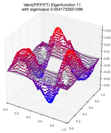
Eigenfunction 11 with eigenvalue 0.0541733551099
