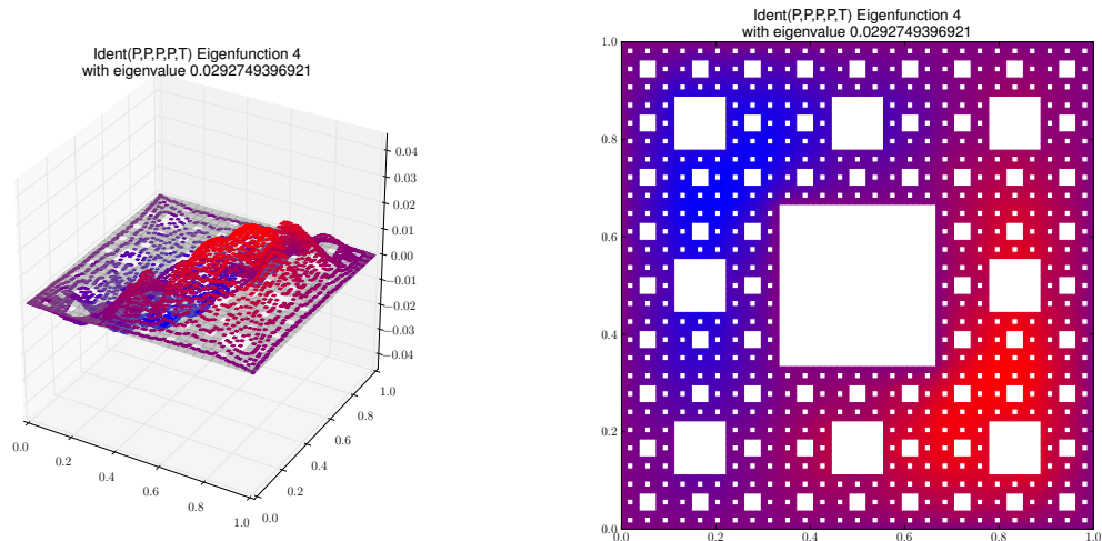
Eigenfunction 4 with eigenvalue 0.0292749396921
