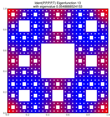
Eigenfunction 13 with eigenvalue 0.0548888524153
