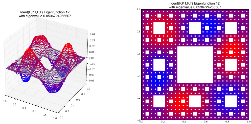
Eigenfunction 12 with eigenvalue 0.0536724255567
