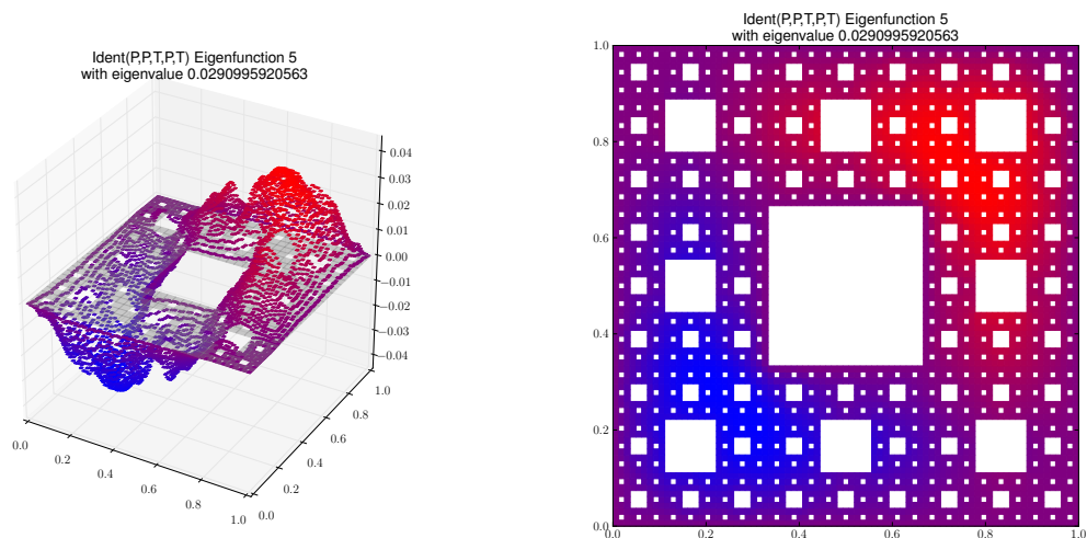
Eigenfunction 5 with eigenvalue 0.0290995920563
