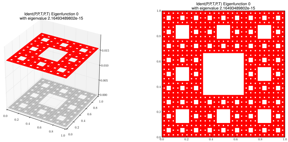
Eigenfunction 0 with eigenvalue 2.16493489802e-15
