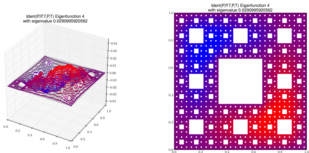
Eigenfunction 4 with eigenvalue 0.0290995920562
