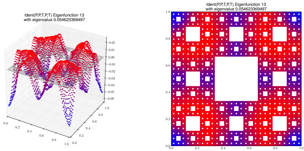
Eigenfunction 13 with eigenvalue 0.054623369497
