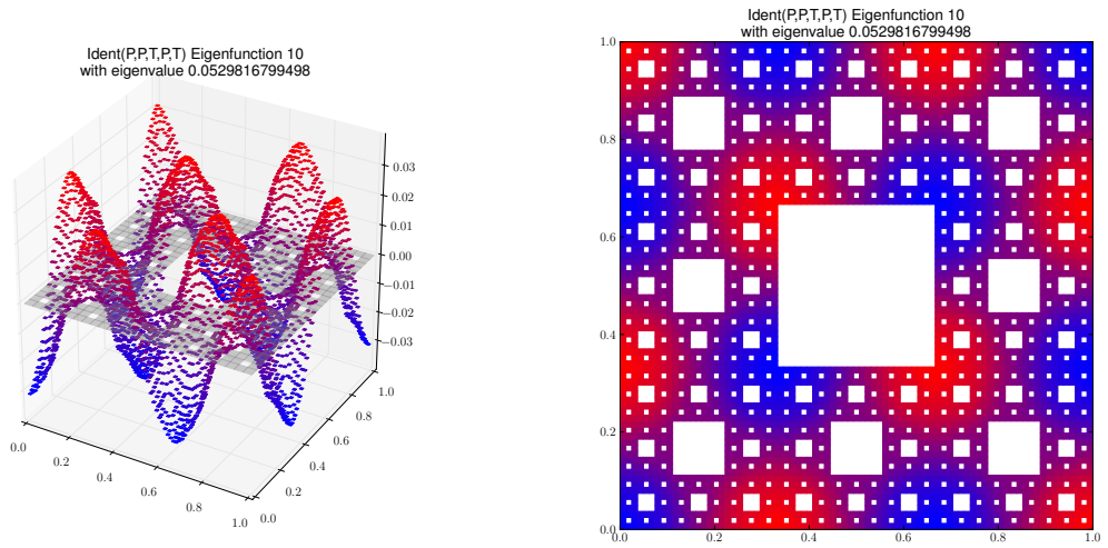
Eigenfunction 10 with eigenvalue 0.0529816799498
