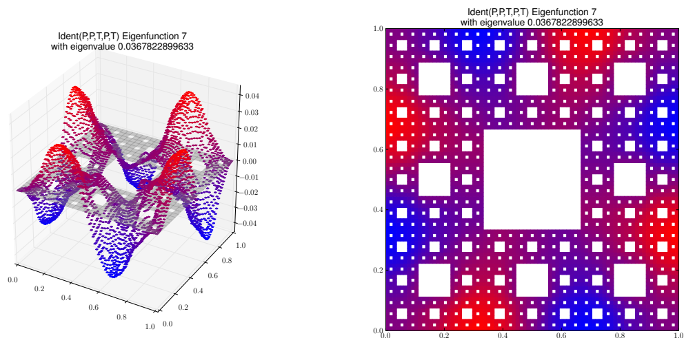
Eigenfunction 7 with eigenvalue 0.0367822899633
