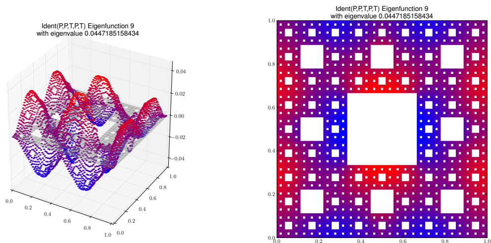
Eigenfunction 9 with eigenvalue 0.0447185158434
