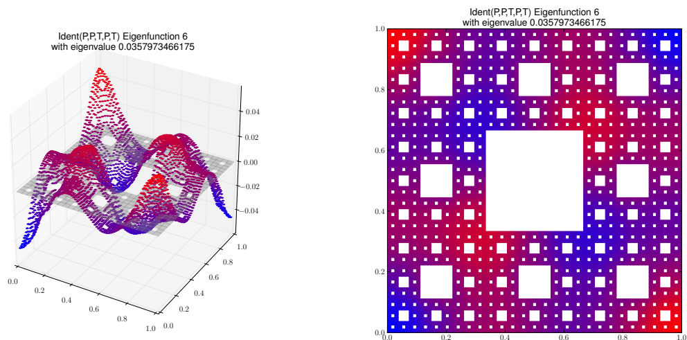
Eigenfunction 6 with eigenvalue 0.0357973466175
