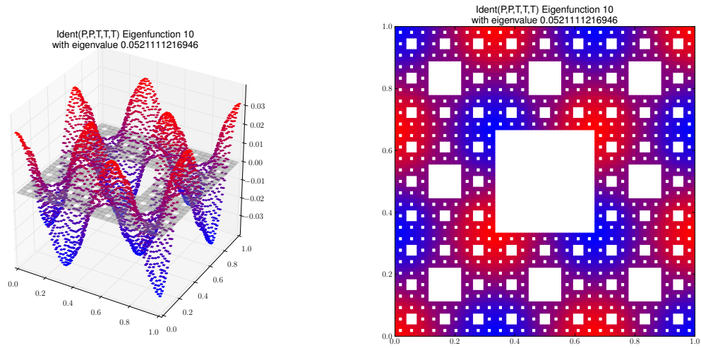
Eigenfunction 10 with eigenvalue 0.0521111216946
