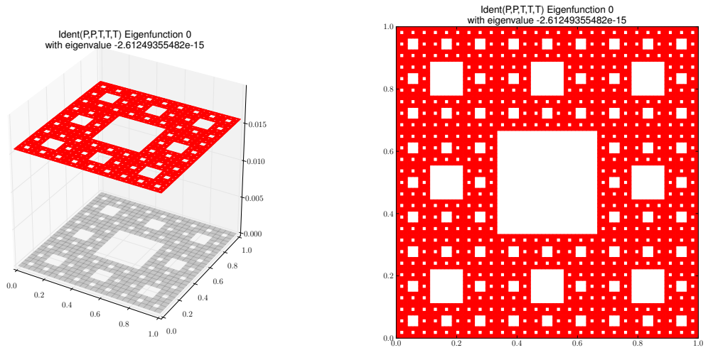
Eigenfunction 0 with eigenvalue -2.61249355482e-15
