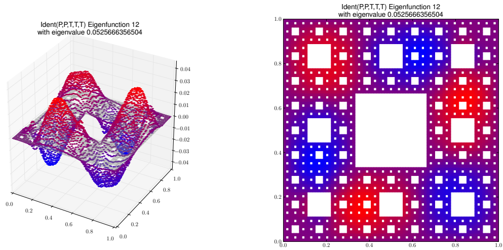
Eigenfunction 12 with eigenvalue 0.0525666356504
