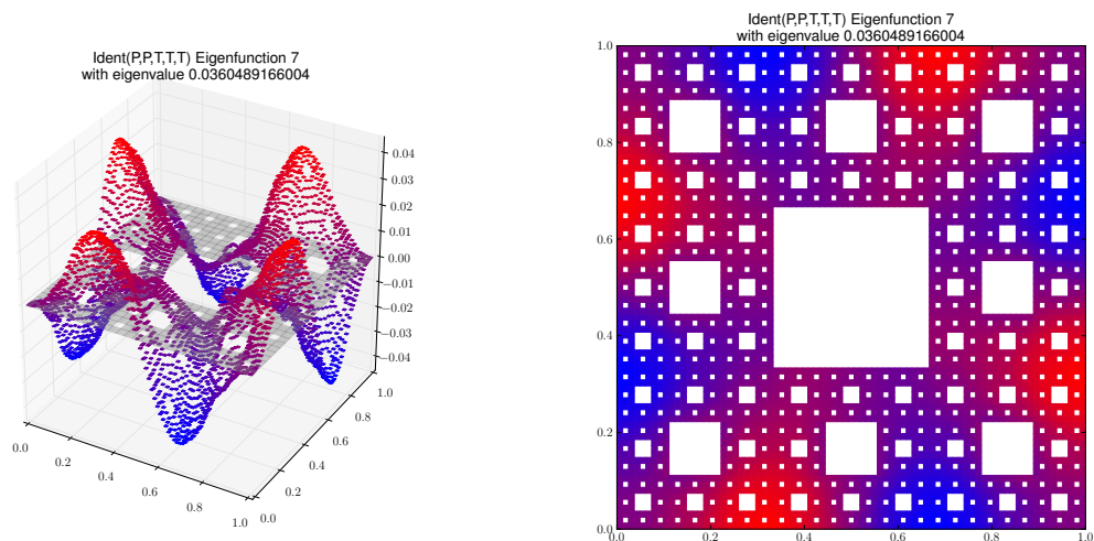
Eigenfunction 7 with eigenvalue 0.0360489166004
