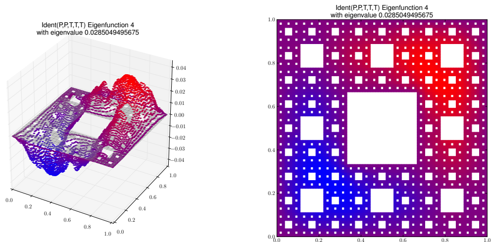
Eigenfunction 4 with eigenvalue 0.0285049495675
