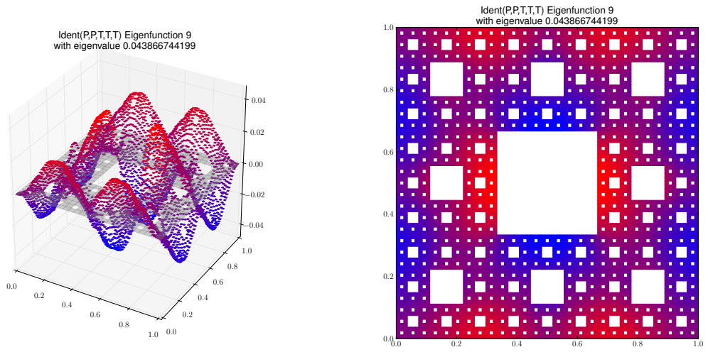
Eigenfunction 9 with eigenvalue 0.043866744199
