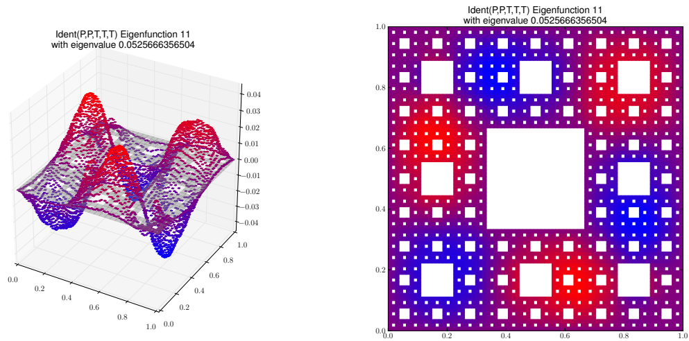
Eigenfunction 11 with eigenvalue 0.0525666356504
