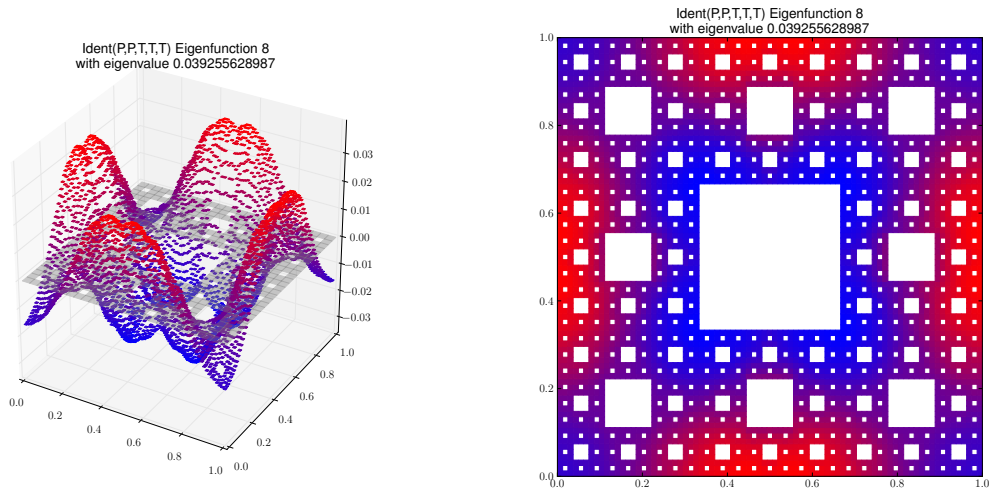
Eigenfunction 8 with eigenvalue 0.039255628987
