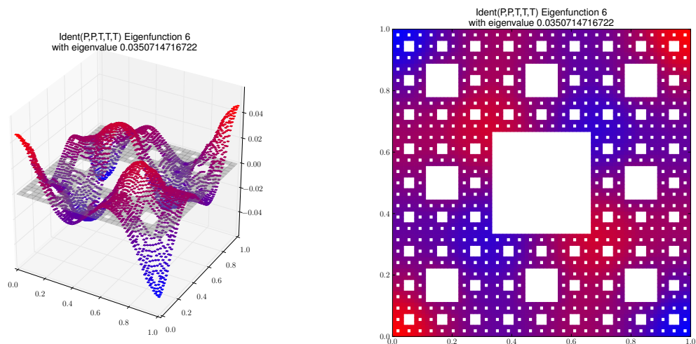
Eigenfunction 6 with eigenvalue 0.0350714716722
