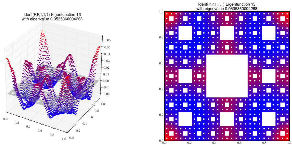
Eigenfunction 13 with eigenvalue 0.0535360004268
