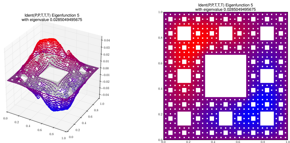
Eigenfunction 5 with eigenvalue 0.0285049495675
