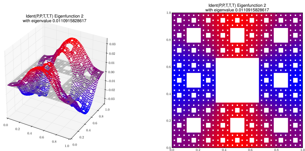
Eigenfunction 2 with eigenvalue 0.0110915828617
