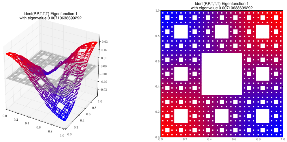
Eigenfunction 1 with eigenvalue 0.00710638699292
