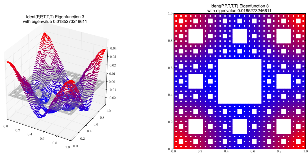
Eigenfunction 3 with eigenvalue 0.0185273246611
