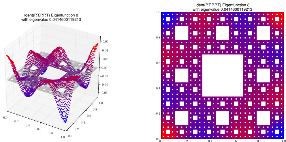
Eigenfunction 8 with eigenvalue 0.0414600119213
