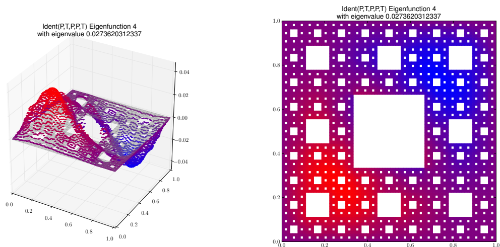
Eigenfunction 4 with eigenvalue 0.0273620312337
