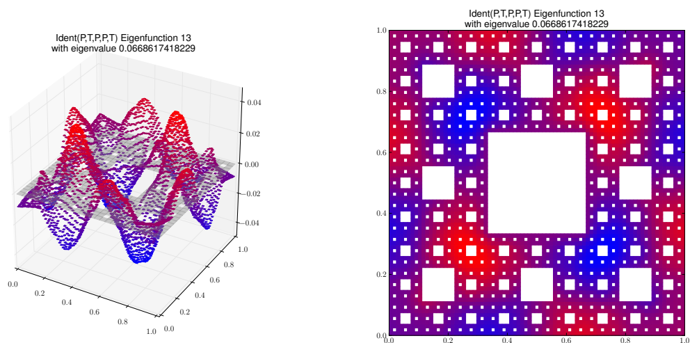
Eigenfunction 13 with eigenvalue 0.0668617418229
