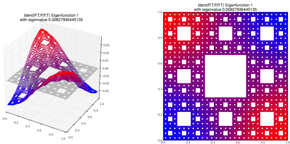
Eigenfunction 1 with eigenvalue 0.00827936445135
