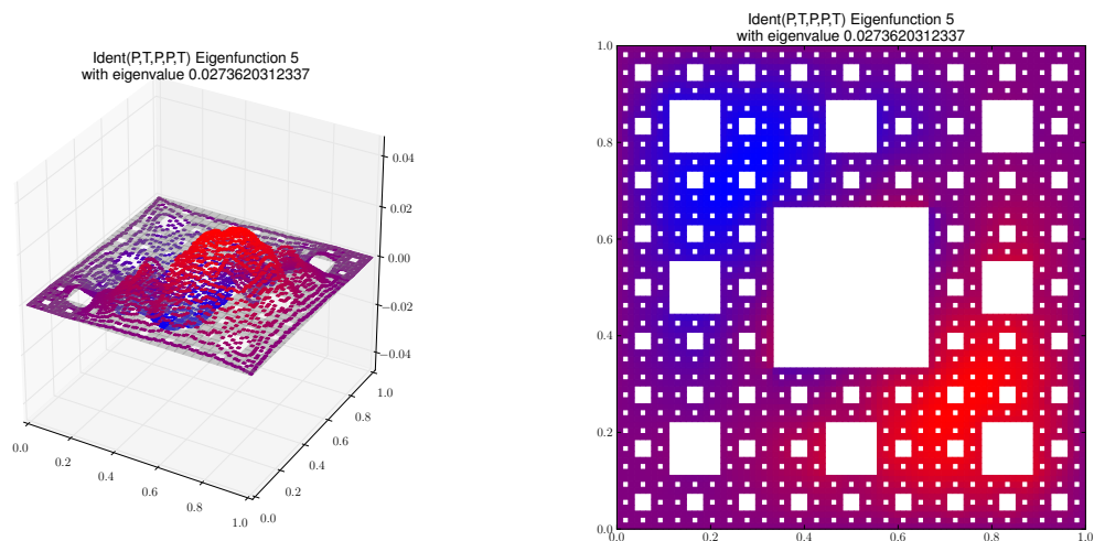
Eigenfunction 5 with eigenvalue 0.0273620312337
