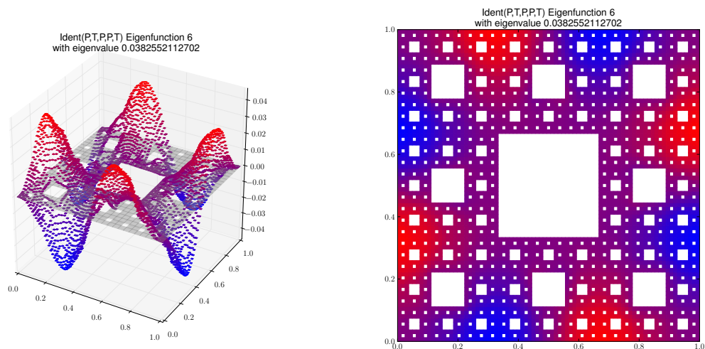
Eigenfunction 6 with eigenvalue 0.0382552112702
