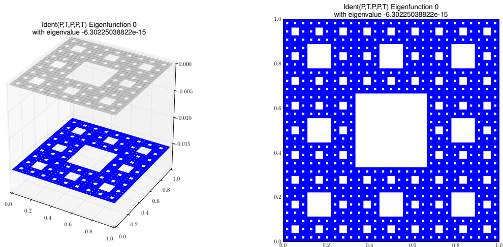
Eigenfunction 0 with eigenvalue -6.30225038822e-15
