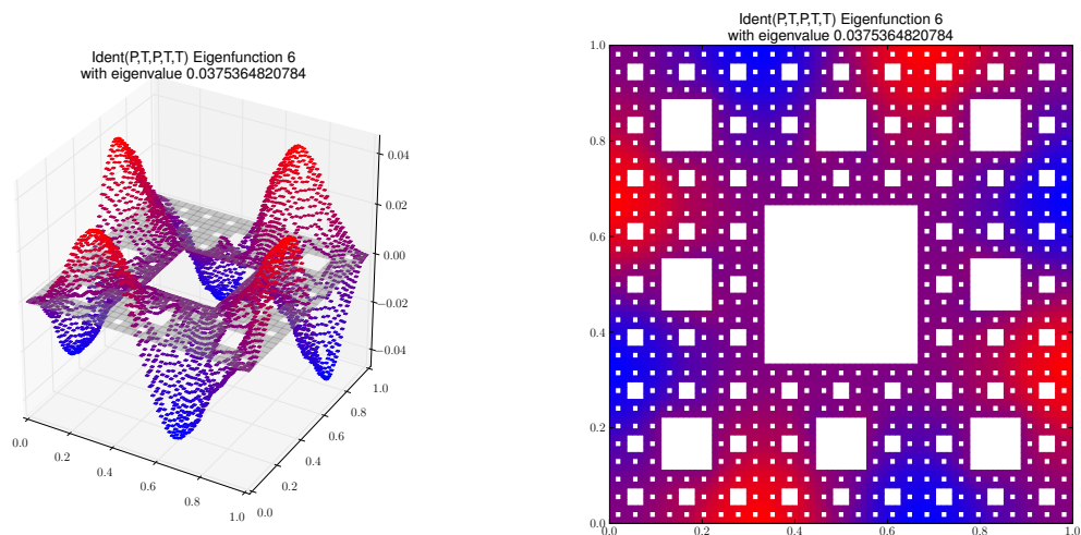
Eigenfunction 6 with eigenvalue 0.0375364820784
