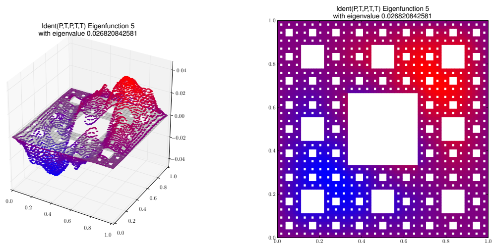
Eigenfunction 5 with eigenvalue 0.026820842581
