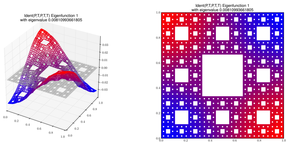
Eigenfunction 1 with eigenvalue 0.00810993661805
