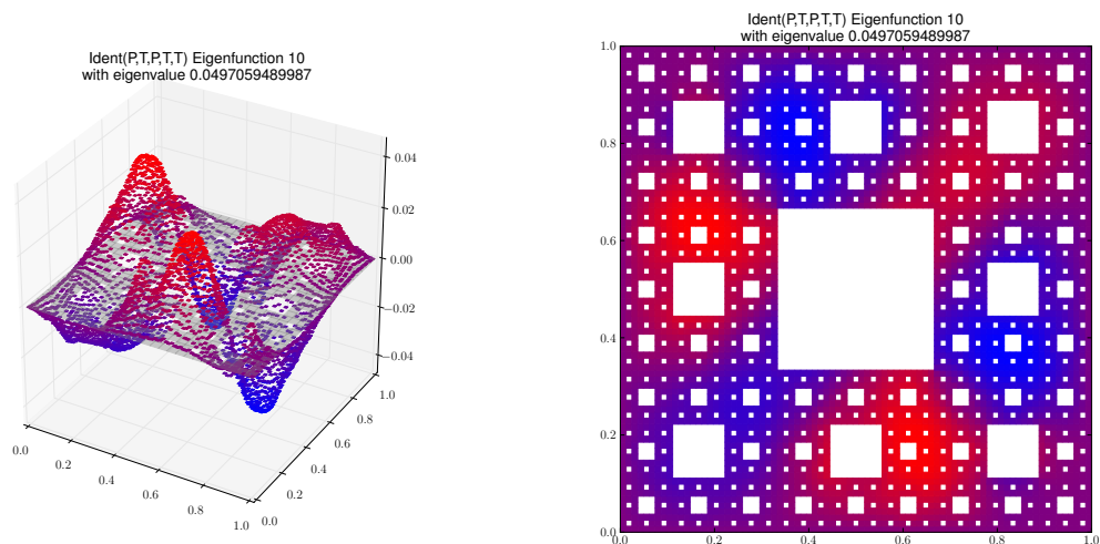
Eigenfunction 10 with eigenvalue 0.0497059489987
