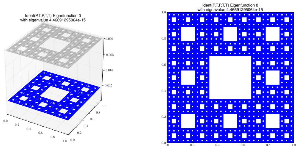
Eigenfunction 0 with eigenvalue 4.46691295064e-15
