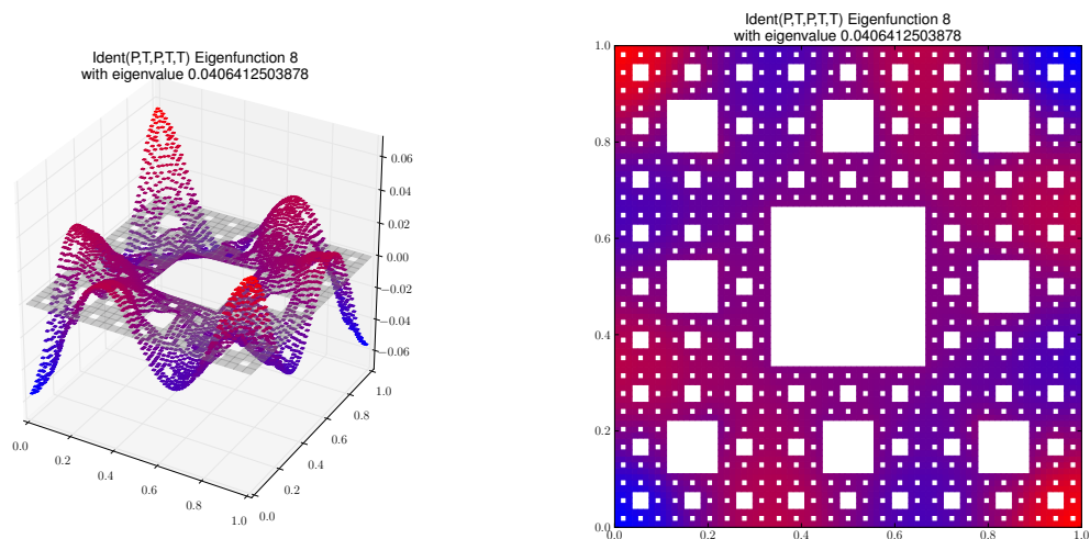
Eigenfunction 8 with eigenvalue 0.0406412503878
