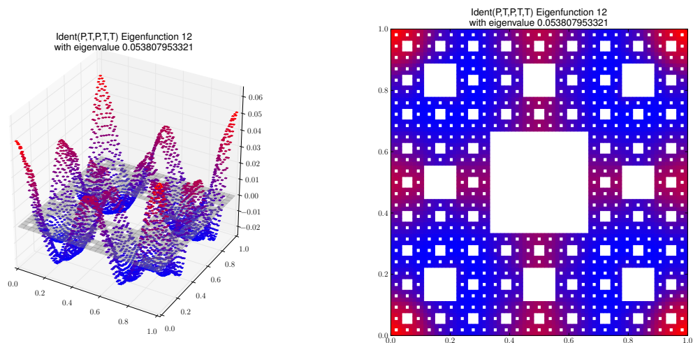
Eigenfunction 12 with eigenvalue 0.053807953321
