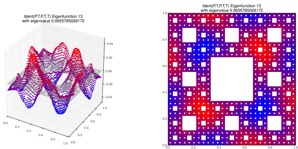
Eigenfunction 13 with eigenvalue 0.0655785028172
