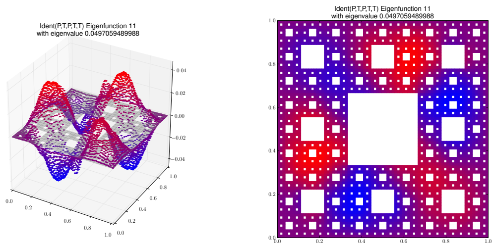
Eigenfunction 11 with eigenvalue 0.0497059489988
