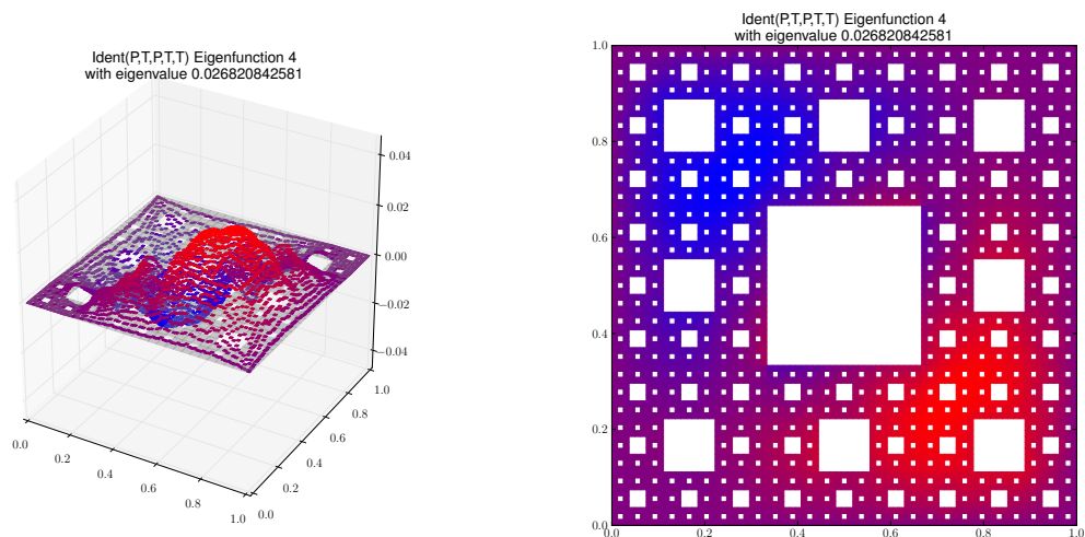
Eigenfunction 4 with eigenvalue 0.026820842581
