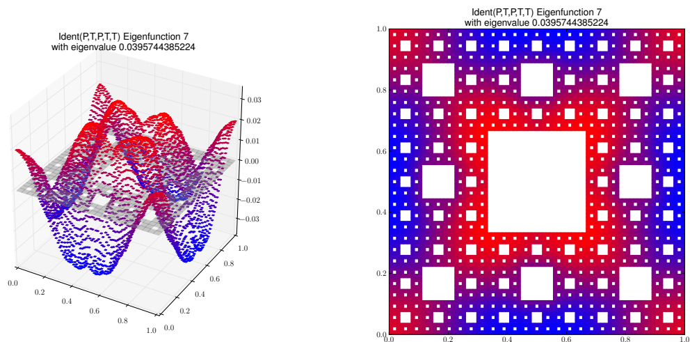
Eigenfunction 7 with eigenvalue 0.0395744385224
