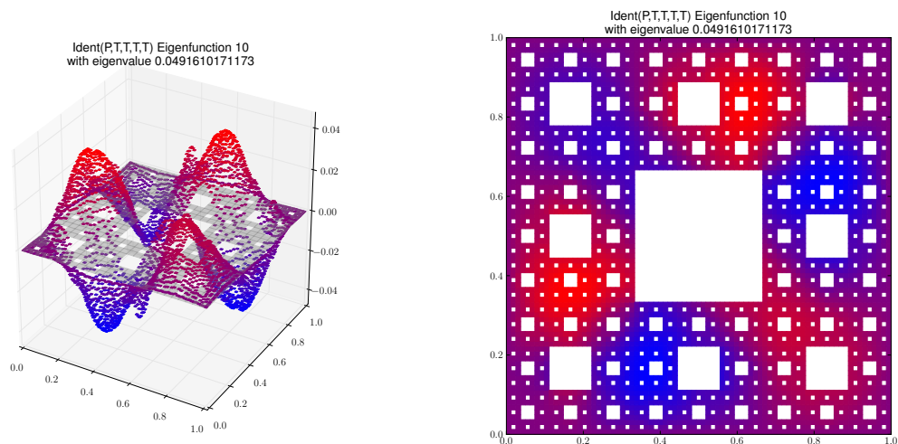
Eigenfunction 10 with eigenvalue 0.0491610171173
