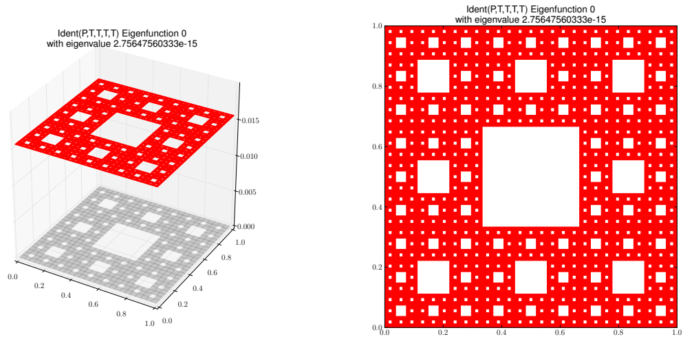
Eigenfunction 0 with eigenvalue 2.75647560333e-15
