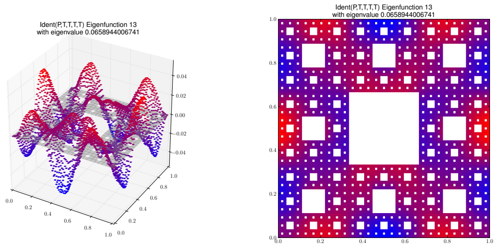
Eigenfunction 13 with eigenvalue 0.0658944006741
