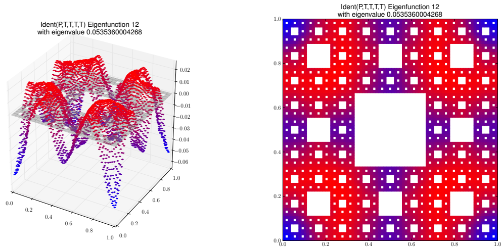
Eigenfunction 12 with eigenvalue 0.0535360004268
