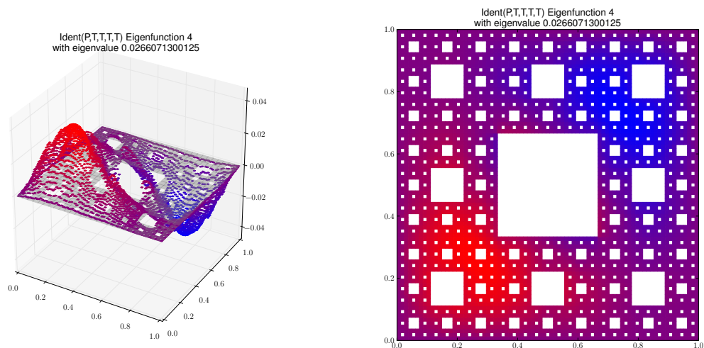
Eigenfunction 4 with eigenvalue 0.0266071300125
