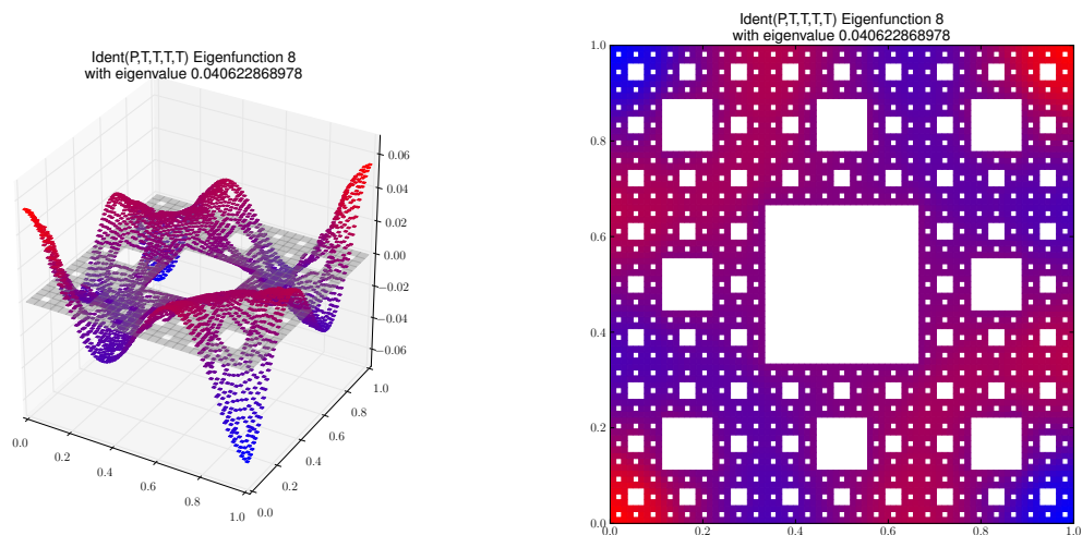
Eigenfunction 8 with eigenvalue 0.040622868978
