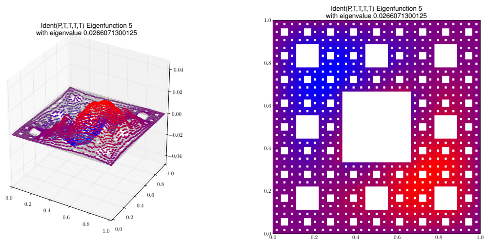
Eigenfunction 5 with eigenvalue 0.0266071300125
