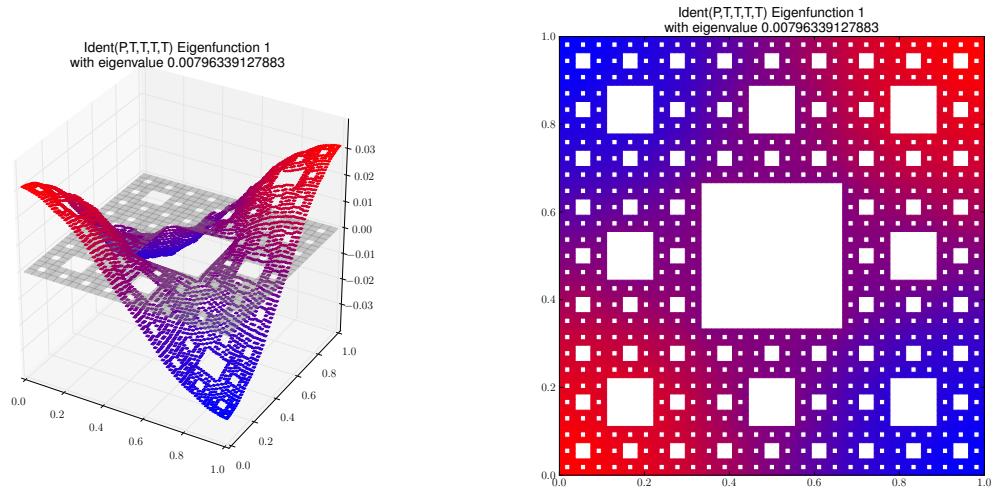
Eigenfunction 1 with eigenvalue 0.00796339127883
