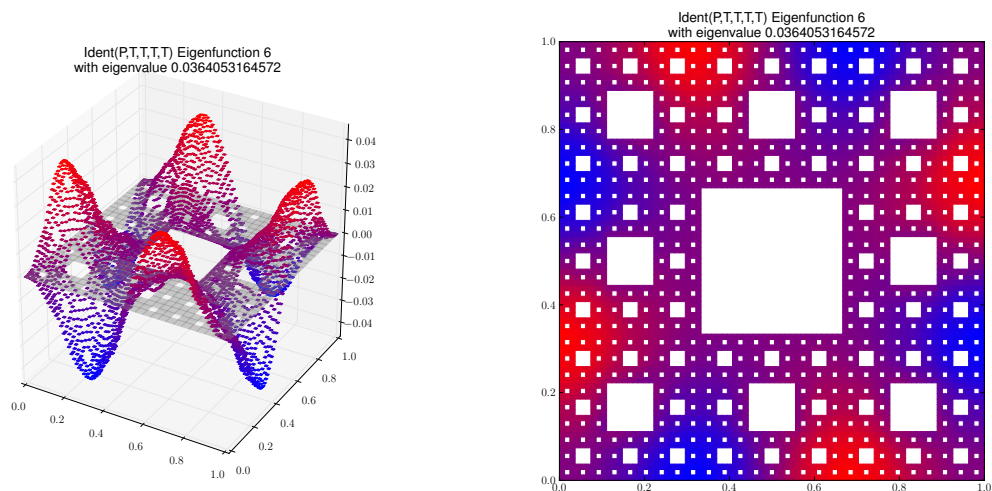
Eigenfunction 6 with eigenvalue 0.0364053164572
