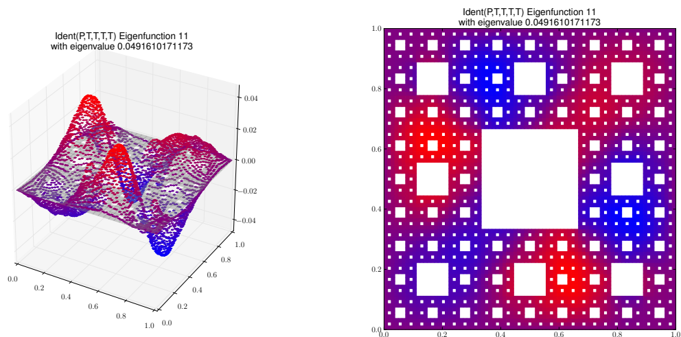
Eigenfunction 11 with eigenvalue 0.0491610171173
