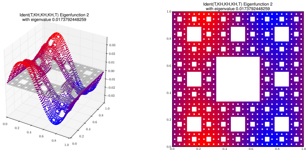
Eigenfunction 2 with eigenvalue 0.0173792448259
