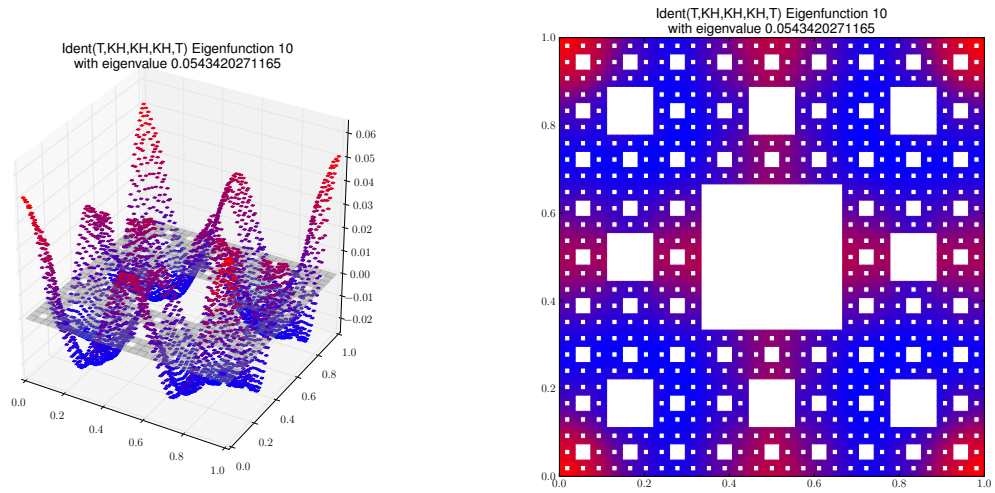
Eigenfunction 10 with eigenvalue 0.0543420271165
