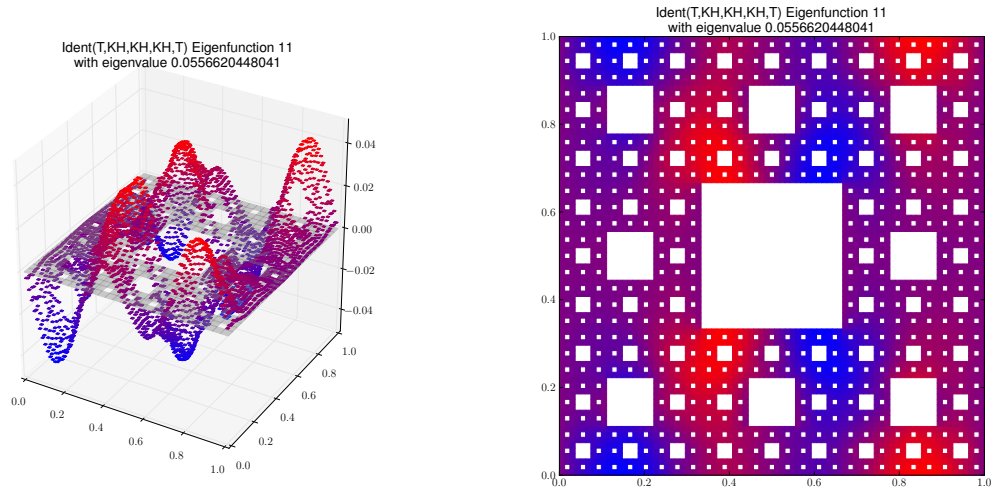
Eigenfunction 11 with eigenvalue 0.0556620448041
