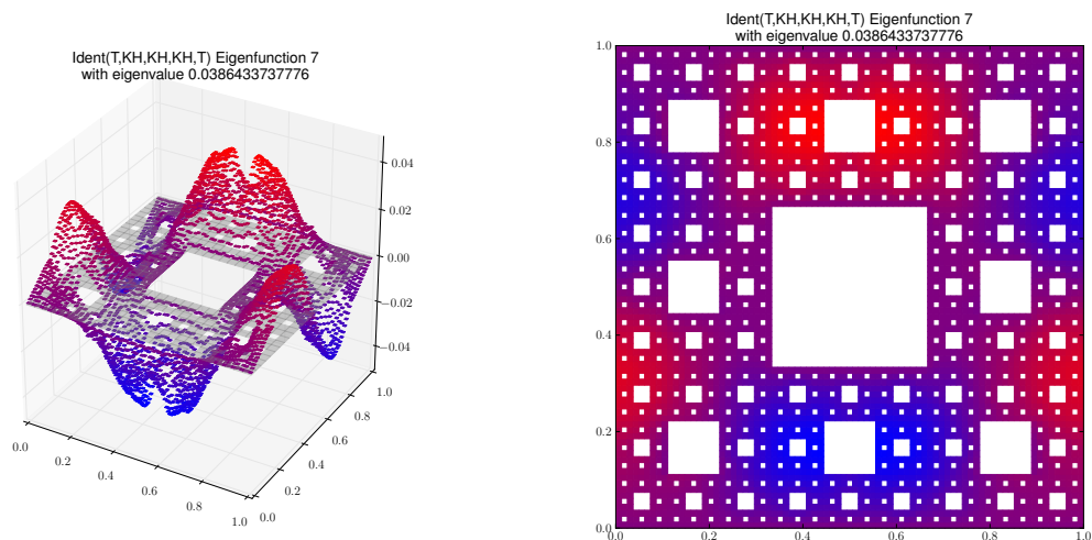
Eigenfunction 7 with eigenvalue 0.0386433737776
