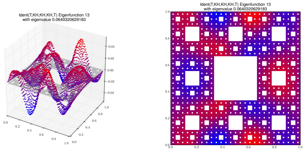
Eigenfunction 13 with eigenvalue 0.0640320629183
