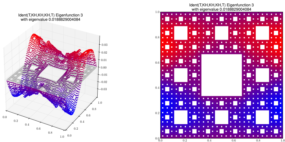
Eigenfunction 3 with eigenvalue 0.0188829004084
