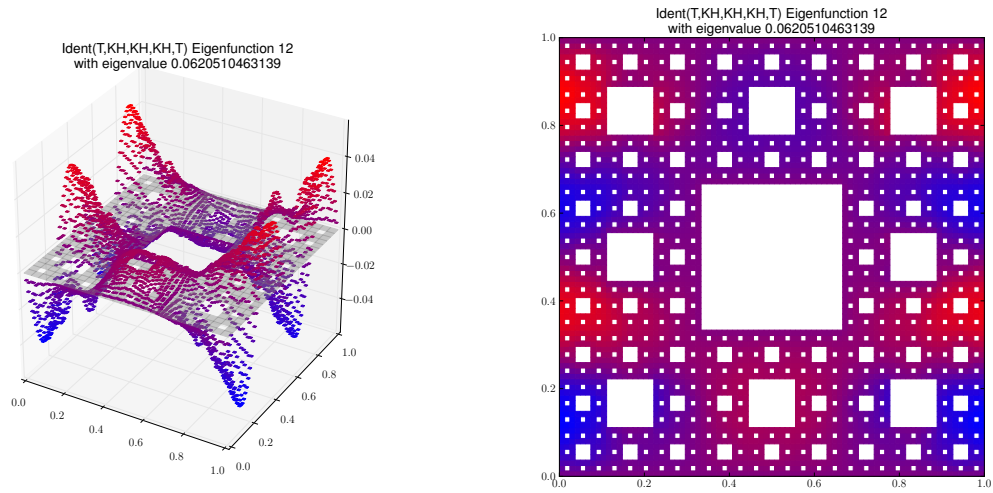
Eigenfunction 12 with eigenvalue 0.0620510463139
