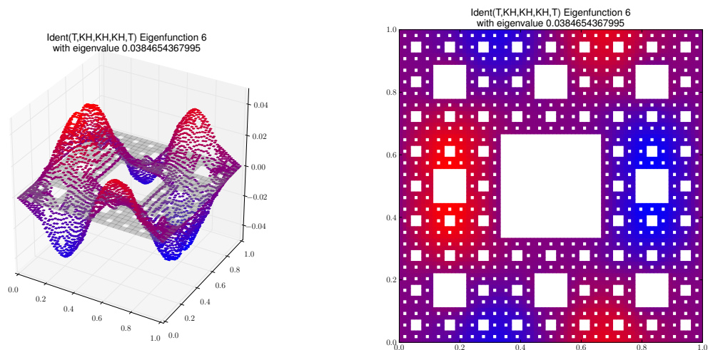
Eigenfunction 6 with eigenvalue 0.0384654367995
