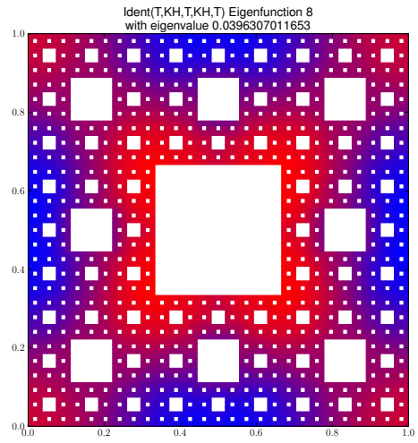
Eigenfunction 8 with eigenvalue 0.0396307011653
