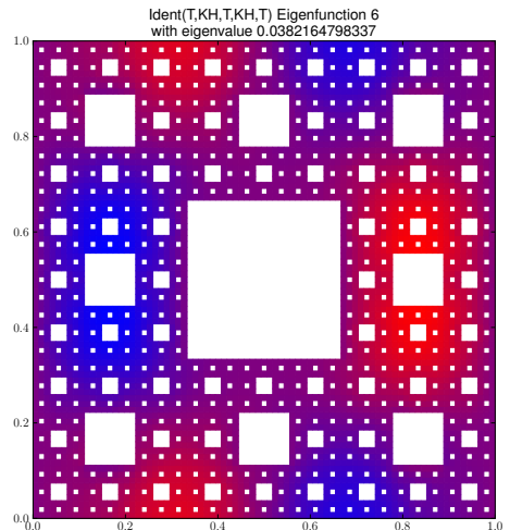
Eigenfunction 6 with eigenvalue 0.0382164798337
