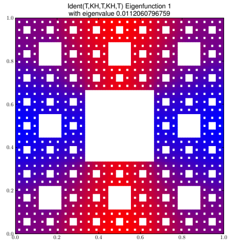
Eigenfunction 1 with eigenvalue 0.0112060796759
