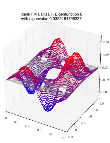
Eigenfunction 6 with eigenvalue 0.0382164798337
