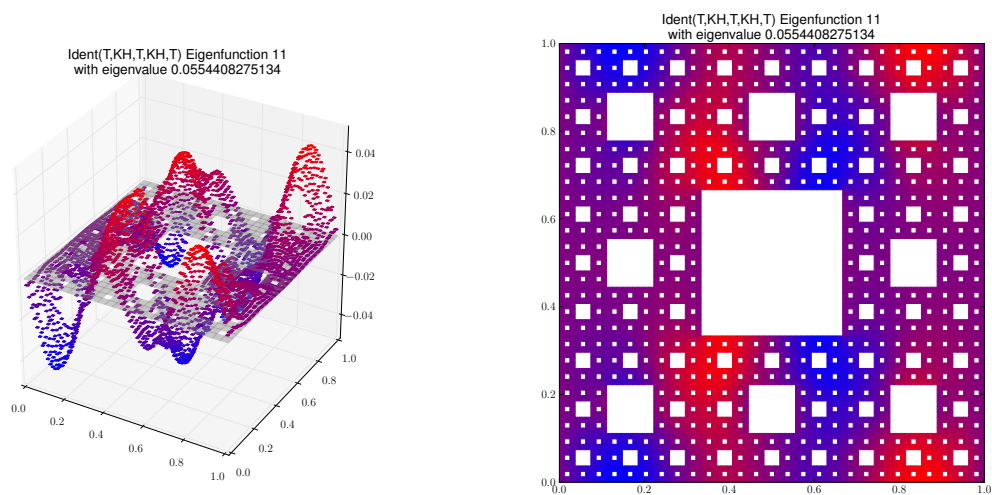
Eigenfunction 11 with eigenvalue 0.0554408275134
