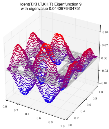
Eigenfunction 9 with eigenvalue 0.0442976404751
