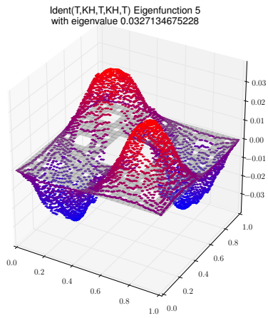
Eigenfunction 5 with eigenvalue 0.0327134675228
