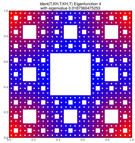
Eigenfunction 4 with eigenvalue 0.0187360475253
