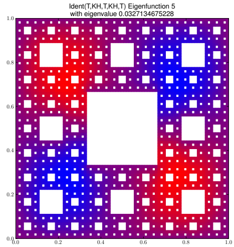
Eigenfunction 5 with eigenvalue 0.0327134675228
