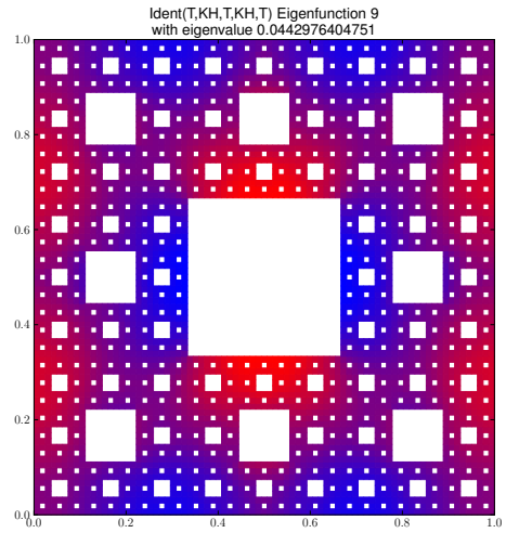
Eigenfunction 9 with eigenvalue 0.0442976404751
