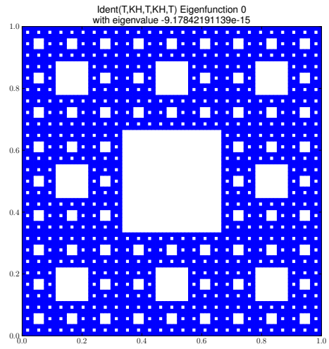
Eigenfunction 0 with eigenvalue -9.17842191139e-15
