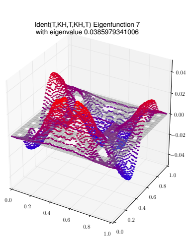
Eigenfunction 7 with eigenvalue 0.0385979341006
