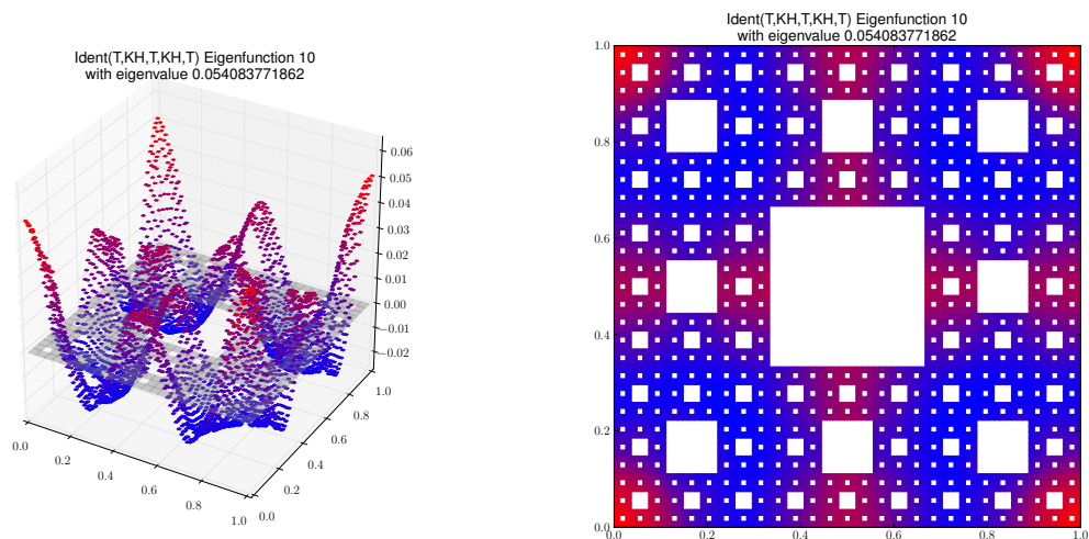
Eigenfunction 10 with eigenvalue 0.054083771862
