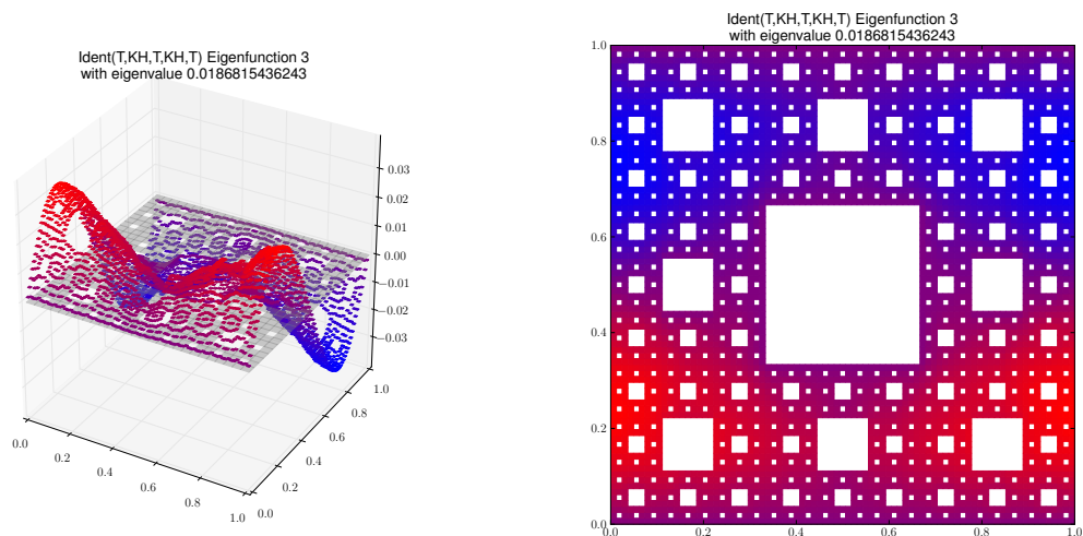
Eigenfunction 3 with eigenvalue 0.0186815436243
