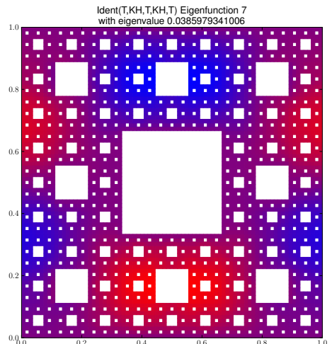
Eigenfunction 7 with eigenvalue 0.0385979341006
