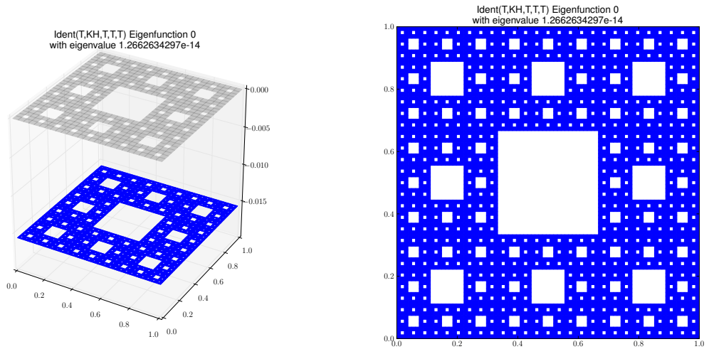
Eigenfunction 0 with eigenvalue 1.2662634297e-14
