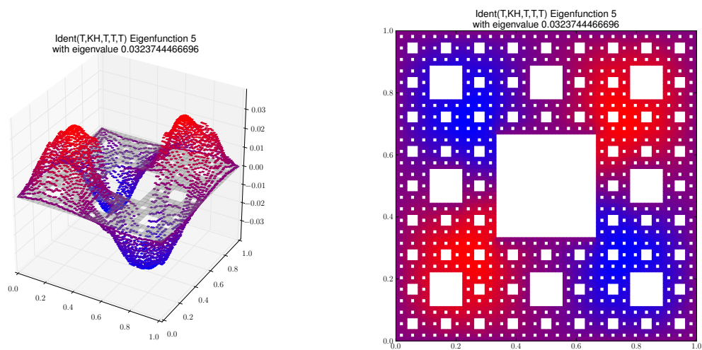
Eigenfunction 5 with eigenvalue 0.0323744466696
