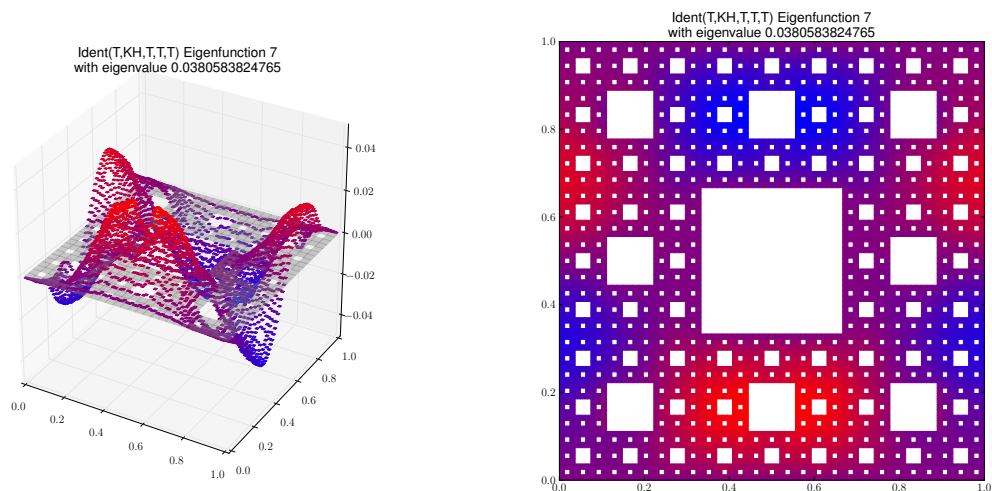
Eigenfunction 7 with eigenvalue 0.0380583824765
